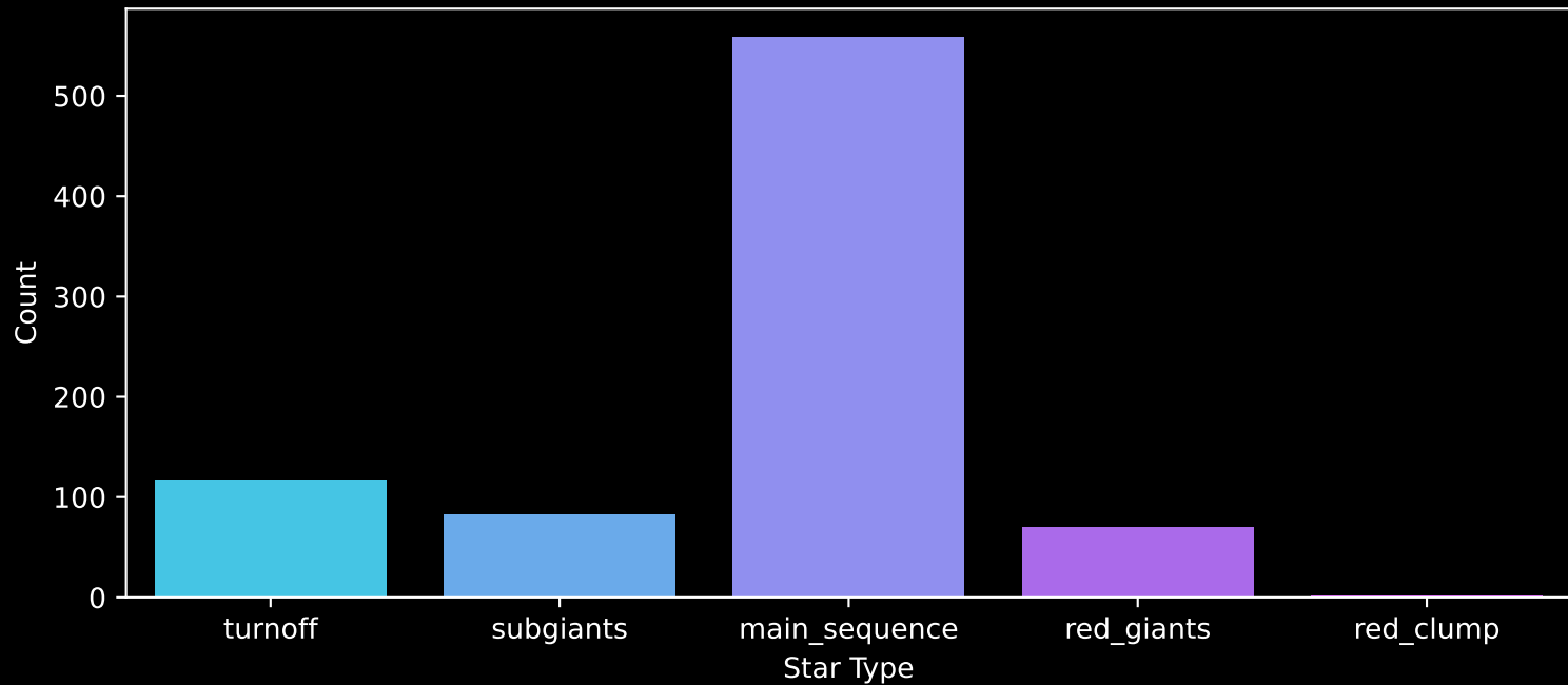
Gaia Cluster: [COIN-Gaia_29] Count plot of Star Type
