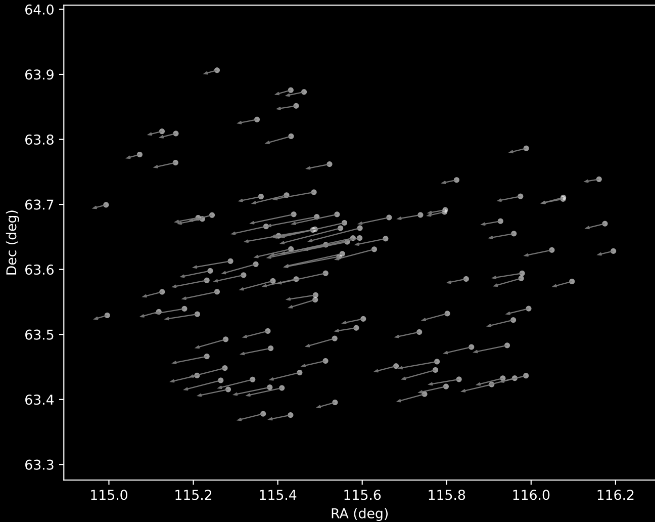
Gaia DR3 Cluster 34 Proper Motion Vectors (n=107)
