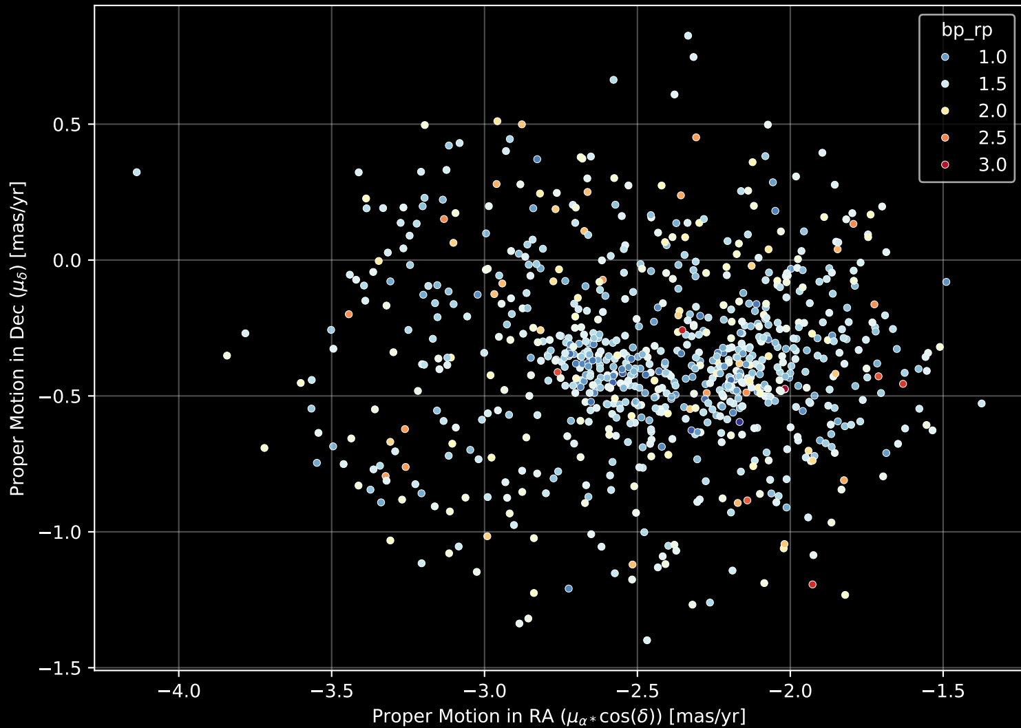
Gaia Cluster: [COIN-Gaia_29] Proper Motion Diagram (n= 830)
