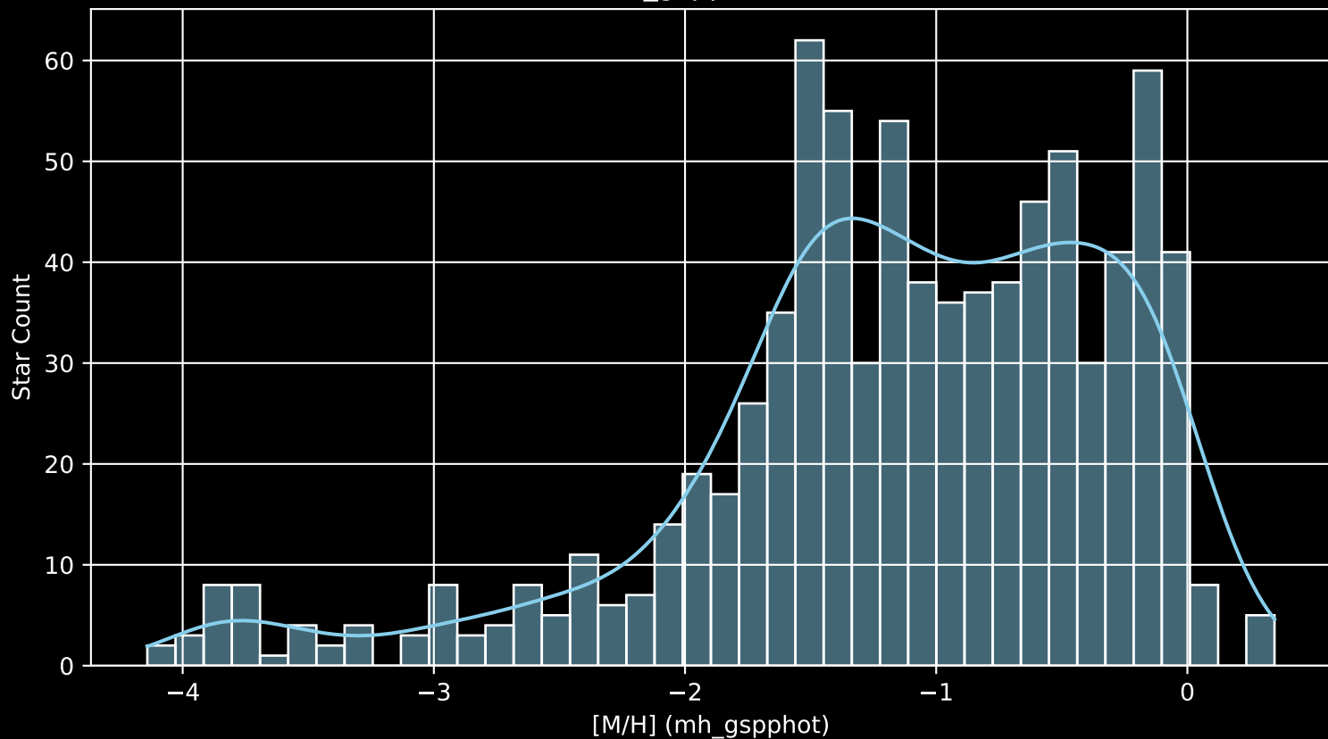
Gaia Cluster: [COIN-Gaia_29 [M/H] (mh_gspphot) (n= 829)
