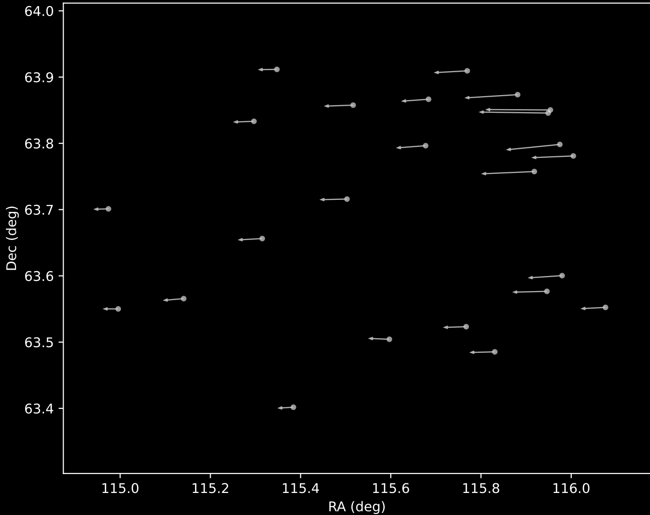
Gaia DR3 Cluster 15 Proper Motion Vectors (n=24)
