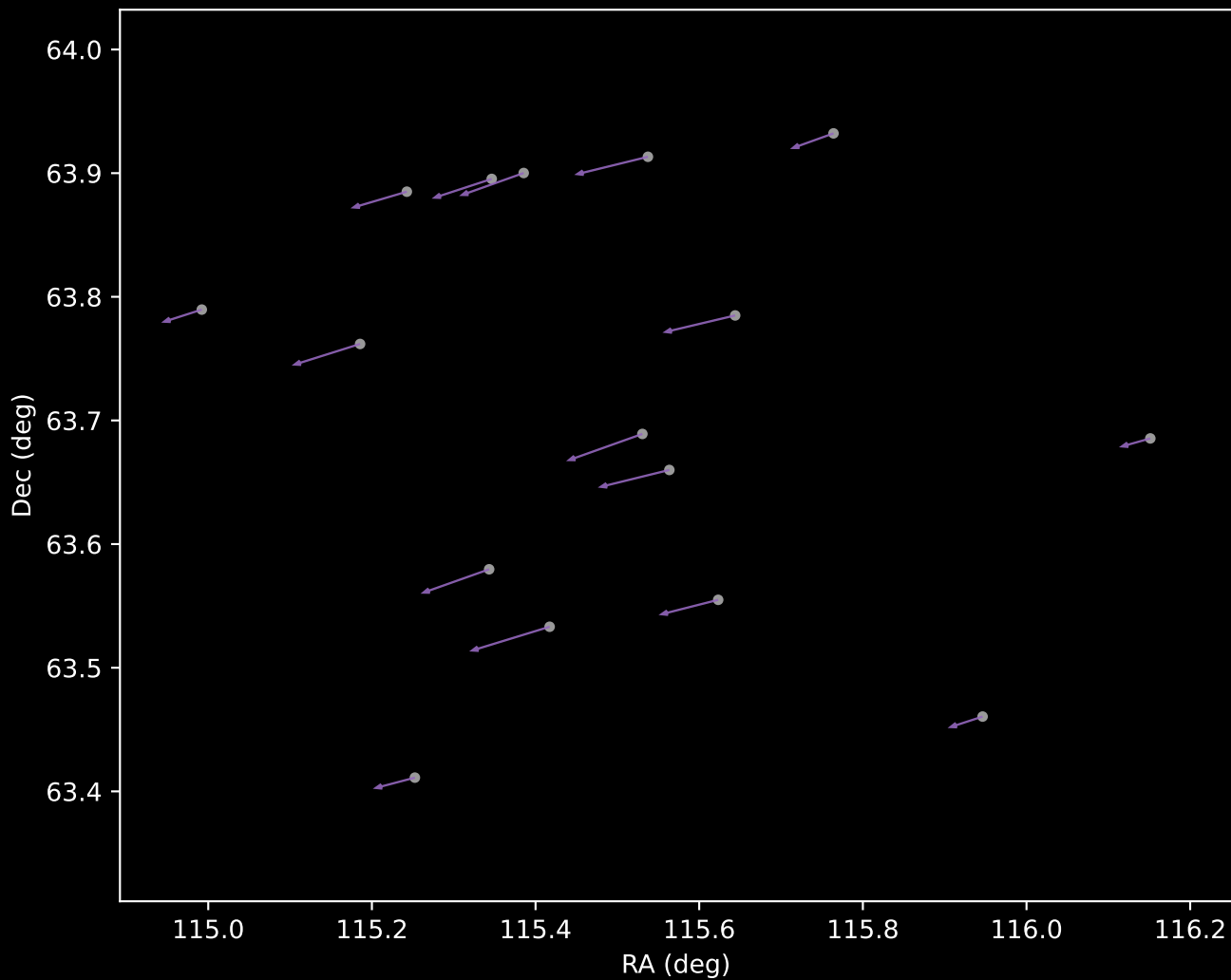
Gaia DR3 Cluster 28 Proper Motion Vectors (n=16)
