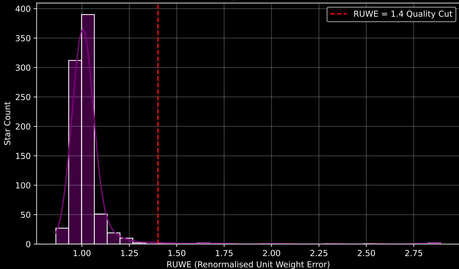
Gaia Cluster: [COIN-Gaia_29] RUWE Distribution (n= 829)
