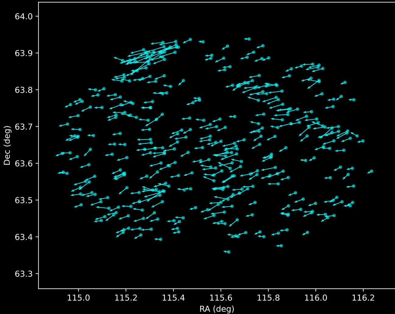
Gaia DR3 Noise Stream Proper Motion Vectors (n=346)
