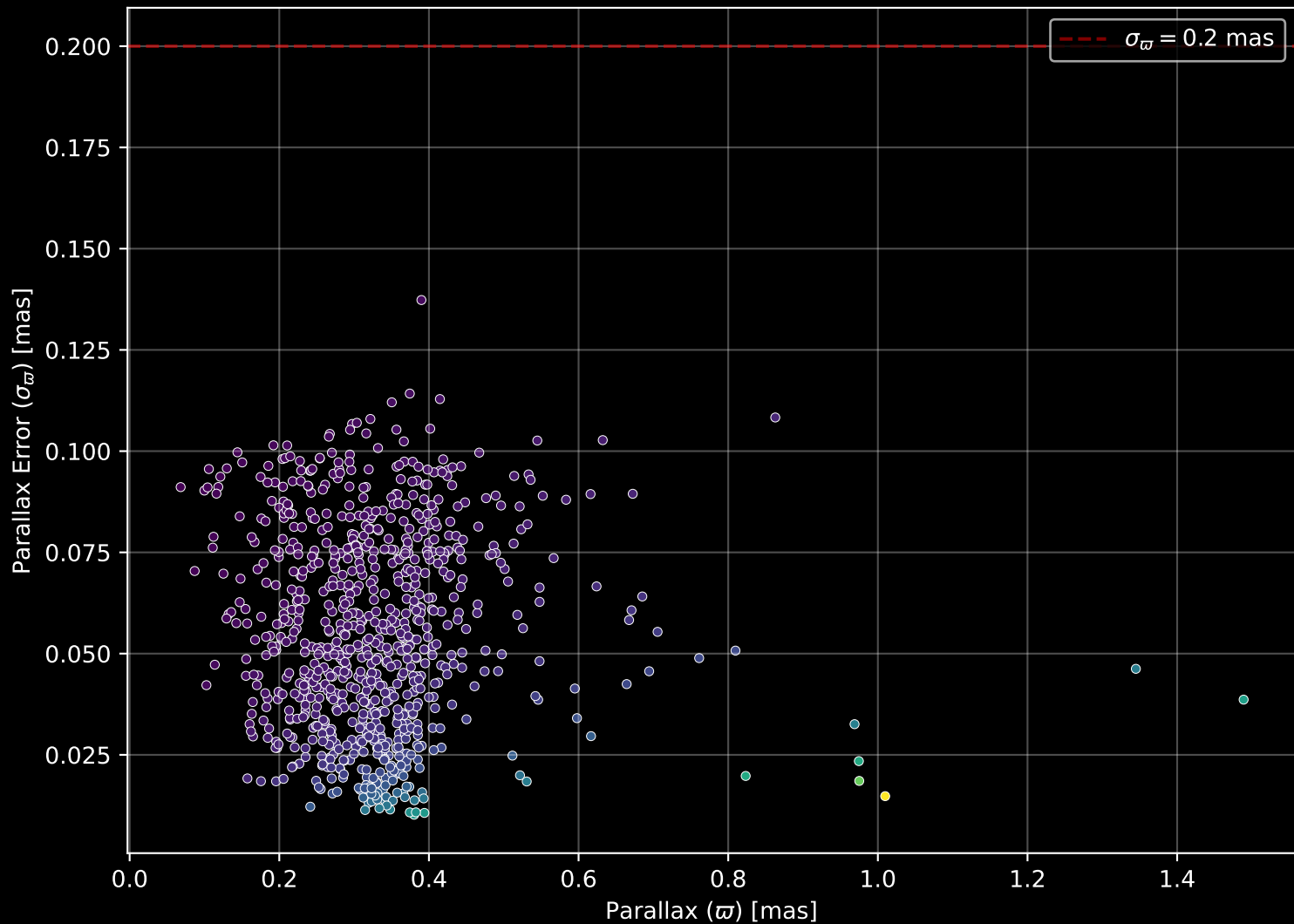
Gaia Cluster: [COIN-Gaia_29] Parallax Quality (n= 830)
