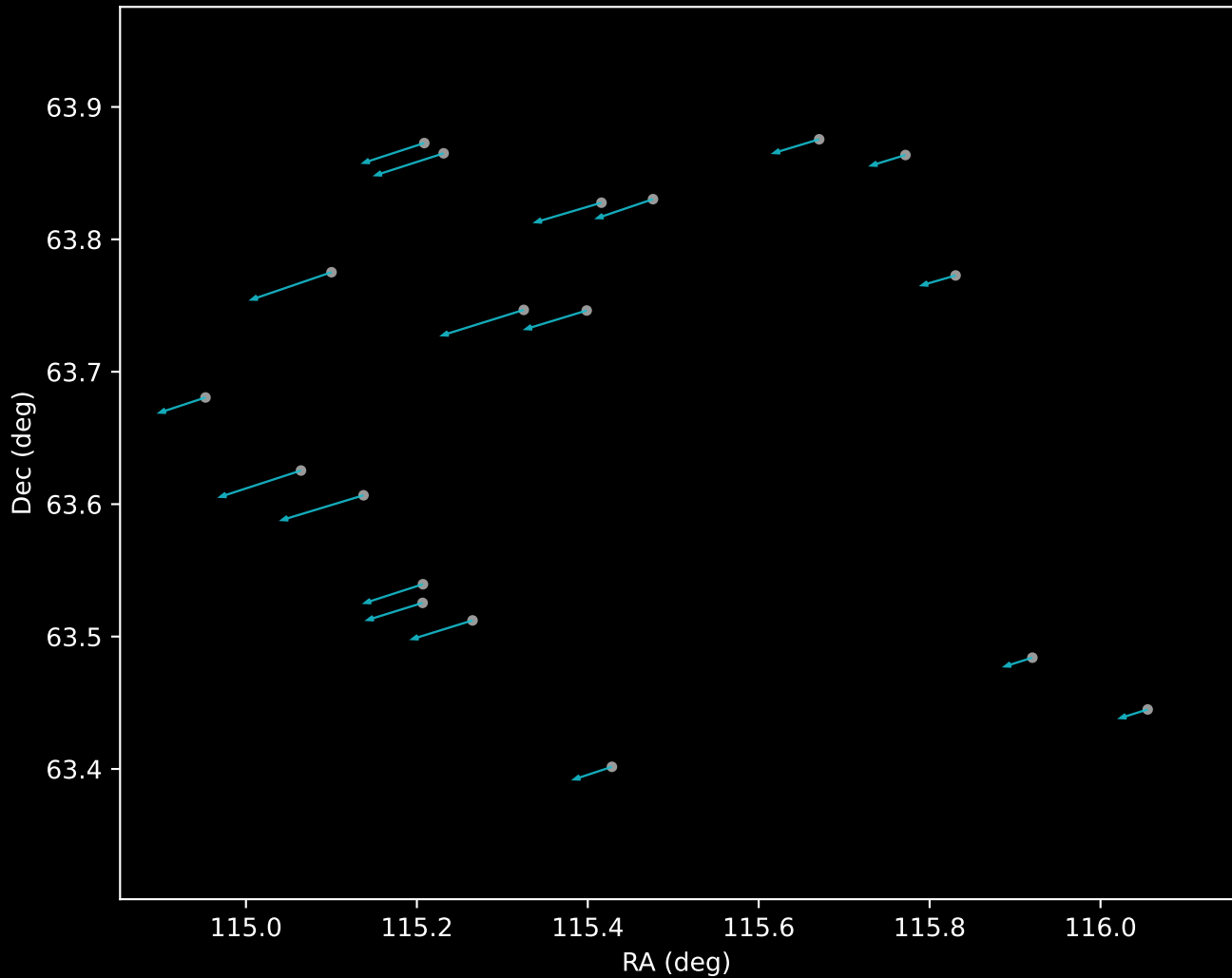
Gaia DR3 Cluster 38 Proper Motion Vectors (n=19)
