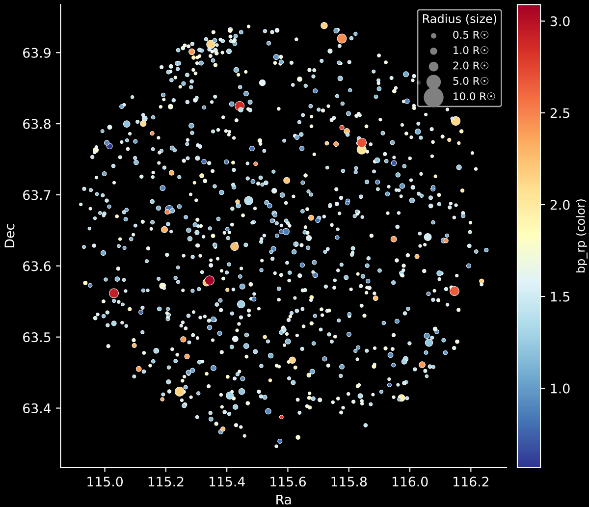
Gaia Cluster: [COIN-Gaia_29] Stars: 830
