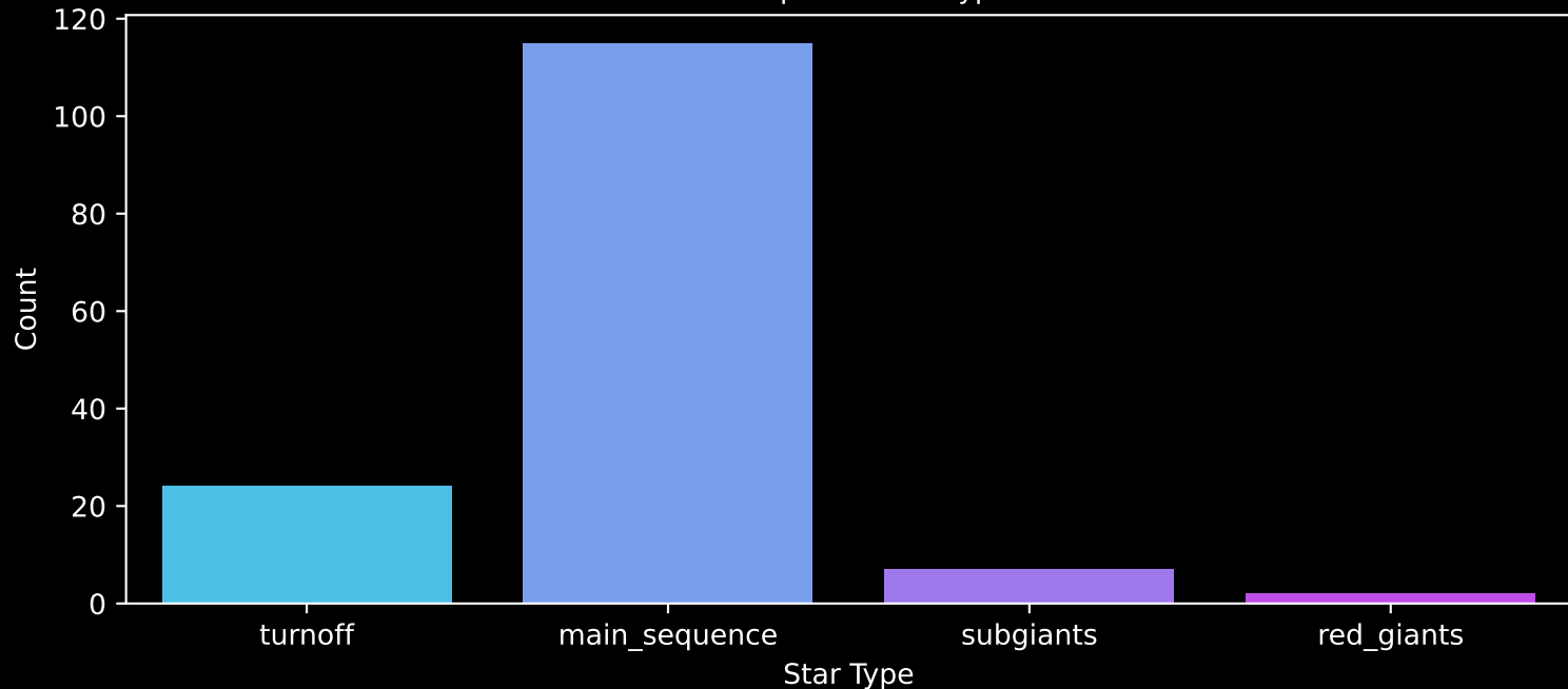
Gaia Cluster: [COIN-Gaia_3] Count plot of Star Type
