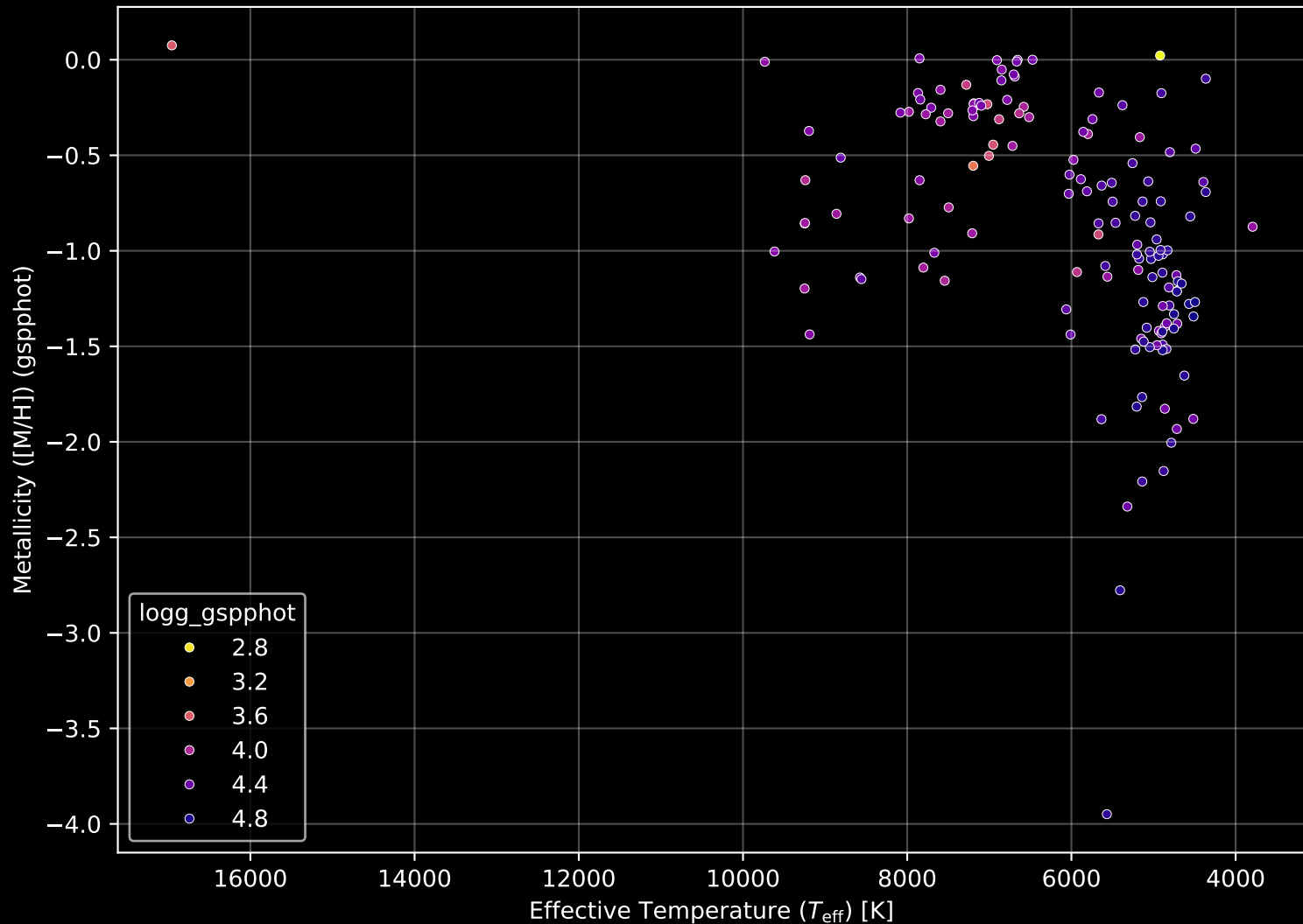
Gaia Cluster: [COIN-Gaia_3] Stellar Population Parameters (n= 148)
