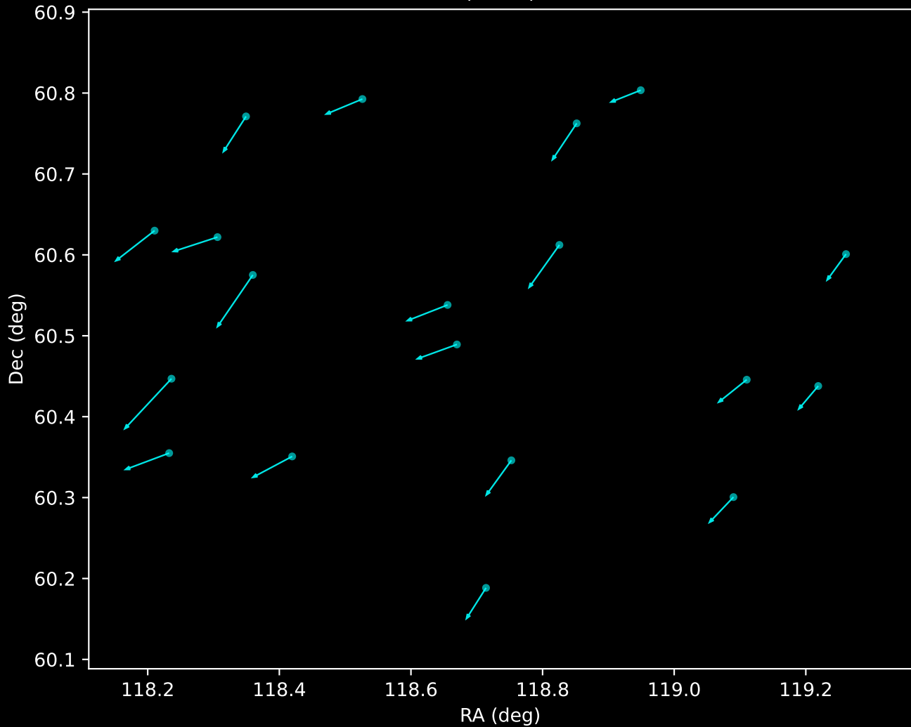
Gaia DR3 Noise Stream Proper Motion Vectors (n=19)
