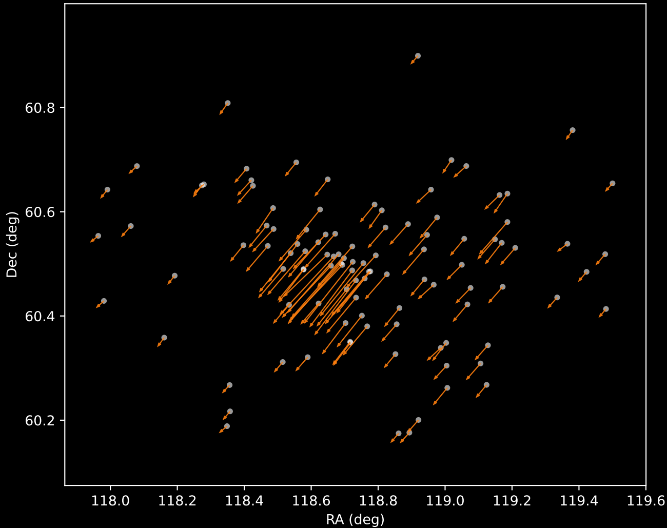
Gaia DR3 Cluster 2 Proper Motion Vectors (n=106)
