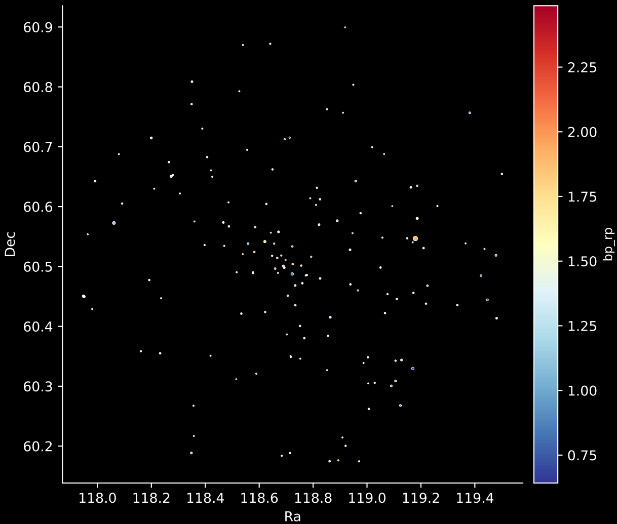
Gaia Cluster: [COIN-Gaia_3] Stars: 148
