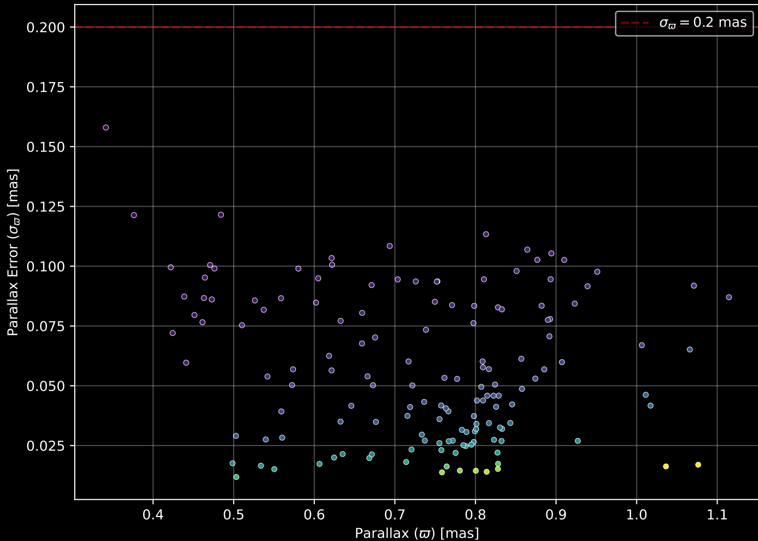
Gaia Cluster: [COIN-Gaia_3] Parallax Quality (n= 148)
