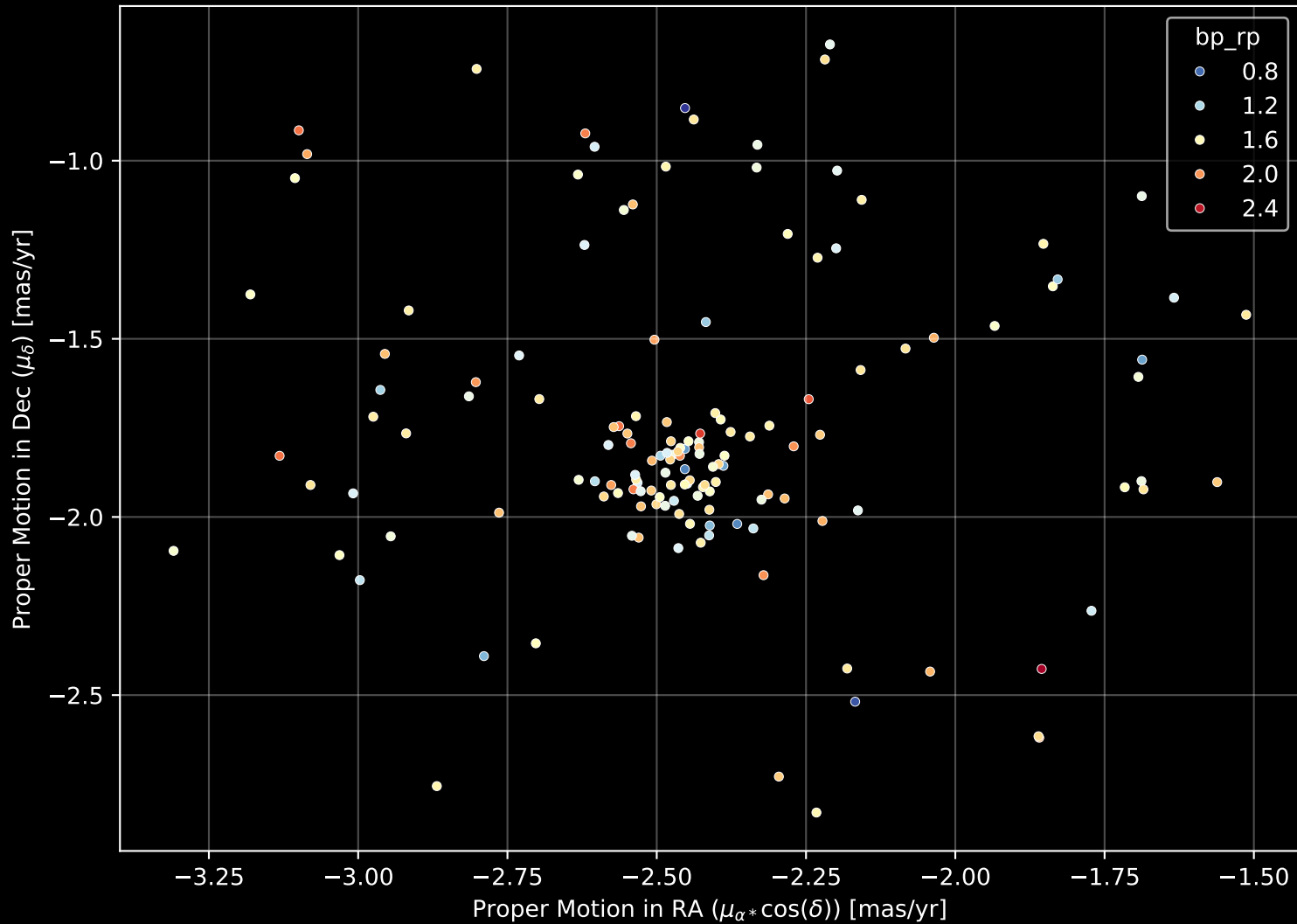
Gaia Cluster: [COIN-Gaia_3] Proper Motion Diagram (n= 148)
