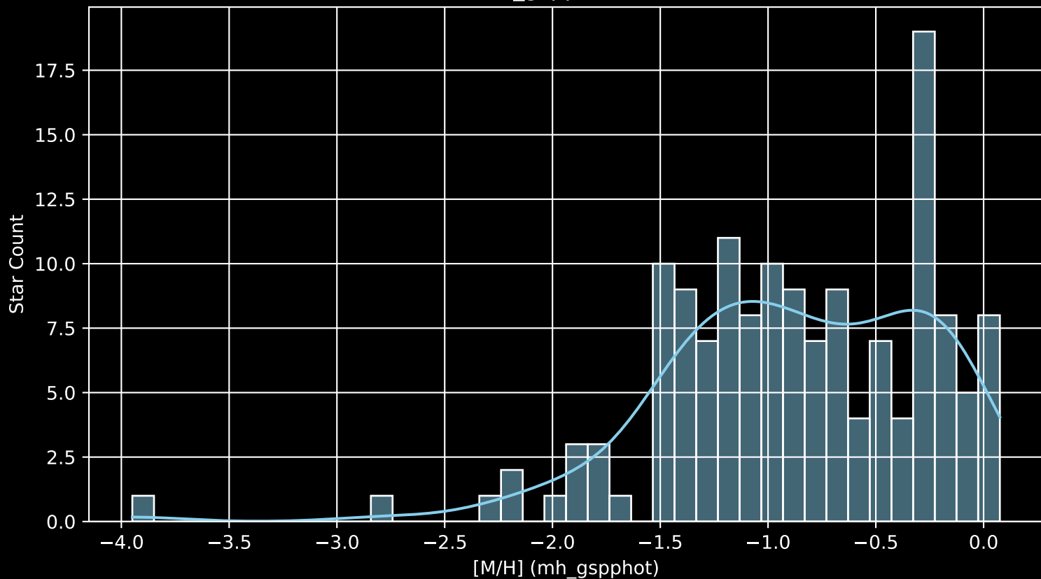
Gaia Cluster: [COIN-Gaia_3 [M/H] (mh_gspphot) (n= 148)
