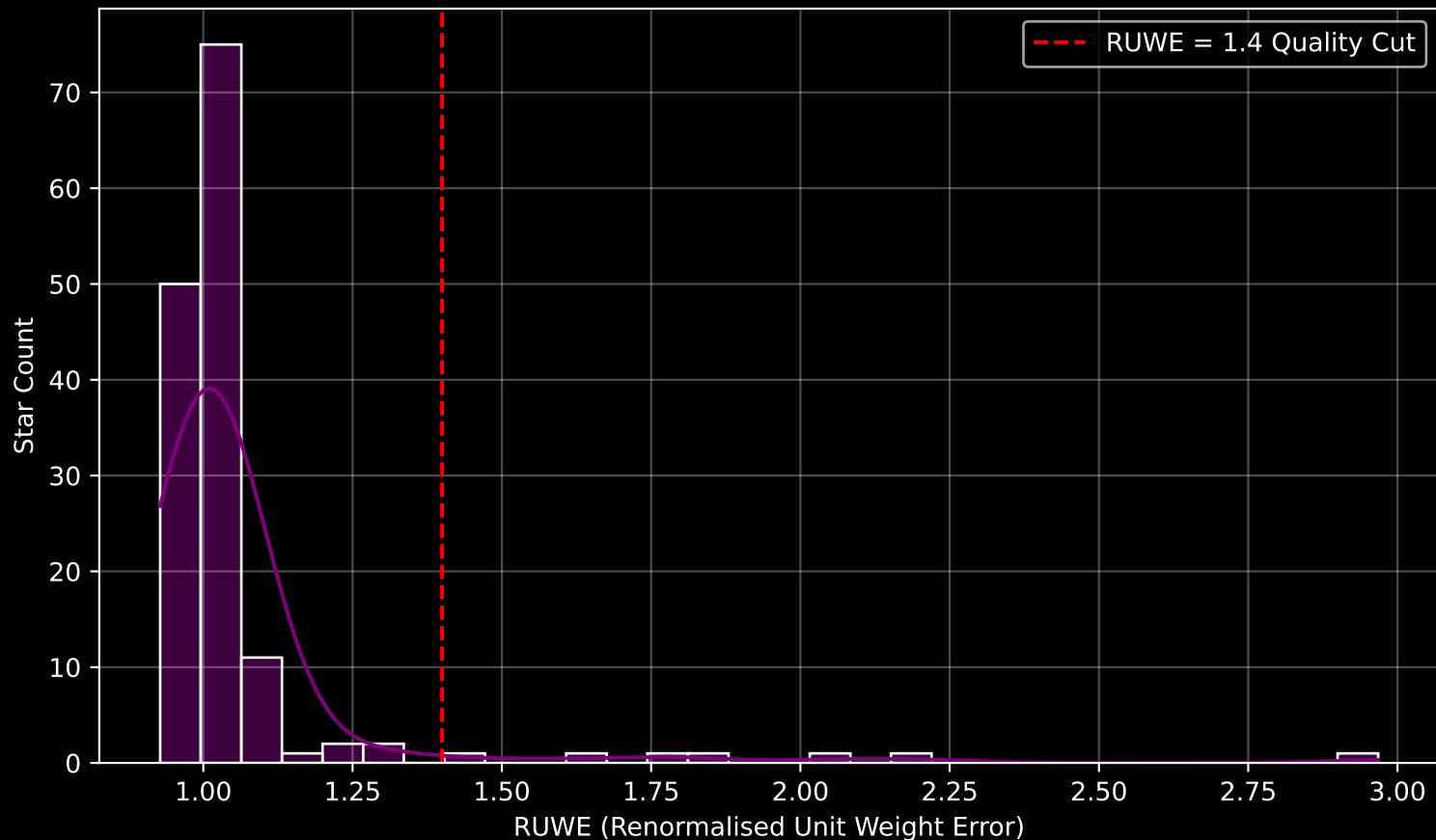
Gaia Cluster: [COIN-Gaia_3] RUWE Distribution (n= 148)
