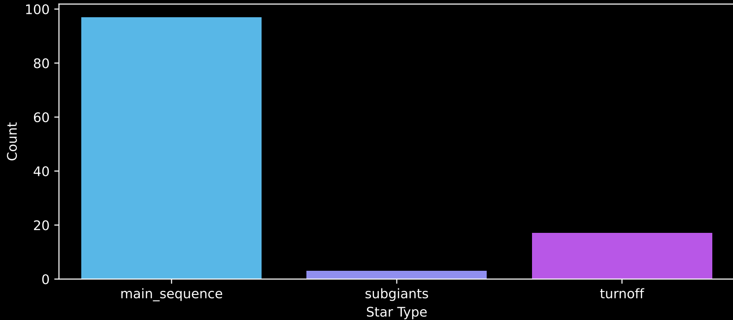
Gaia Cluster: [COIN-Gaia_30] Count plot of Star Type
