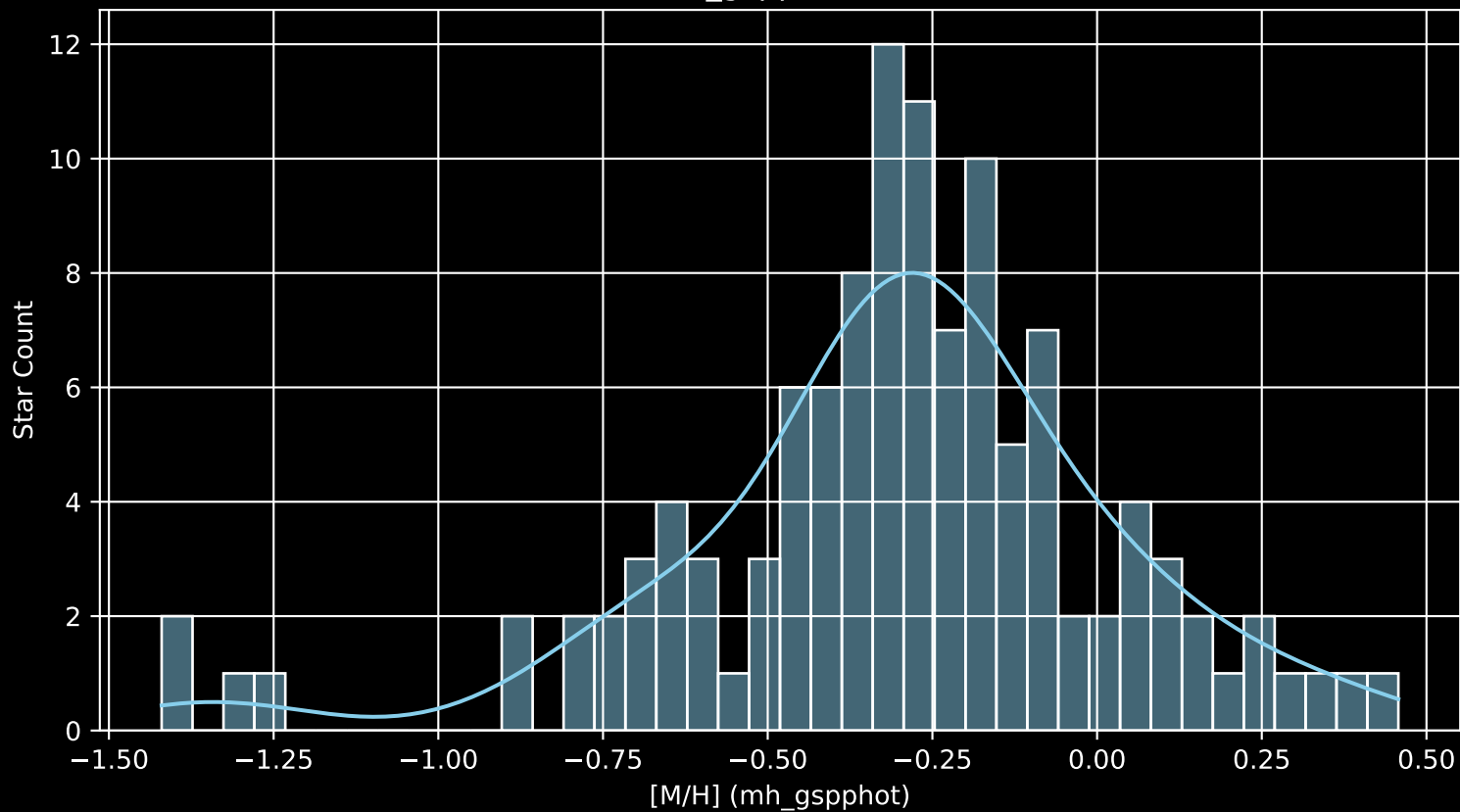
Gaia Cluster: [COIN-Gaia_30 [M/H] (mh_gspphot) (n= 116)
