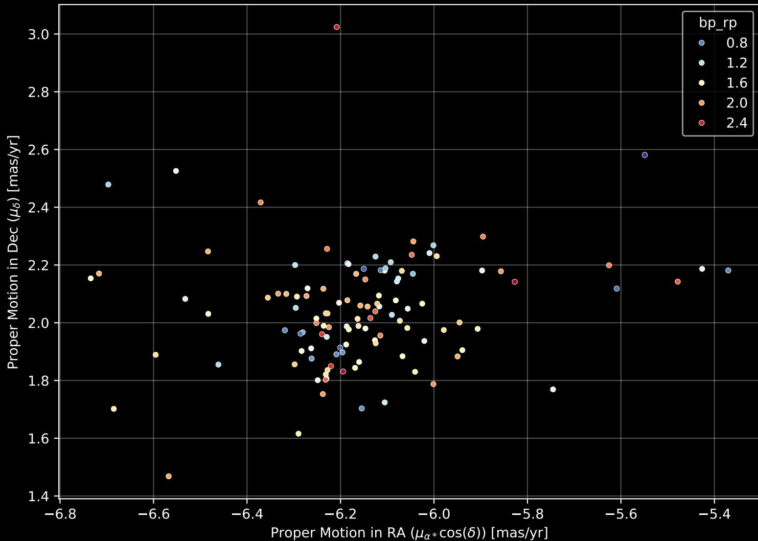
Gaia Cluster: [COIN-Gaia_30] Proper Motion Diagram (n= 117)
