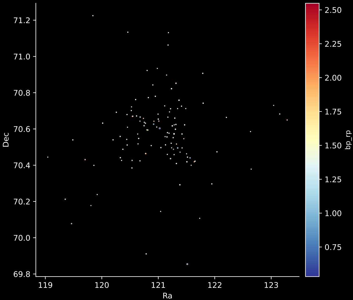
Gaia Cluster: [COIN-Gaia_30] Stars: 117
