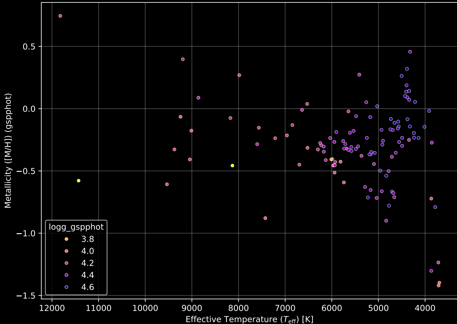
Gaia Cluster: [COIN-Gaia_30] Stellar Population Parameters (n= 117)
