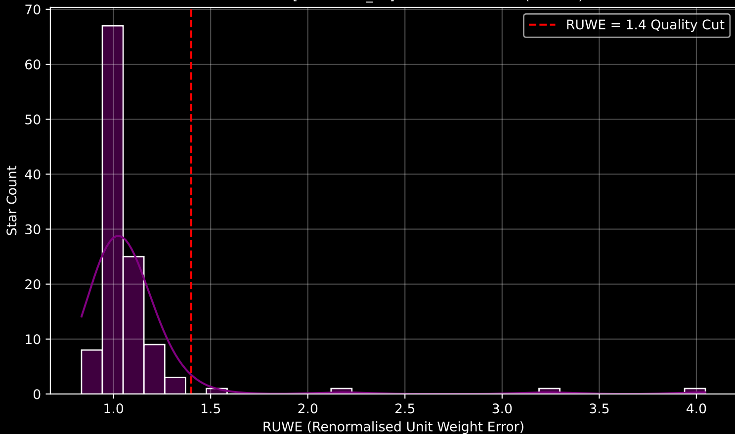
Gaia Cluster: [COIN-Gaia_30] RUWE Distribution (n= 116)
