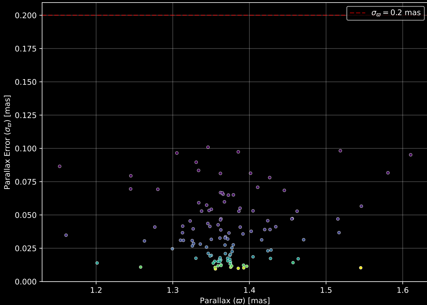
Gaia Cluster: [COIN-Gaia_30] Parallax Quality (n= 117)
