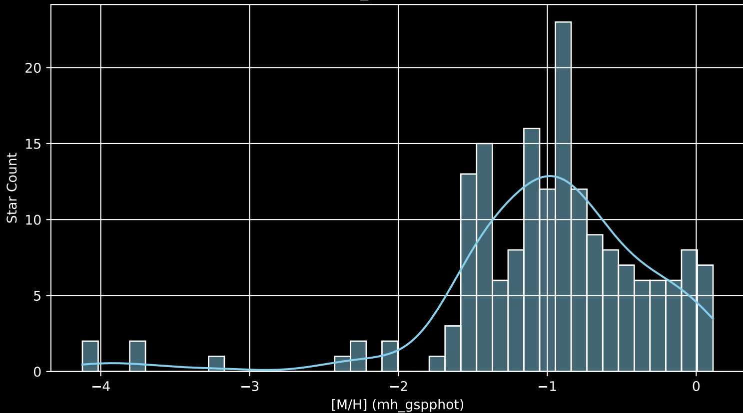
Gaia Cluster: [COIN-Gaia_33 [M/H] (mh_gspphot) (n= 176)
