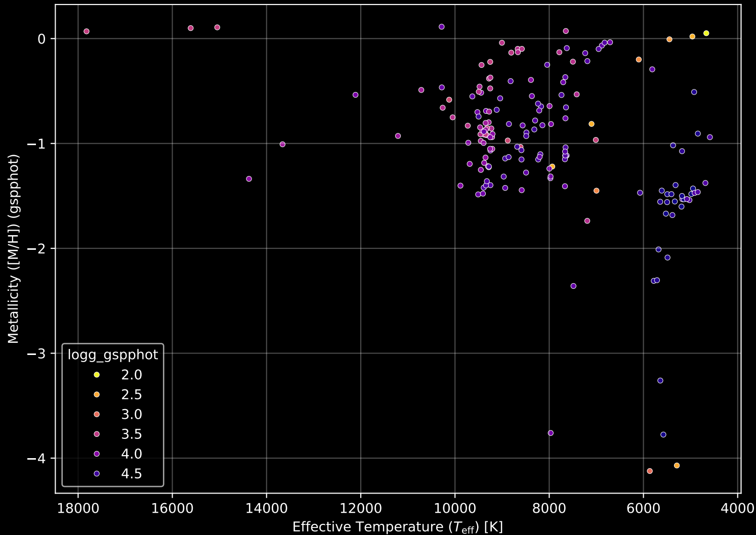
Gaia Cluster: [COIN-Gaia_33] Stellar Population Parameters (n= 176)
