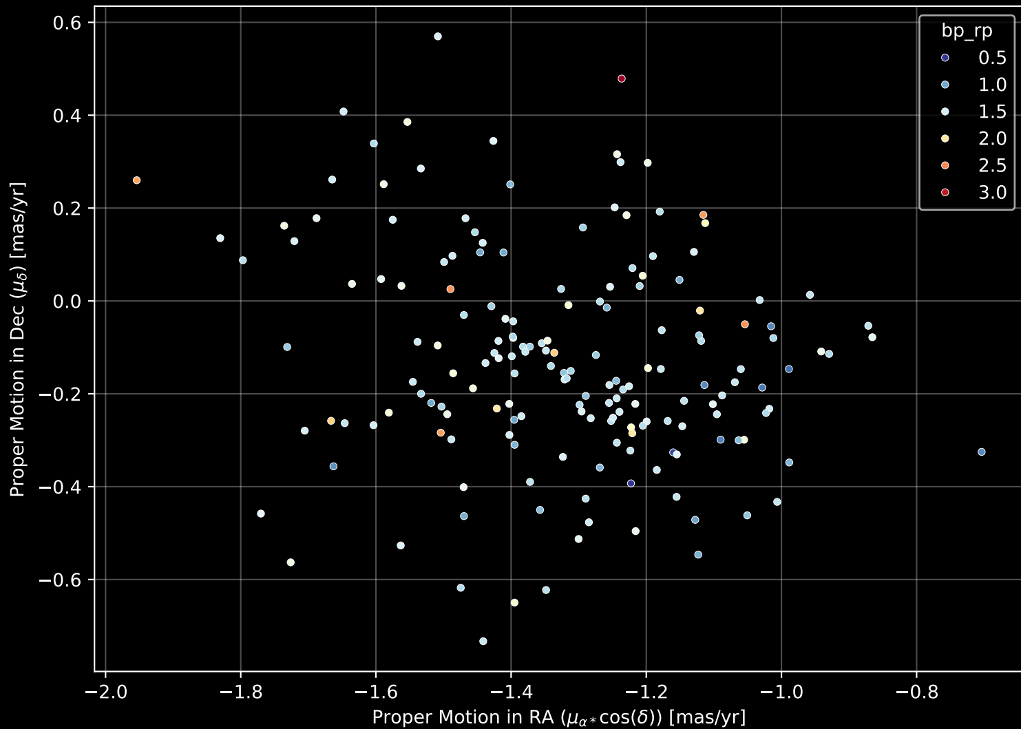
Gaia Cluster: [COIN-Gaia_33] Proper Motion Diagram (n= 176)
