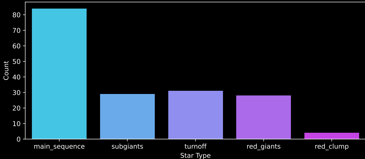
Gaia Cluster: [COIN-Gaia_33] Count plot of Star Type
