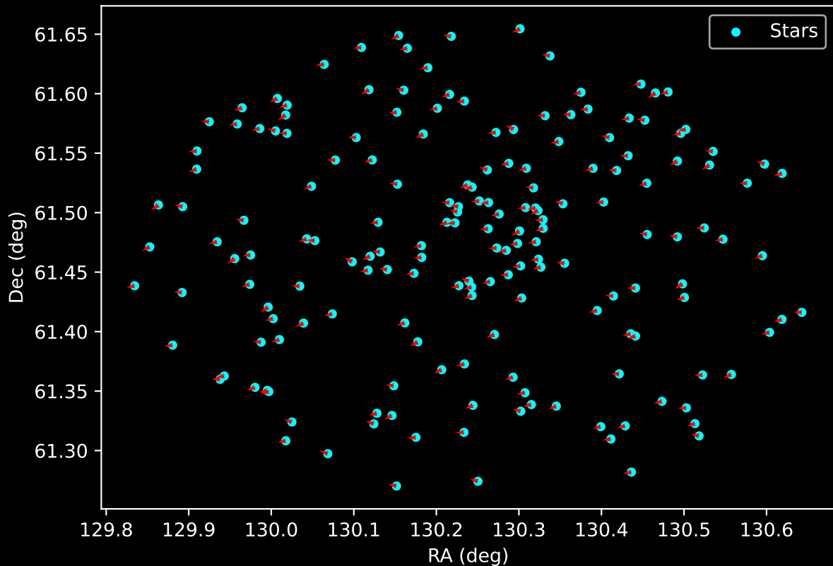
Gaia Cluster: [COIN-Gaia_33] Proper Motion Vectors for Gaia Star Field (n= 176)
