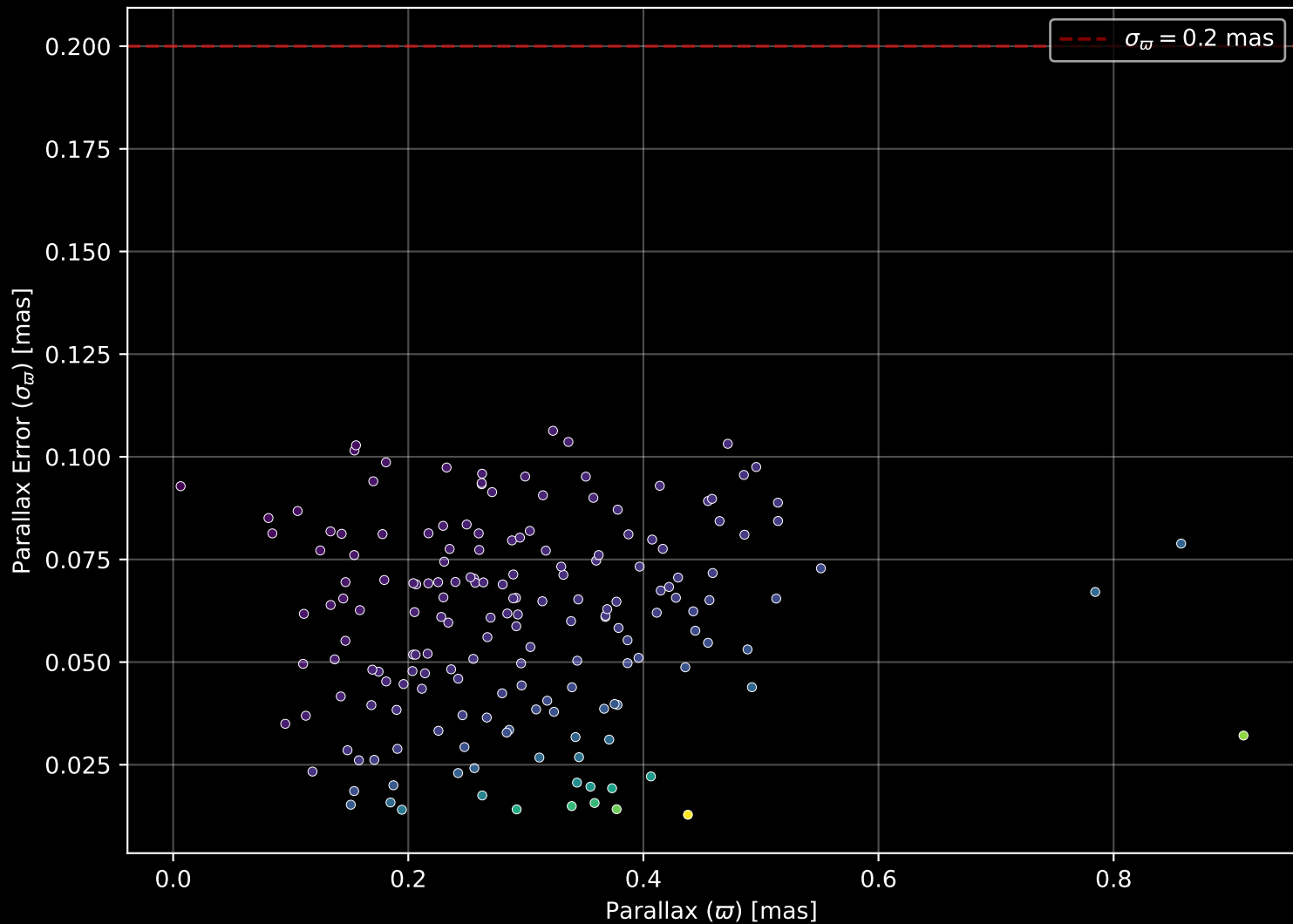
Gaia Cluster: [COIN-Gaia_33] Parallax Quality (n= 176)
