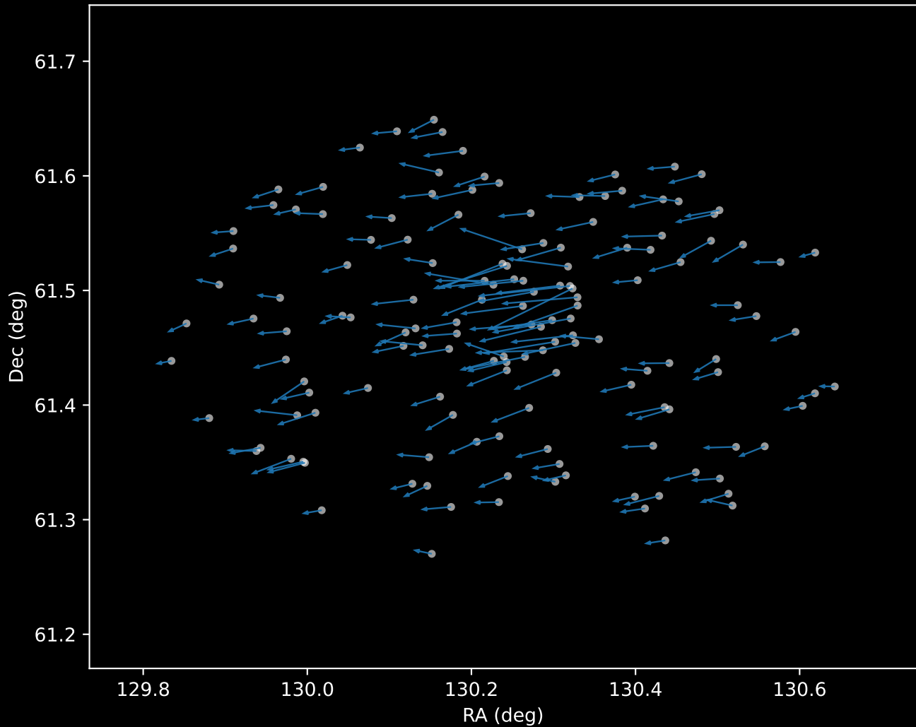
Gaia DR3 Cluster 0 Proper Motion Vectors (n=146)
