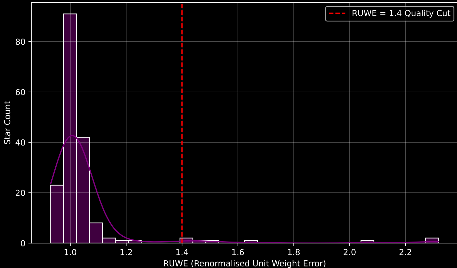
Gaia Cluster: [COIN-Gaia_33] RUWE Distribution (n= 176)
