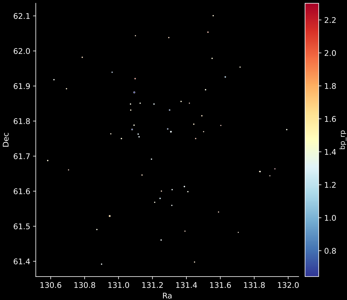
Gaia Cluster: [COIN-Gaia_34] Stars: 58
