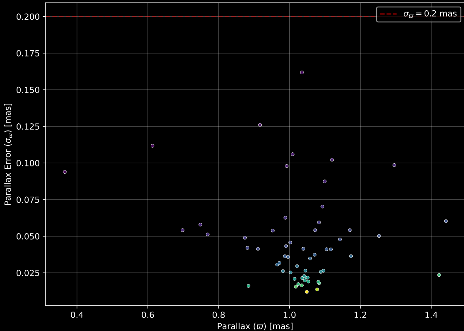
Gaia Cluster: [COIN-Gaia_34] Parallax Quality (n= 58)
