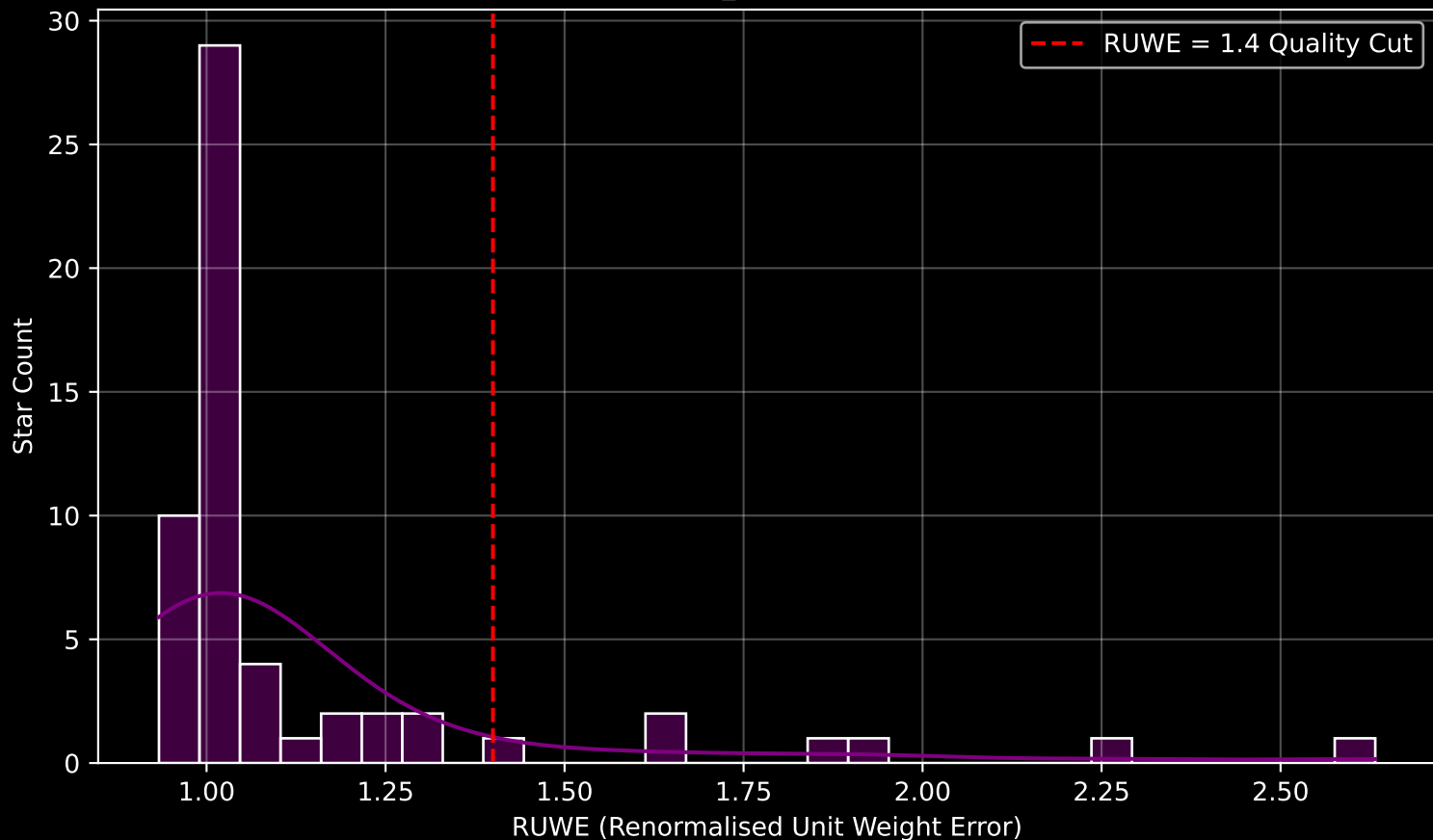
Gaia Cluster: [COIN-Gaia_34] RUWE Distribution (n= 57)
