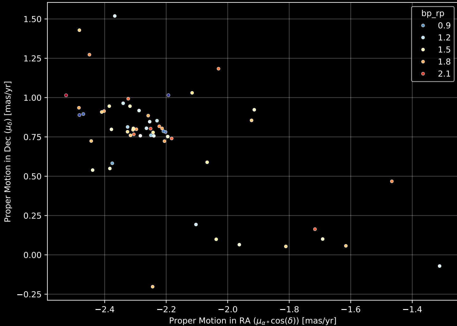
Gaia Cluster: [COIN-Gaia_34] Proper Motion Diagram (n= 58)
