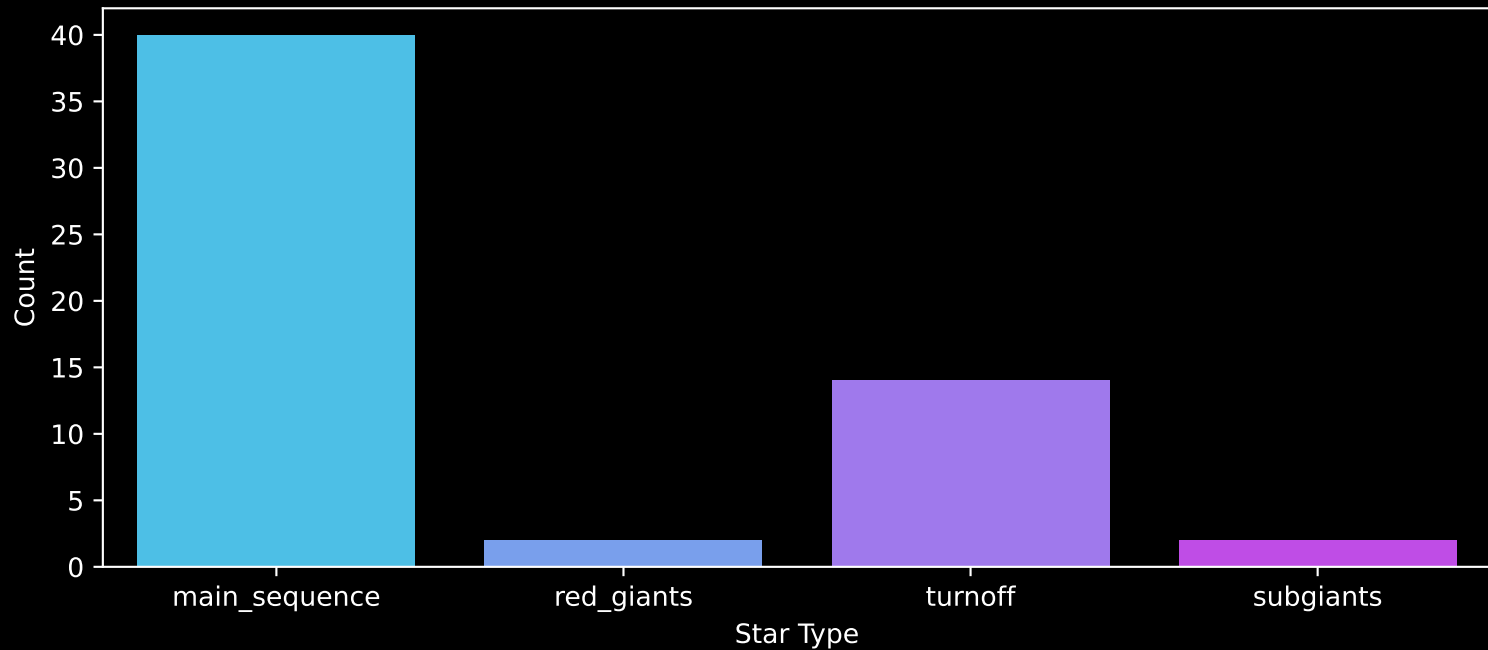
Gaia Cluster: [COIN-Gaia_34] Count plot of Star Type
