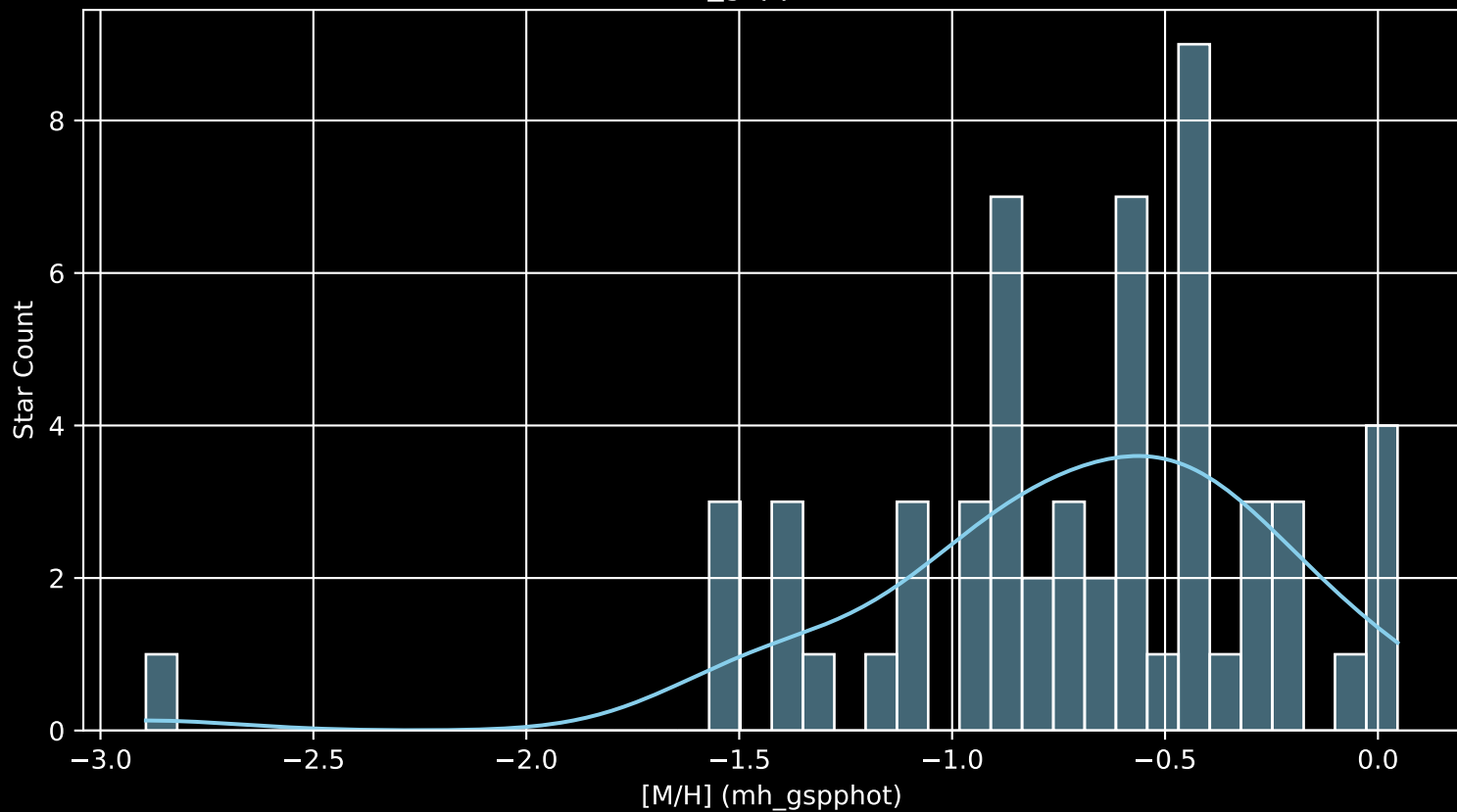
Gaia Cluster: [COIN-Gaia_34 [M/H] (mh_gspphot) (n= 58)
