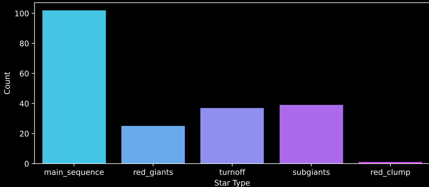
Gaia Cluster: [COIN-Gaia_35] Count plot of Star Type
