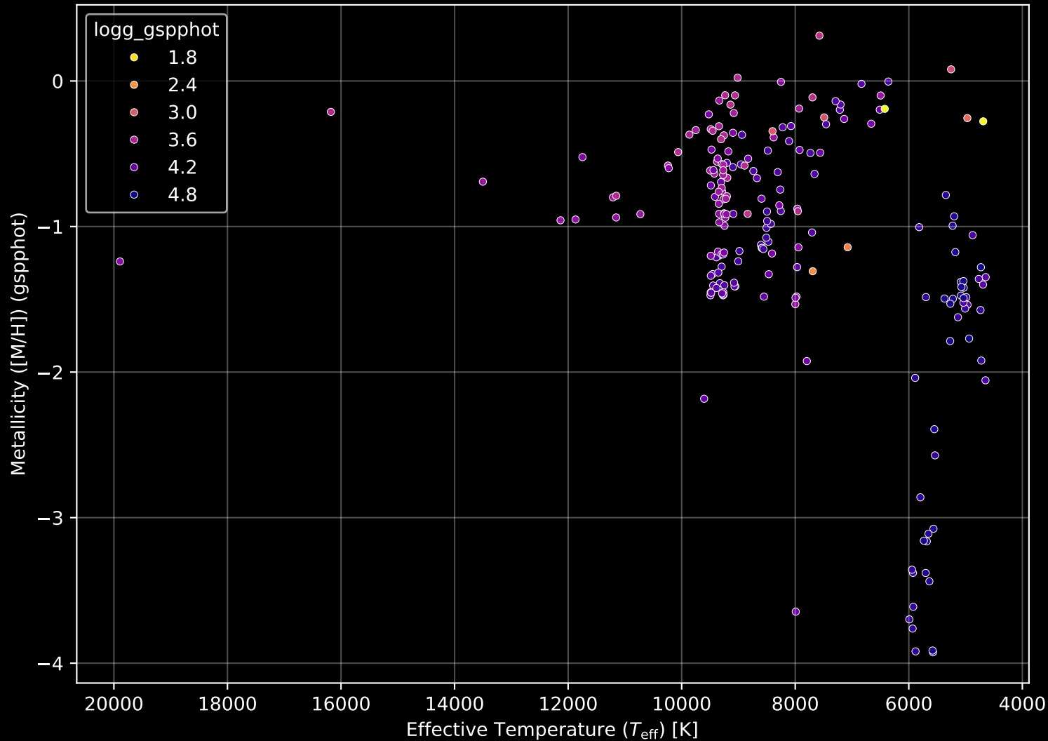
Gaia Cluster: [COIN-Gaia_35] Stellar Population Parameters (n= 204)
