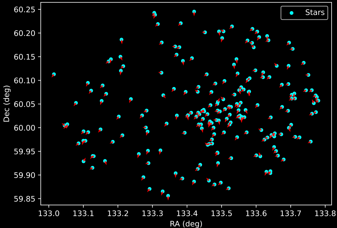
Gaia Cluster: [COIN-Gaia_35] Proper Motion Vectors for Gaia Star Field (n= 204)
