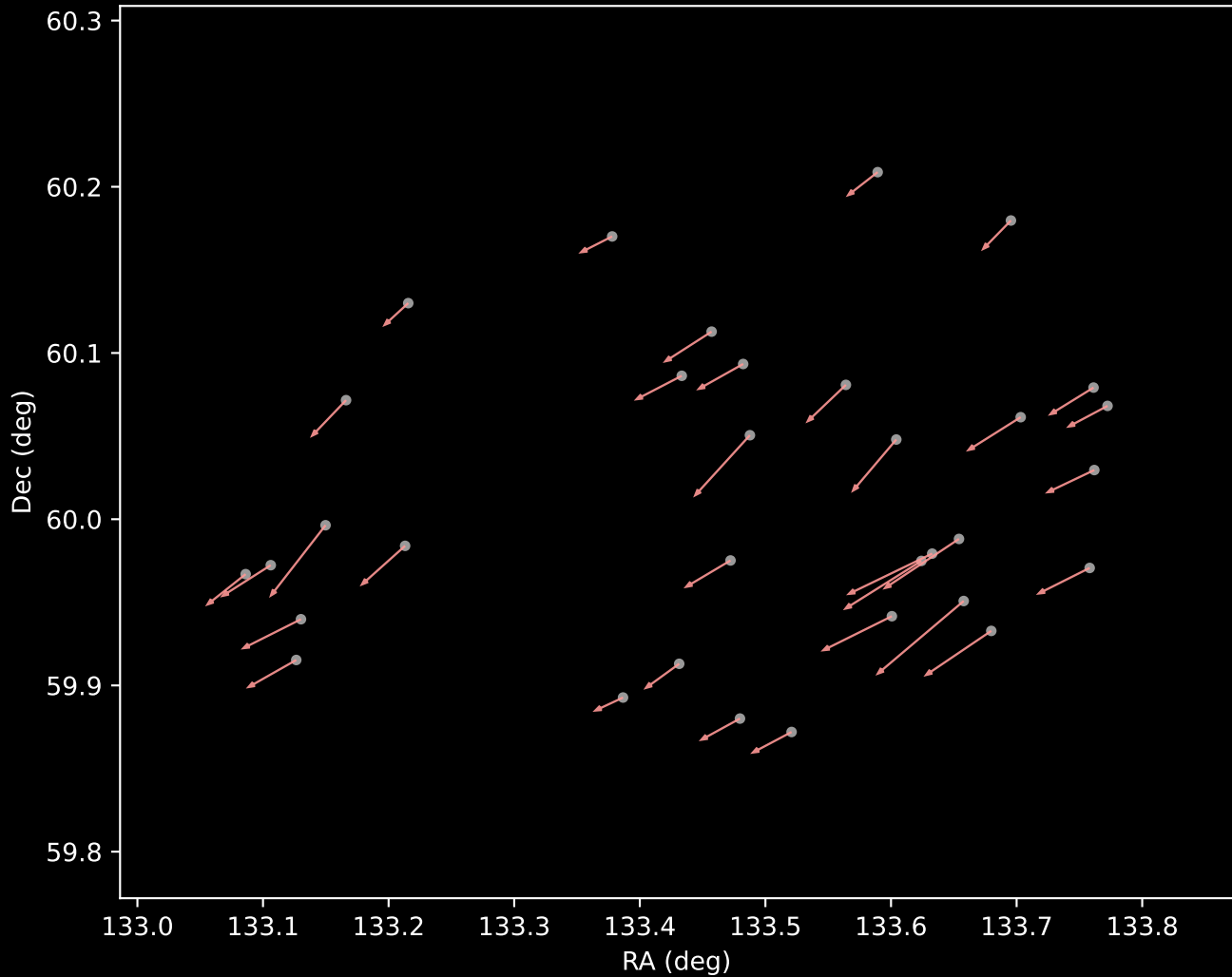
Gaia DR3 Cluster 7 Proper Motion Vectors (n=33)
