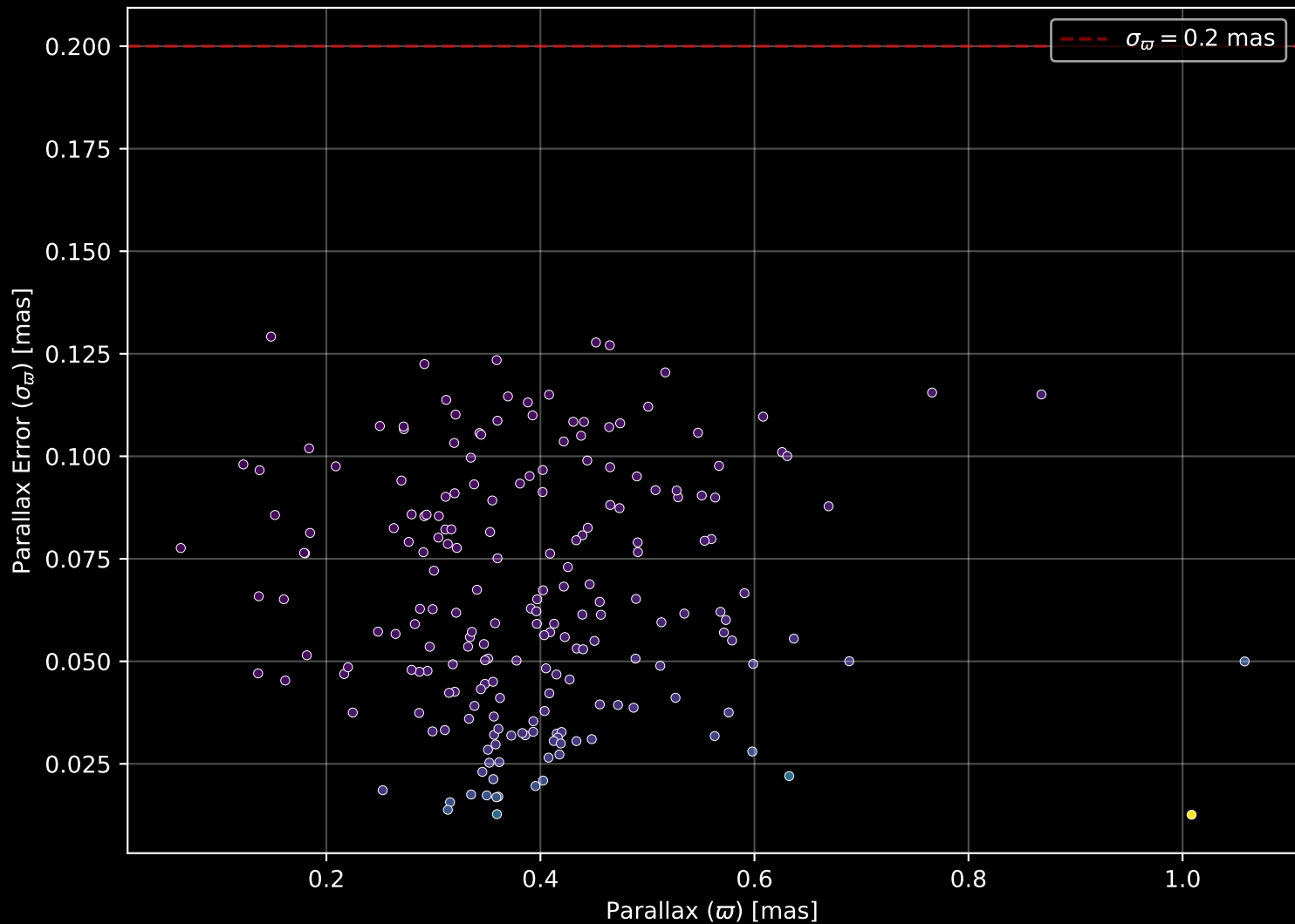
Gaia Cluster: [COIN-Gaia_35] Parallax Quality (n= 204)
