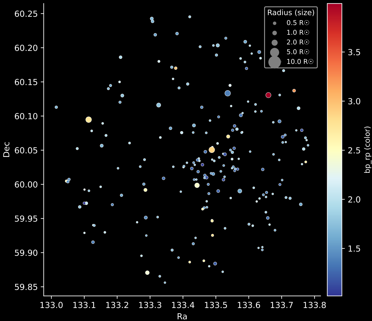
Gaia Cluster: [COIN-Gaia_35] Stars: 204
