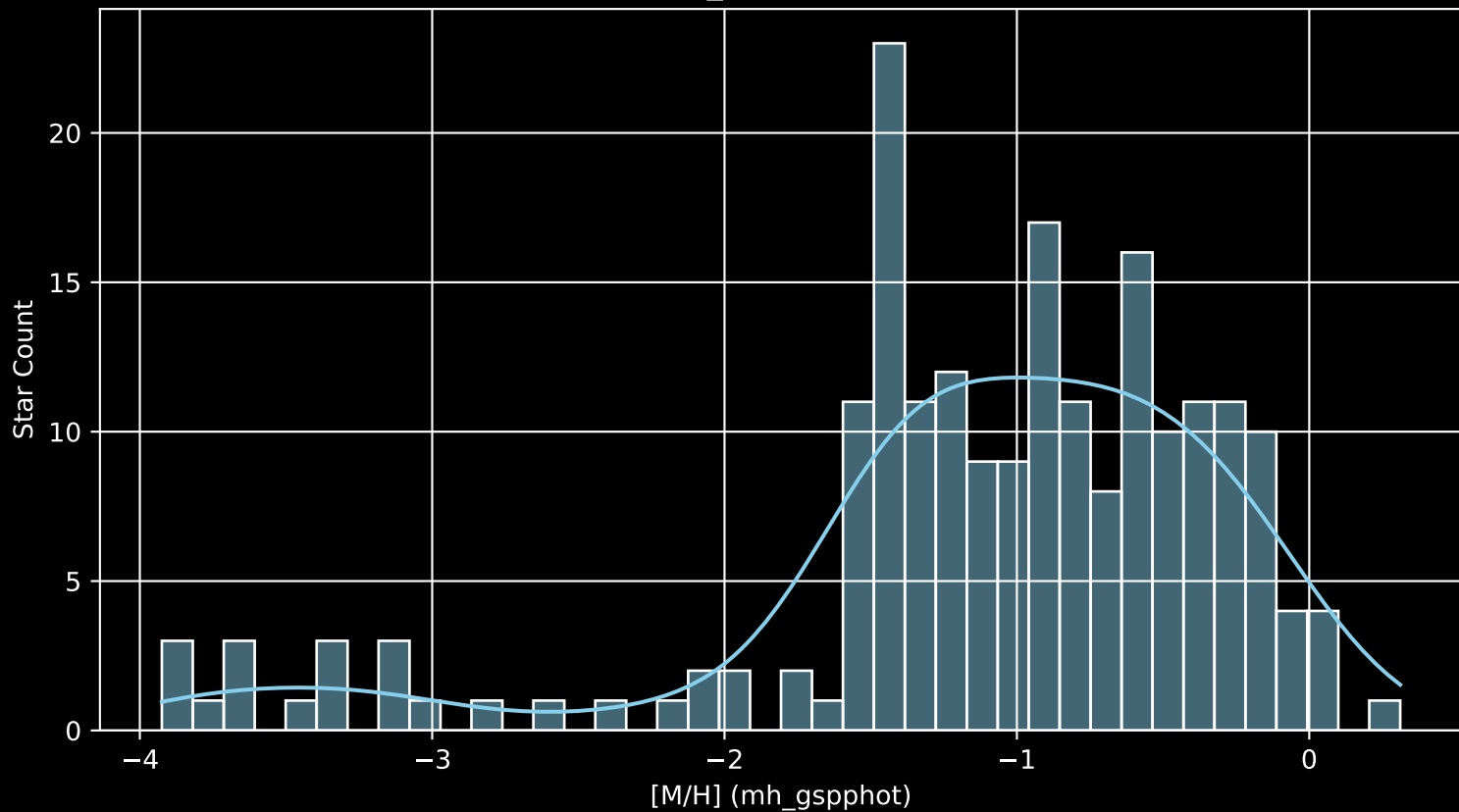
Gaia Cluster: [COIN-Gaia_35 [M/H] (mh_gspphot) (n= 204)
