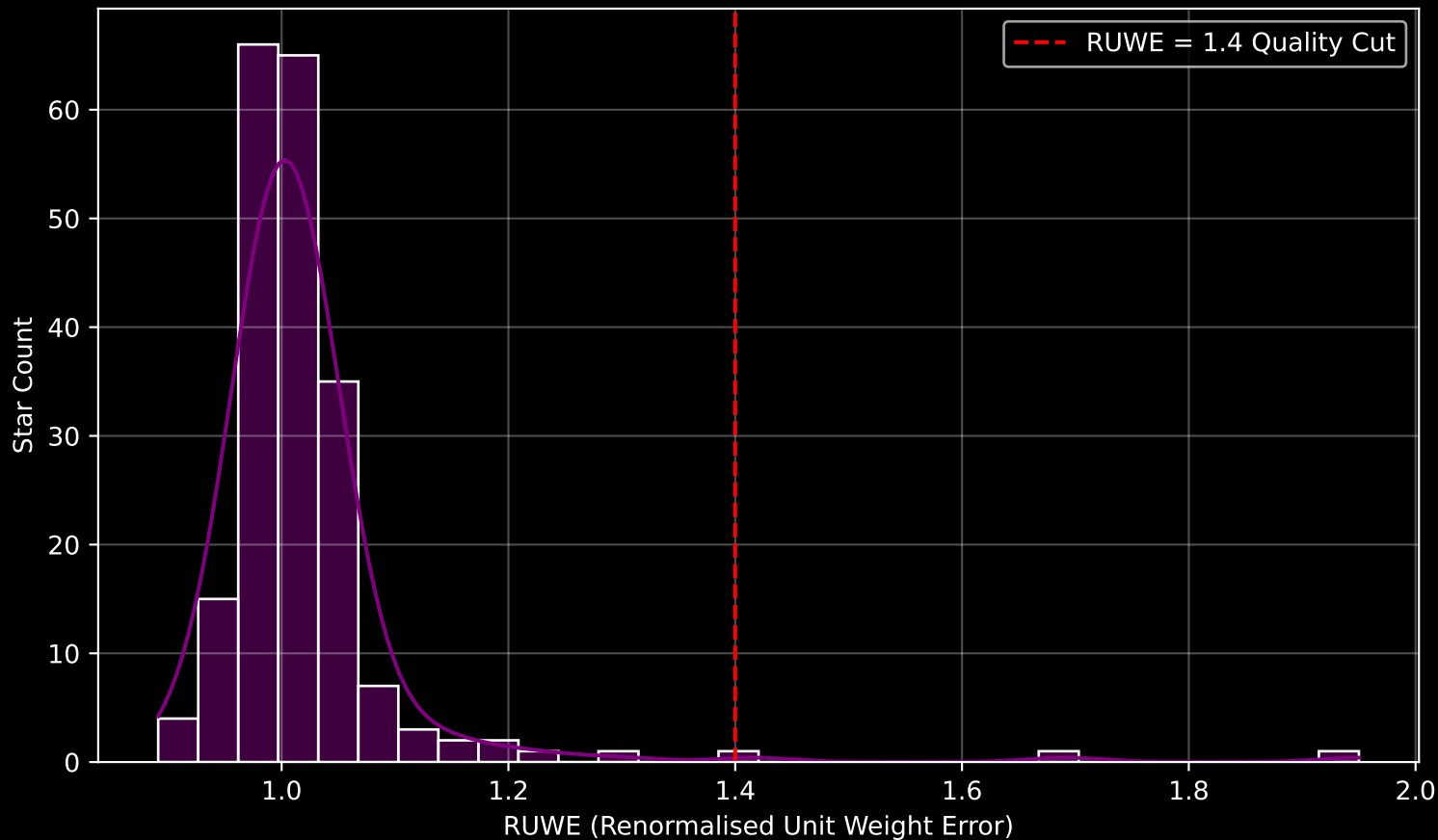
Gaia Cluster: [COIN-Gaia_35] RUWE Distribution (n= 204)
