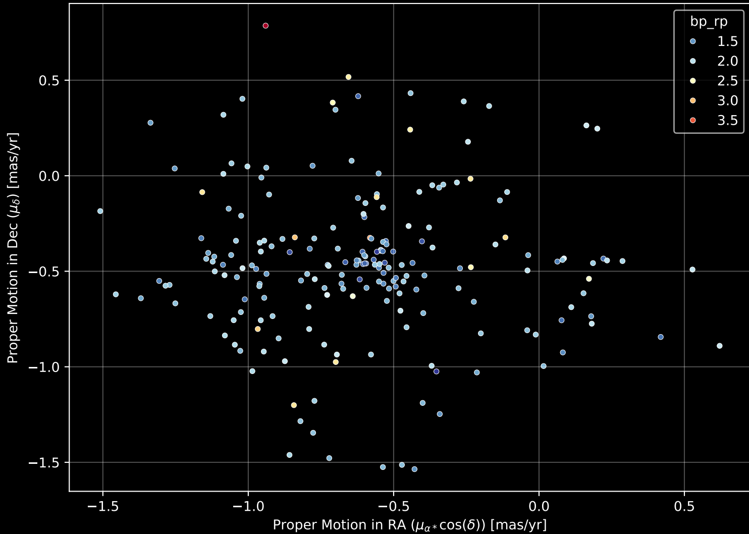
Gaia Cluster: [COIN-Gaia_35] Proper Motion Diagram (n= 204)
