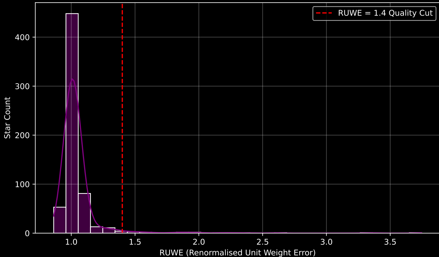
Gaia Cluster: [COIN-Gaia_36] RUWE Distribution (n= 627)
