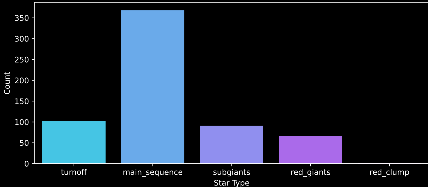
Gaia Cluster: [COIN-Gaia_36] Count plot of Star Type
