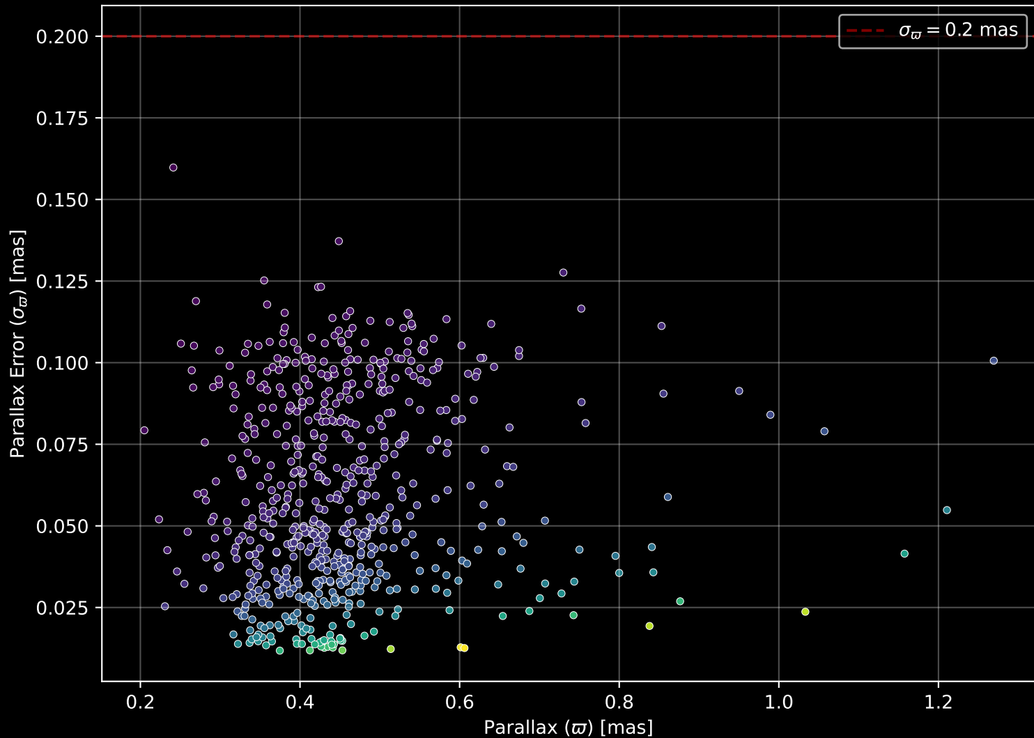
Gaia Cluster: [COIN-Gaia_36] Parallax Quality (n= 629)
