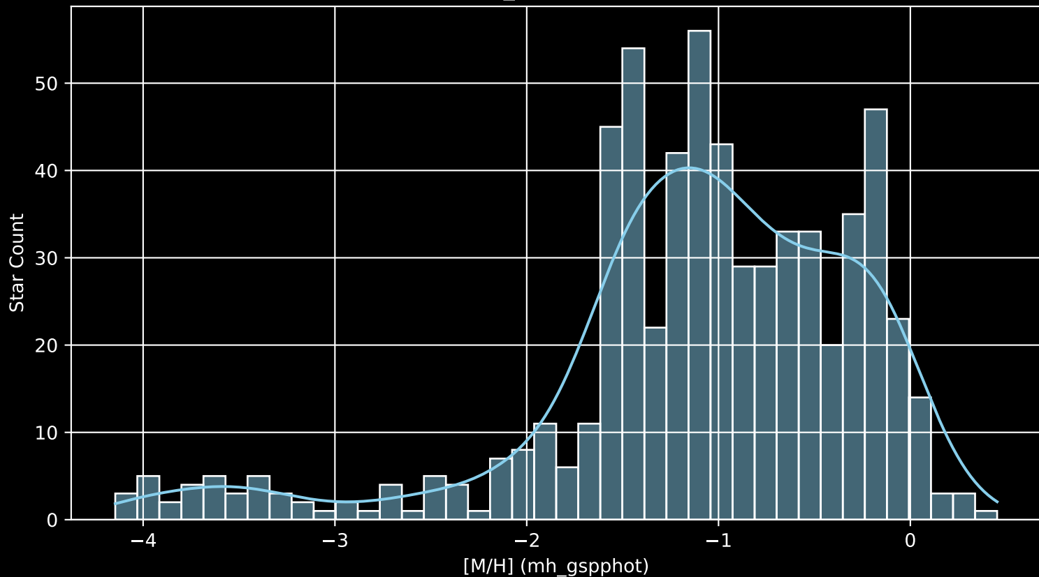
Gaia Cluster: [COIN-Gaia_36 [M/H] (mh_gspphot) (n= 626)
