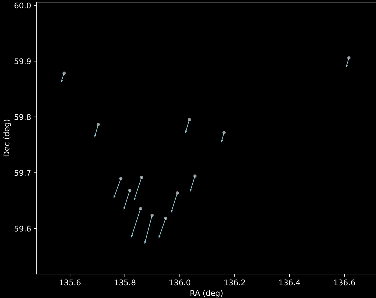
Gaia DR3 Cluster 19 Proper Motion Vectors (n=13)
