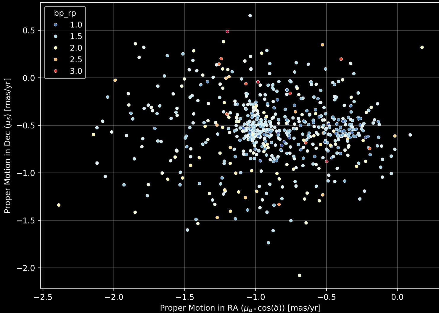
Gaia Cluster: [COIN-Gaia_36] Proper Motion Diagram (n= 629)
