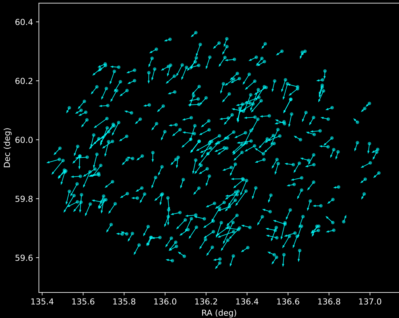
Gaia DR3 Noise Stream Proper Motion Vectors (n=308)
