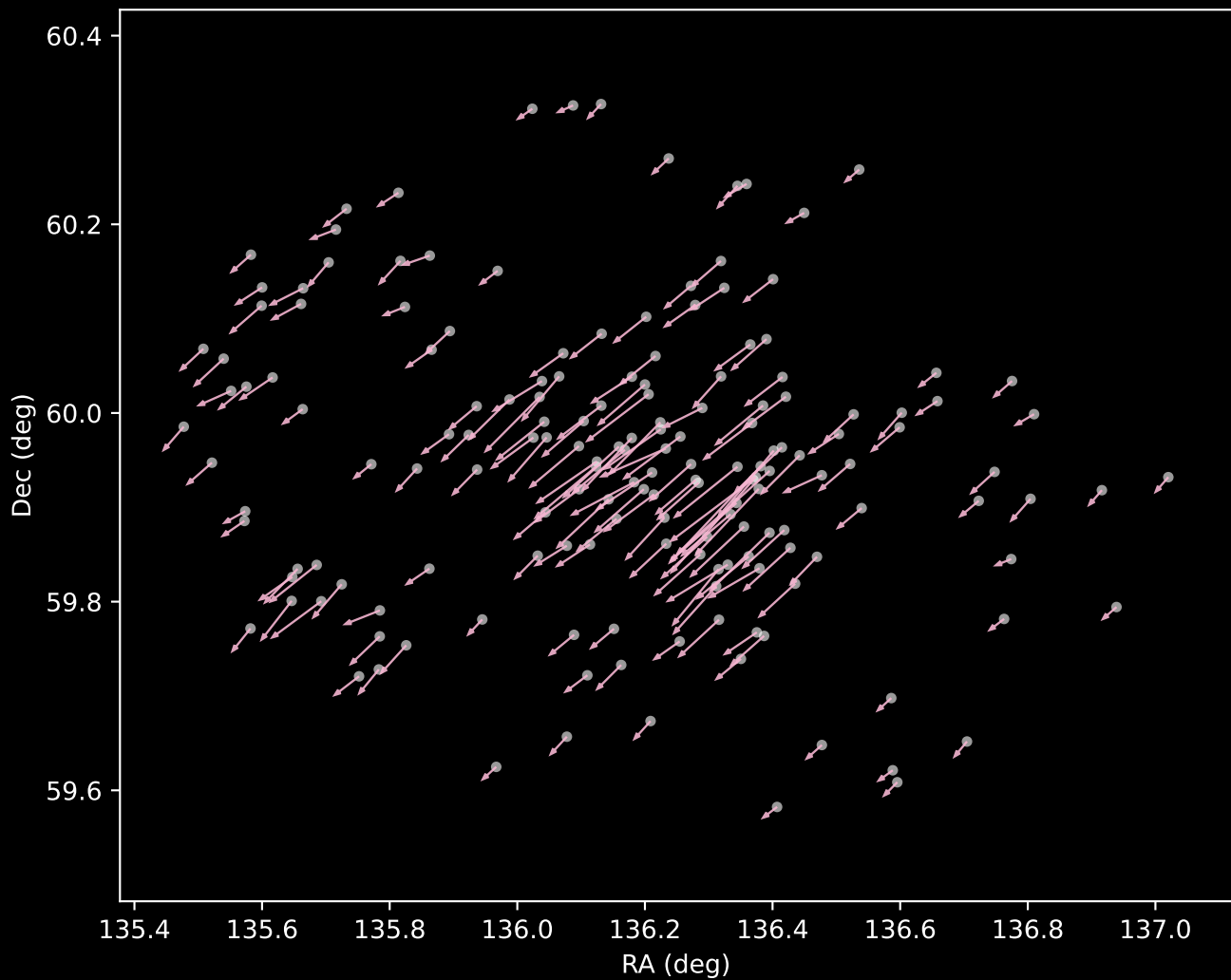
Gaia DR3 Cluster 13 Proper Motion Vectors (n=169)
