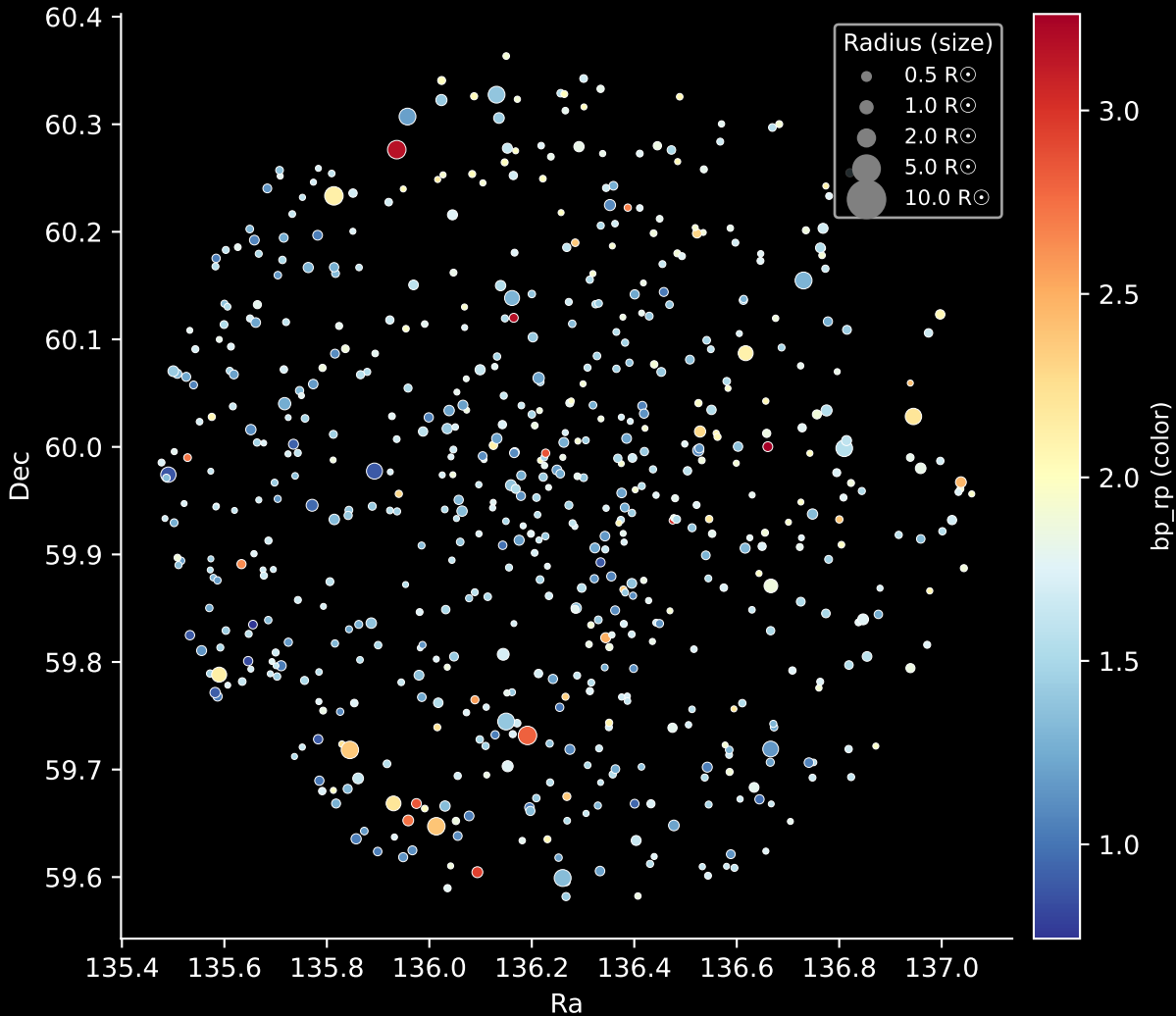
Gaia Cluster: [COIN-Gaia_36] Stars: 629
