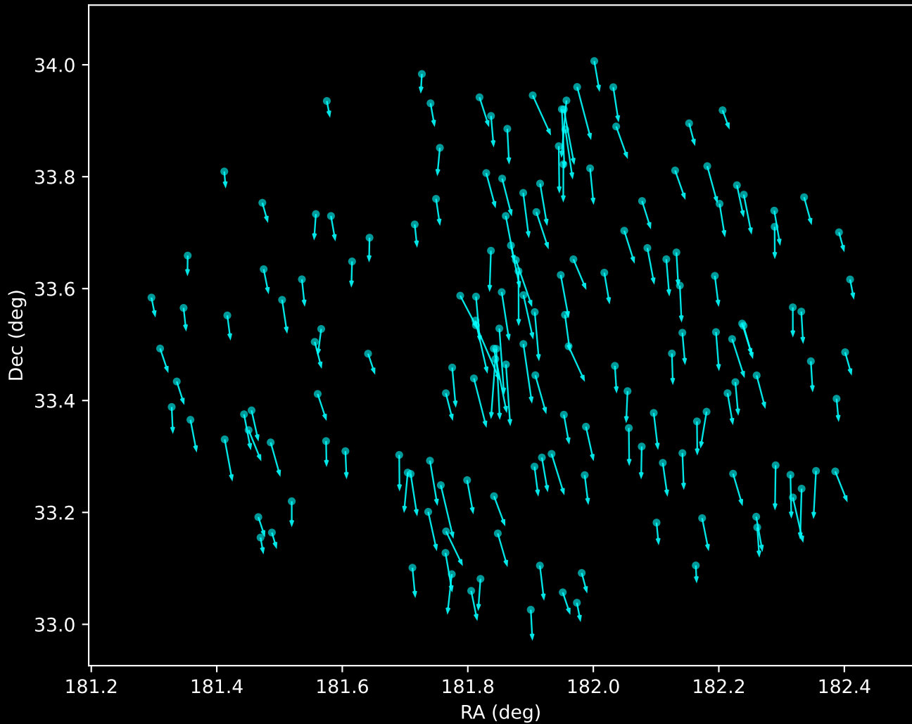
Gaia DR3 Noise Stream Proper Motion Vectors (n=165)
