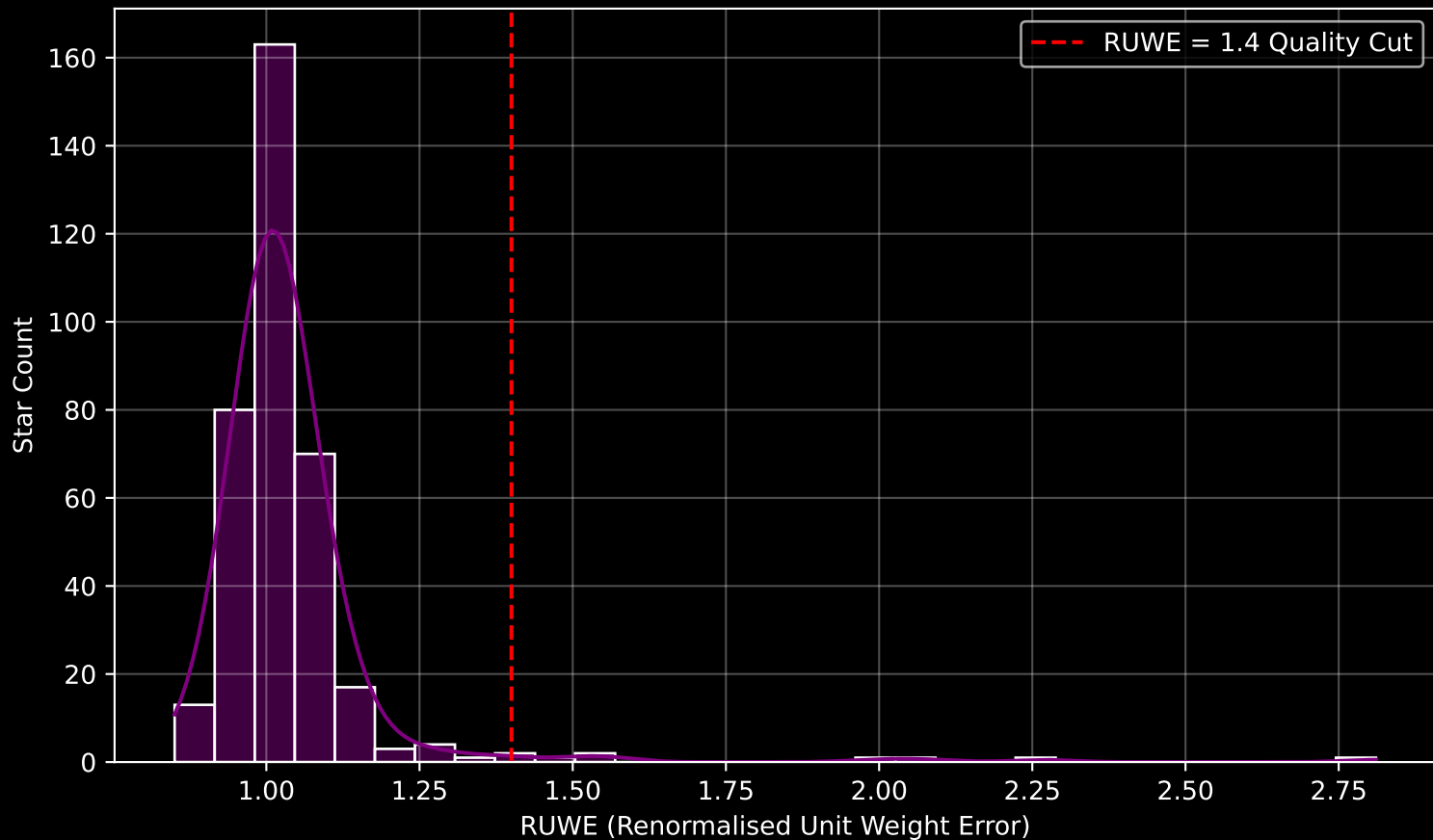
Gaia Cluster: [COIN-Gaia_40] RUWE Distribution (n= 360)
