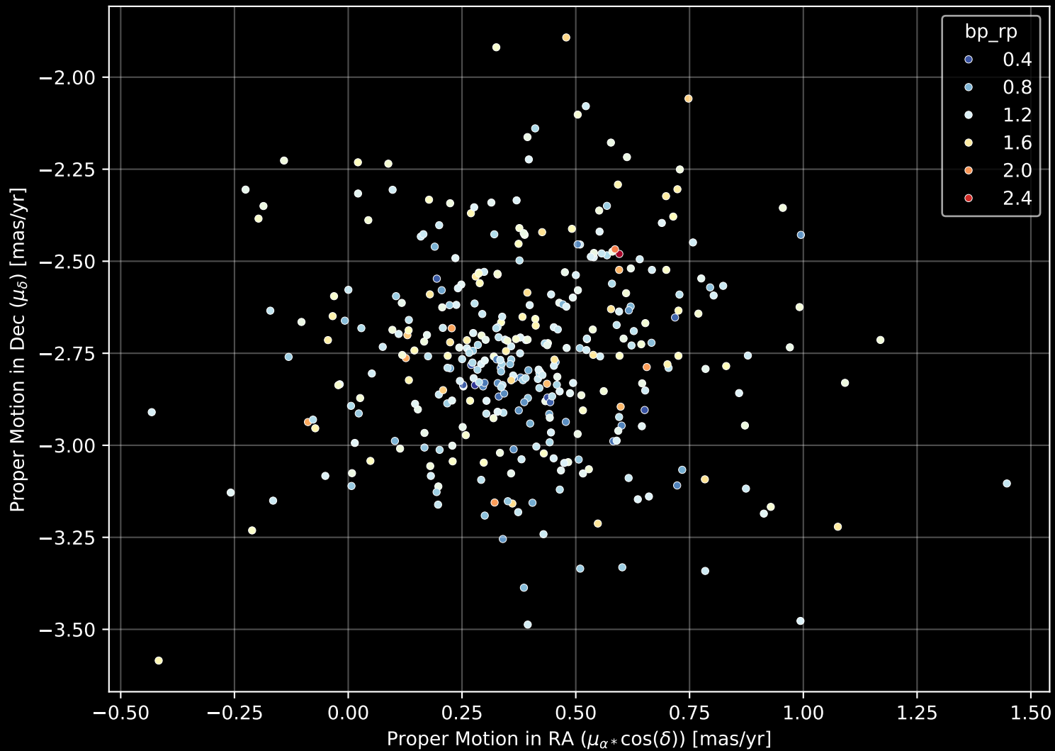
Gaia Cluster: [COIN-Gaia_40] Proper Motion Diagram (n= 360)
