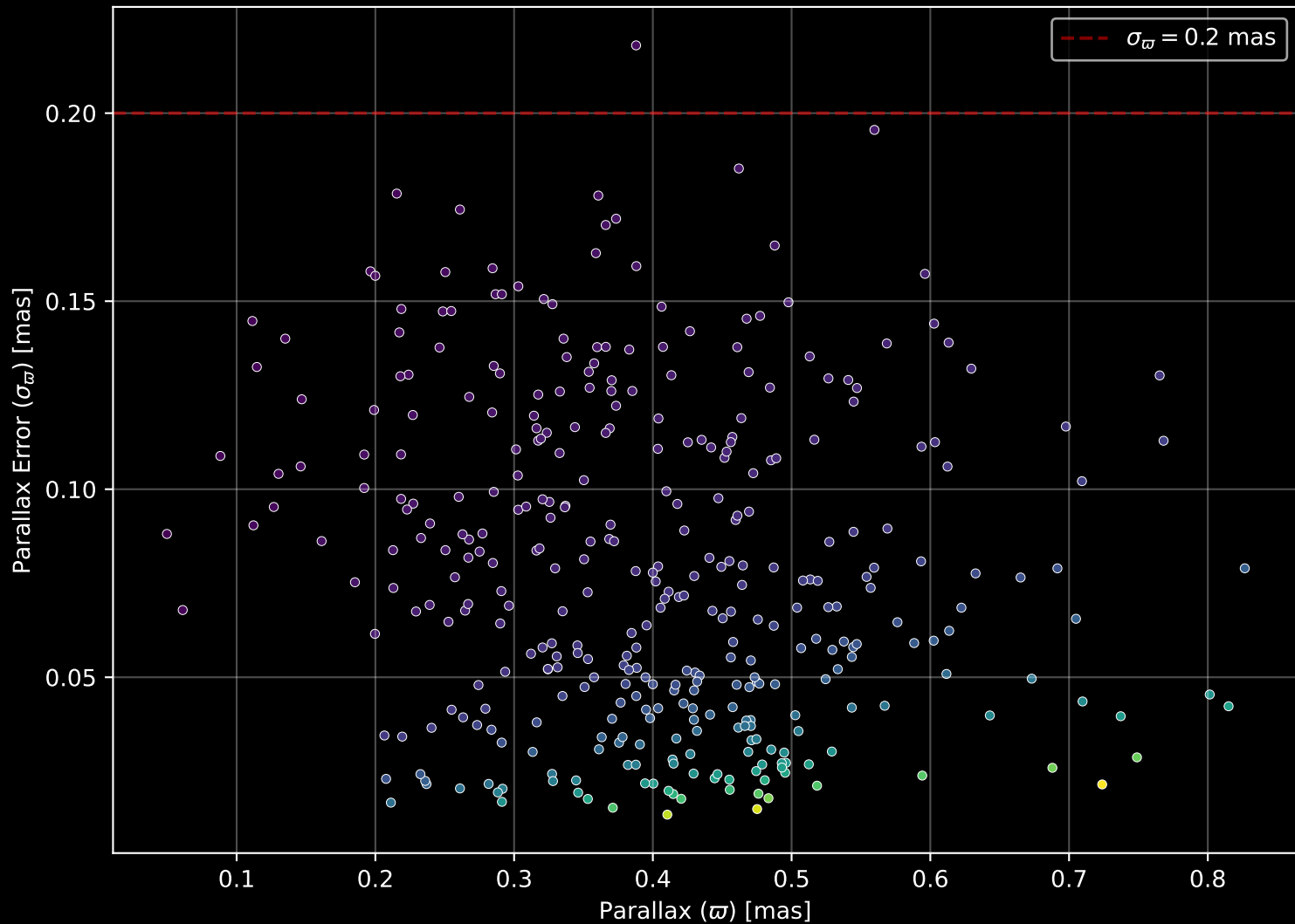
Gaia Cluster: [COIN-Gaia_40] Parallax Quality (n= 360)
