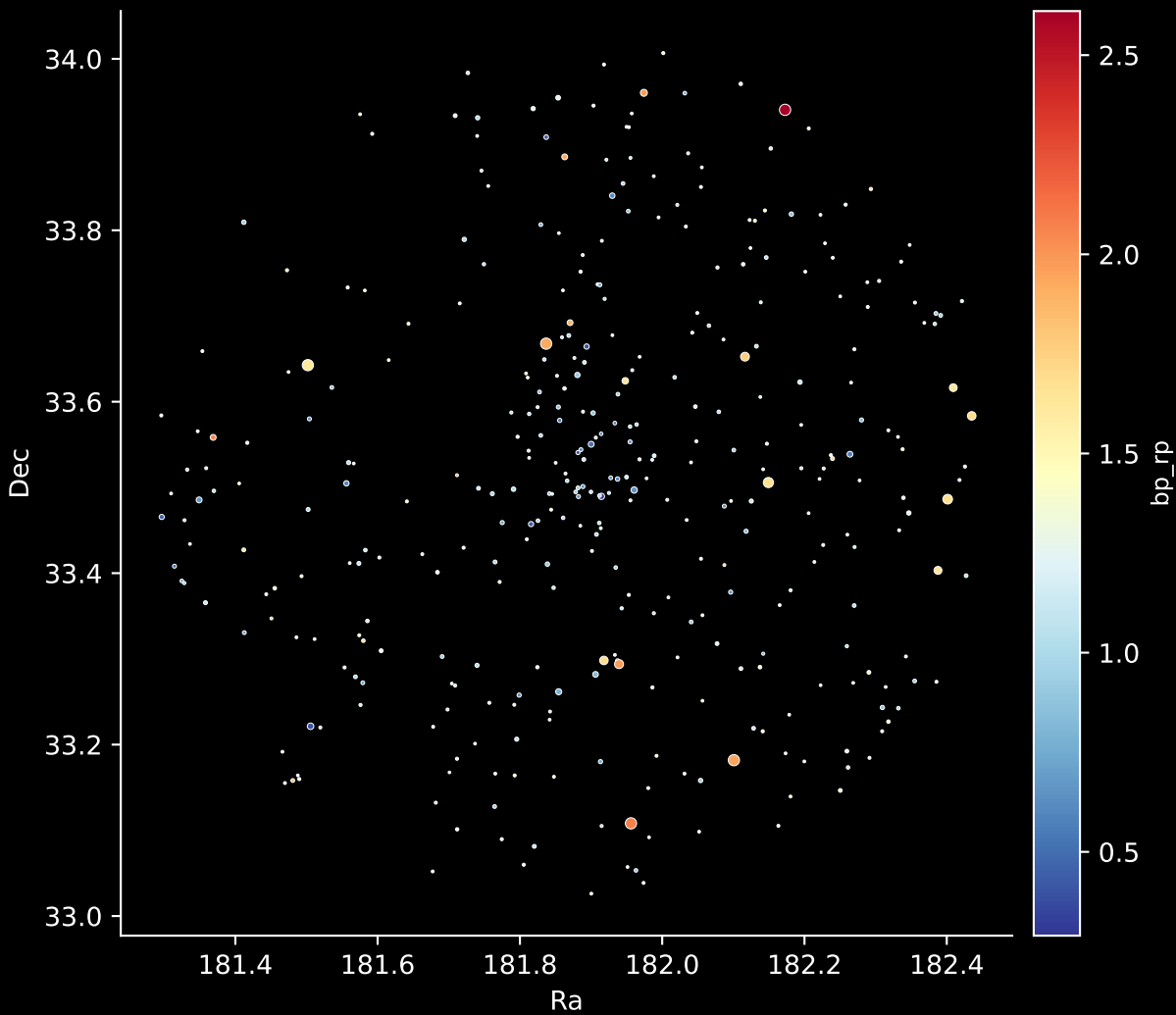
Gaia Cluster: [COIN-Gaia_40] Stars: 360
