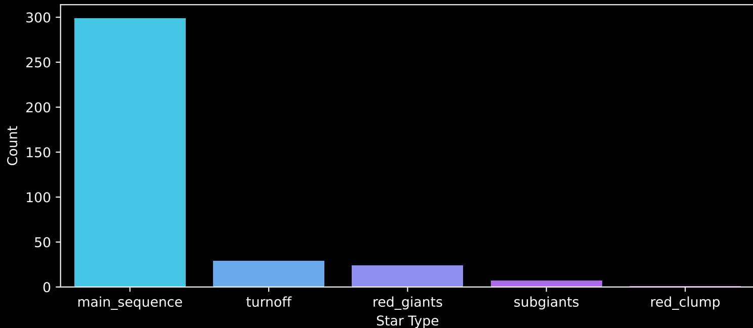
Gaia Cluster: [COIN-Gaia_40] Count plot of Star Type
