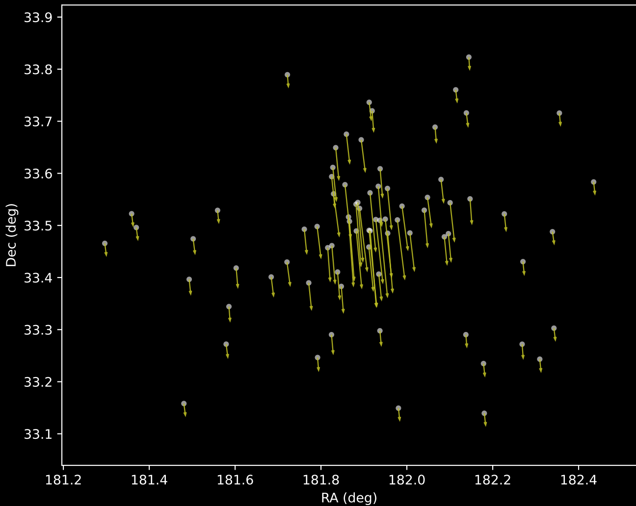
Gaia DR3 Cluster 16 Proper Motion Vectors (n=76)
