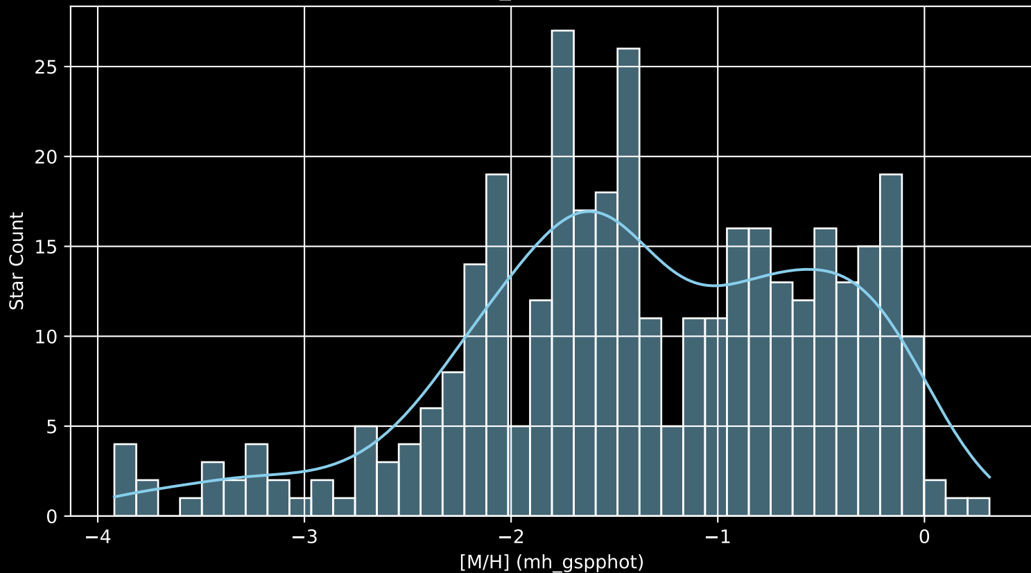
Gaia Cluster: [COIN-Gaia_40 [M/H] (mh_gspphot) (n= 358)
