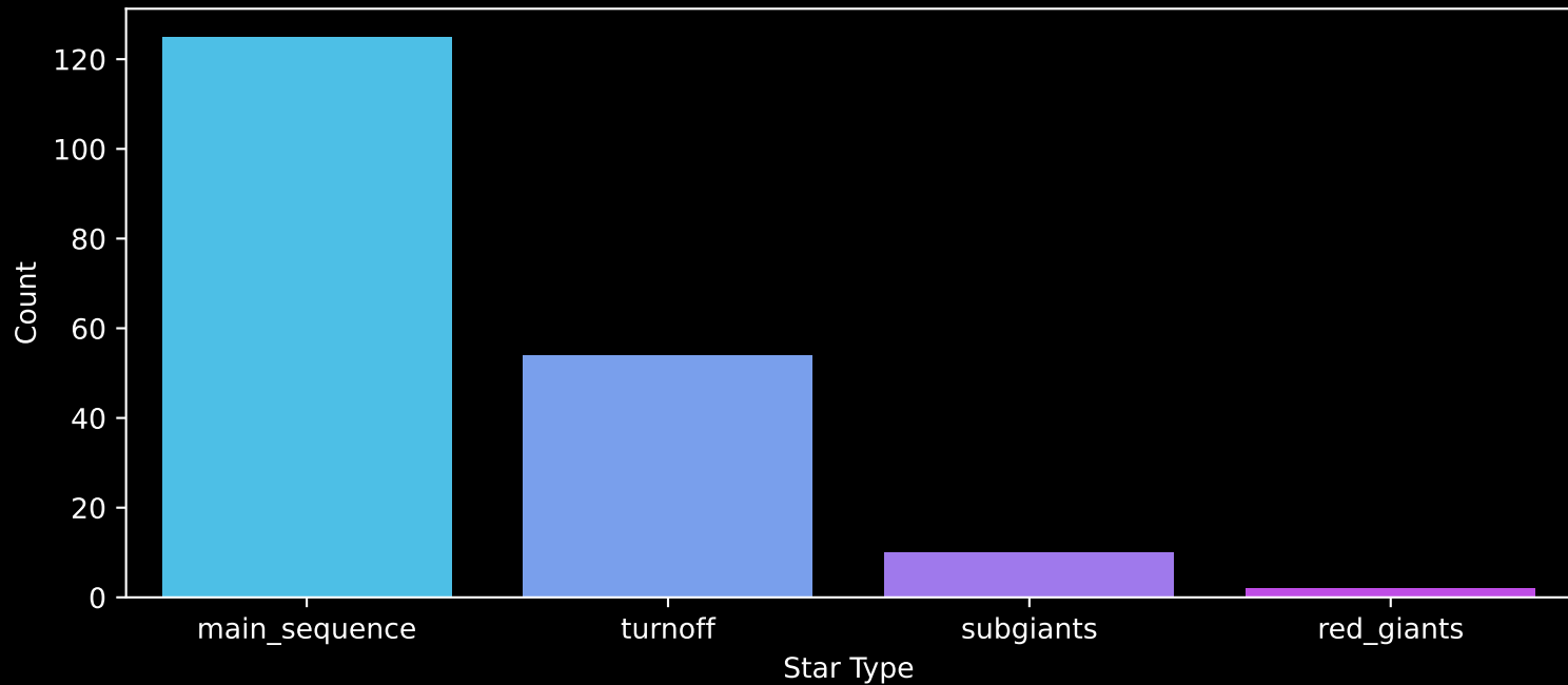
Gaia Cluster: [Collinder_106] Count plot of Star Type
