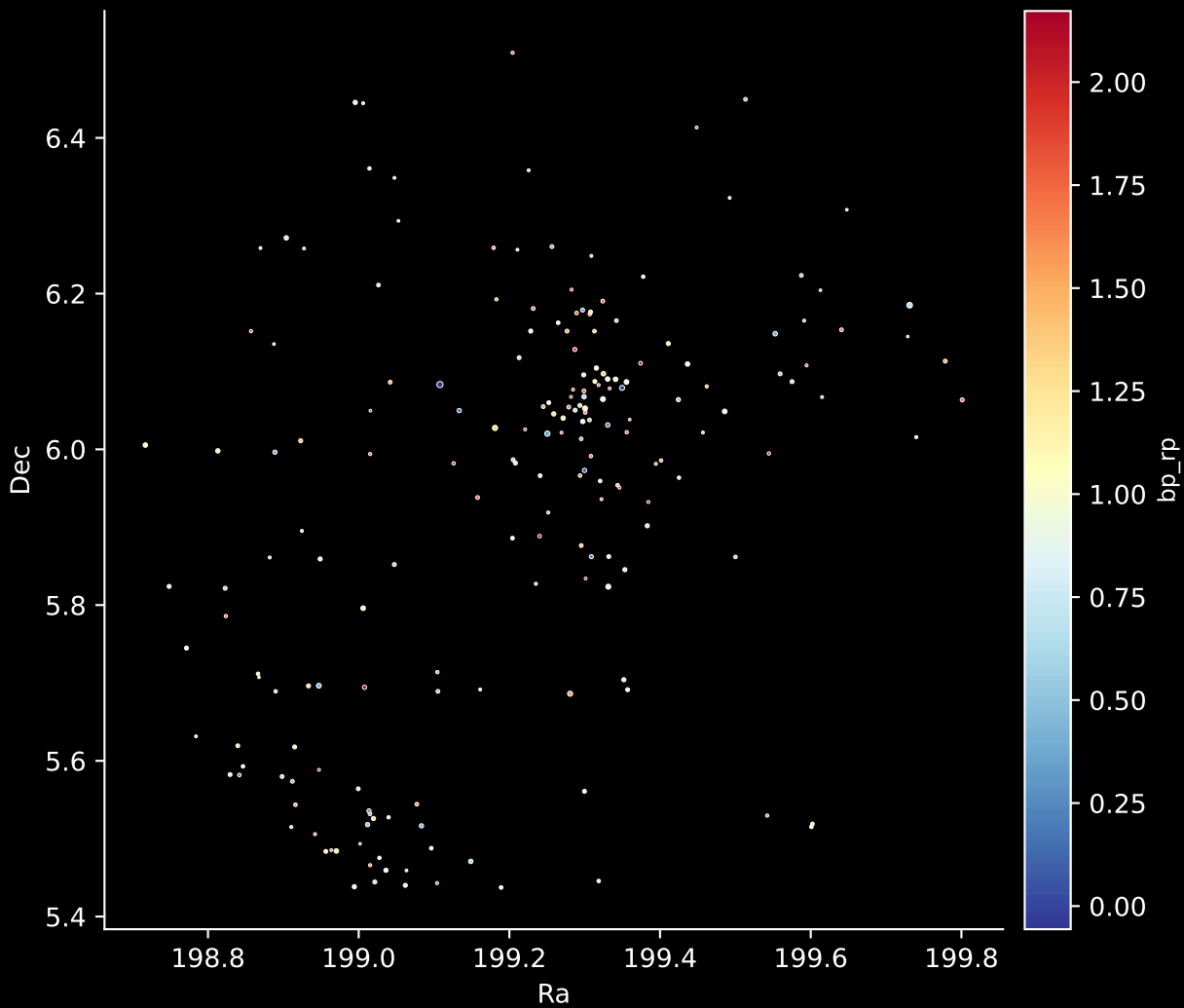
Gaia Cluster: [Collinder_106] Stars: 191
