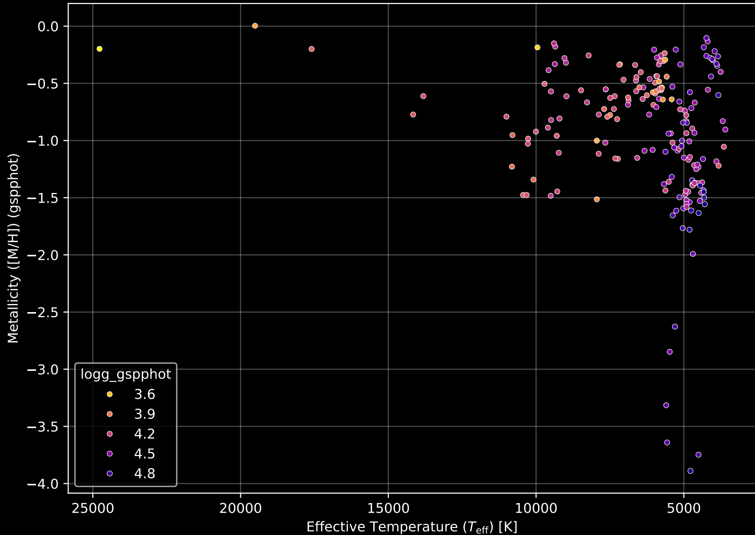
Gaia Cluster: [Collinder_106] Stellar Population Parameters (n= 191)
