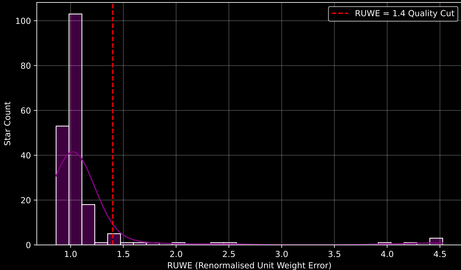
Gaia Cluster: [Collinder_106] RUWE Distribution (n= 191)
