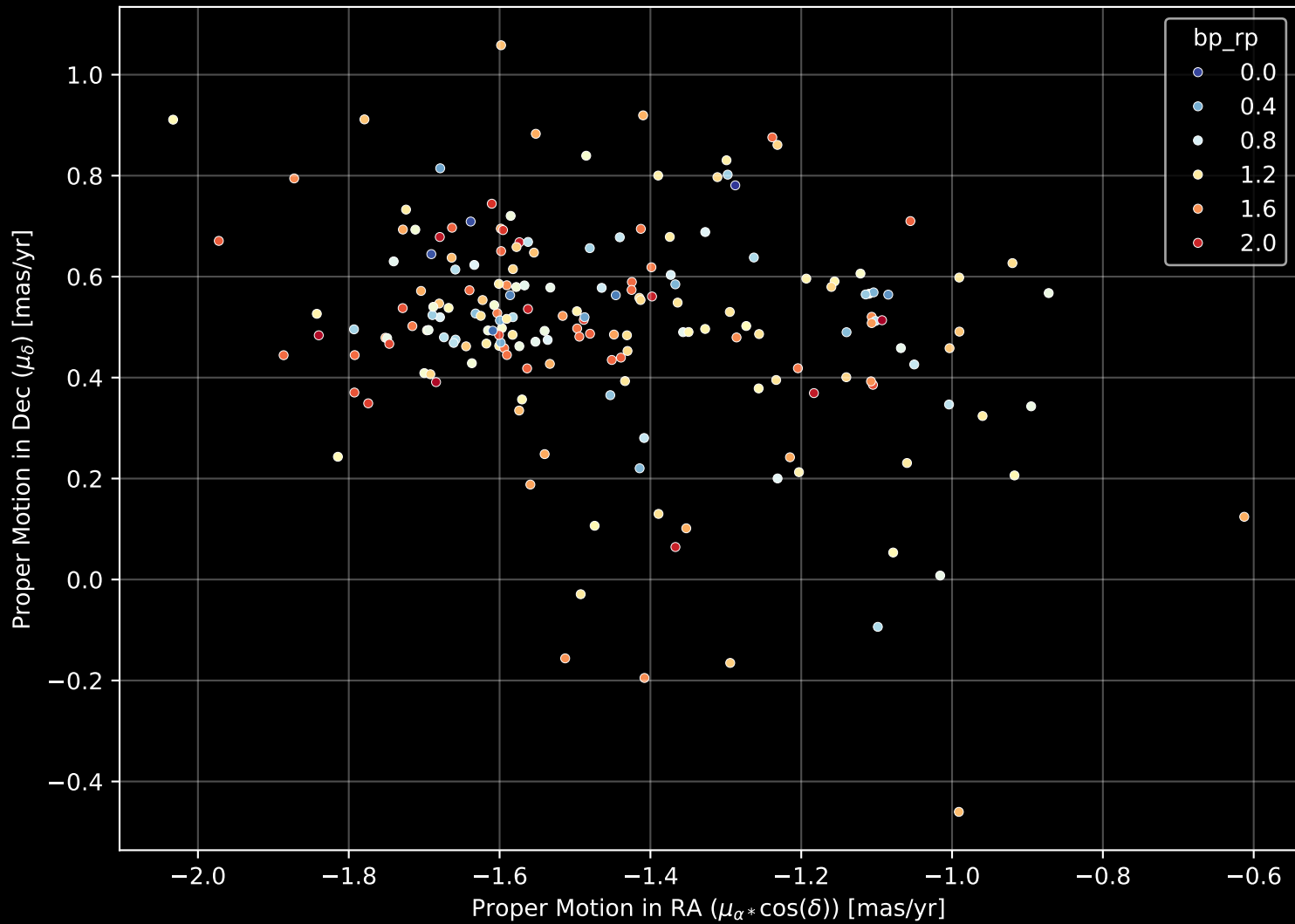
Gaia Cluster: [Collinder_106] Proper Motion Diagram (n= 191)
