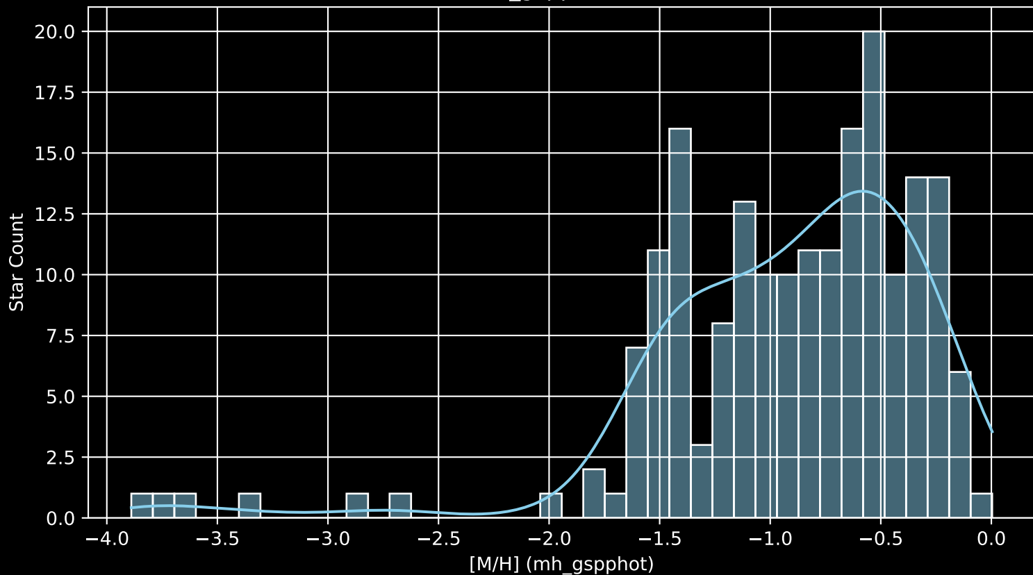
Gaia Cluster: [Collinder_106 [M/H] (mh_gspphot) (n= 191)
