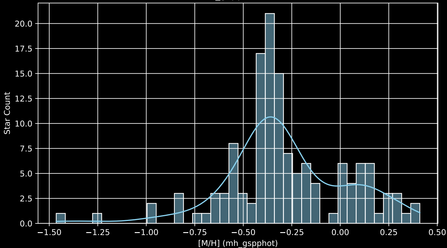
Gaia Cluster: [Collinder_140 [M/H] (mh_gspphot) (n= 136)
