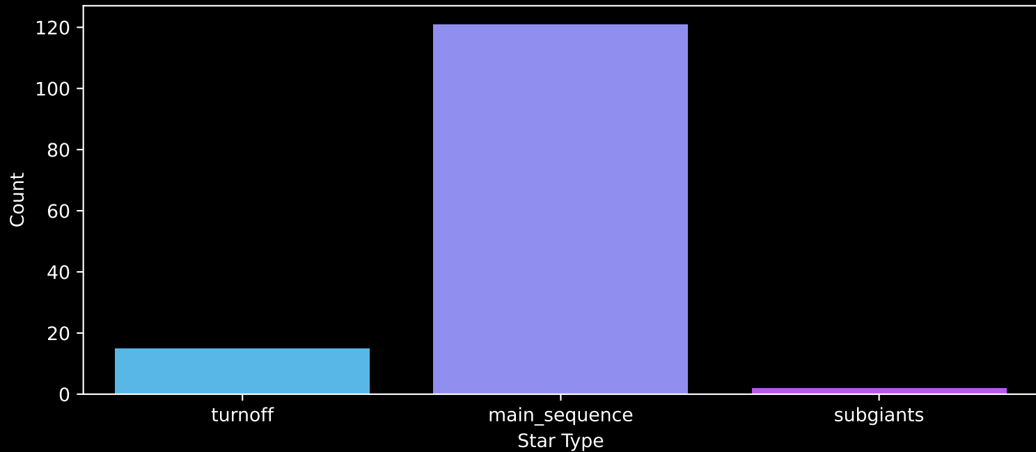
Gaia Cluster: [Collinder_140] Count plot of Star Type
