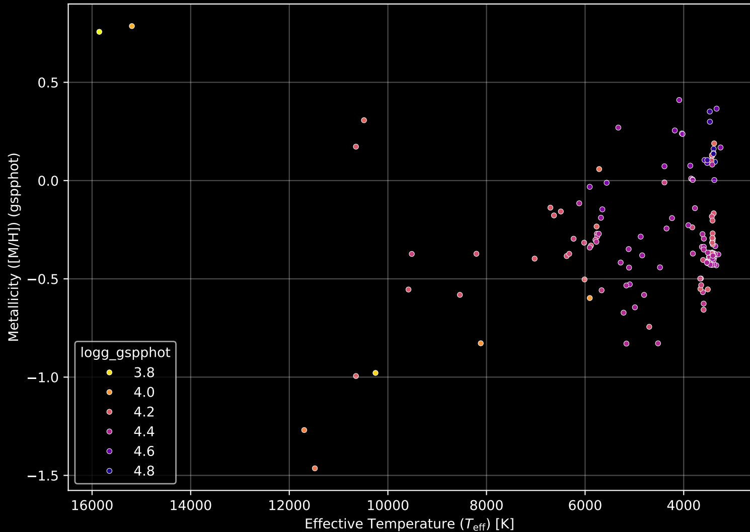
Gaia Cluster: [Collinder_140] Stellar Population Parameters (n= 138)
