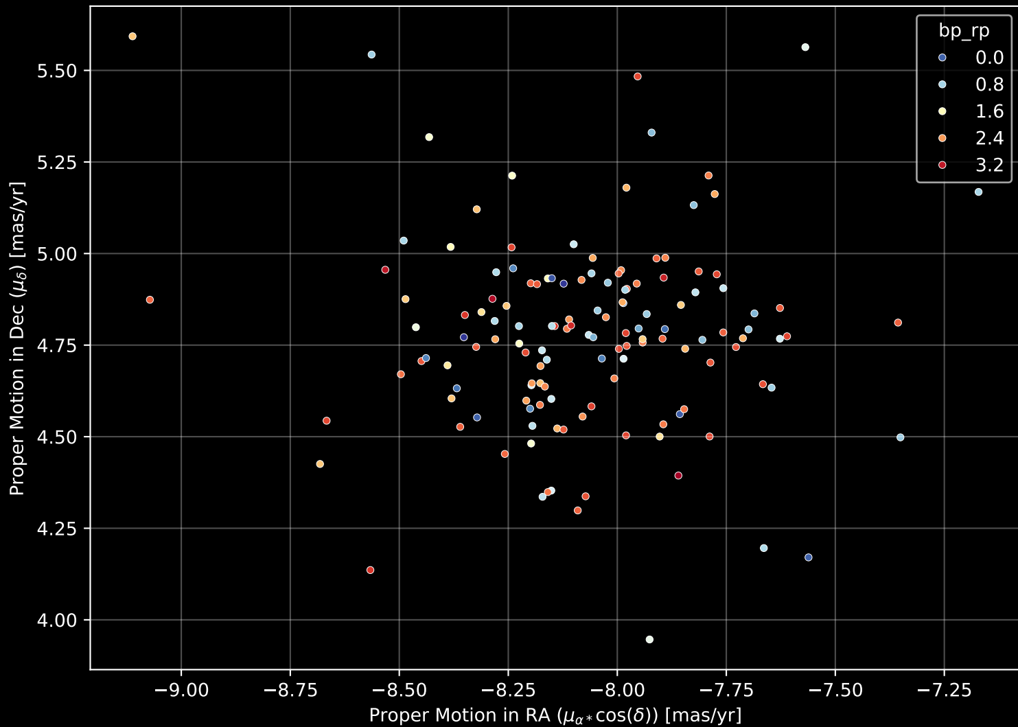
Gaia Cluster: [Collinder_140] Proper Motion Diagram (n= 138)
