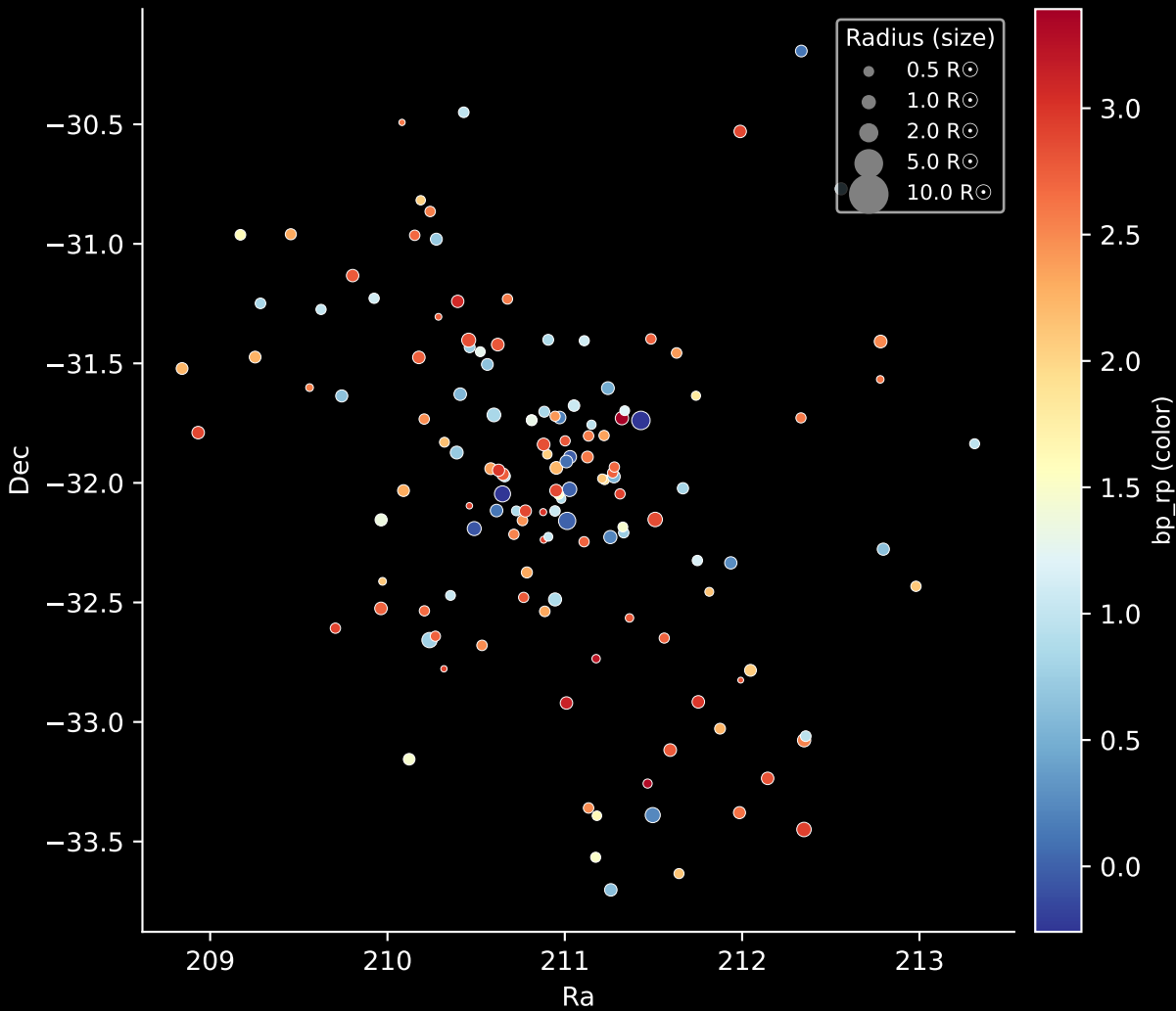
Gaia Cluster: [Collinder_140] Stars: 138
