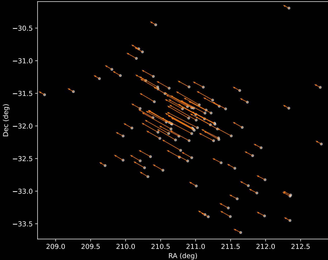
Gaia DR3 Cluster 2 Proper Motion Vectors (n=97)
