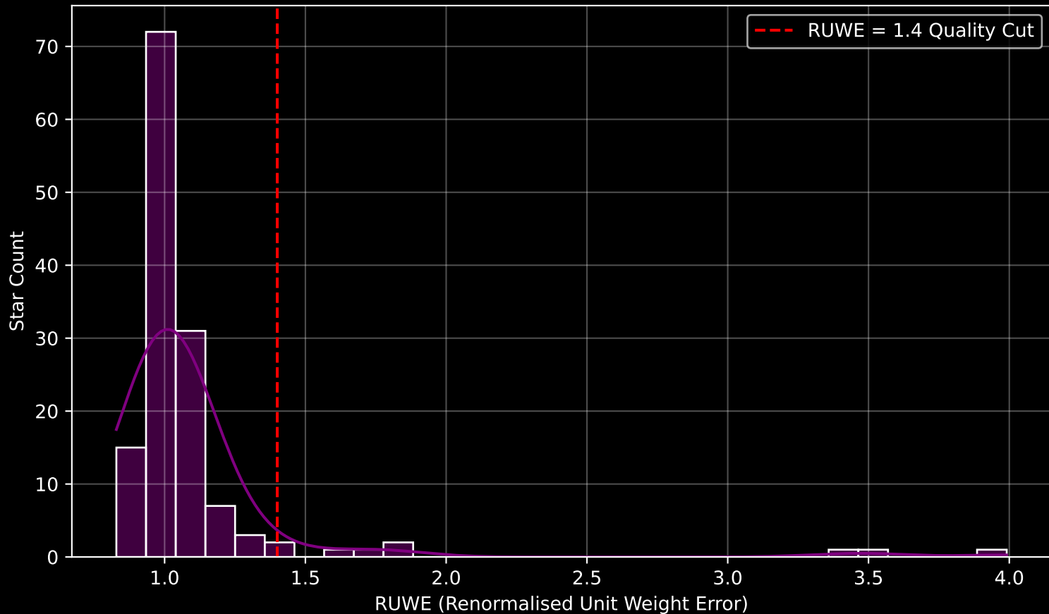
Gaia Cluster: [Collinder_140] RUWE Distribution (n= 137)
