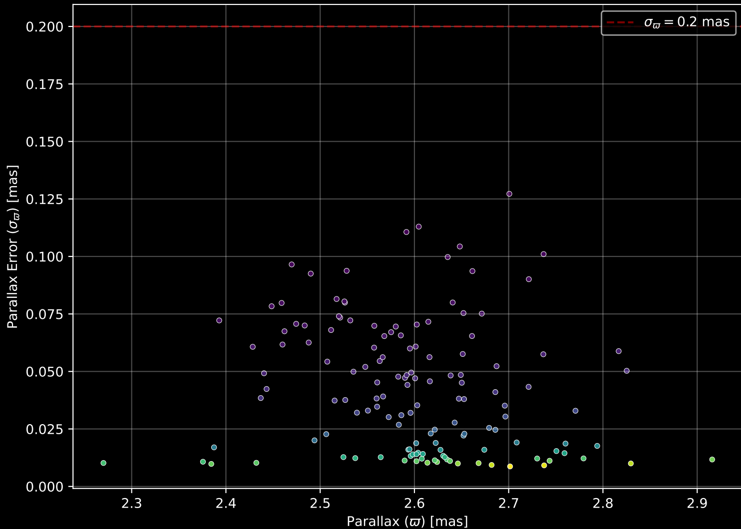
Gaia Cluster: [Collinder_140] Parallax Quality (n= 138)
