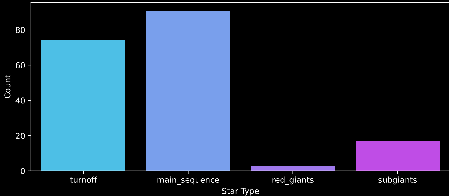
Gaia Cluster: [Collinder_197] Count plot of Star Type
