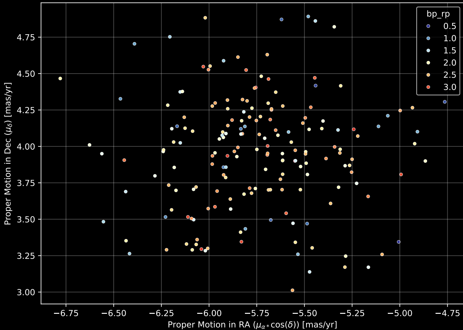
Gaia Cluster: [Collinder_197] Proper Motion Diagram (n= 185)
