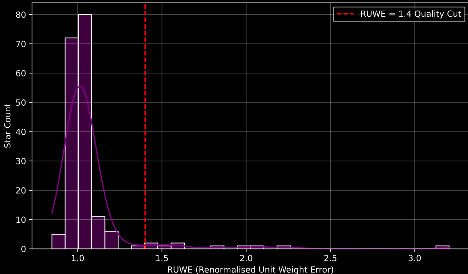
Gaia Cluster: [Collinder_197] RUWE Distribution (n= 185)
