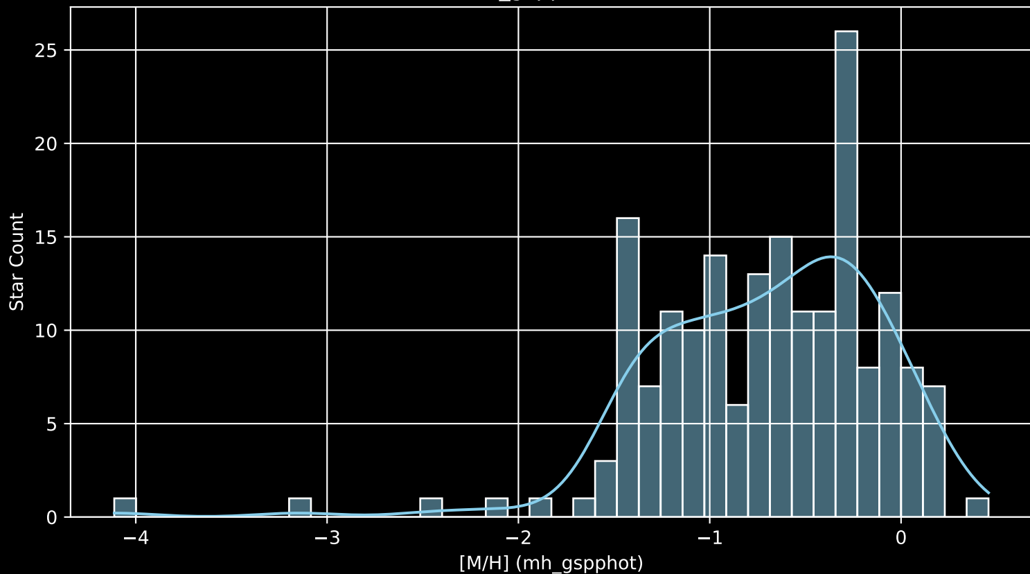
Gaia Cluster: [Collinder_197 [M/H] (mh_gspphot) (n= 185)
