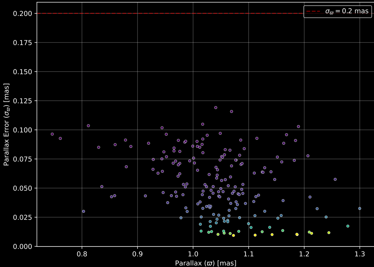
Gaia Cluster: [Collinder_197] Parallax Quality (n= 185)
