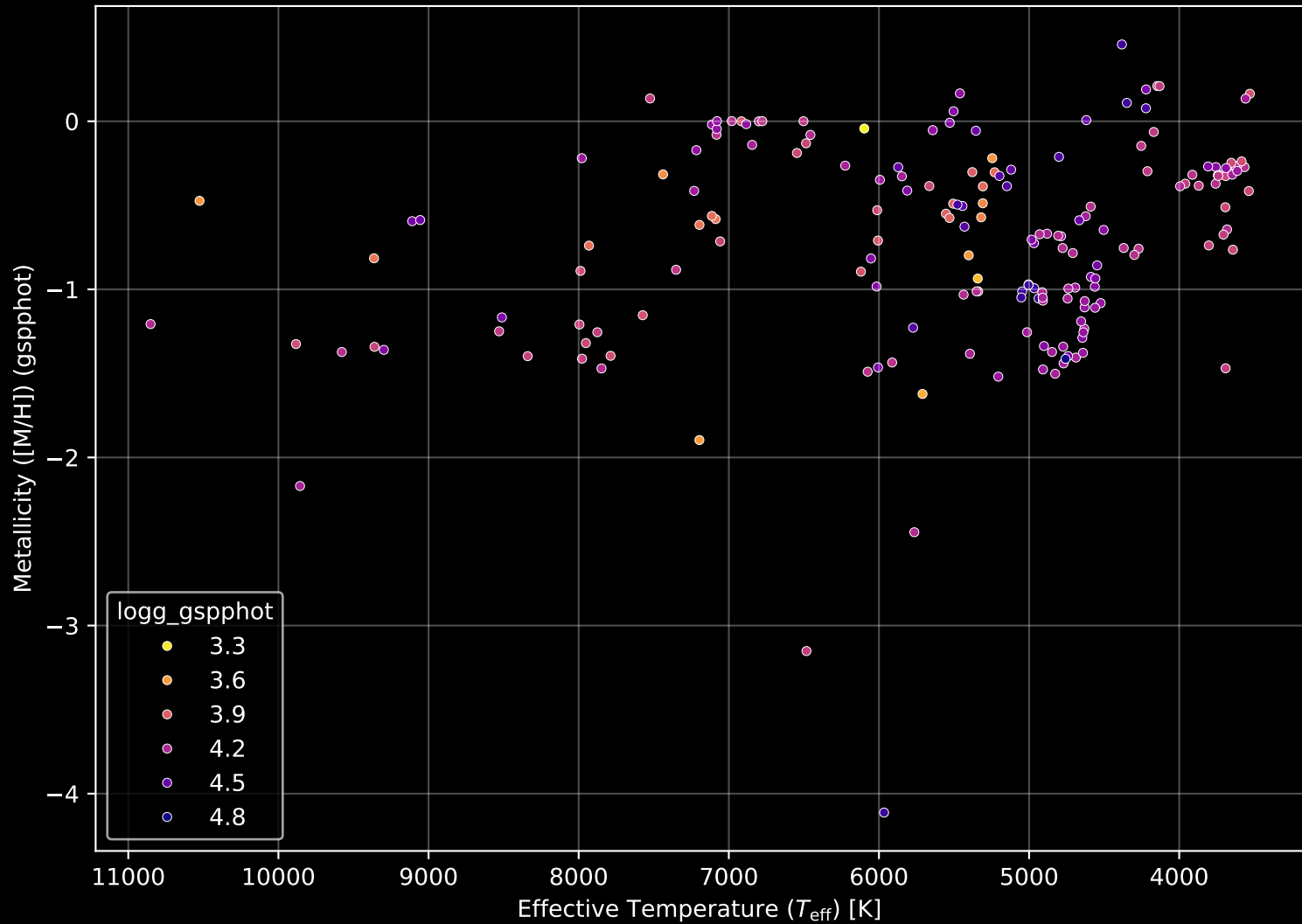
Gaia Cluster: [Collinder_197] Stellar Population Parameters (n= 185)
