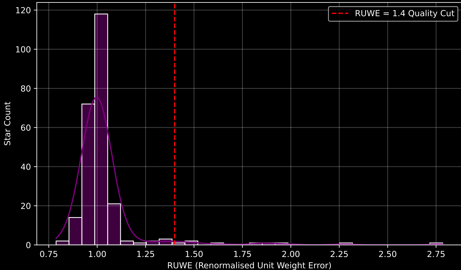
Gaia Cluster: [Collinder_220] RUWE Distribution (n= 244)
