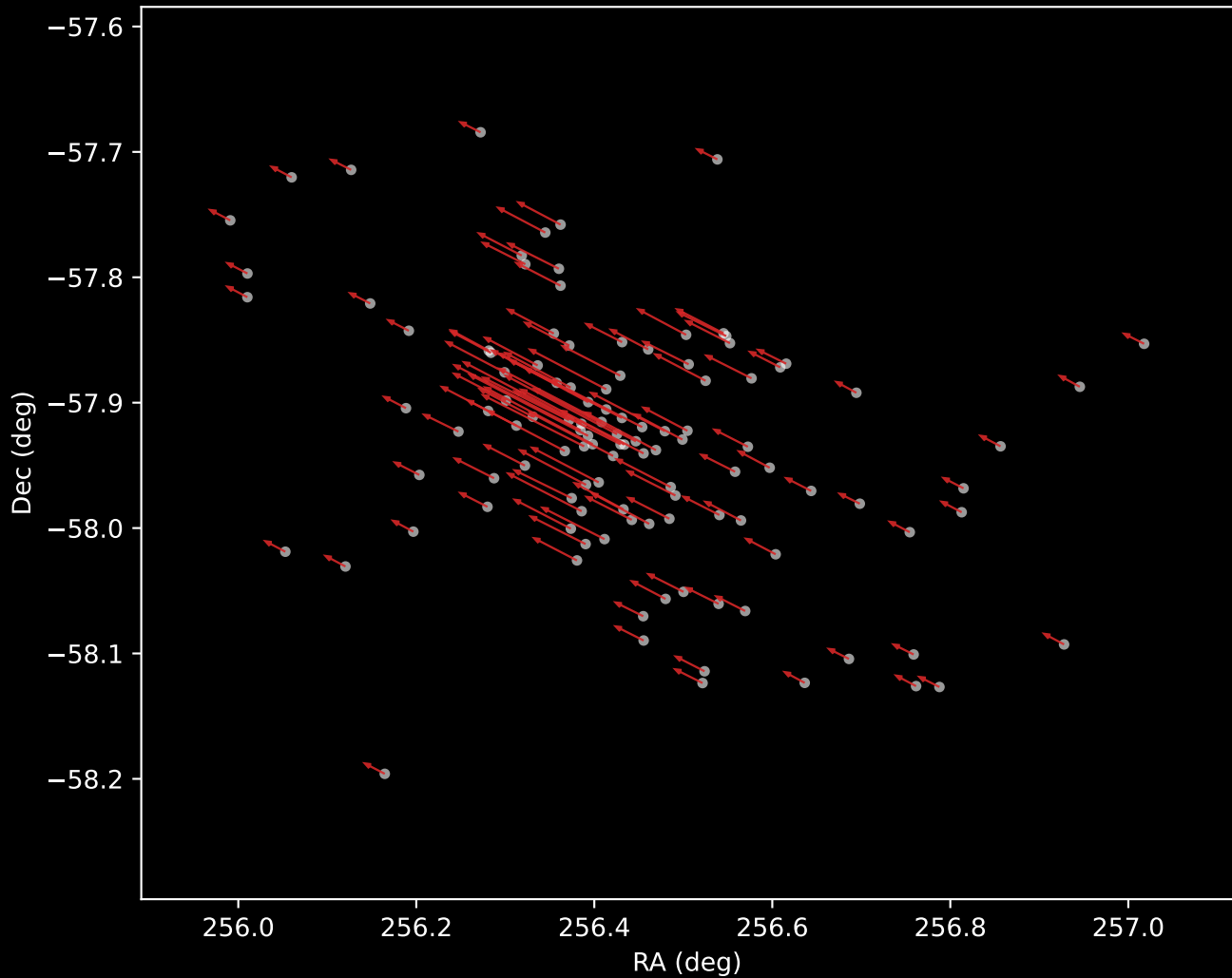
Gaia DR3 Cluster 6 Proper Motion Vectors (n=115)
