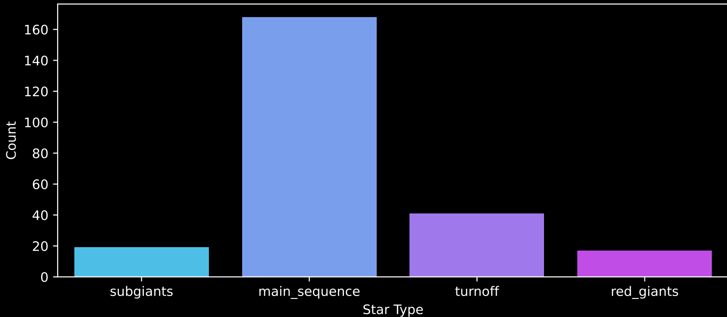
Gaia Cluster: [Collinder_220] Count plot of Star Type
