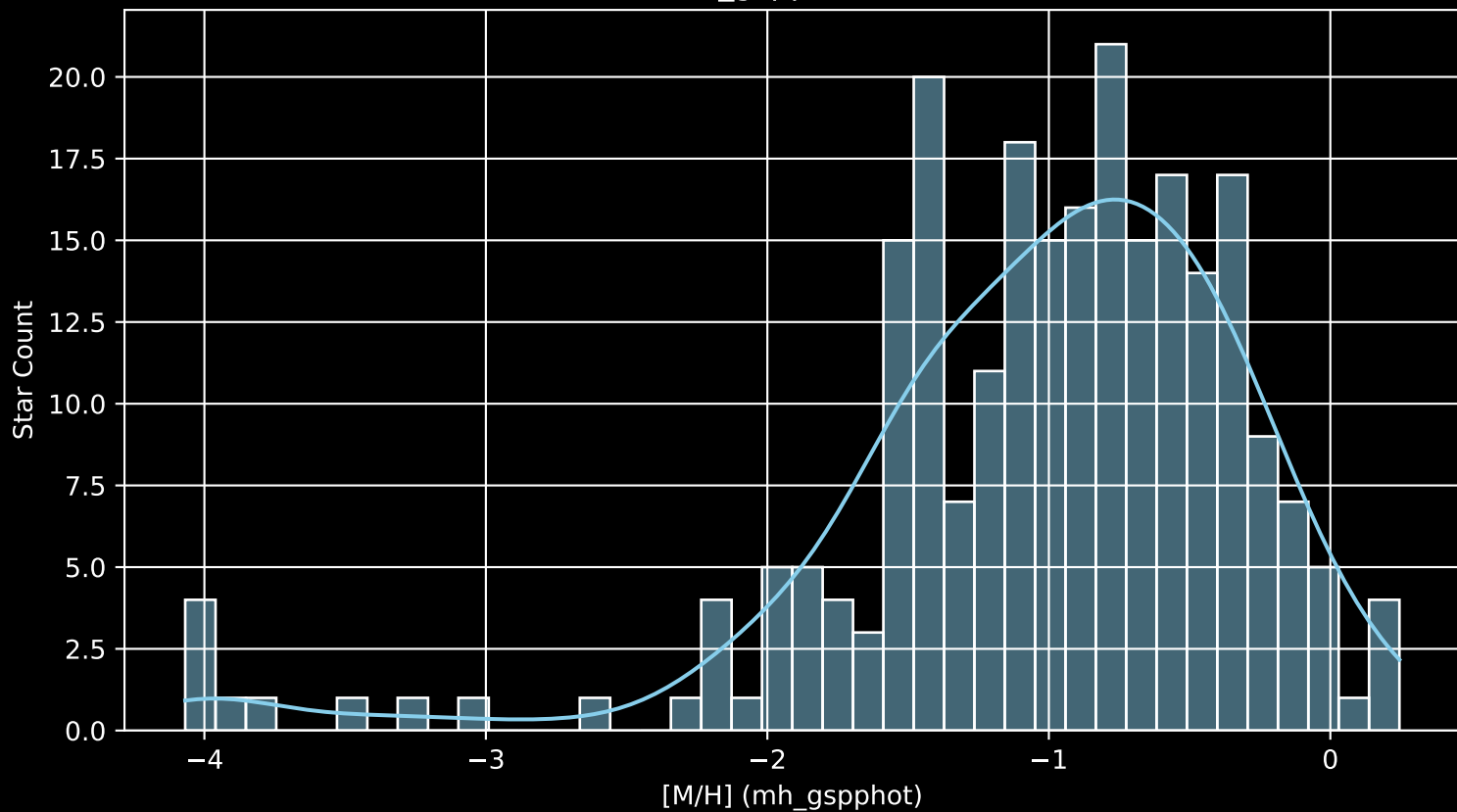
Gaia Cluster: [Collinder_220 [M/H] (mh_gspphot) (n= 245)
