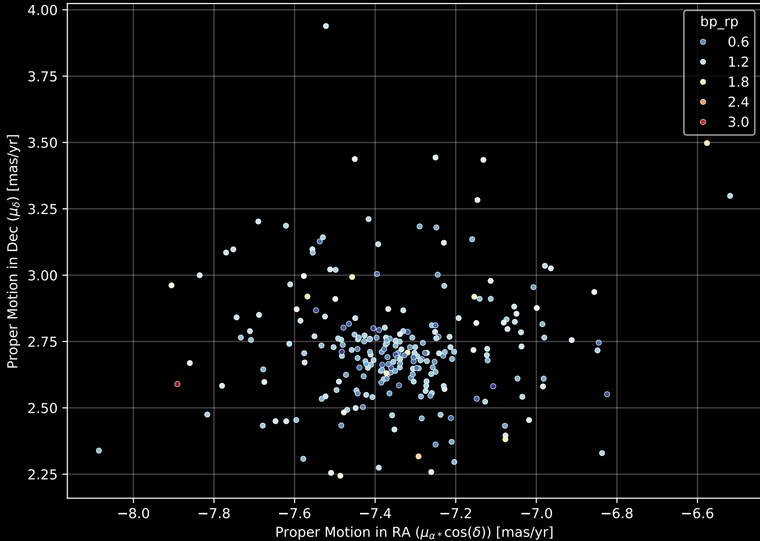
Gaia Cluster: [Collinder_220] Proper Motion Diagram (n= 245)
