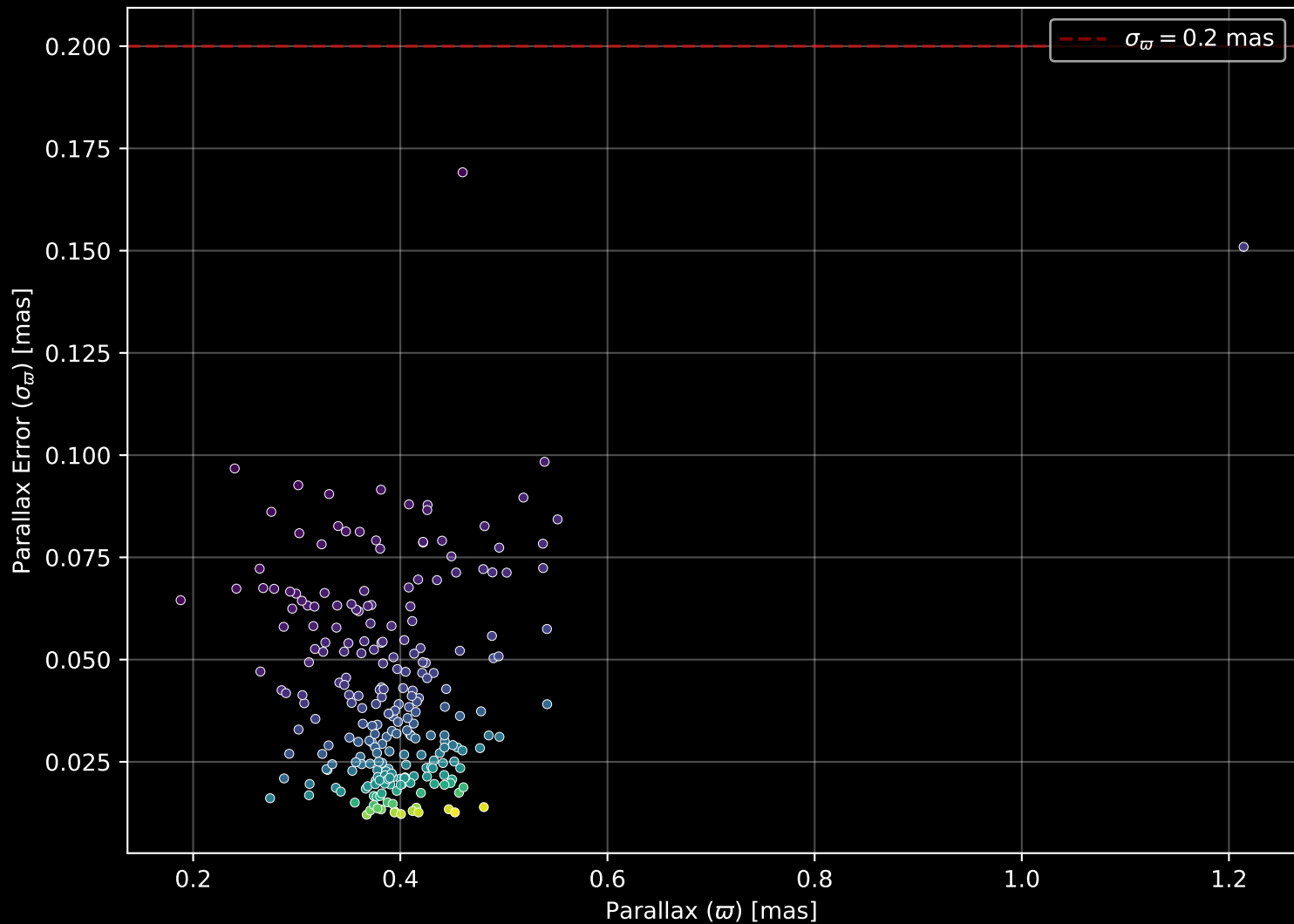
Gaia Cluster: [Collinder_220] Parallax Quality (n= 245)
