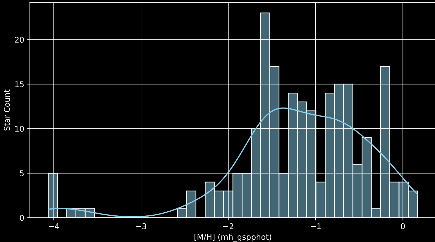
Gaia Cluster: [Collinder_268 [M/H] (mh_gspphot) (n= 218)
