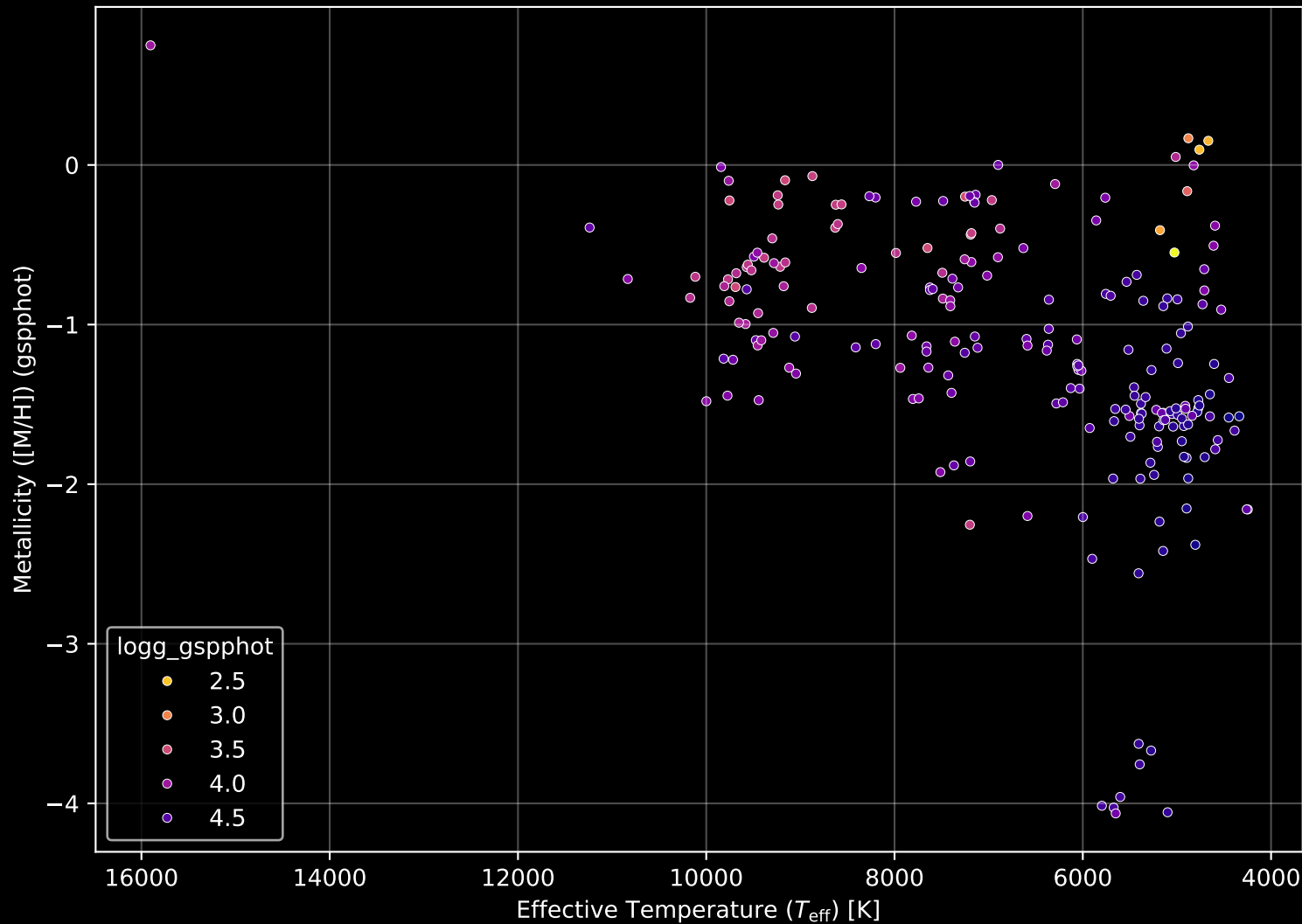
Gaia Cluster: [Collinder_268] Stellar Population Parameters (n= 219)
