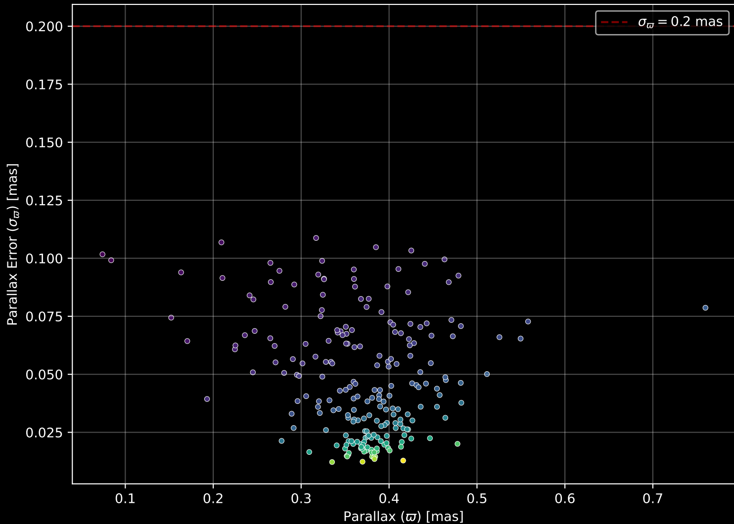
Gaia Cluster: [Collinder_268] Parallax Quality (n= 219)
