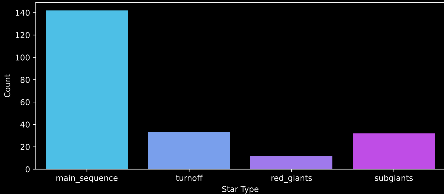
Gaia Cluster: [Collinder_268] Count plot of Star Type
