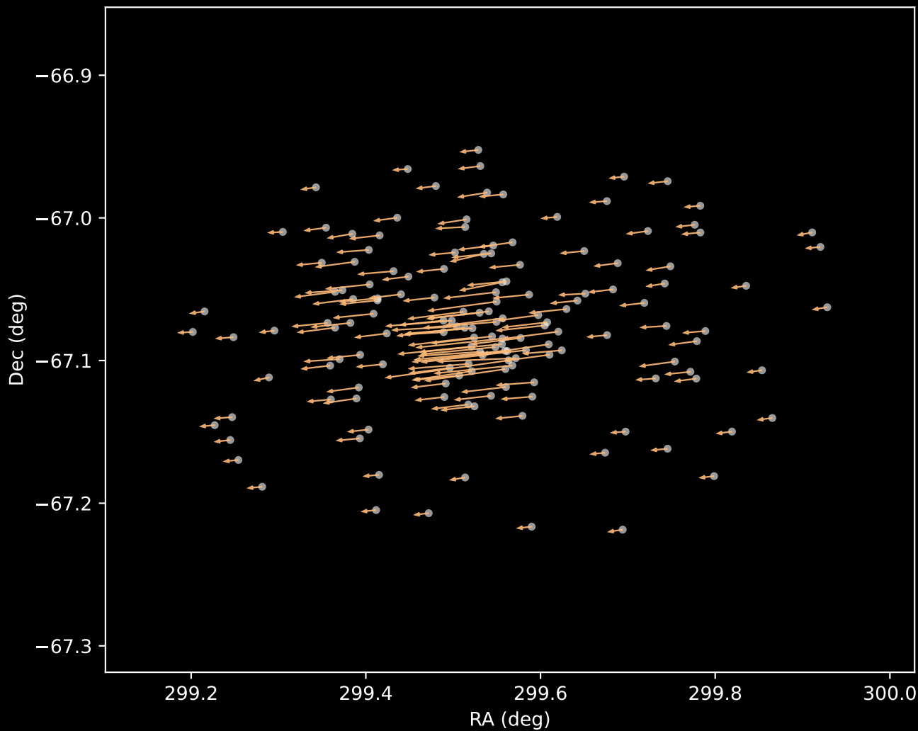
Gaia DR3 Cluster 3 Proper Motion Vectors (n=152)
