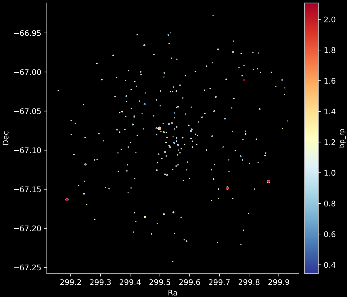
Gaia Cluster: [Collinder_268] Stars: 219
