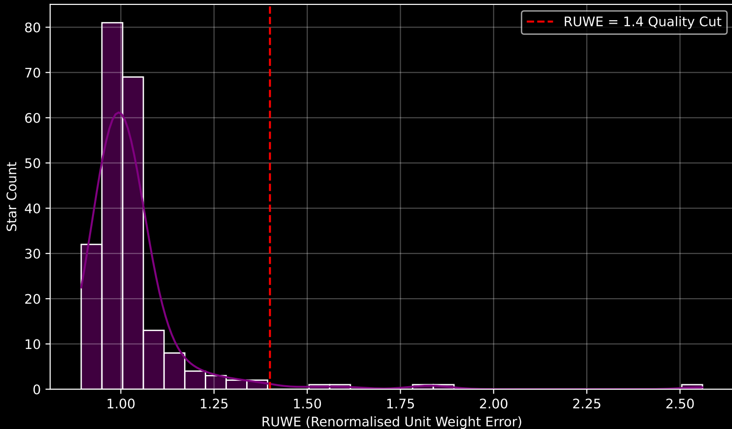
Gaia Cluster: [Collinder_268] RUWE Distribution (n= 219)
