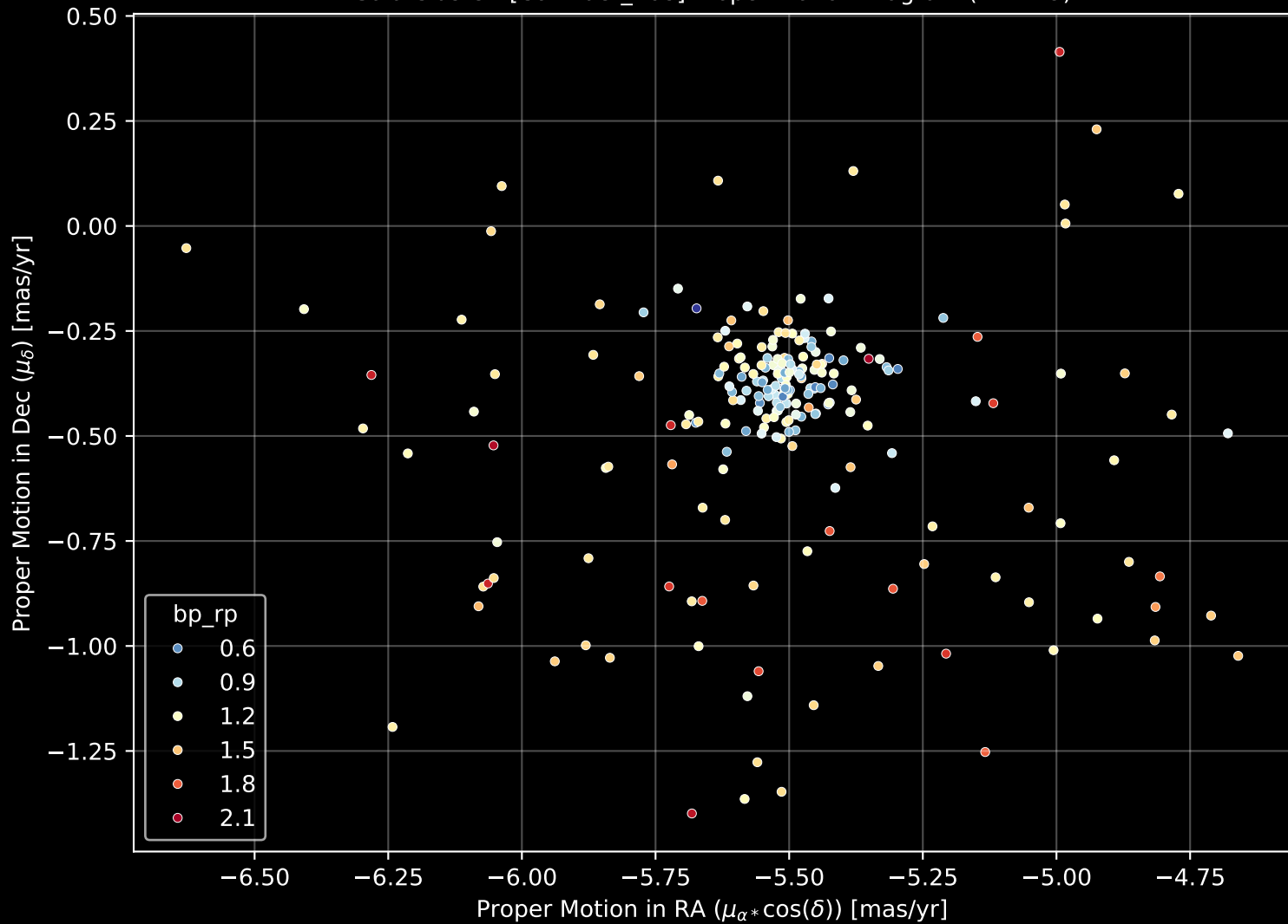
Gaia Cluster: [Collinder_268] Proper Motion Diagram (n= 219)
