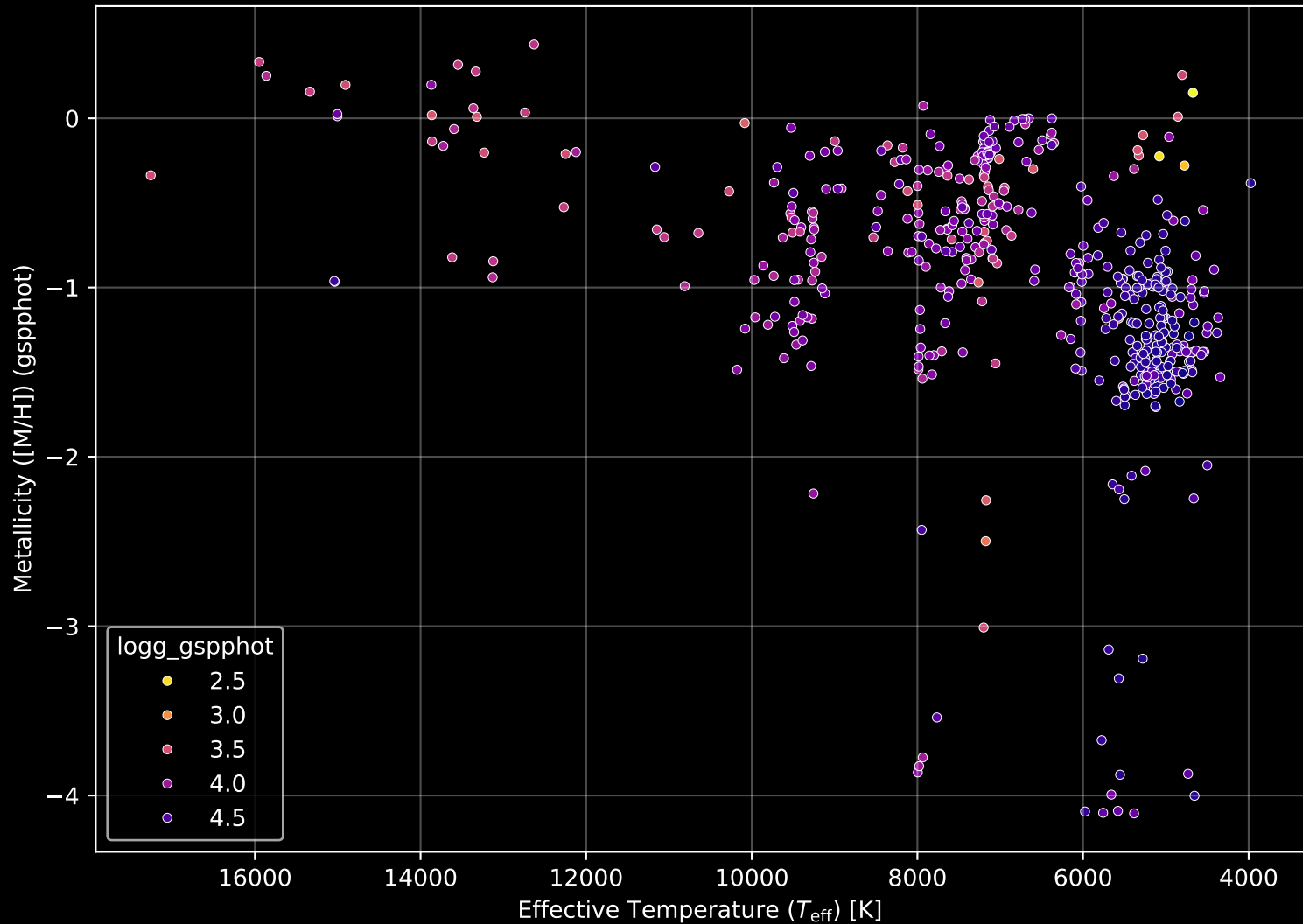
Gaia Cluster: [Collinder_272] Stellar Population Parameters (n= 513)
