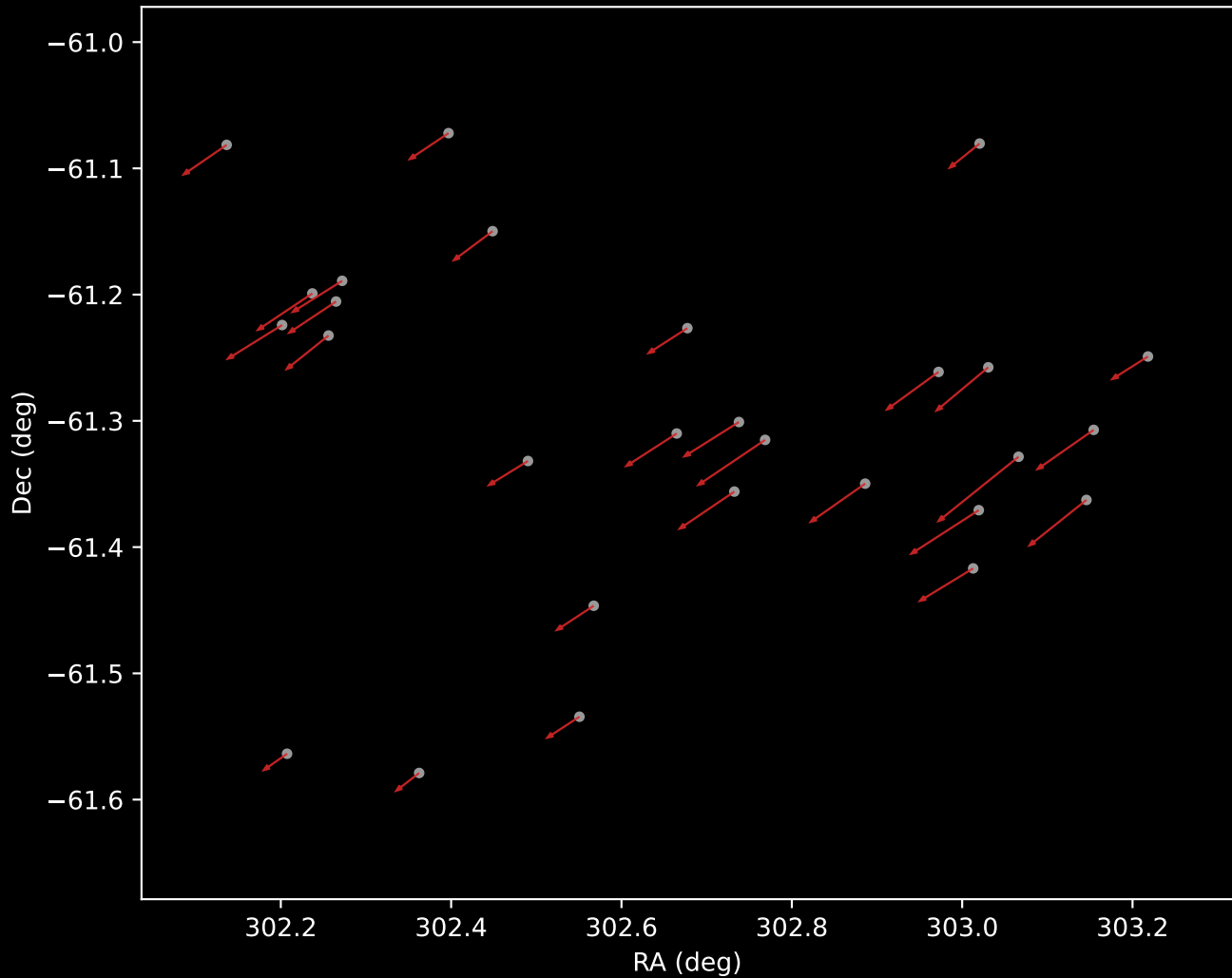
Gaia DR3 Cluster 6 Proper Motion Vectors (n=28)
