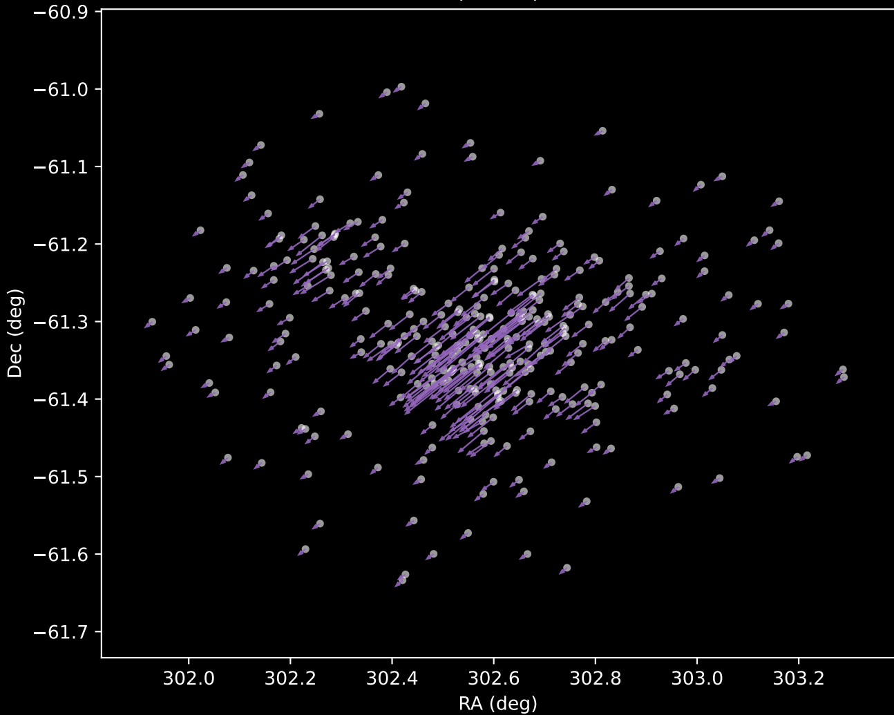
Gaia DR3 Cluster 8 Proper Motion Vectors (n=328)
