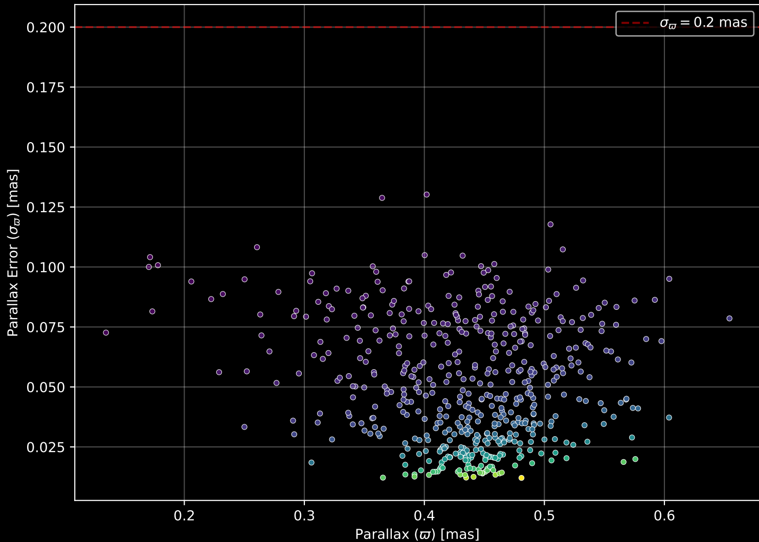
Gaia Cluster: [Collinder_272] Parallax Quality (n= 513)
