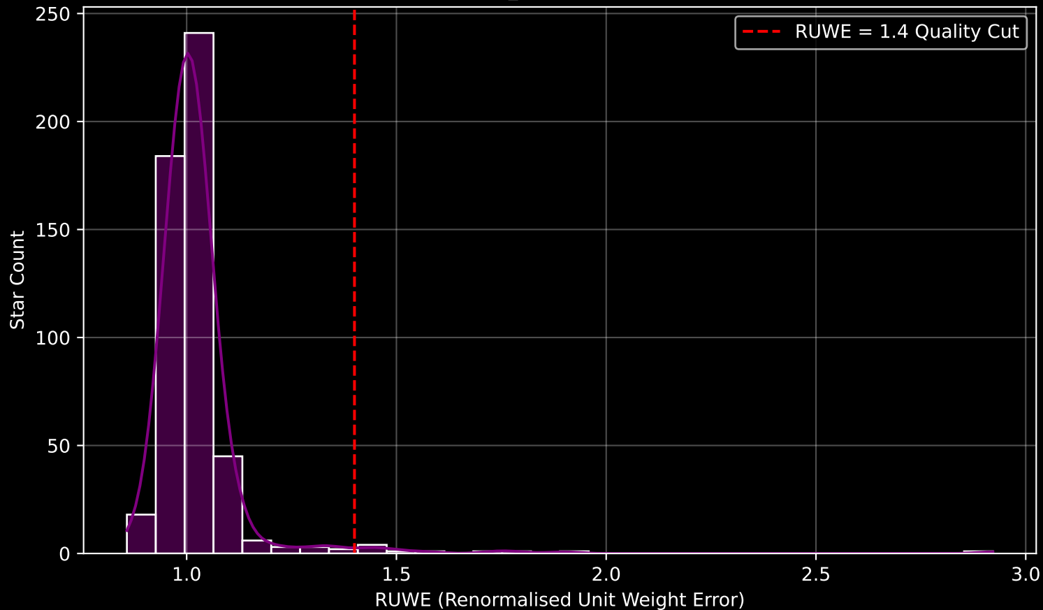
Gaia Cluster: [Collinder_272] RUWE Distribution (n= 512)
