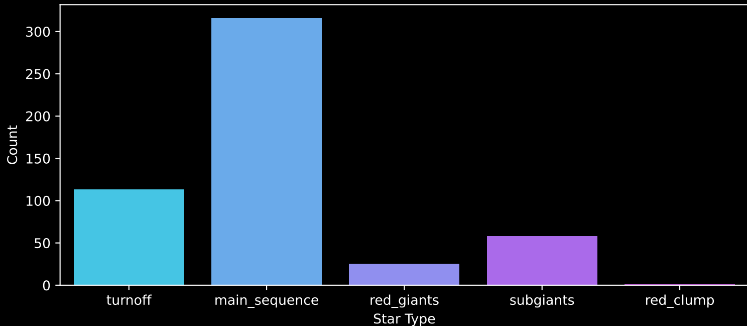
Gaia Cluster: [Collinder_272] Count plot of Star Type
