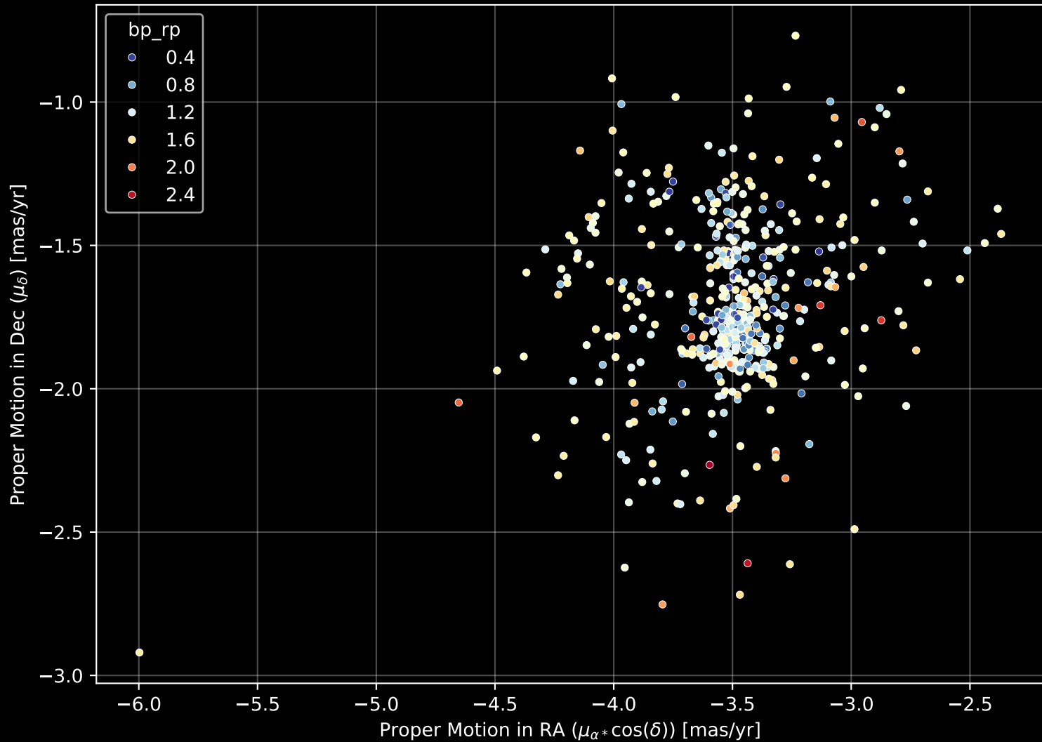
Gaia Cluster: [Collinder_272] Proper Motion Diagram (n= 513)
