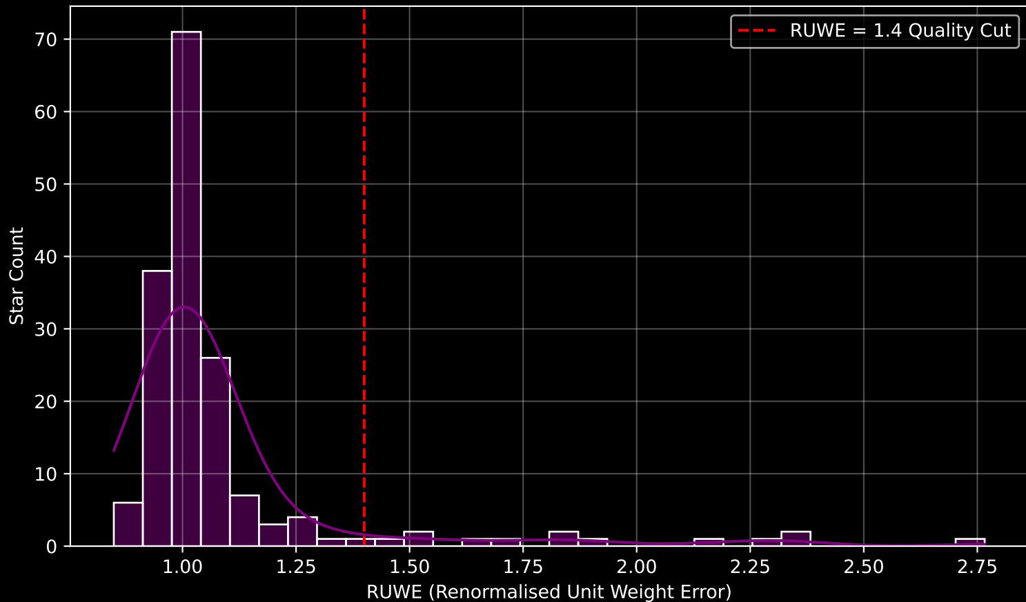
Gaia Cluster: [Collinder_350] RUWE Distribution (n= 170)
