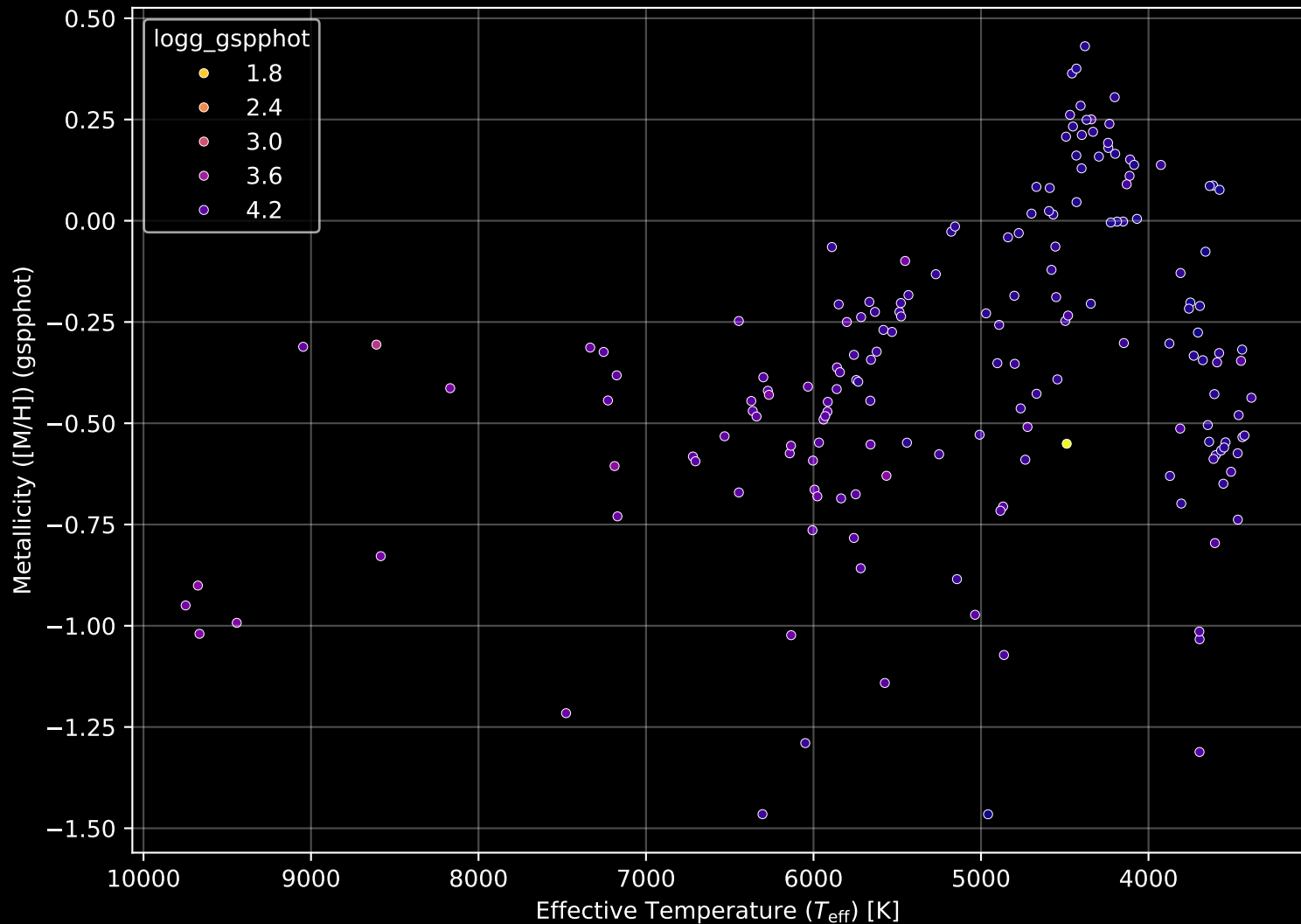
Gaia Cluster: [Collinder_350] Stellar Population Parameters (n= 175)
