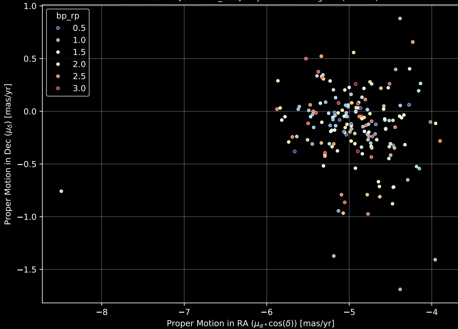
Gaia Cluster: [Collinder_350] Proper Motion Diagram (n= 175)
