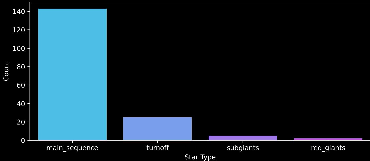
Gaia Cluster: [Collinder_350] Count plot of Star Type
