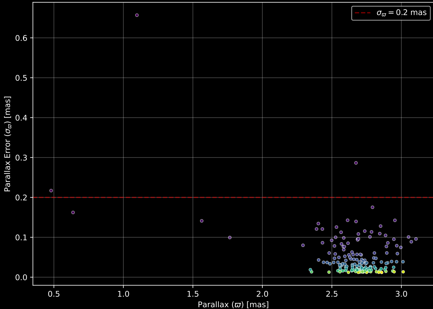
Gaia Cluster: [Collinder_350] Parallax Quality (n= 175)
