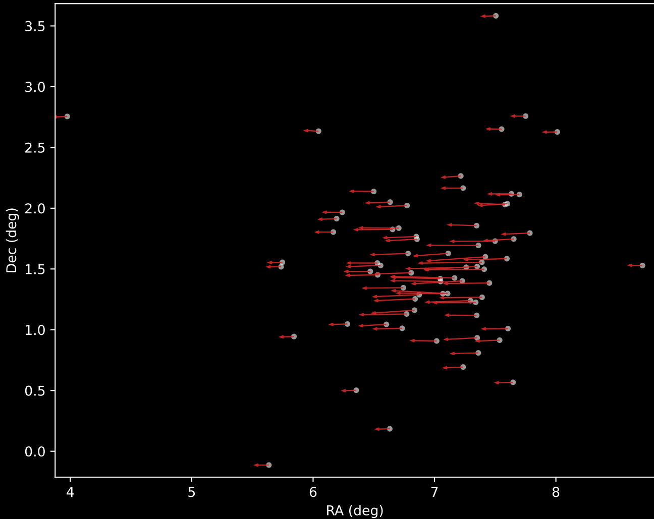
Gaia DR3 Cluster 6 Proper Motion Vectors (n=73)
