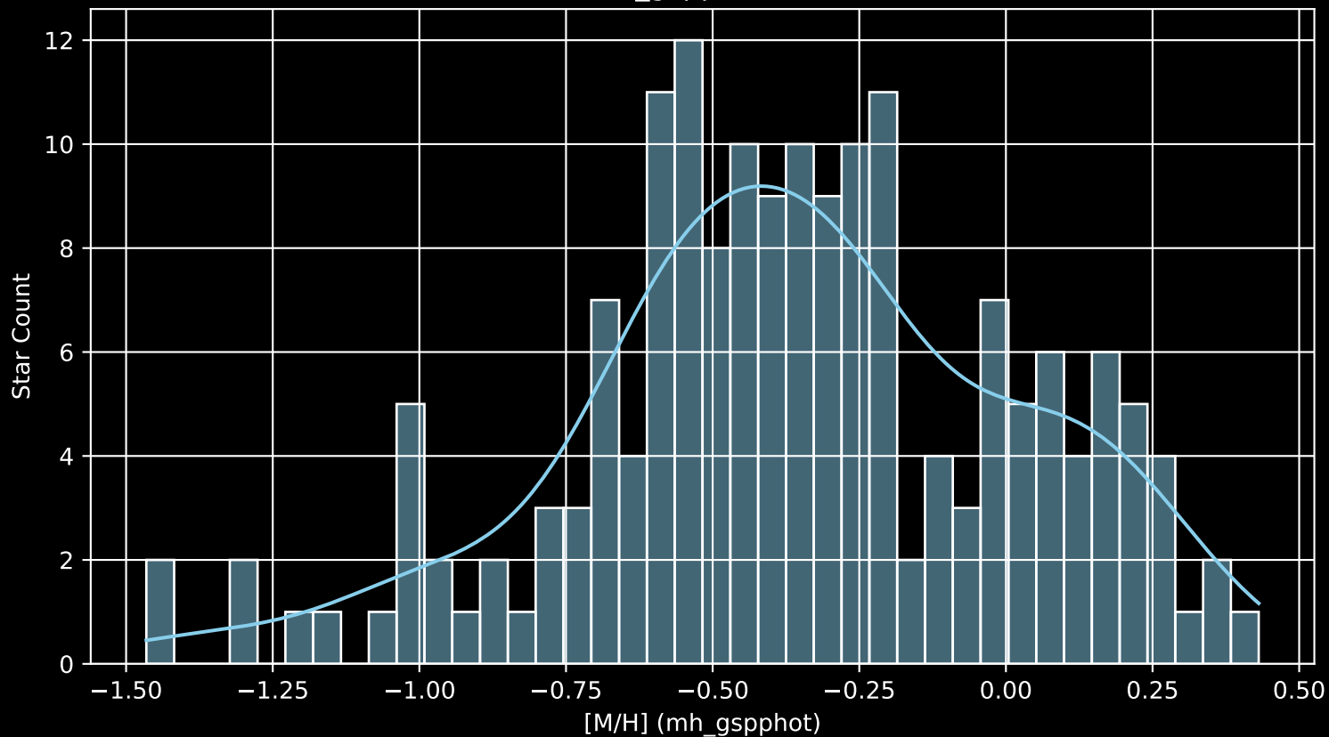
Gaia Cluster: [Collinder_350 [M/H] (mh_gspphot) (n= 175)
