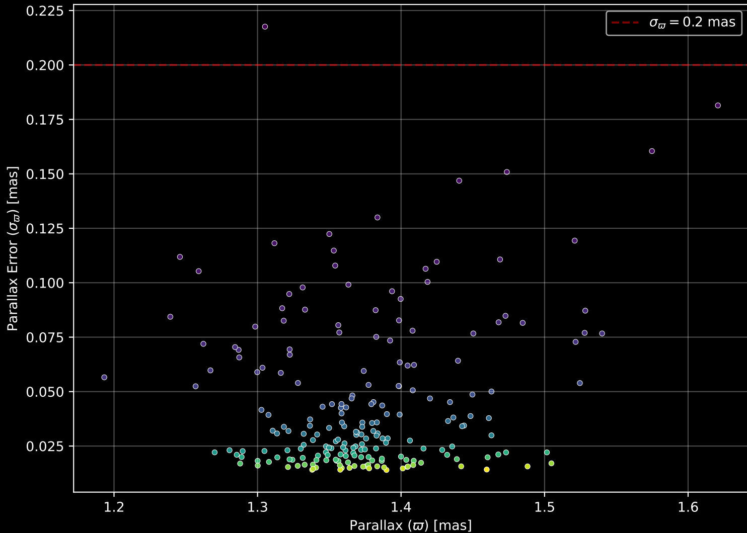
Gaia Cluster: [Collinder_394] Parallax Quality (n= 208)
