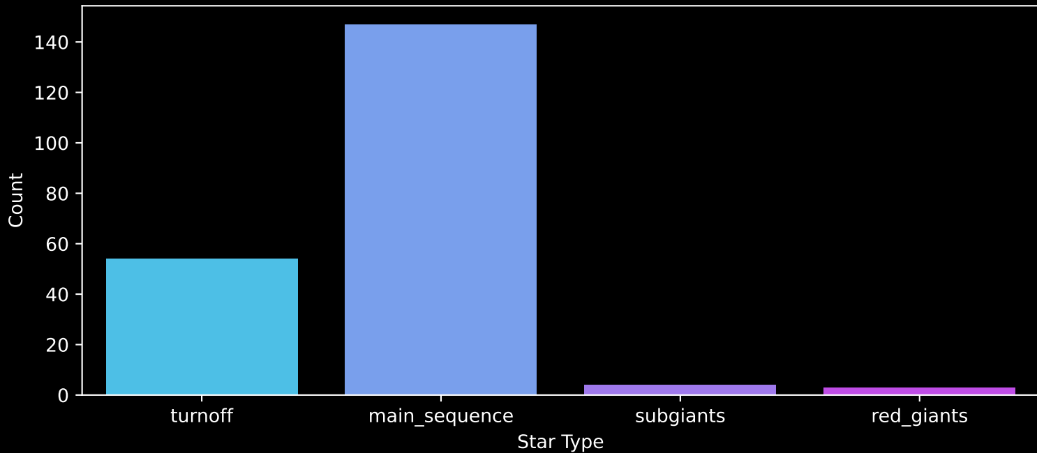
Gaia Cluster: [Collinder_394] Count plot of Star Type
