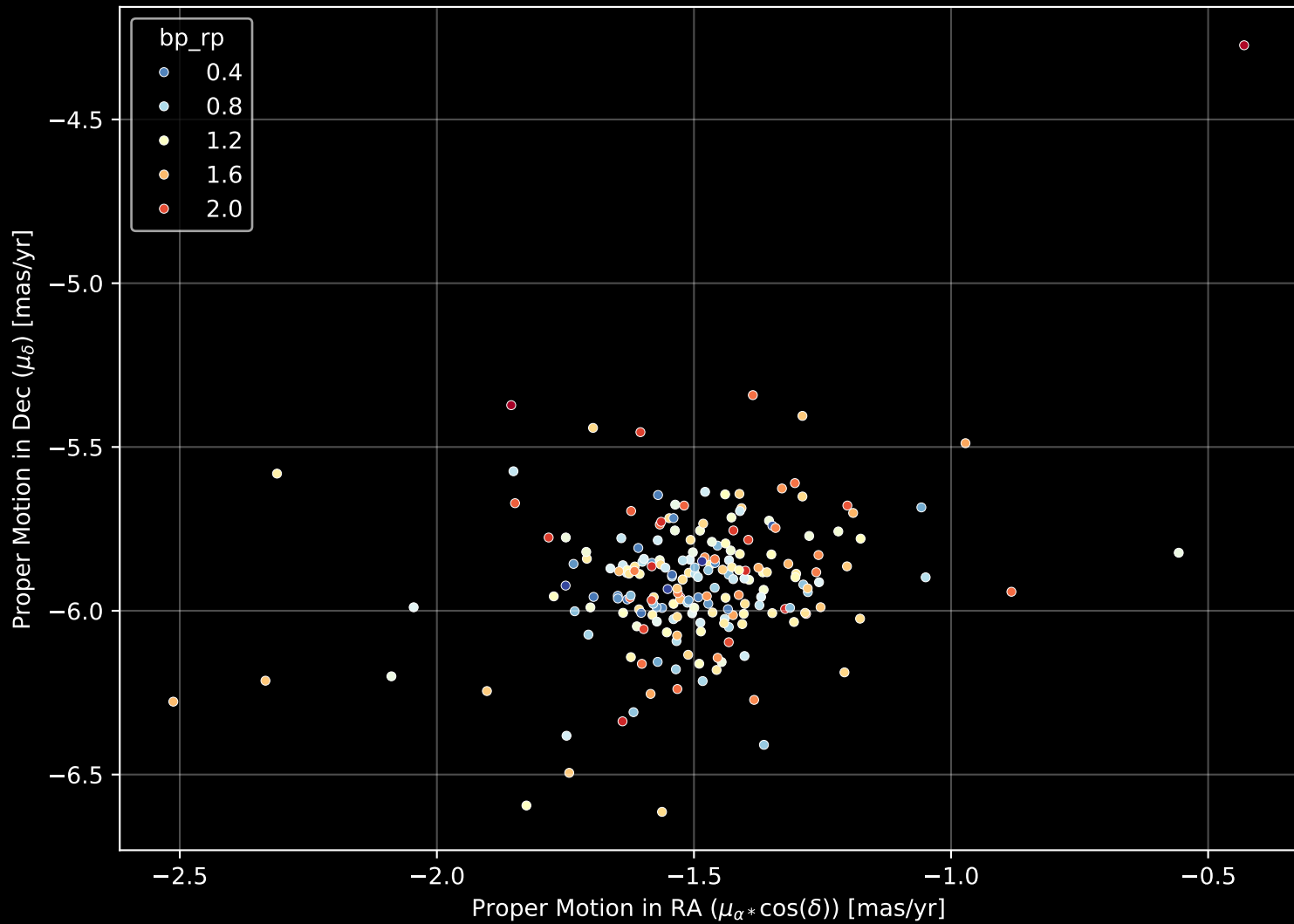
Gaia Cluster: [Collinder_394] Proper Motion Diagram (n= 208)
