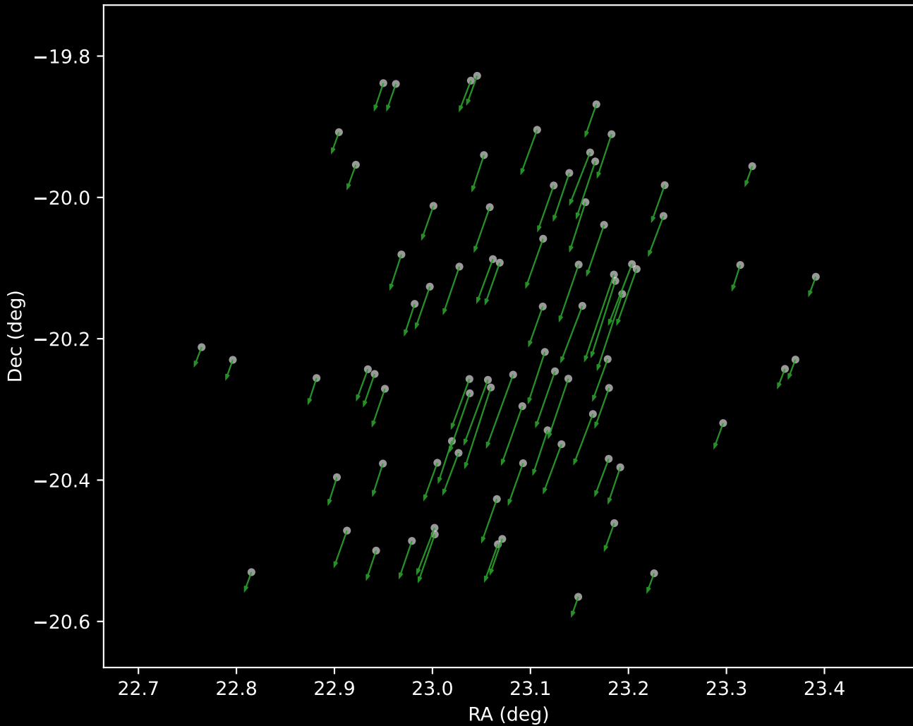
Gaia DR3 Cluster 4 Proper Motion Vectors (n=81)
