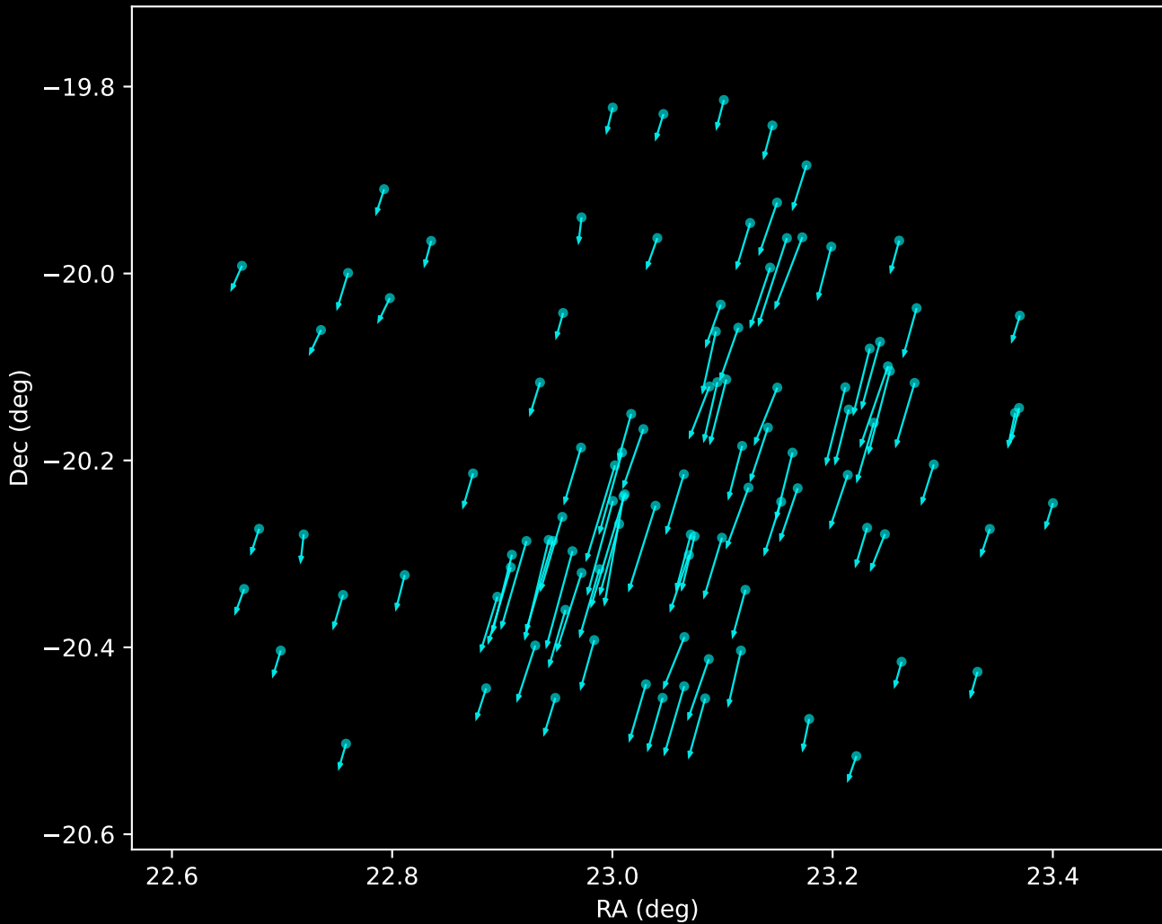
Gaia DR3 Noise Stream Proper Motion Vectors (n=103)
