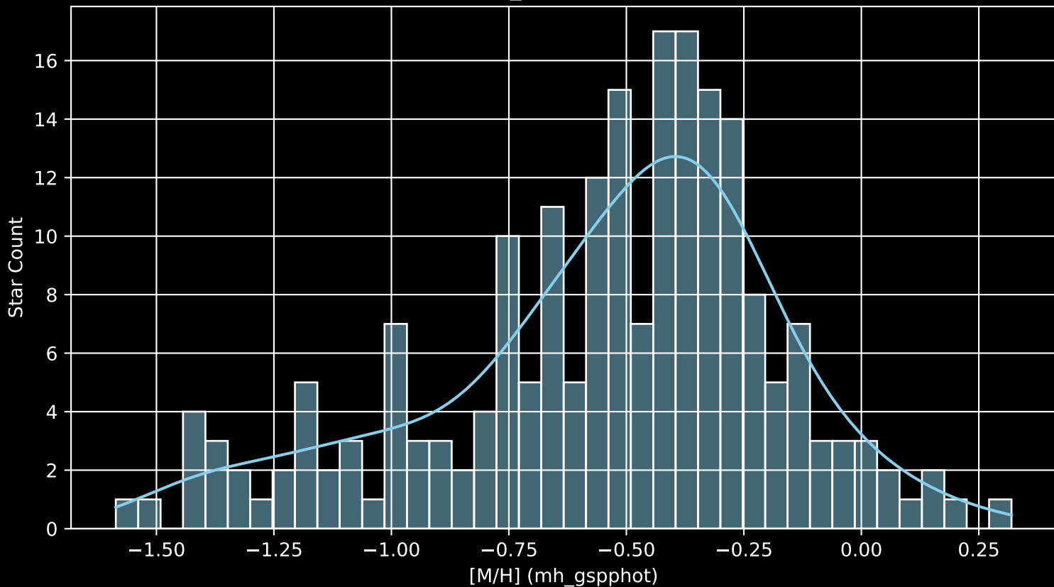
Gaia Cluster: [Collinder_394 [M/H] (mh_gspphot) (n= 208)
