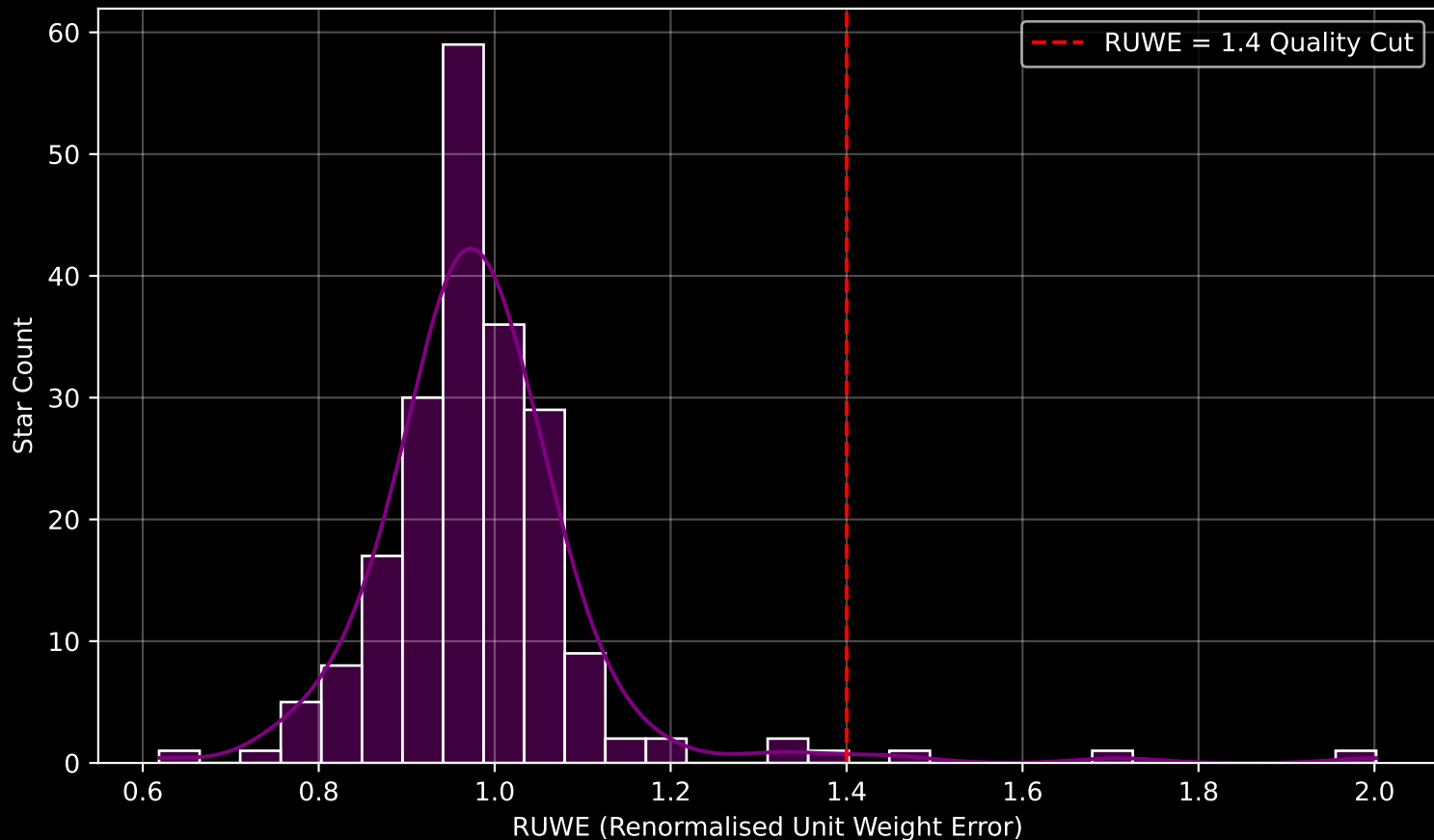
Gaia Cluster: [Collinder_394] RUWE Distribution (n= 205)
