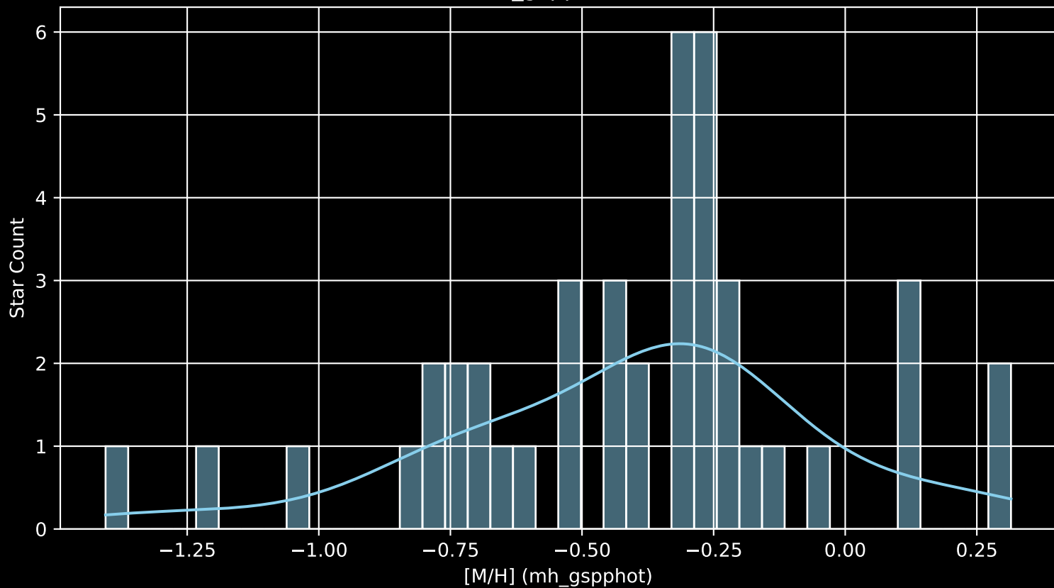
Gaia Cluster: [Collinder_419 [M/H] (mh_gspphot) (n= 43)
