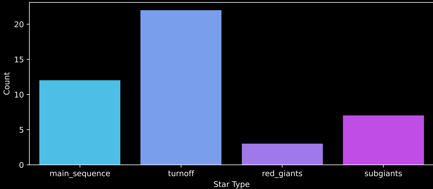
Gaia Cluster: [Collinder_419] Count plot of Star Type
