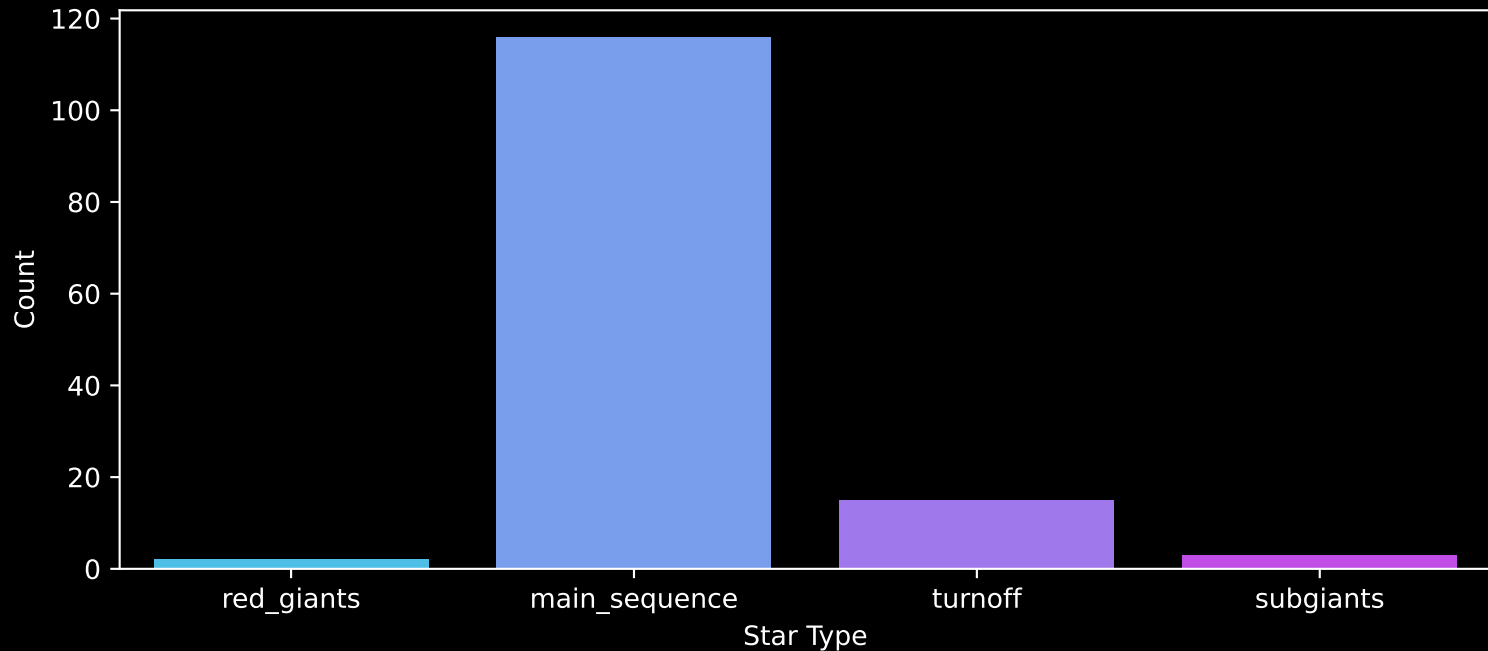
Gaia Cluster: [Collinder_421] Count plot of Star Type
