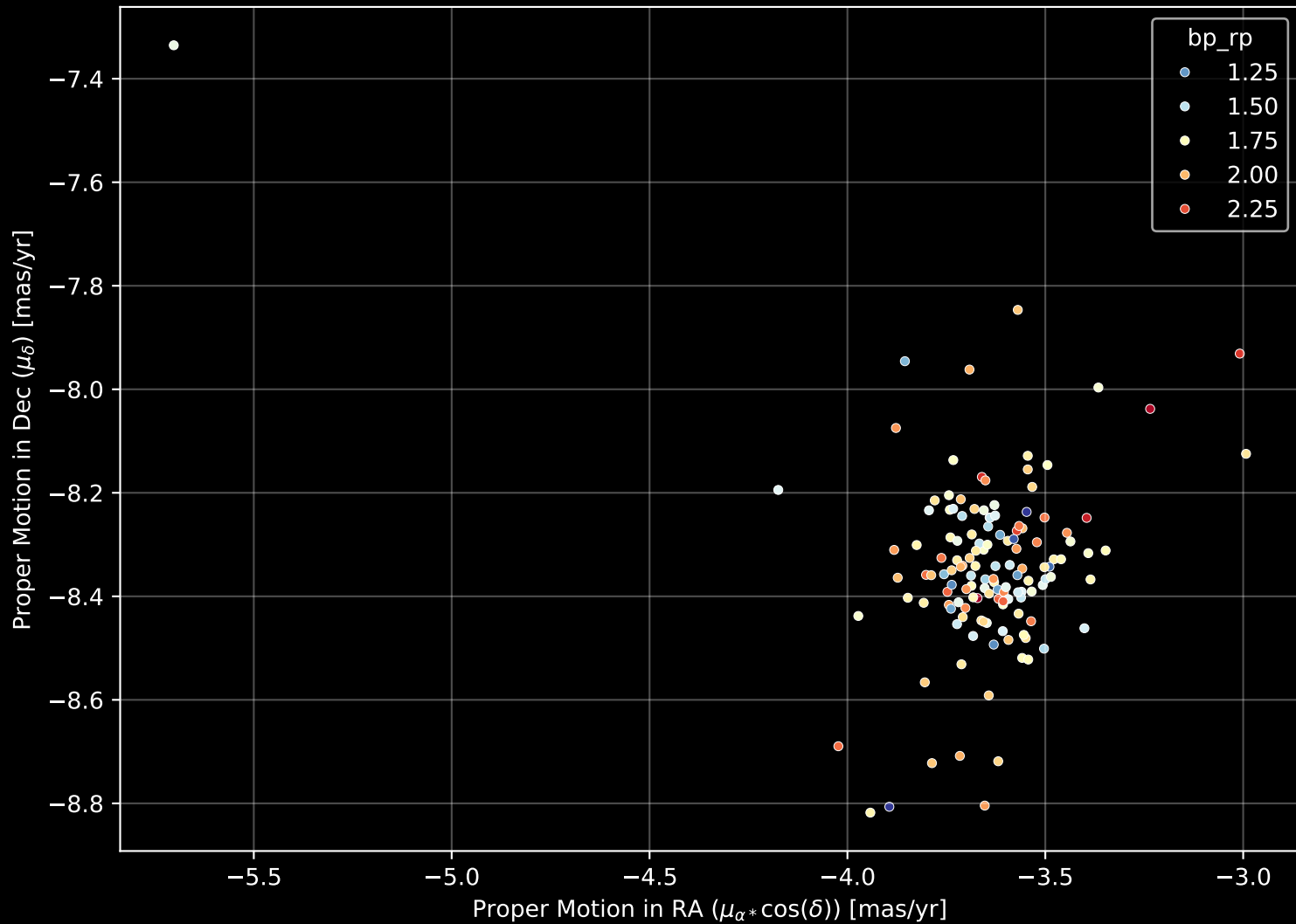
Gaia Cluster: [Collinder_421] Proper Motion Diagram (n= 136)
