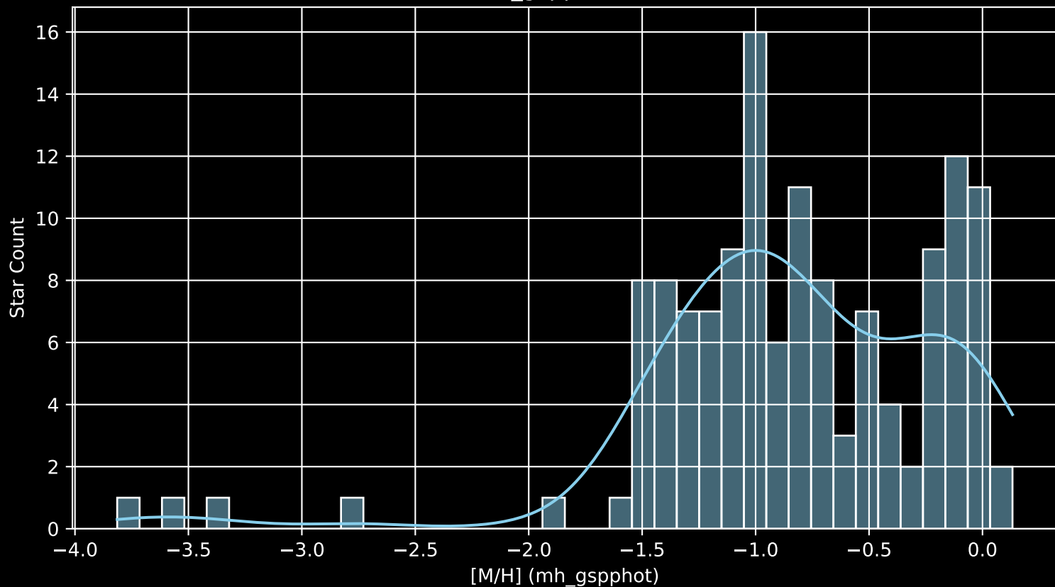
Gaia Cluster: [Collinder_421 [M/H] (mh_gspphot) (n= 136)
