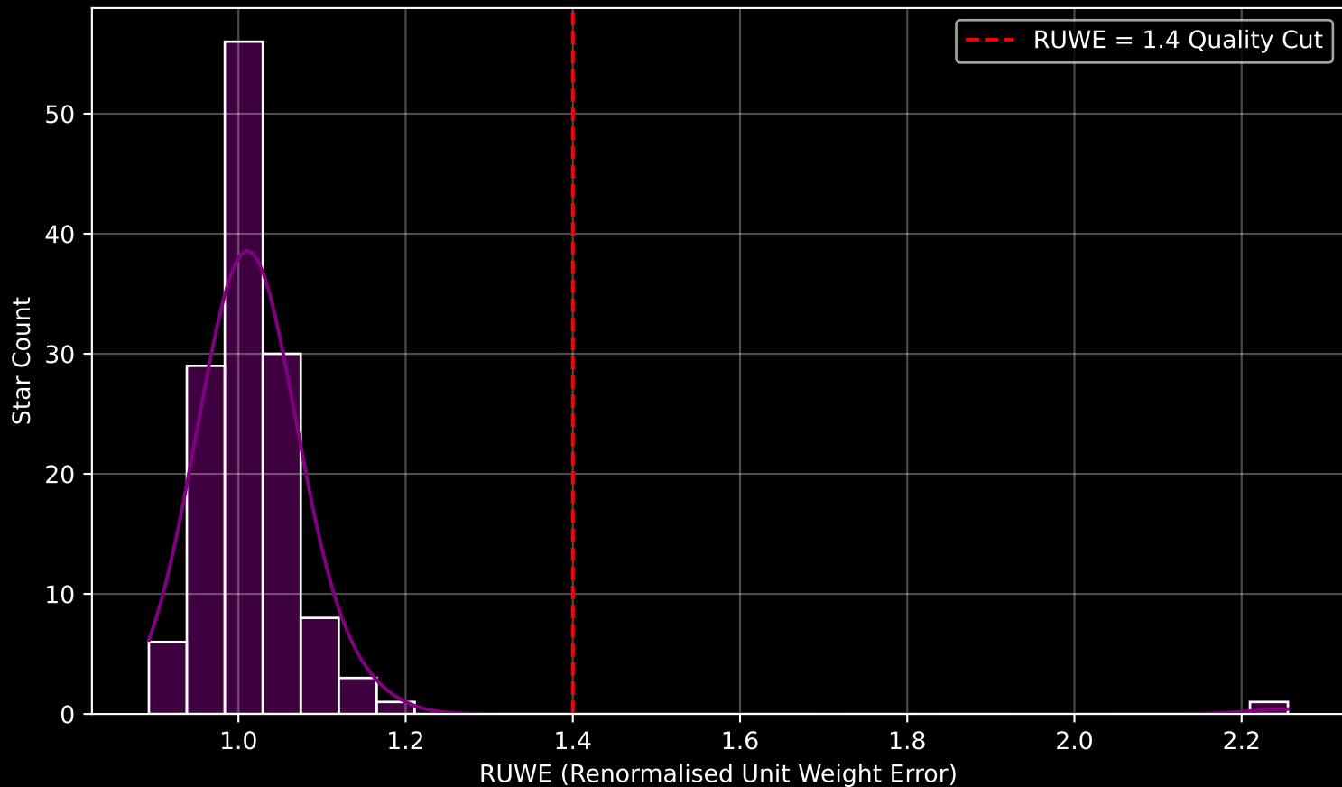
Gaia Cluster: [Collinder_421] RUWE Distribution (n= 134)
