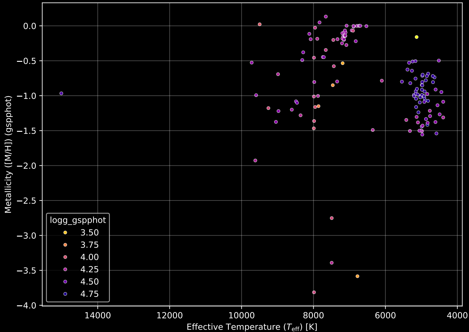
Gaia Cluster: [Collinder_421] Stellar Population Parameters (n= 136)
