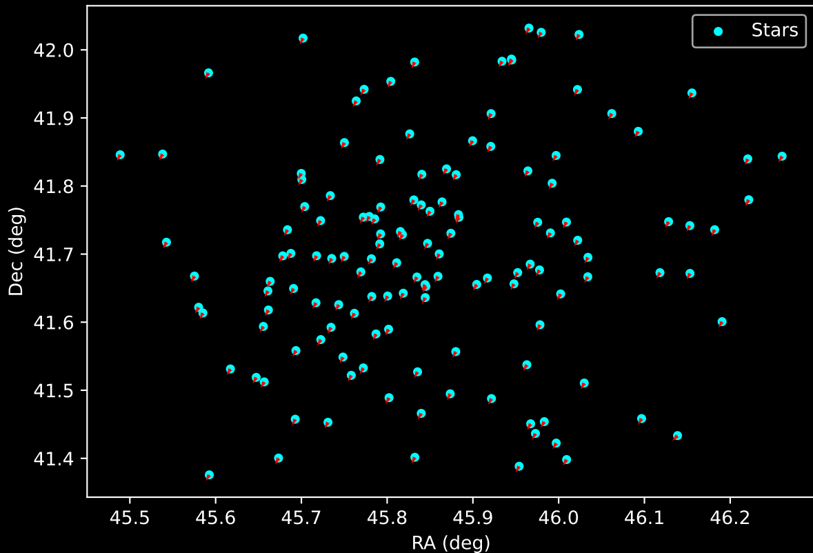
Gaia Cluster: [Collinder_421] Proper Motion Vectors for Gaia Star Field (n= 136)
