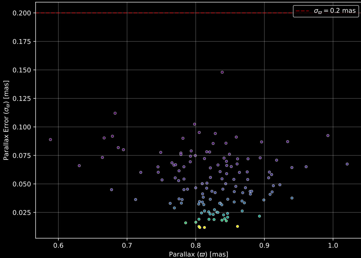
Gaia Cluster: [Collinder_421] Parallax Quality (n= 136)
