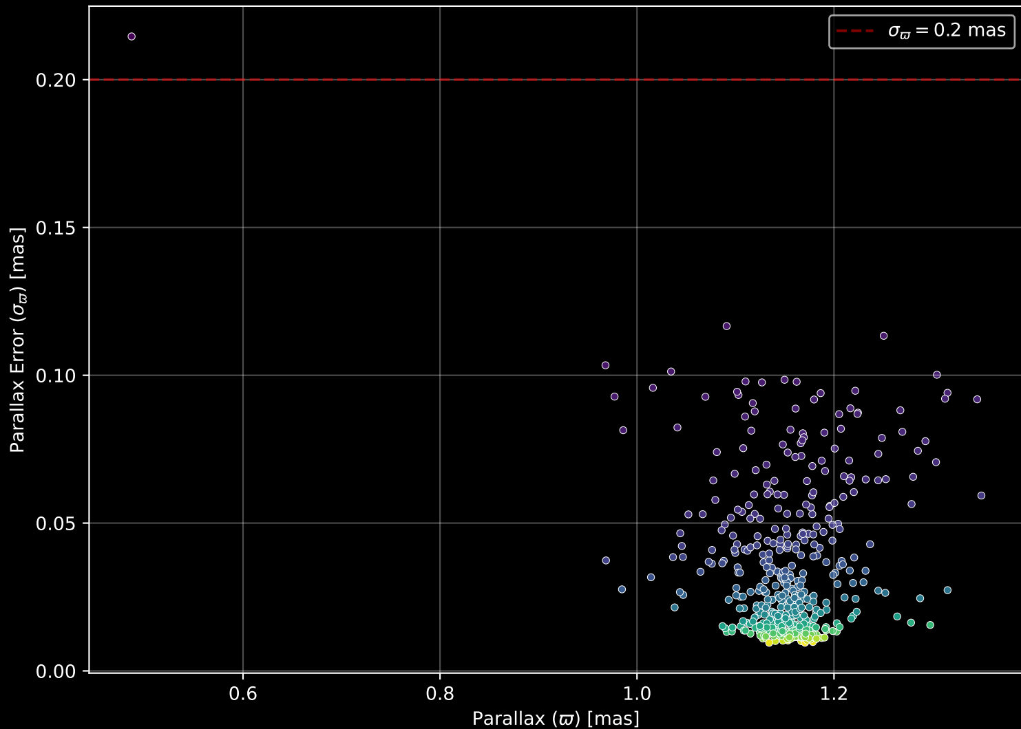
Gaia Cluster: [Collinder_463] Parallax Quality (n= 466)
