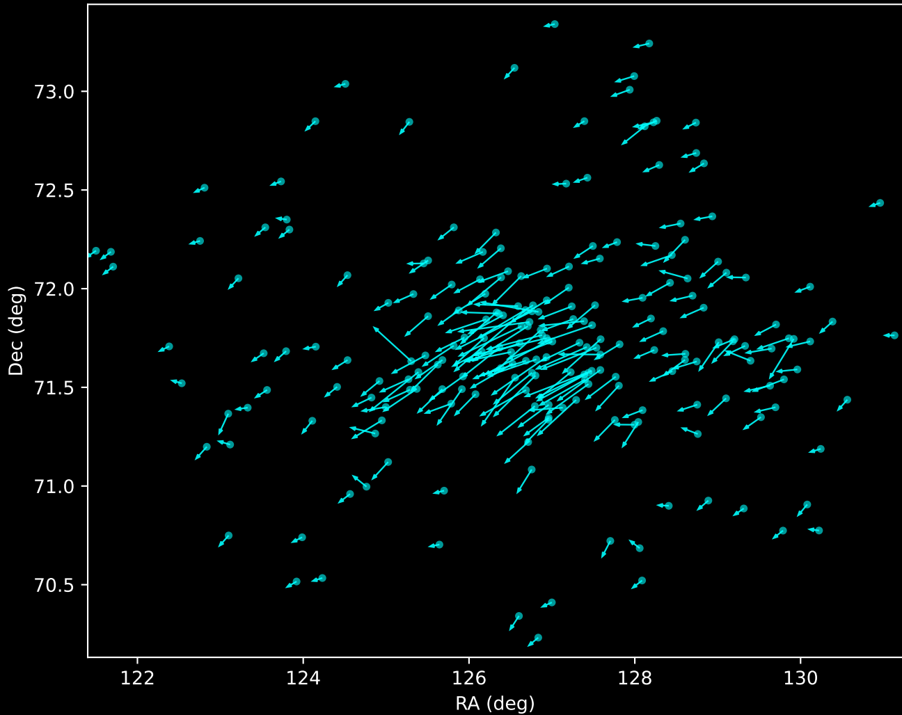
Gaia DR3 Noise Stream Proper Motion Vectors (n=213)
