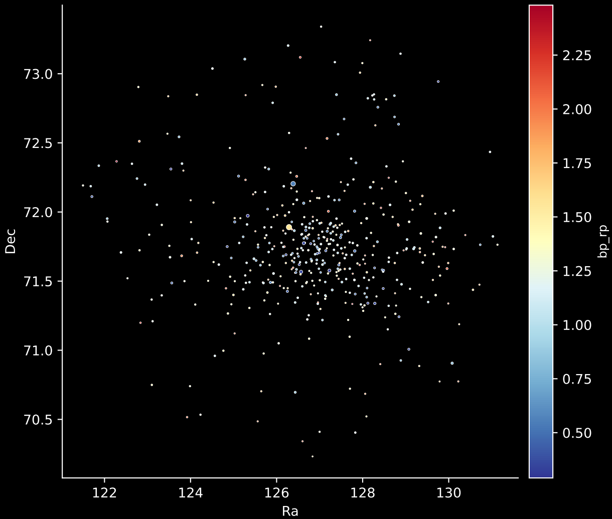
Gaia Cluster: [Collinder_463] Stars: 466
