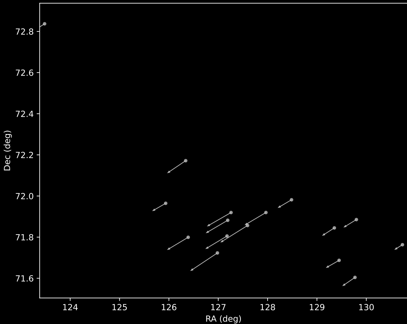
Gaia DR3 Cluster 15 Proper Motion Vectors (n=16)
