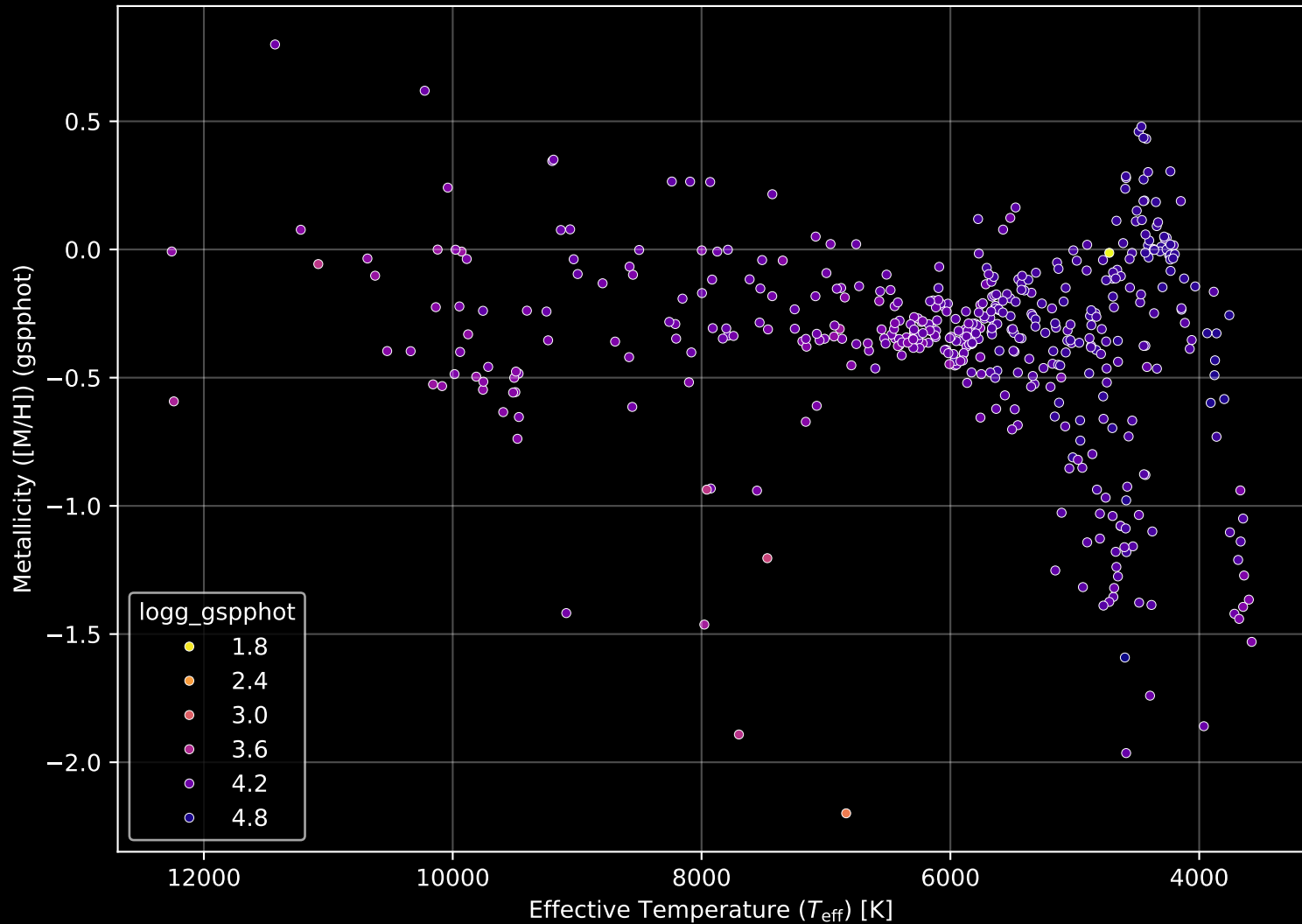
Gaia Cluster: [Collinder_463] Stellar Population Parameters (n= 466)
