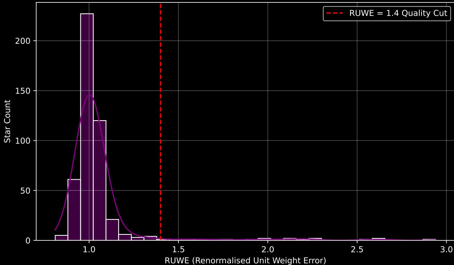
Gaia Cluster: [Collinder_463] RUWE Distribution (n= 465)
