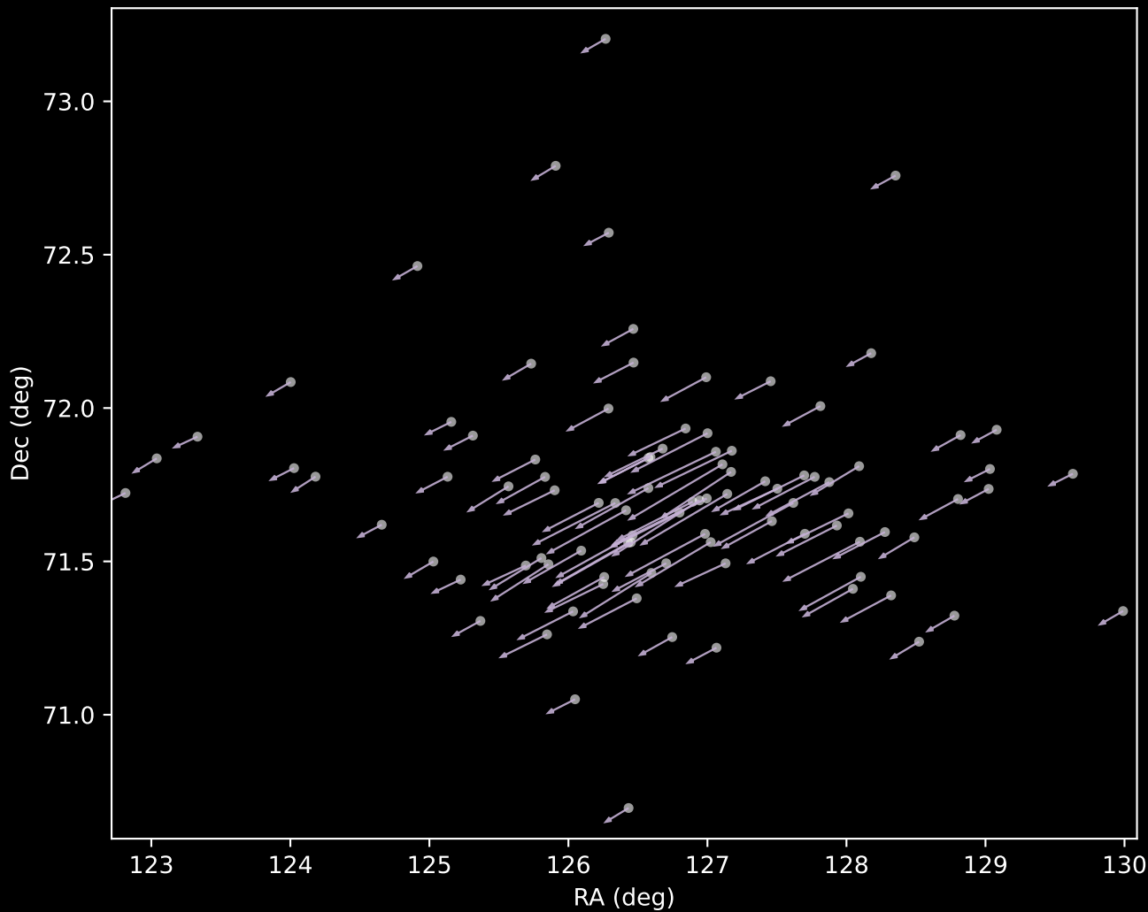
Gaia DR3 Cluster 9 Proper Motion Vectors (n=95)
