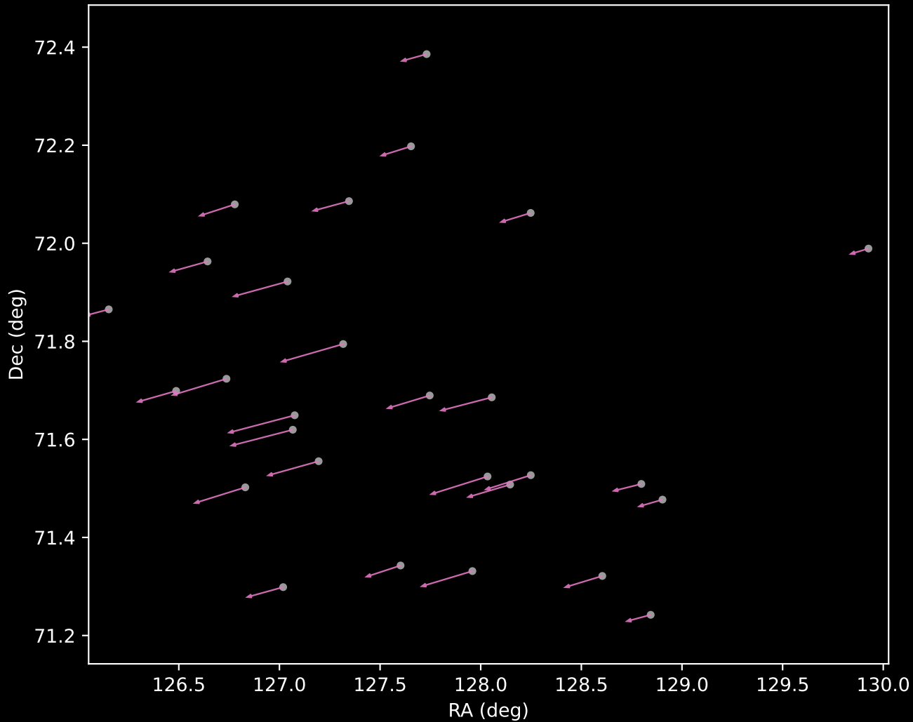
Gaia DR3 Cluster 12 Proper Motion Vectors (n=28)
