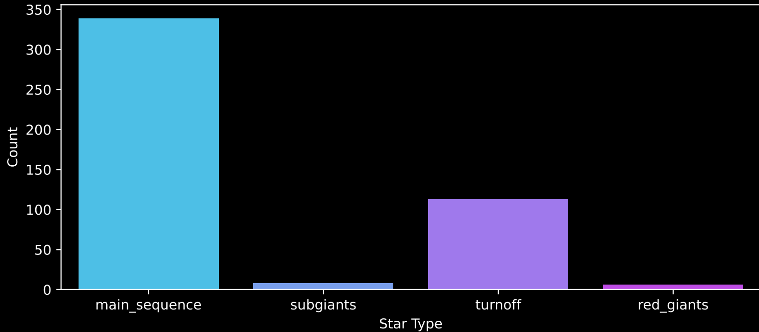
Gaia Cluster: [Collinder_463] Count plot of Star Type
