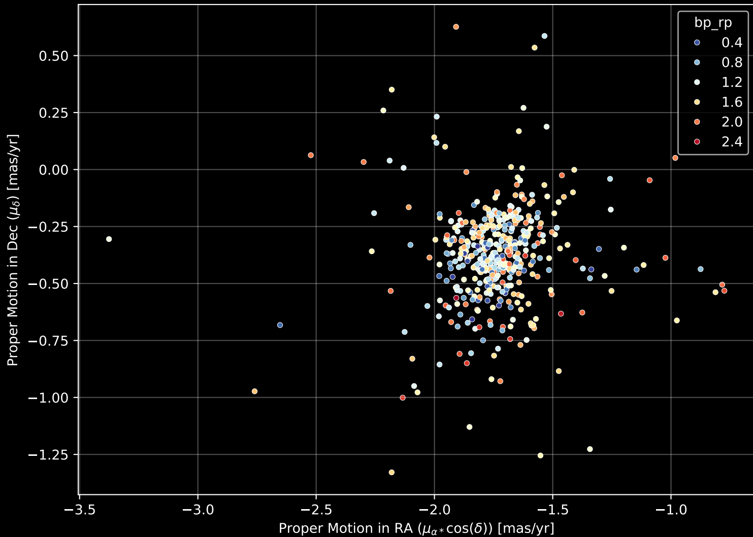
Gaia Cluster: [Collinder_463] Proper Motion Diagram (n= 466)
