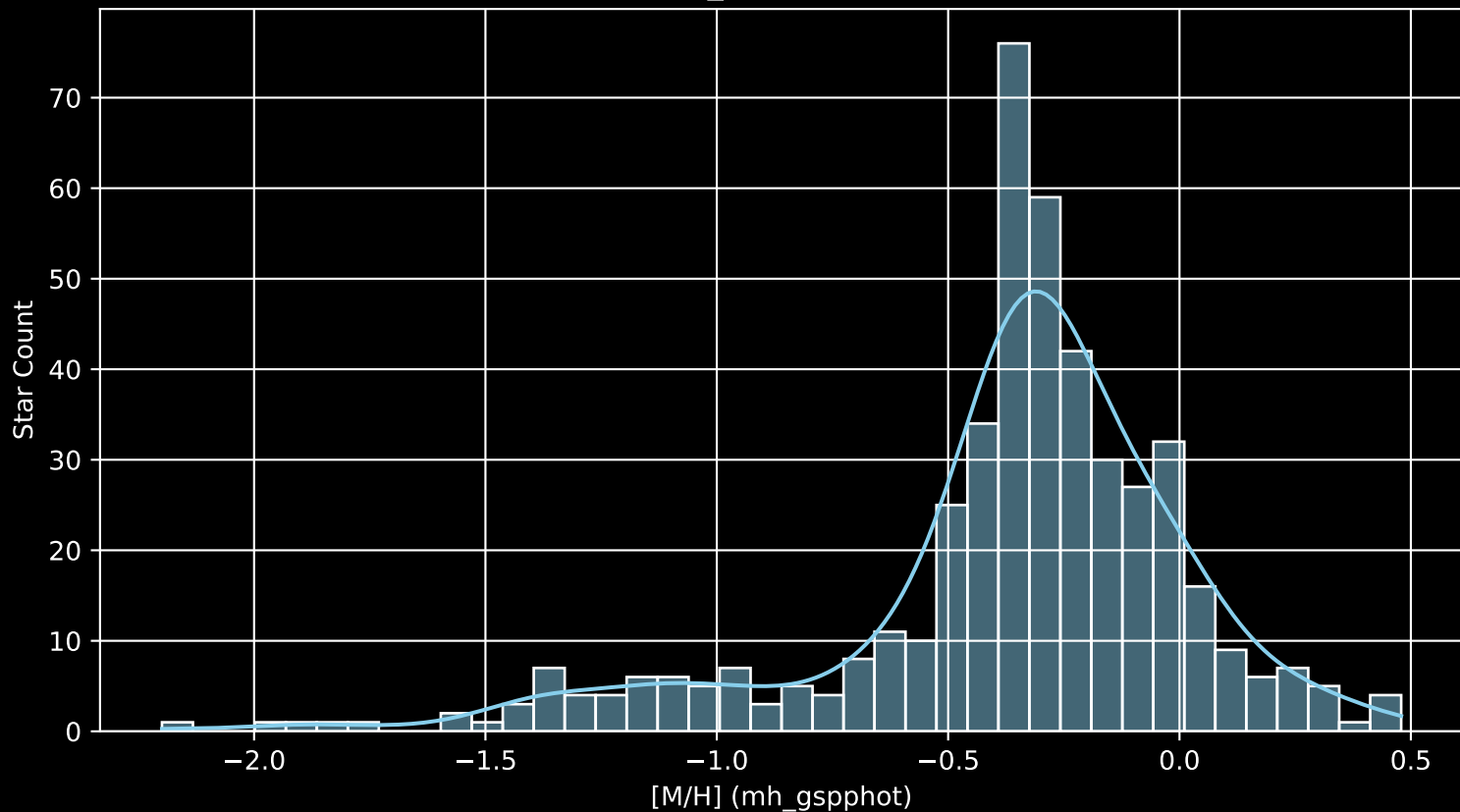
Gaia Cluster: [Collinder_463 [M/H] (mh_gspphot) (n= 464)
