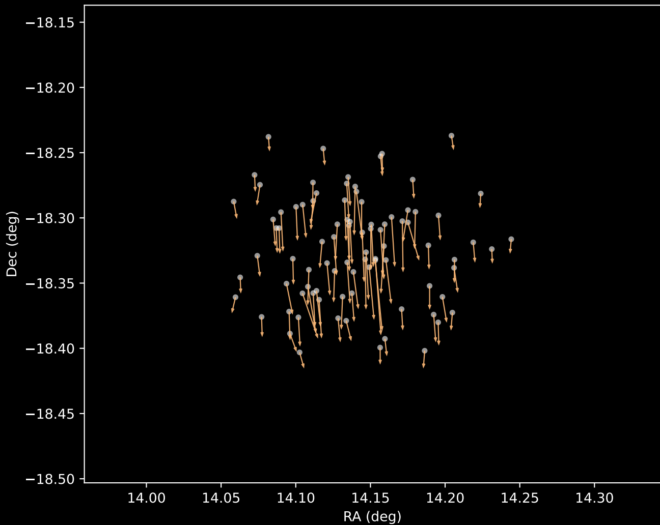
Gaia DR3 Cluster 3 Proper Motion Vectors (n=88)
