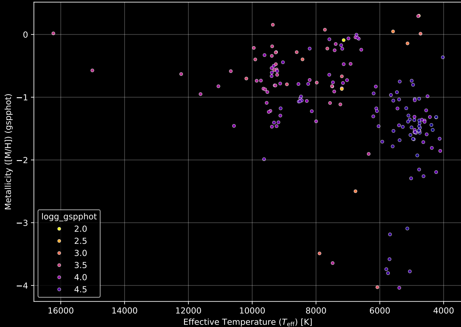
Gaia Cluster: [Collinder_469] Stellar Population Parameters (n= 171)
