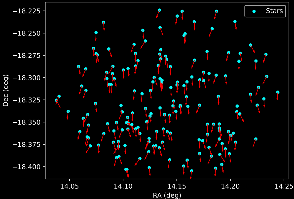
Gaia Cluster: [Collinder_469] Proper Motion Vectors for Gaia Star Field (n= 171)
