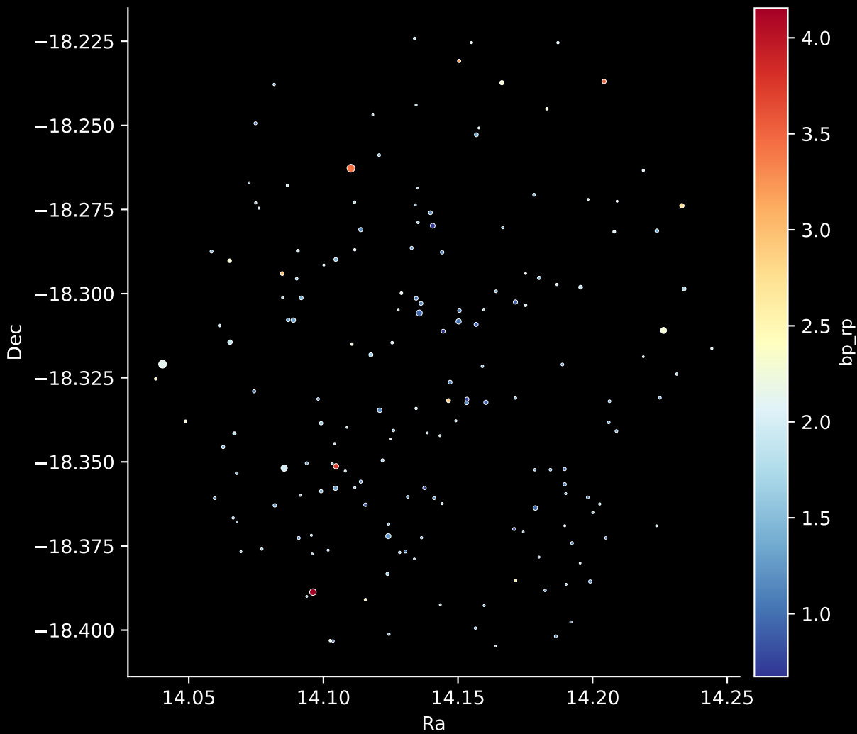
Gaia Cluster: [Collinder_469] Stars: 171
