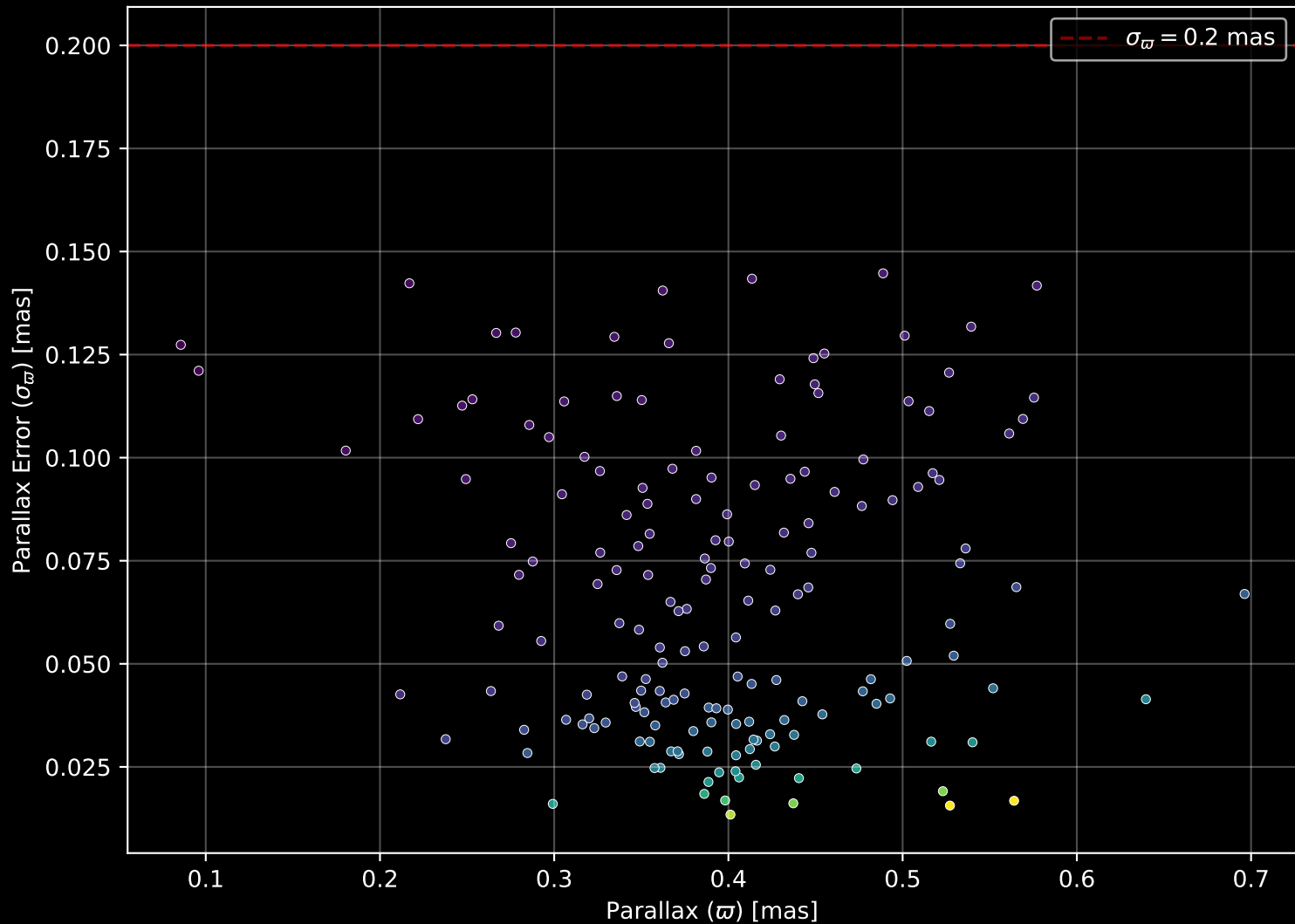
Gaia Cluster: [Collinder_469] Parallax Quality (n= 171)
