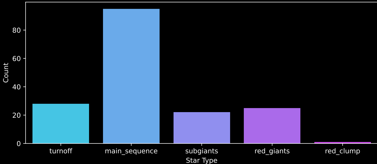
Gaia Cluster: [Collinder_469] Count plot of Star Type
