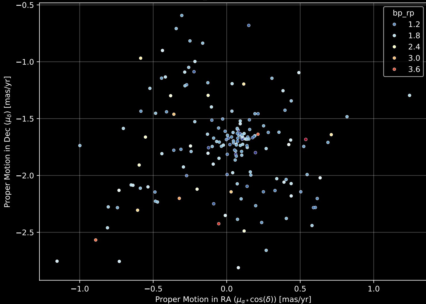
Gaia Cluster: [Collinder_469] Proper Motion Diagram (n= 171)
