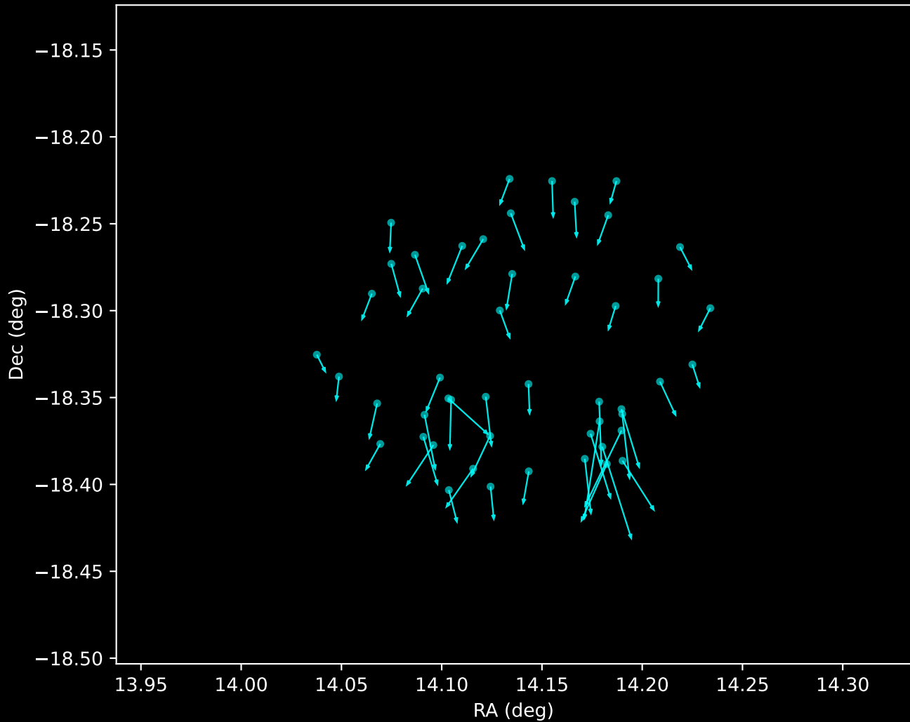
Gaia DR3 Noise Stream Proper Motion Vectors (n=49)
