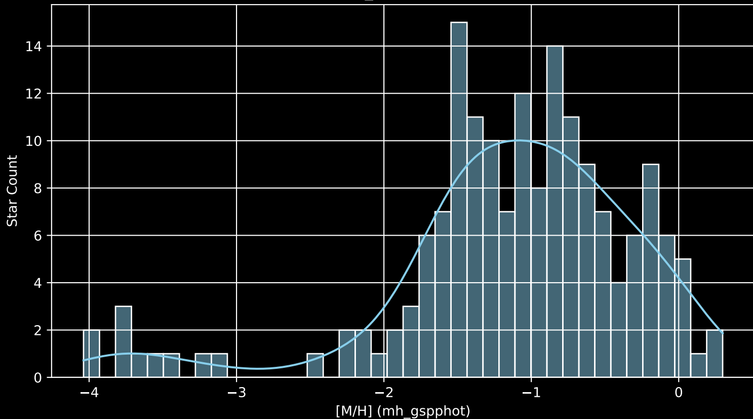
Gaia Cluster: [Collinder_469 [M/H] (mh_gspphot) (n= 171)
