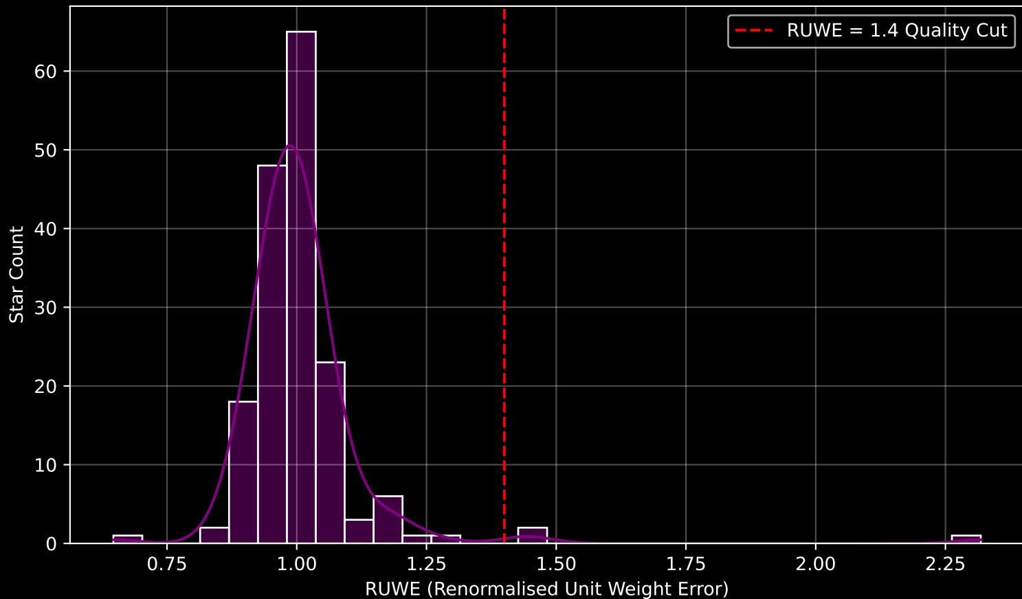
Gaia Cluster: [Collinder_469] RUWE Distribution (n= 171)
