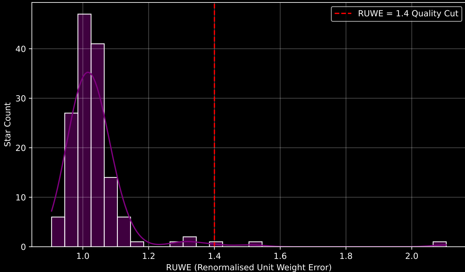
Gaia Cluster: [Collinder_74] RUWE Distribution (n= 148)
