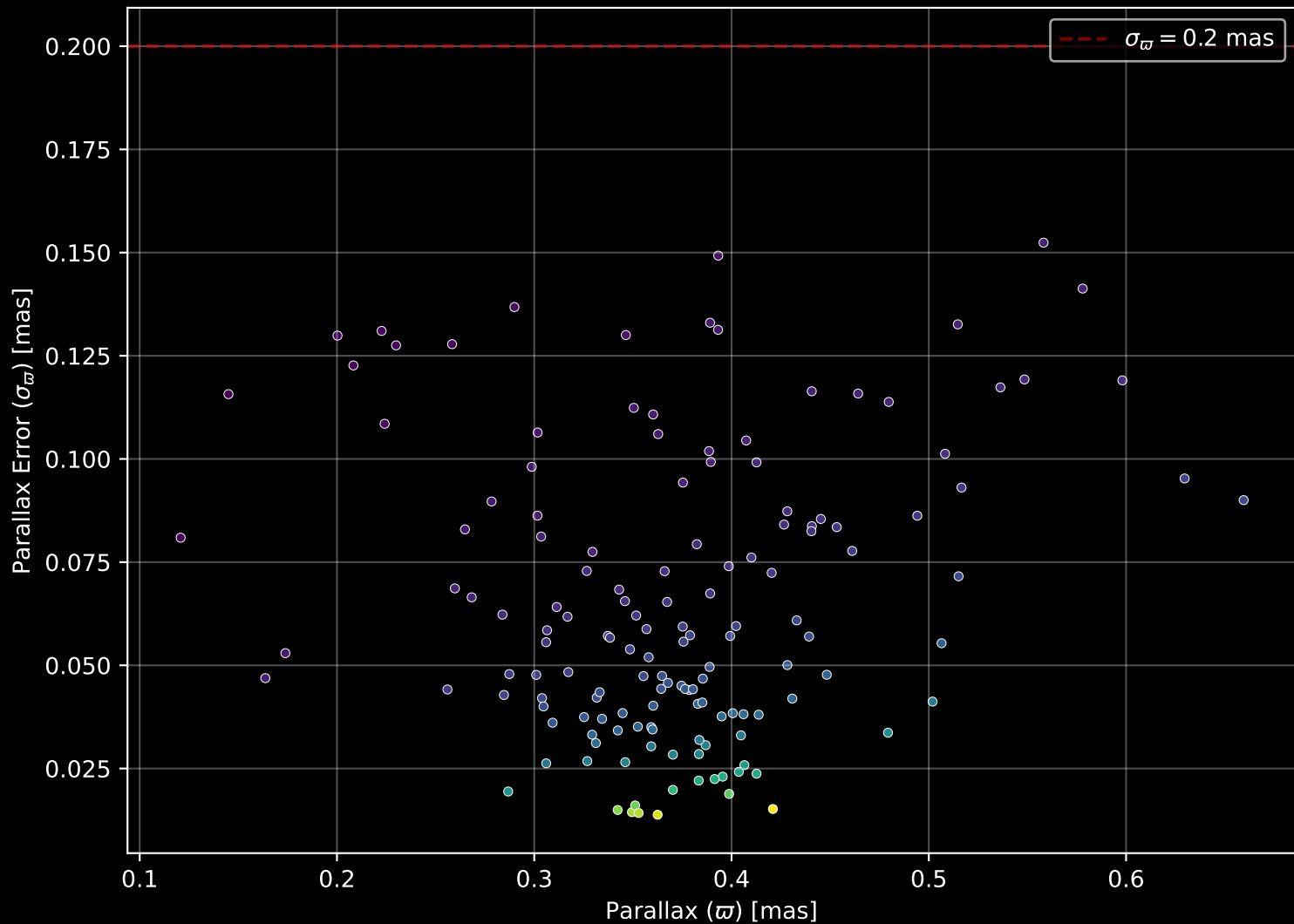
Gaia Cluster: [Collinder_74] Parallax Quality (n= 148)
