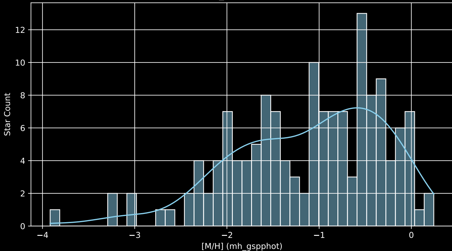
Gaia Cluster: [Collinder_74 [M/H] (mh_gspphot) (n= 147)
