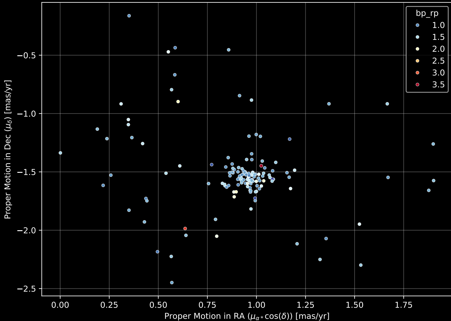
Gaia Cluster: [Collinder_74] Proper Motion Diagram (n= 148)
