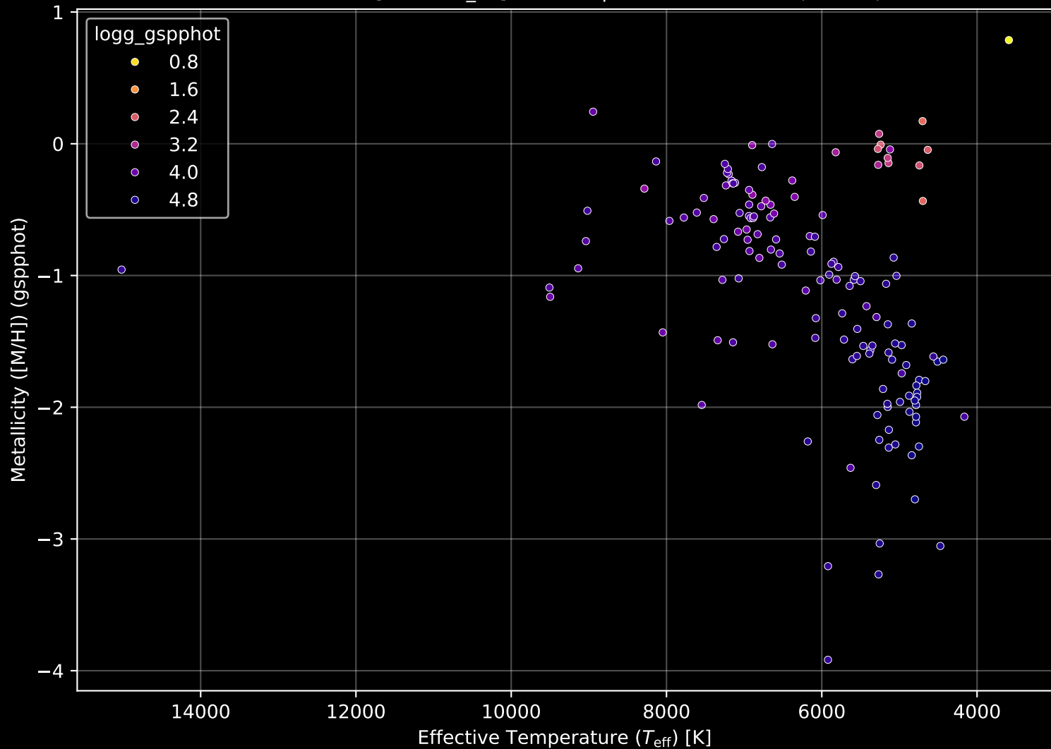
Gaia Cluster: [Collinder_74] Stellar Population Parameters (n= 148)
