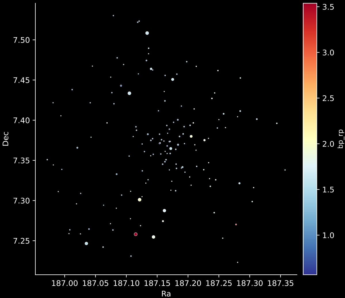
Gaia Cluster: [Collinder_74] Stars: 148
