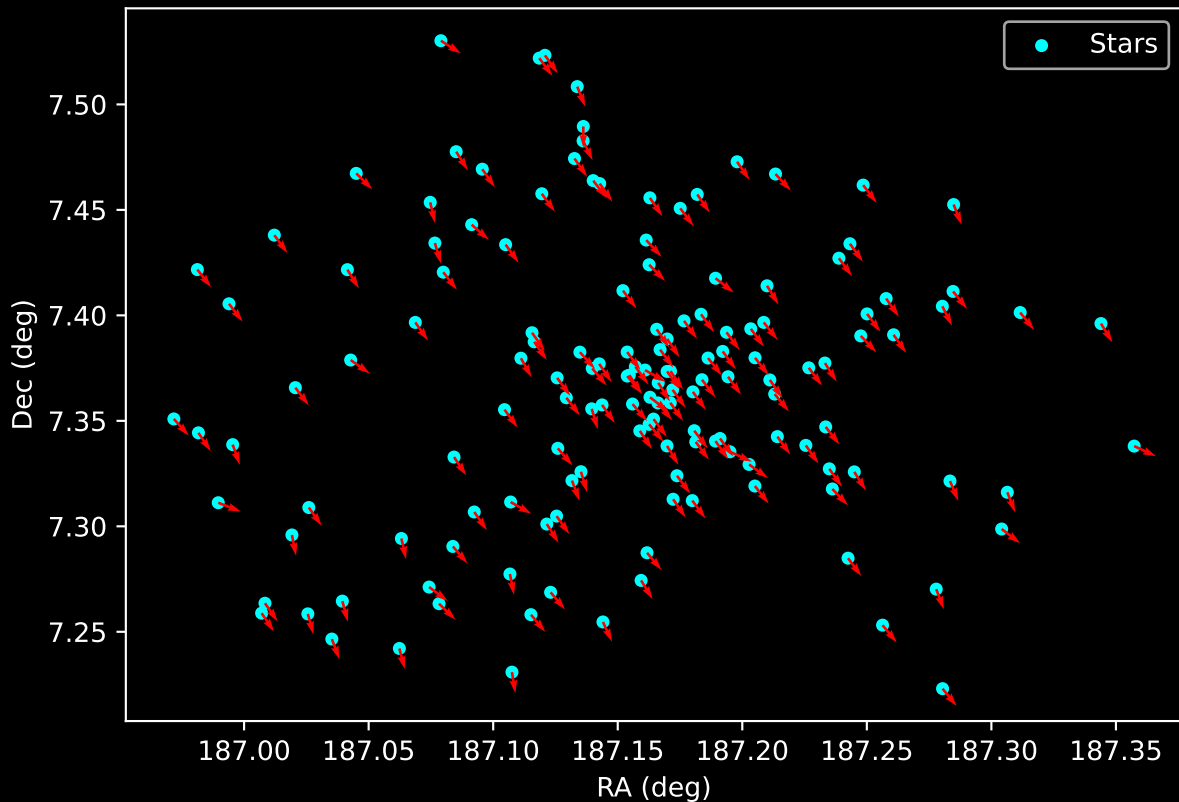
Gaia Cluster: [Collinder_74] Proper Motion Vectors for Gaia Star Field (n= 148)
