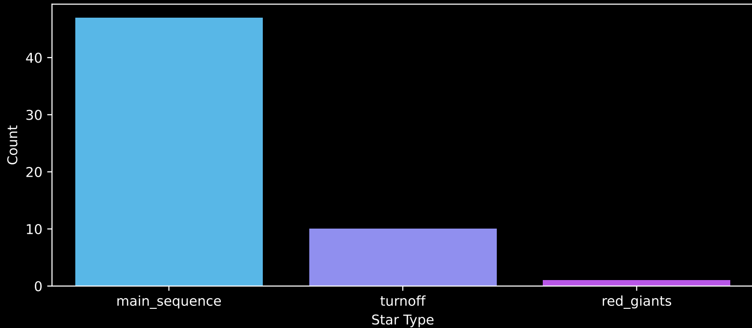
Gaia Cluster: [Czernik_18] Count plot of Star Type
