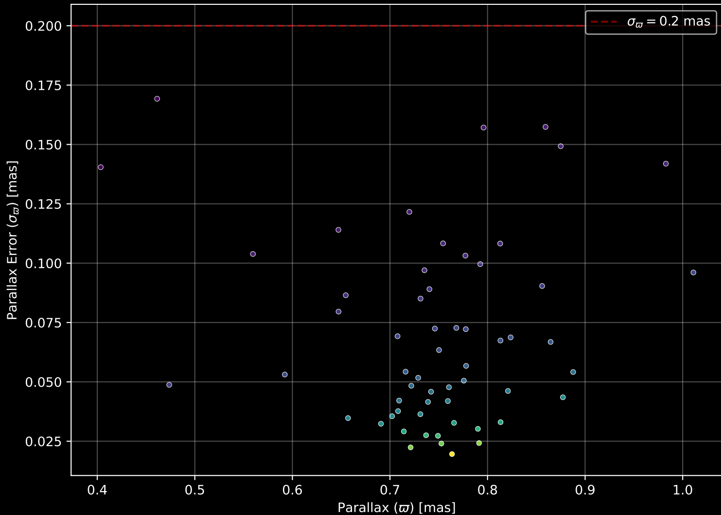
Gaia Cluster: [Czernik_18] Parallax Quality (n= 58)
