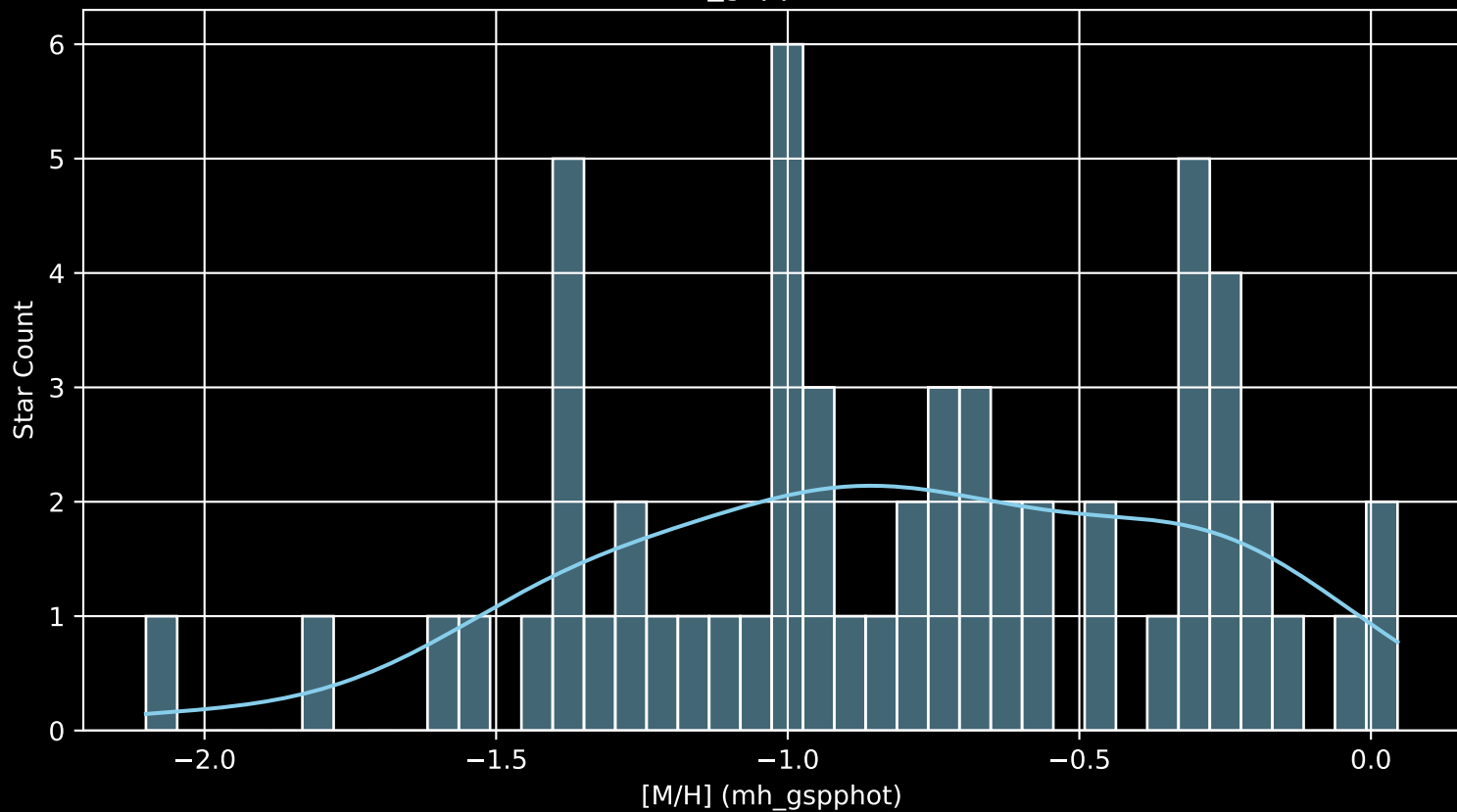
Gaia Cluster: [Czernik_18 [M/H] (mh_gspphot) (n= 58)
