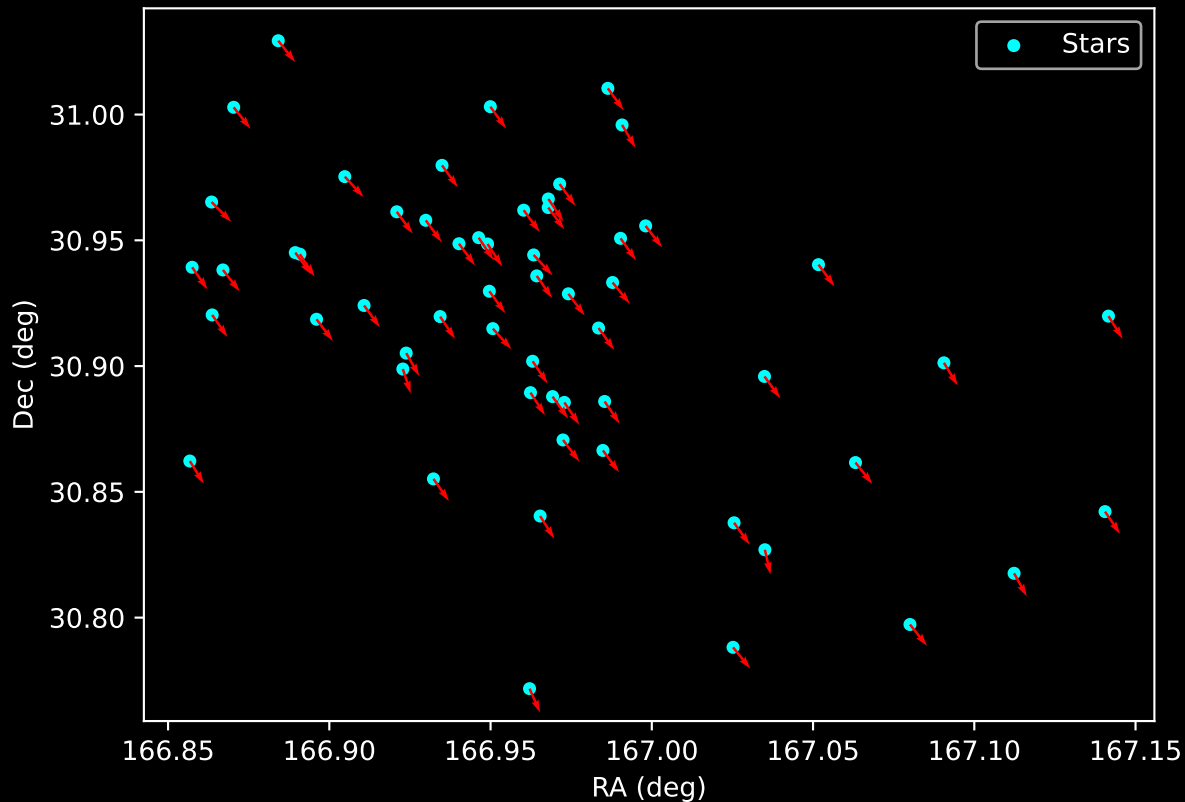
Gaia Cluster: [Czernik_18] Proper Motion Vectors for Gaia Star Field (n= 58)
