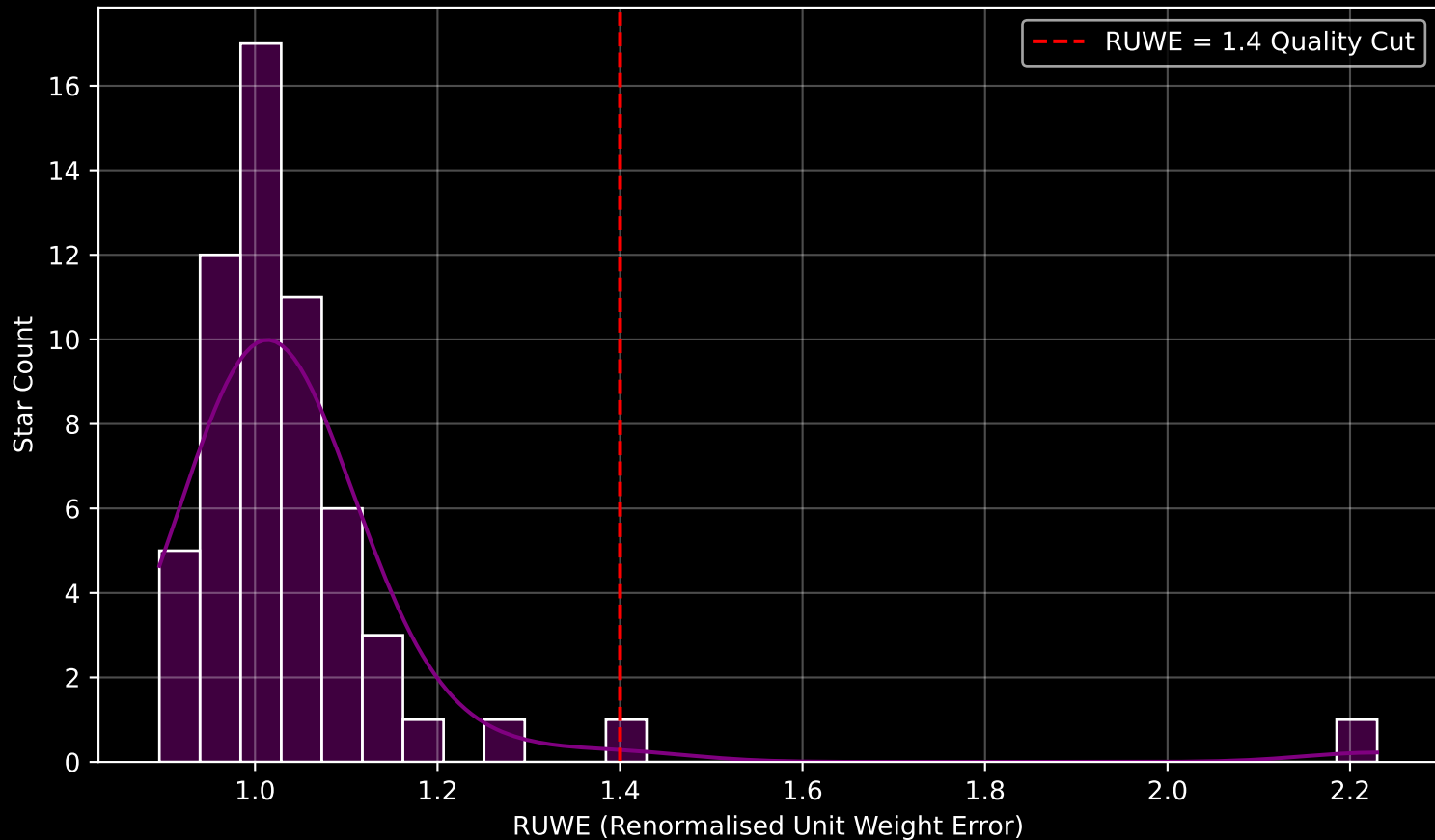
Gaia Cluster: [Czernik_18] RUWE Distribution (n= 58)
