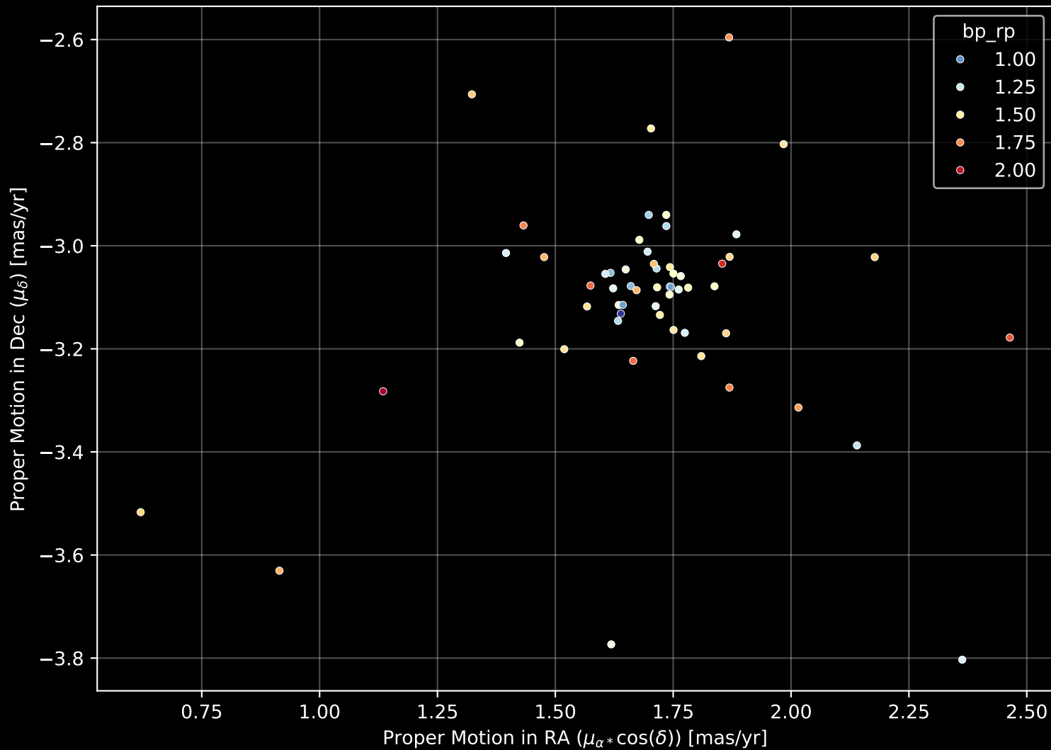
Gaia Cluster: [Czernik_18] Proper Motion Diagram (n= 58)
