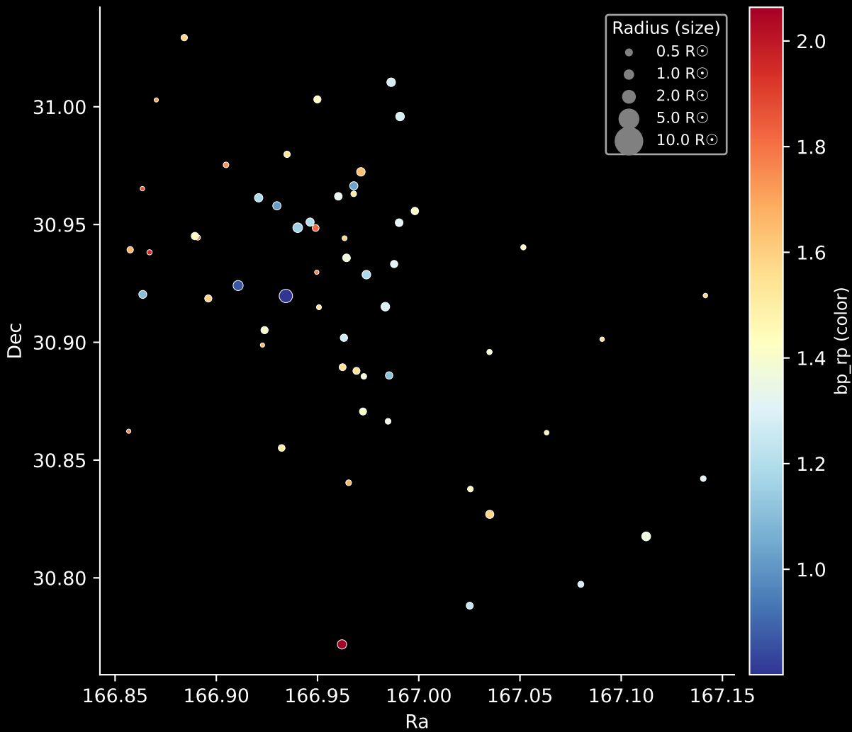
Gaia Cluster: [Czernik_18] Stars: 58
