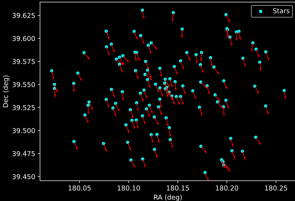
Gaia Cluster: [Czernik_20] Proper Motion Vectors for Gaia Star Field (n= 113)
