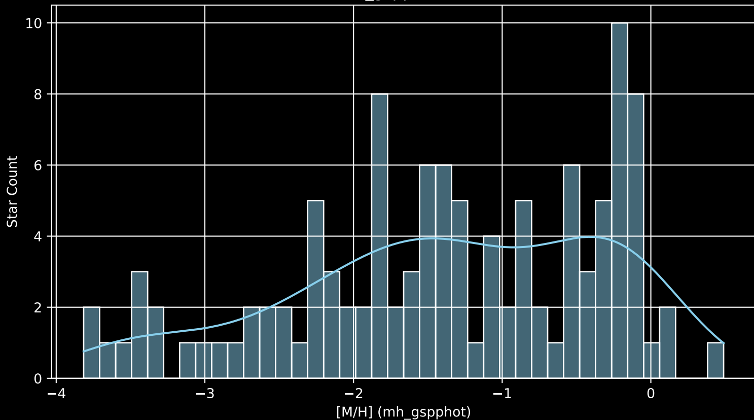
Gaia Cluster: [Czernik_20 [M/H] (mh_gspphot) (n= 113)
