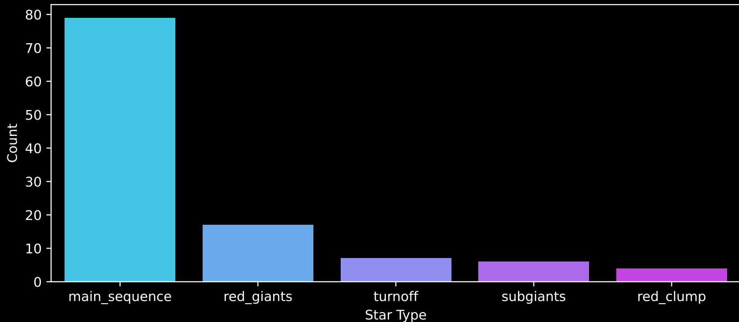
Gaia Cluster: [Czernik_20] Count plot of Star Type
