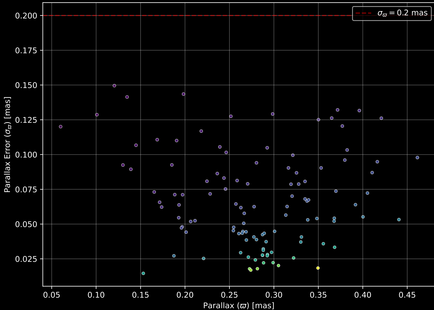
Gaia Cluster: [Czernik_20] Parallax Quality (n= 113)
