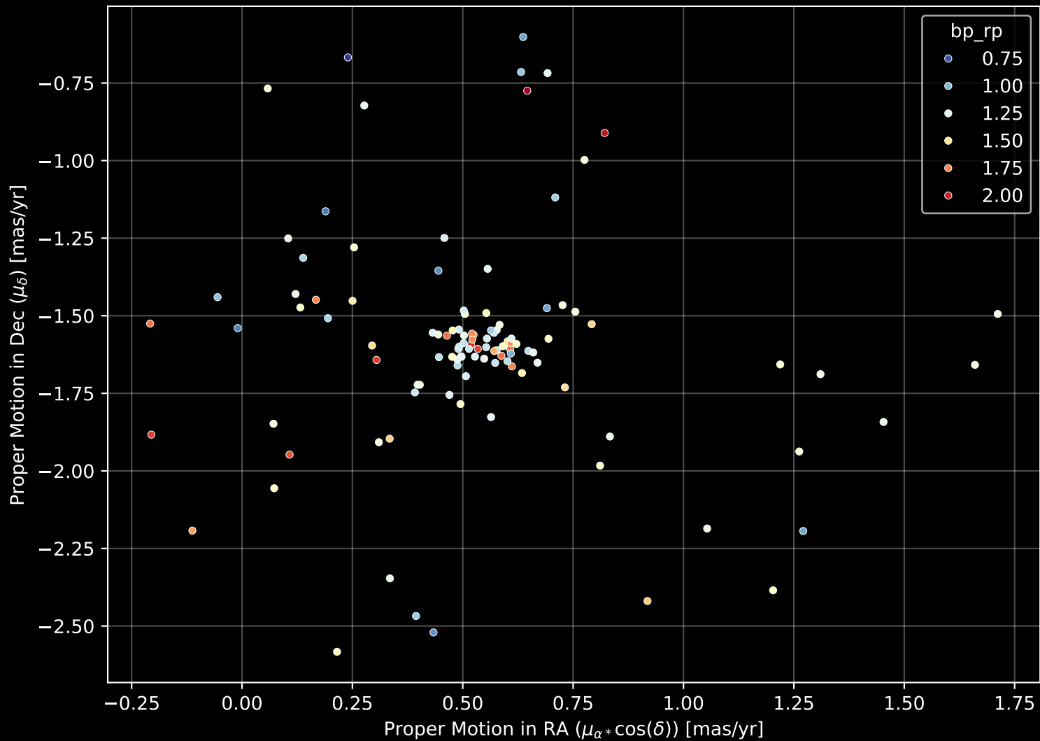
Gaia Cluster: [Czernik_20] Proper Motion Diagram (n= 113)
