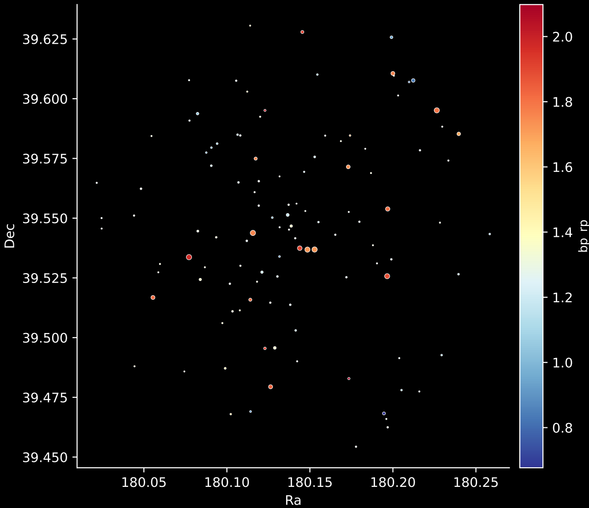
Gaia Cluster: [Czernik_20] Stars: 113
