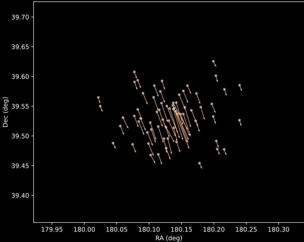
Gaia DR3 Cluster 3 Proper Motion Vectors (n=66)
