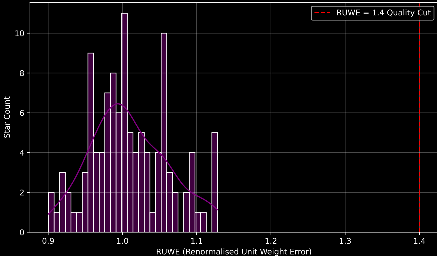
Gaia Cluster: [Czernik_20] RUWE Distribution (n= 113)
