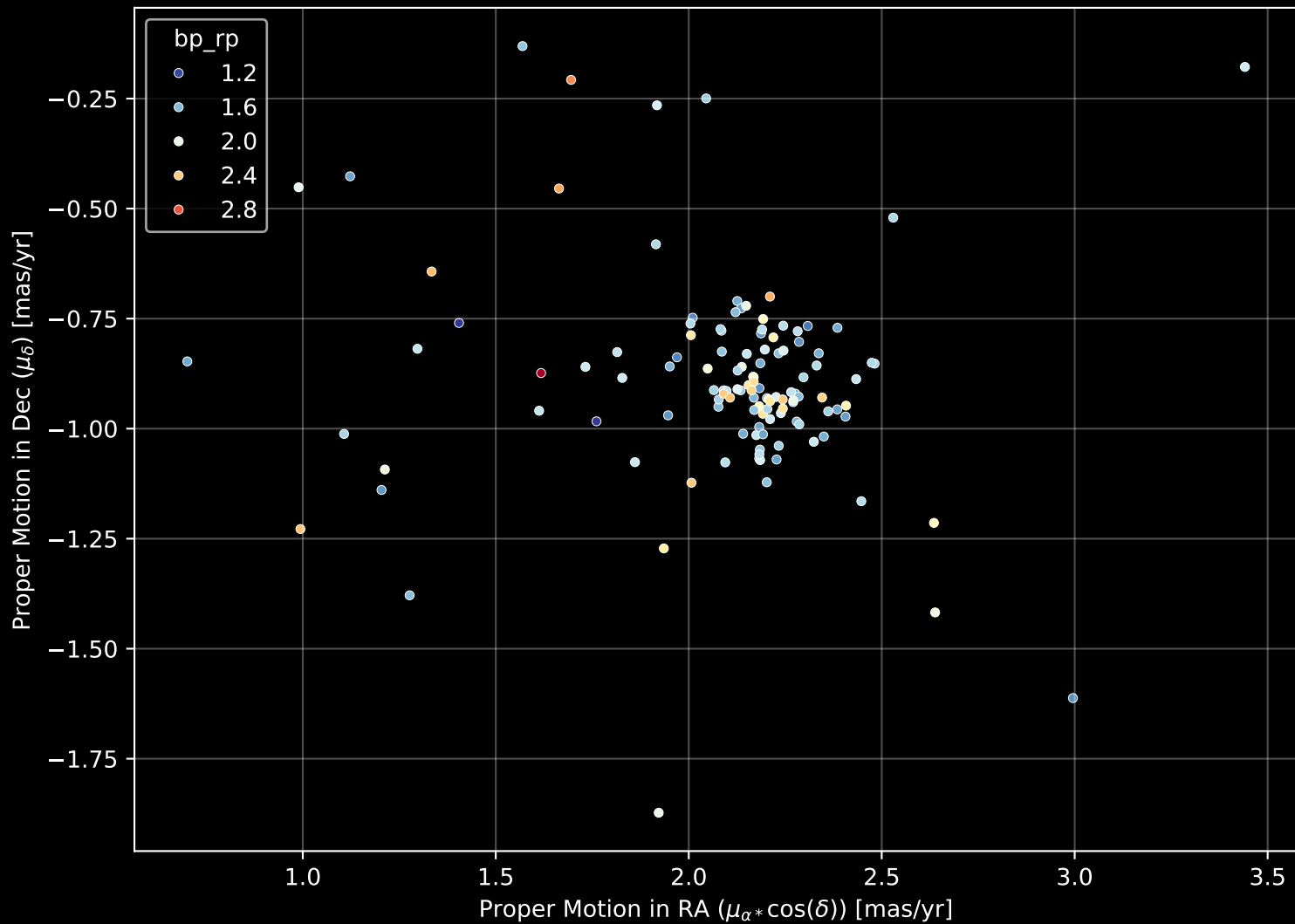
Gaia Cluster: [Czernik_21] Proper Motion Diagram (n= 124)
