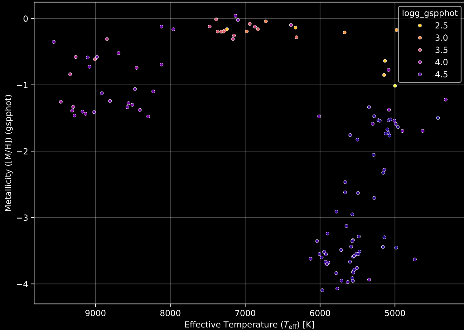
Gaia Cluster: [Czernik_21] Stellar Population Parameters (n= 124)
