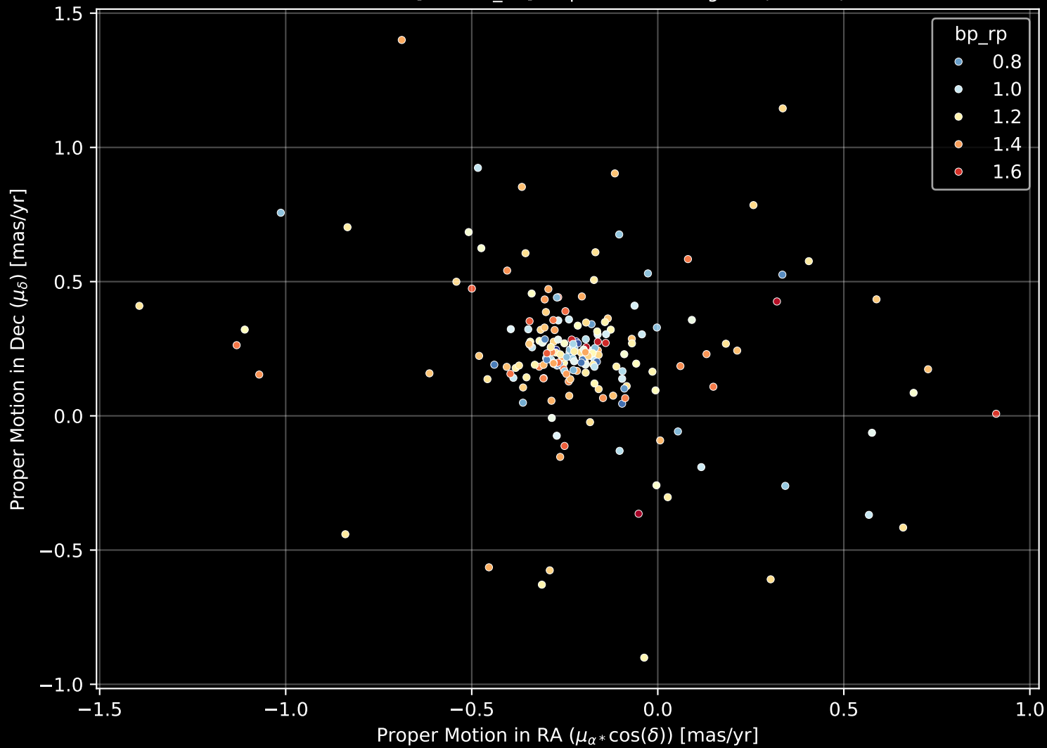
Gaia Cluster: [Czernik_25] Proper Motion Diagram (n= 199)
