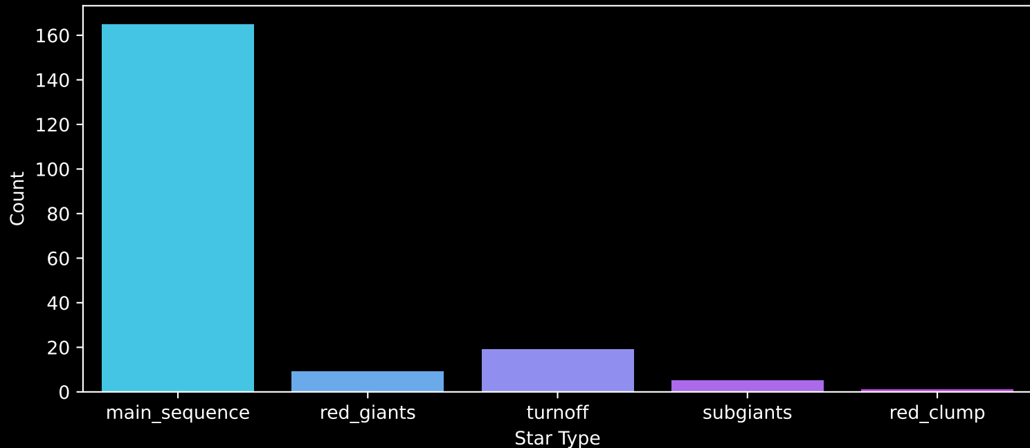
Gaia Cluster: [Czernik_25] Count plot of Star Type
