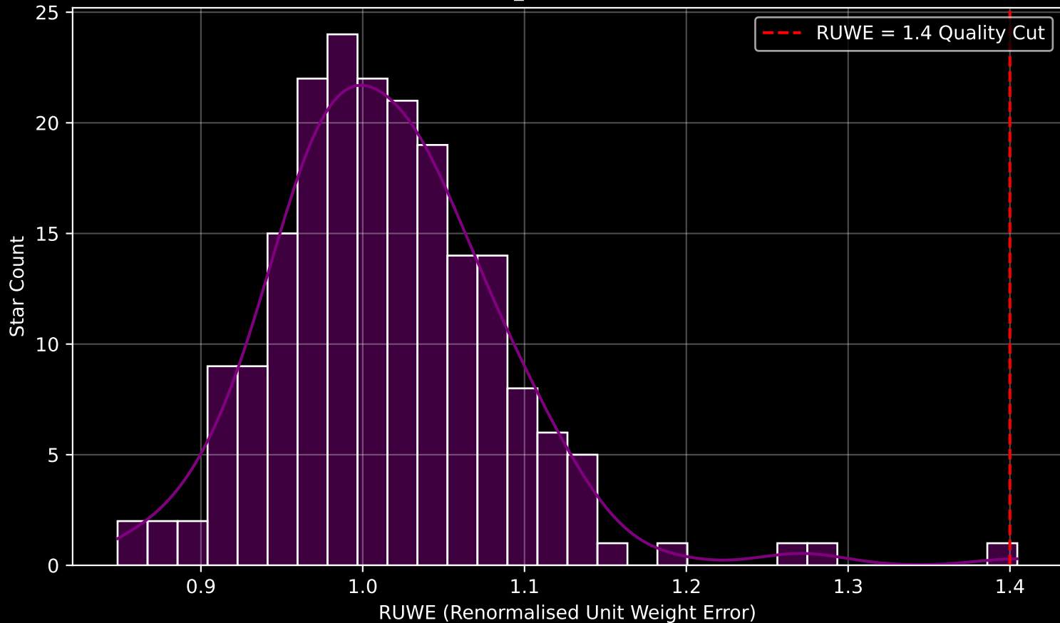
Gaia Cluster: [Czernik_25] RUWE Distribution (n= 199)
