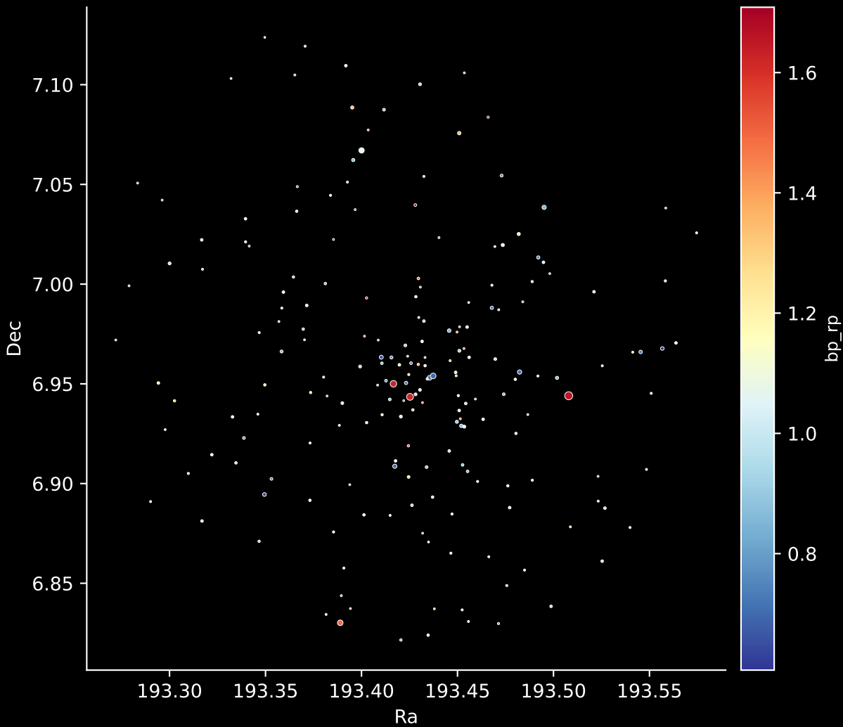
Gaia Cluster: [Czernik_25] Stars: 199
