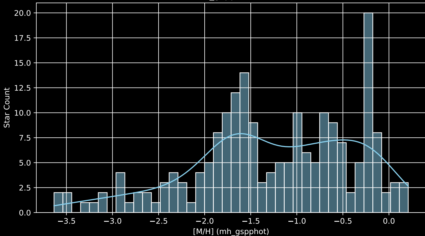
Gaia Cluster: [Czernik_25 [M/H] (mh_gspphot) (n= 198)
