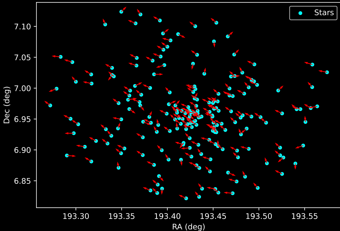
Gaia Cluster: [Czernik_25] Proper Motion Vectors for Gaia Star Field (n= 199)
