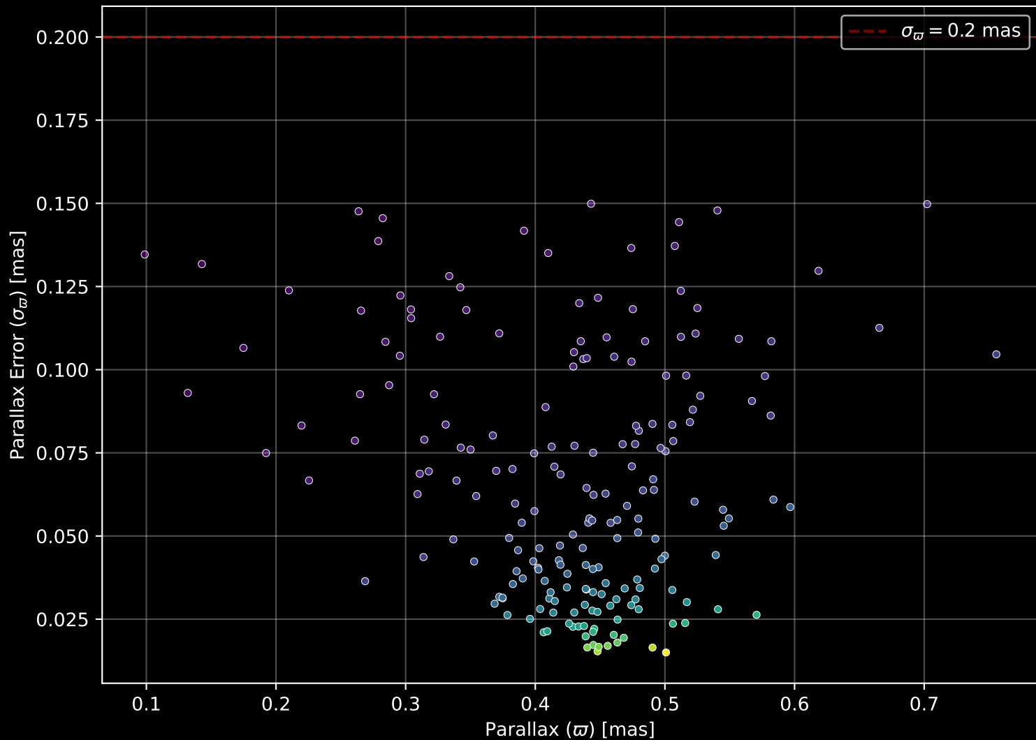
Gaia Cluster: [Czernik_25] Parallax Quality (n= 199)
