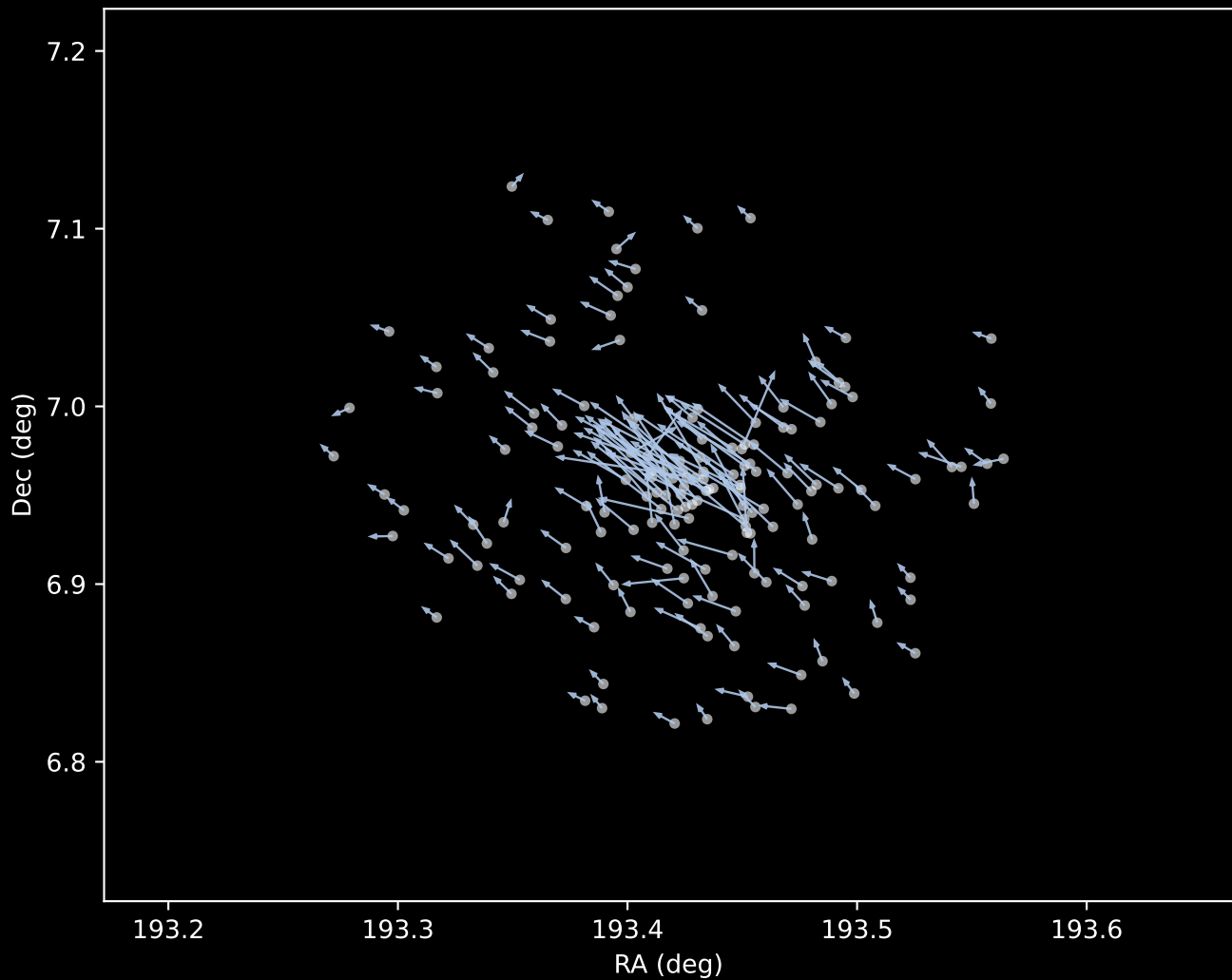
Gaia DR3 Cluster 1 Proper Motion Vectors (n=157)
