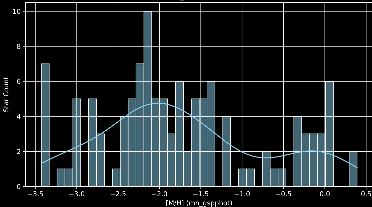
Gaia Cluster: [Czernik_26 [M/H] (mh_gspphot) (n= 117)
