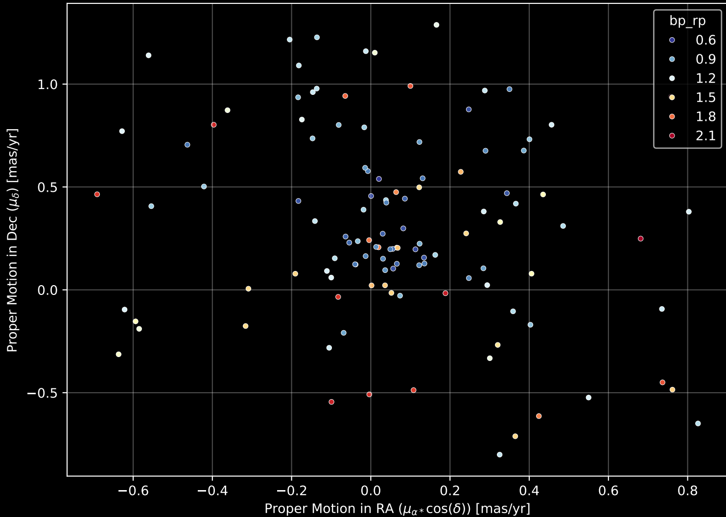
Gaia Cluster: [Czernik_26] Proper Motion Diagram (n= 117)
