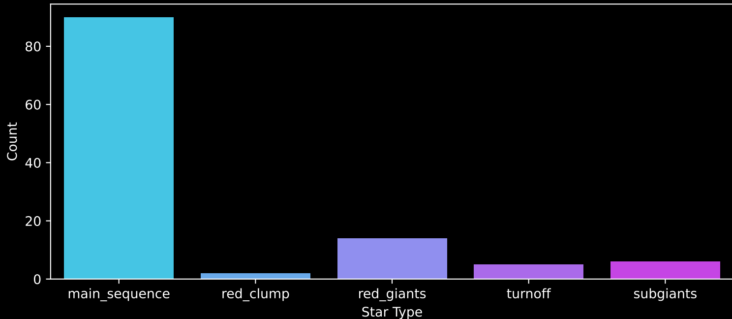
Gaia Cluster: [Czernik_26] Count plot of Star Type
