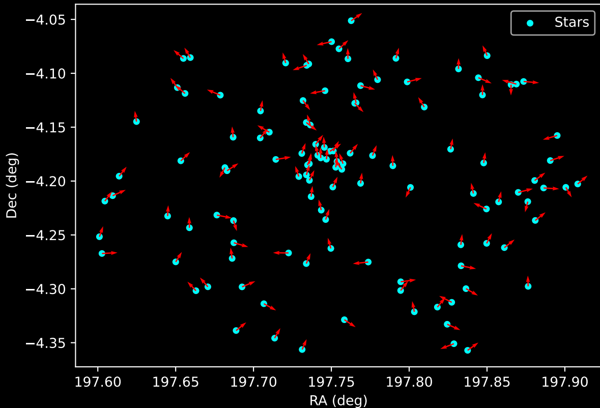
Gaia Cluster: [Czernik_26] Proper Motion Vectors for Gaia Star Field (n= 117)
