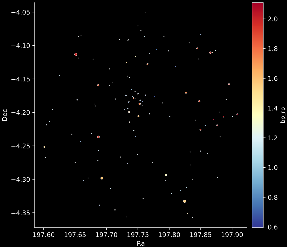
Gaia Cluster: [Czernik_26] Stars: 117
