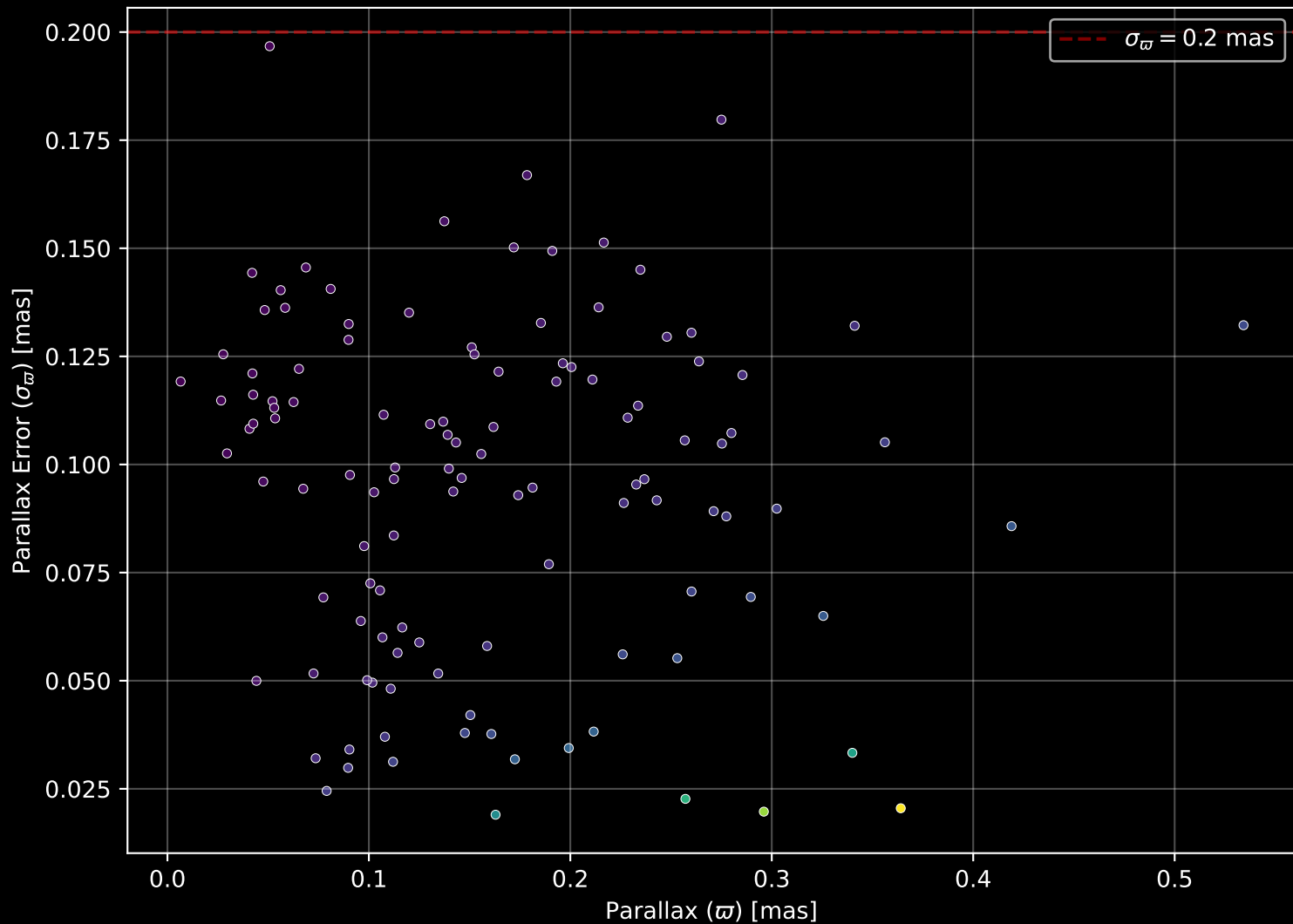
Gaia Cluster: [Czernik_26] Parallax Quality (n= 117)
