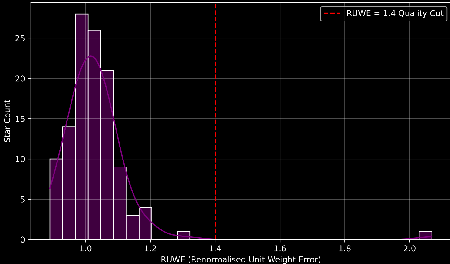
Gaia Cluster: [Czernik_26] RUWE Distribution (n= 117)
