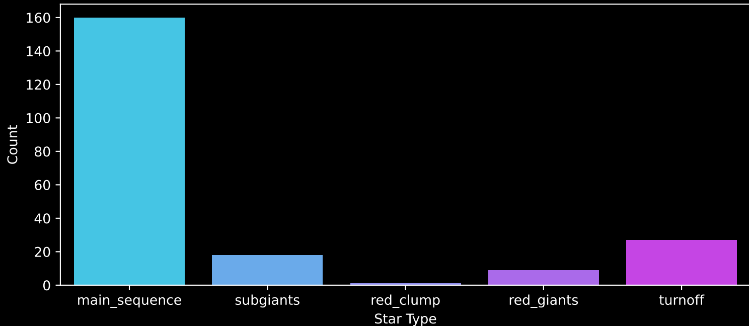
Gaia Cluster: [Czernik_31] Count plot of Star Type
