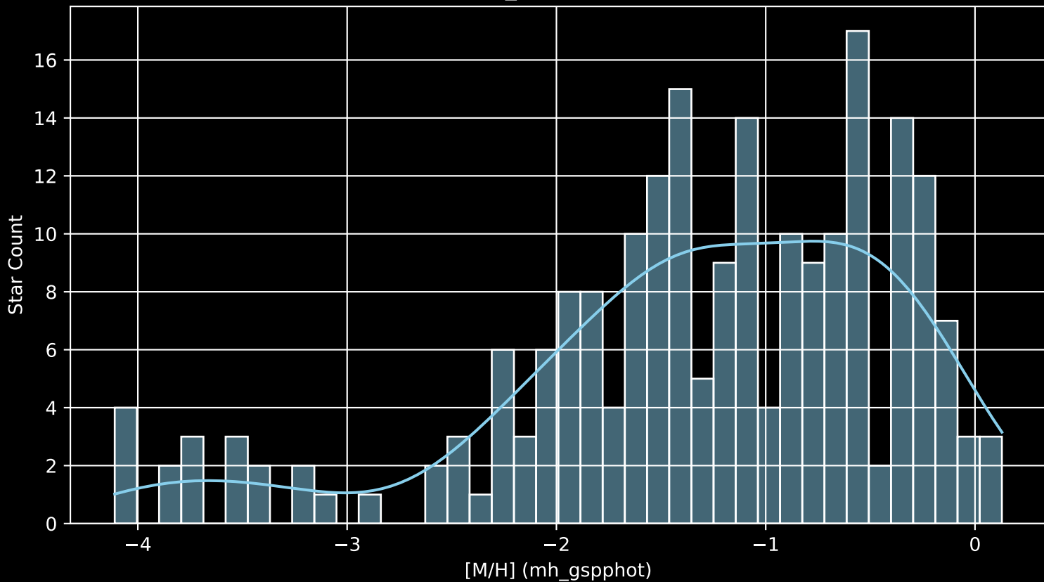
Gaia Cluster: [Czernik_31 [M/H] (mh_gspphot) (n= 215)
