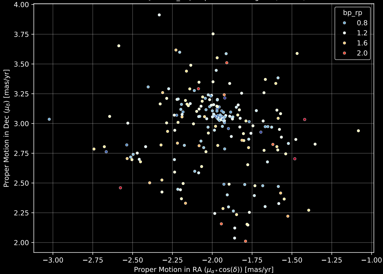
Gaia Cluster: [Czernik_31] Proper Motion Diagram (n= 215)
