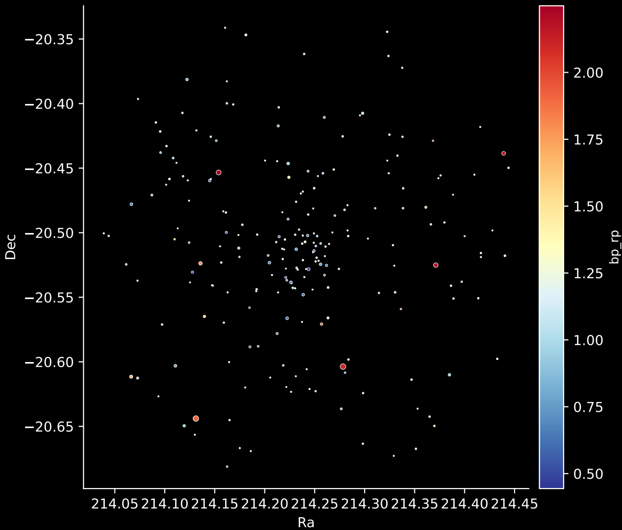
Gaia Cluster: [Czernik_31] Stars: 215
