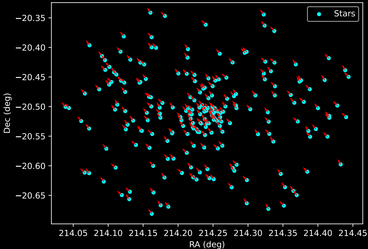
Gaia Cluster: [Czernik_31] Proper Motion Vectors for Gaia Star Field (n= 215)
