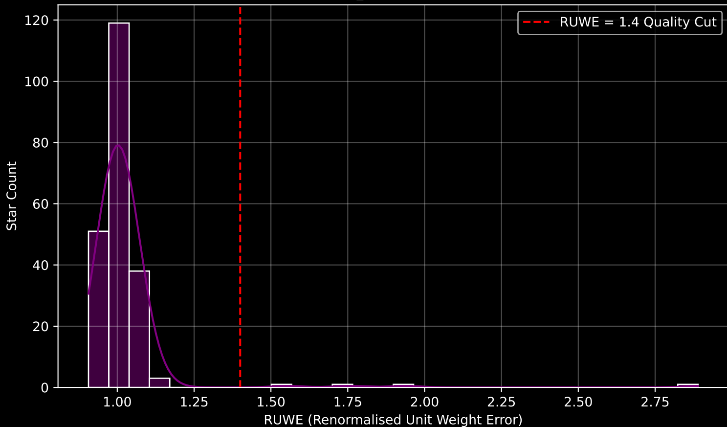
Gaia Cluster: [Czernik_31] RUWE Distribution (n= 215)
