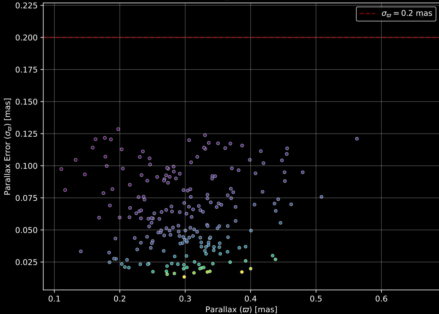
Gaia Cluster: [Czernik_31] Parallax Quality (n= 215)
