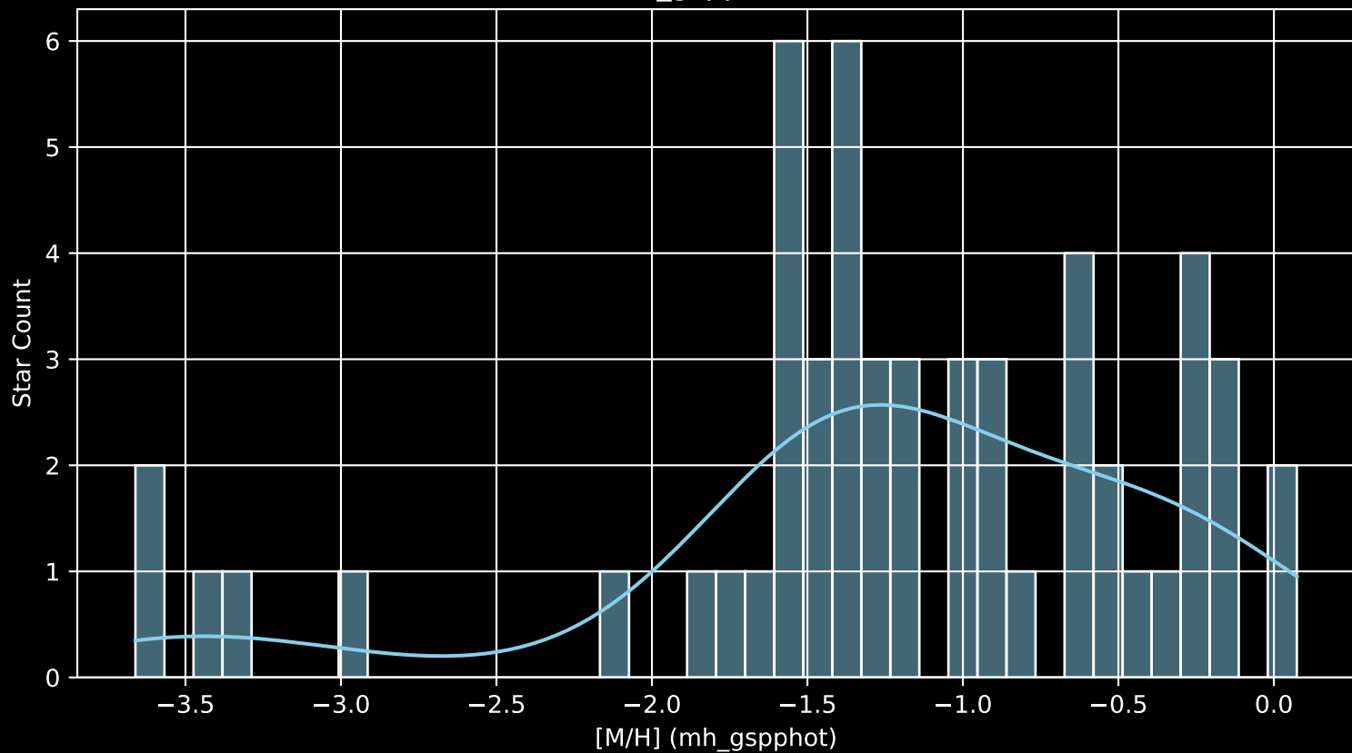
Gaia Cluster: [Czernik_8 [M/H] (mh_gspphot) (n= 54)
