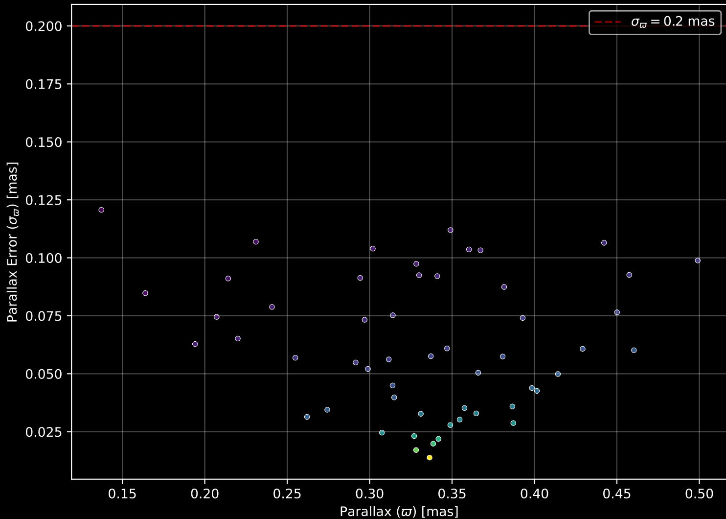
Gaia Cluster: [Czernik_8] Parallax Quality (n= 54)
