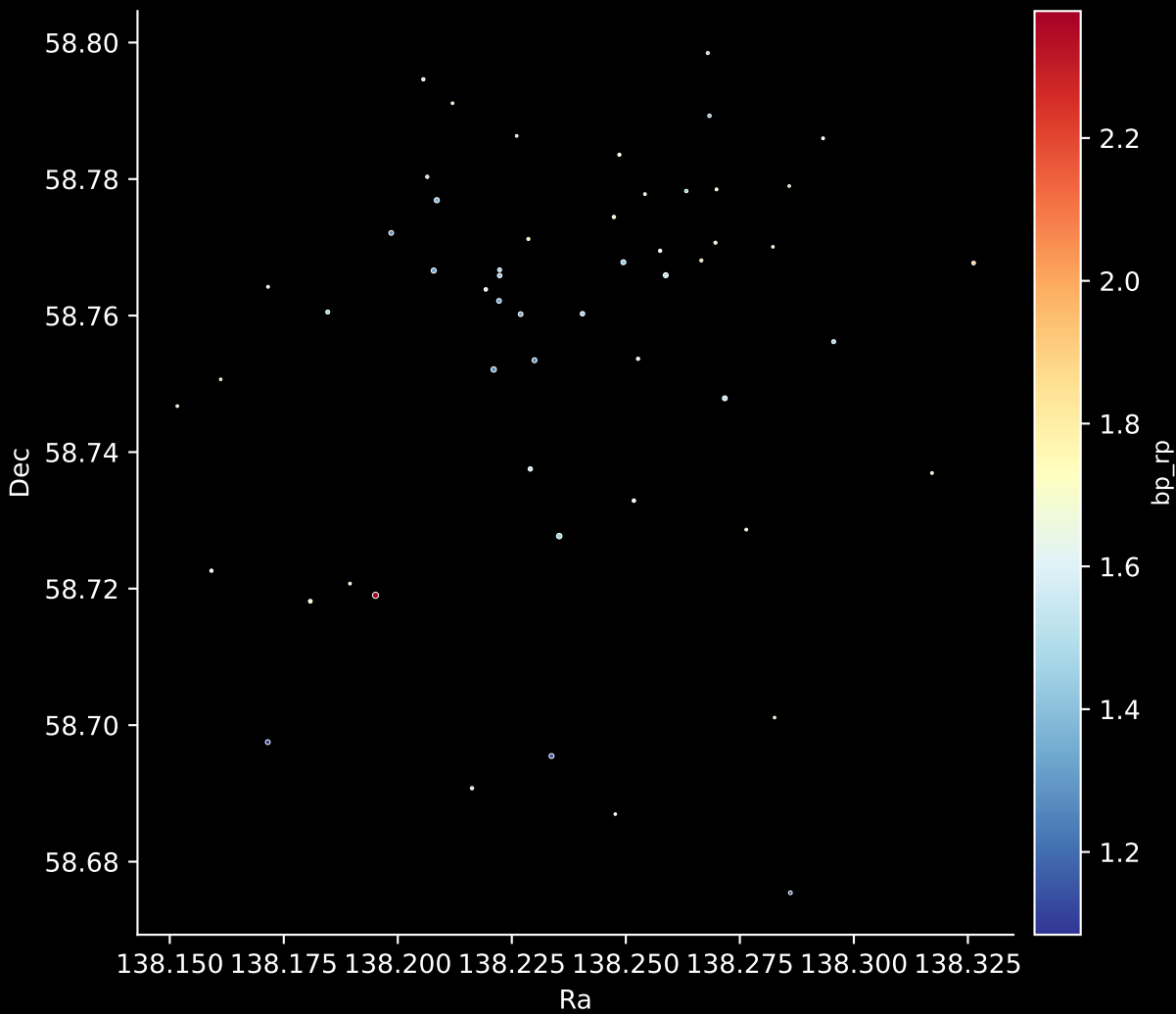
Gaia Cluster: [Czernik_8] Stars: 54
