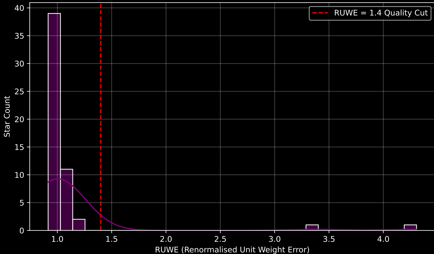
Gaia Cluster: [Czernik_8] RUWE Distribution (n= 54)
