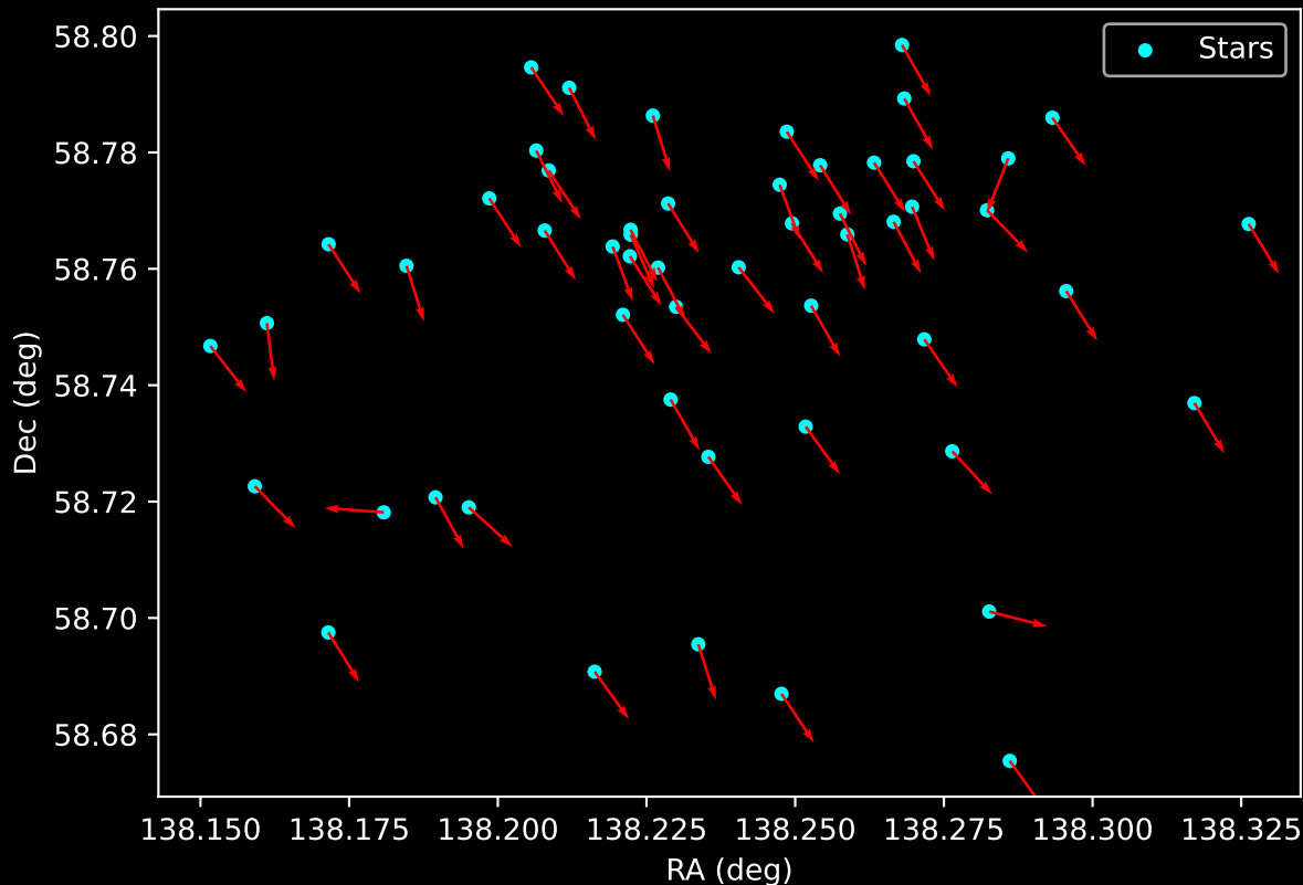
Gaia Cluster: [Czernik_8] Proper Motion Vectors for Gaia Star Field (n= 54)
