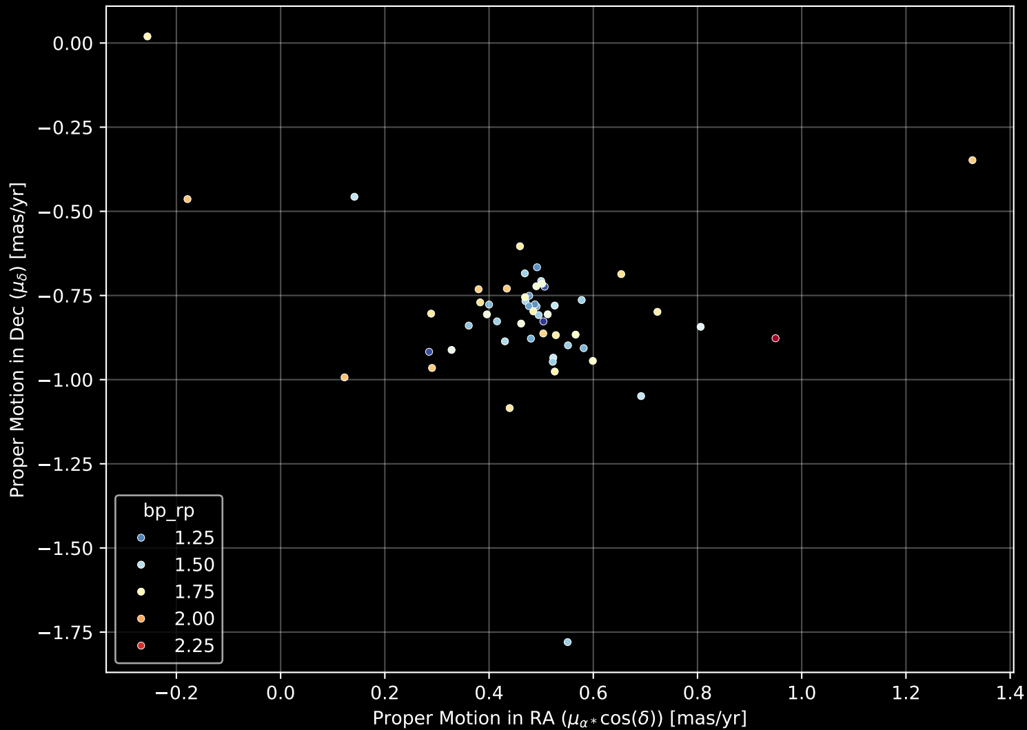
Gaia Cluster: [Czernik_8] Proper Motion Diagram (n= 54)
