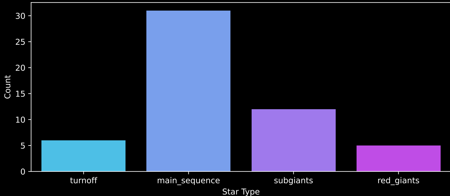
Gaia Cluster: [Czernik_8] Count plot of Star Type
