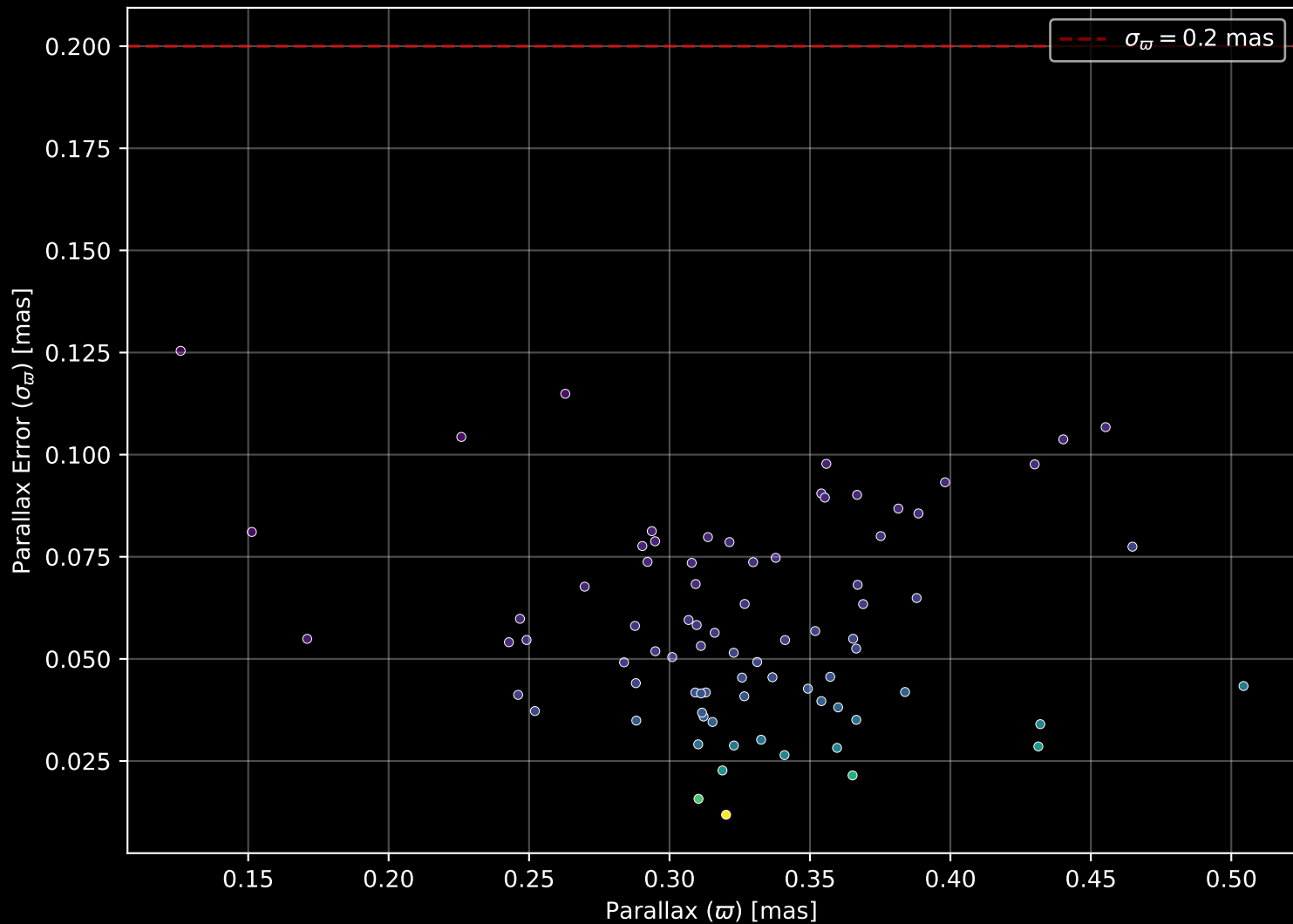
Gaia Cluster: [Czernik_9] Parallax Quality (n= 80)
