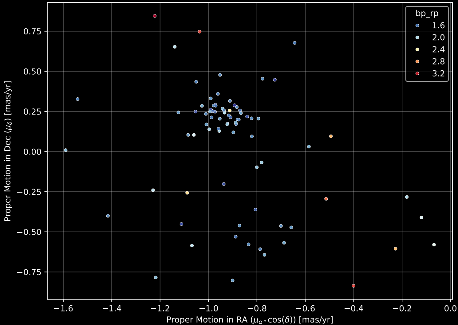
Gaia Cluster: [Czernik_9] Proper Motion Diagram (n= 80)
