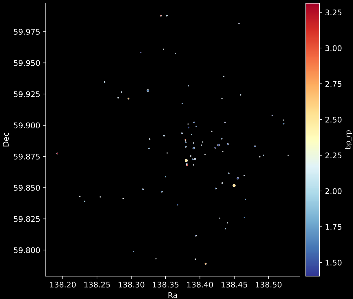
Gaia Cluster: [Czernik_9] Stars: 80
