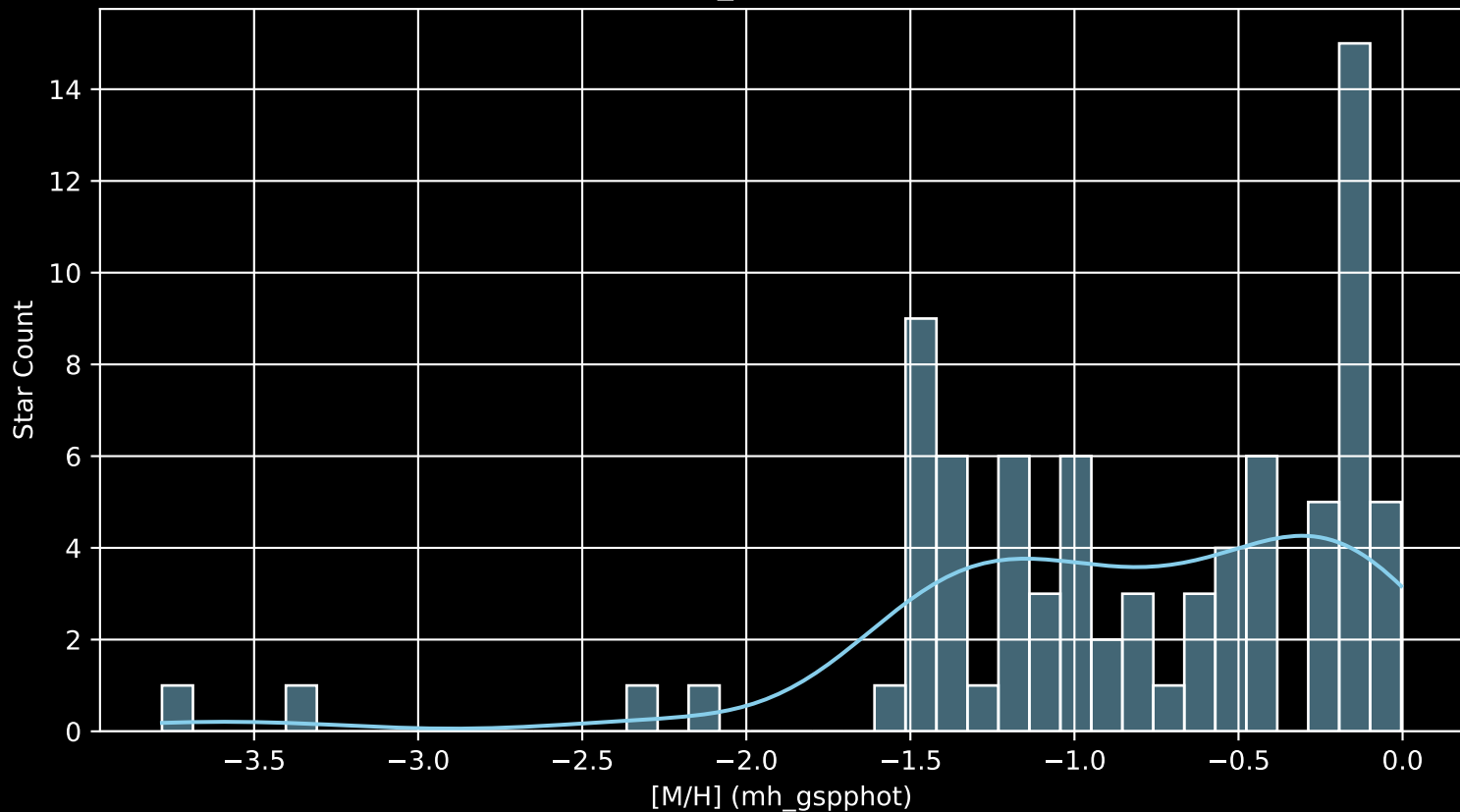
Gaia Cluster: [Czernik_9 [M/H] (mh_gspphot) (n= 80)
