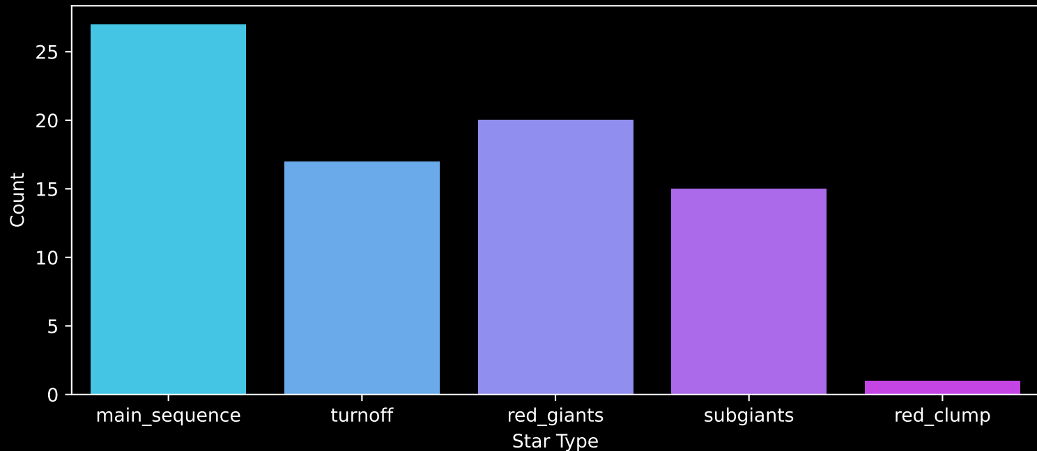
Gaia Cluster: [Czernik_9] Count plot of Star Type
