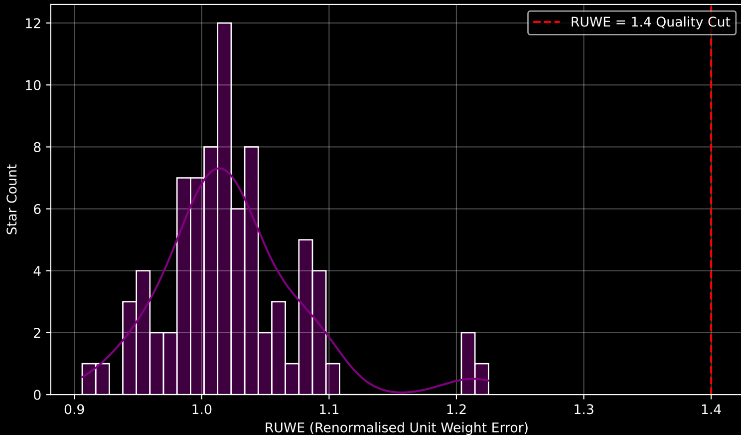
Gaia Cluster: [Czernik_9] RUWE Distribution (n= 80)
