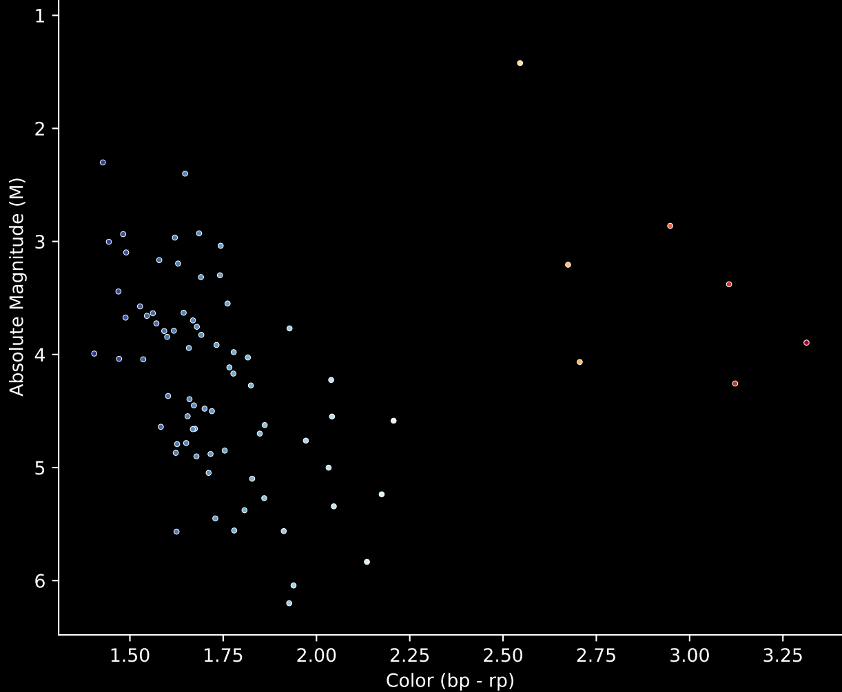
Gaia Cluster: [Czernik_9] Stars (n= 80) Hertzprung-Russel Diagram
