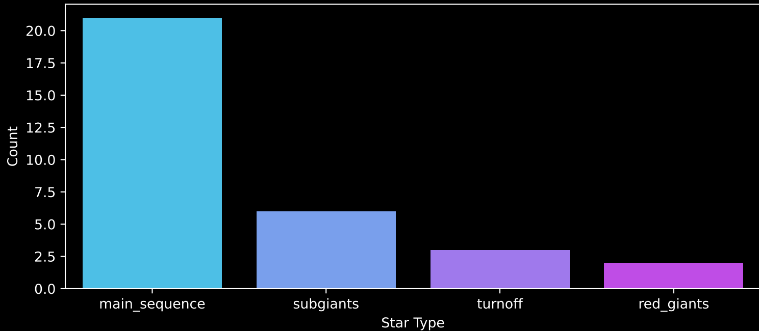
Gaia Cluster: [DBSB_104] Count plot of Star Type
