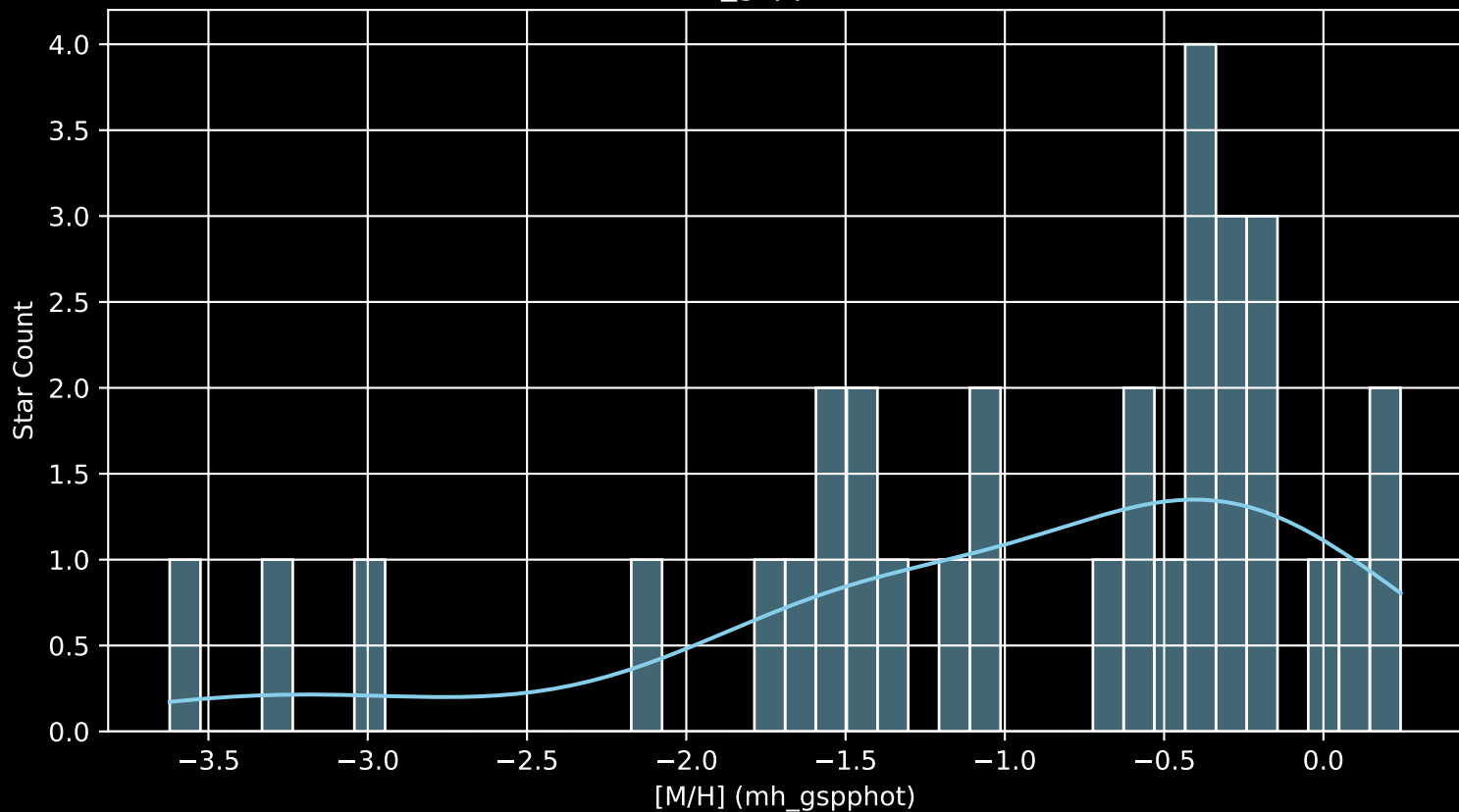
Gaia Cluster: [DBSB_104 [M/H] (mh_gspphot) (n= 32)
