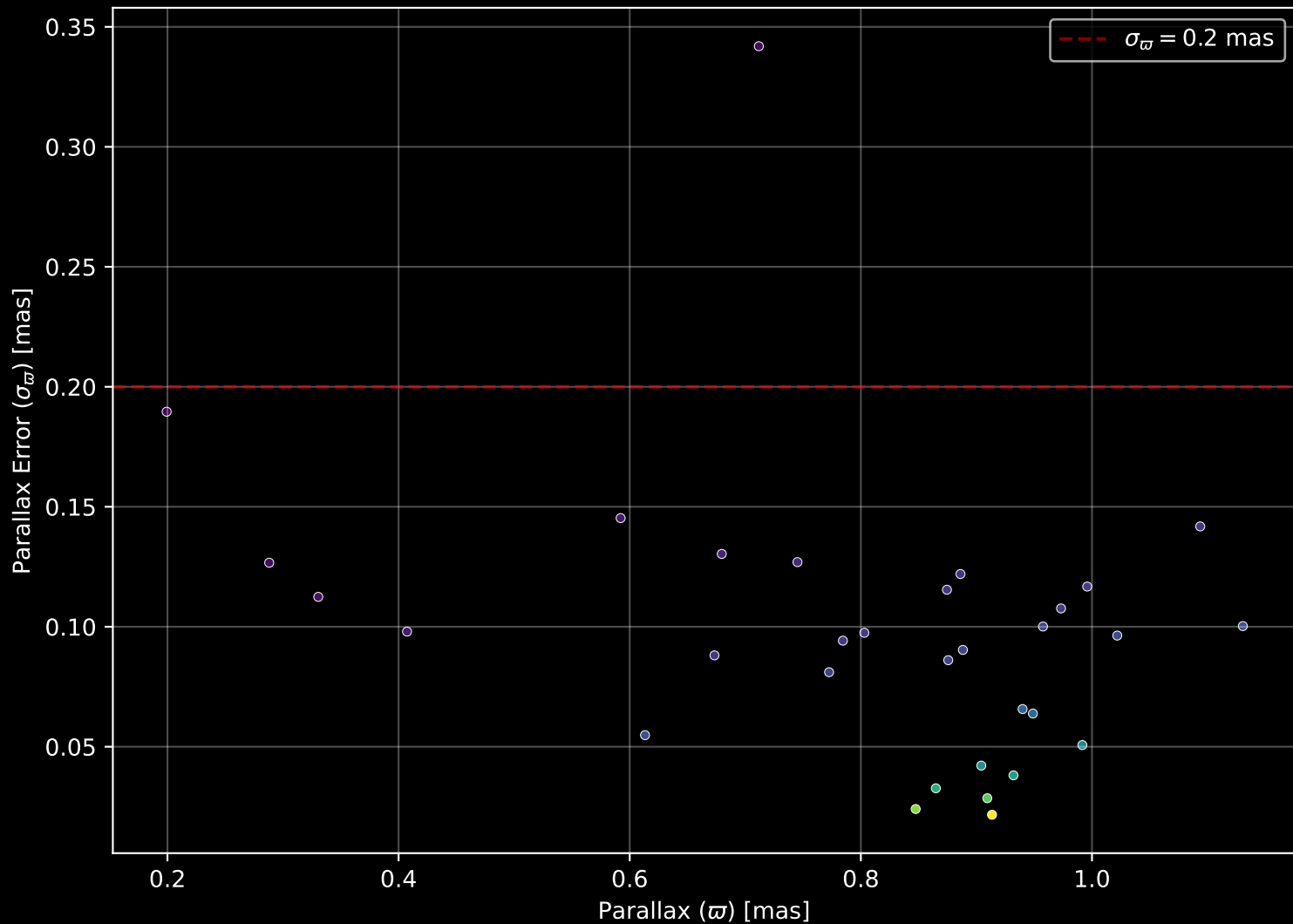
Gaia Cluster: [DBSB_104] Parallax Quality (n= 32)
