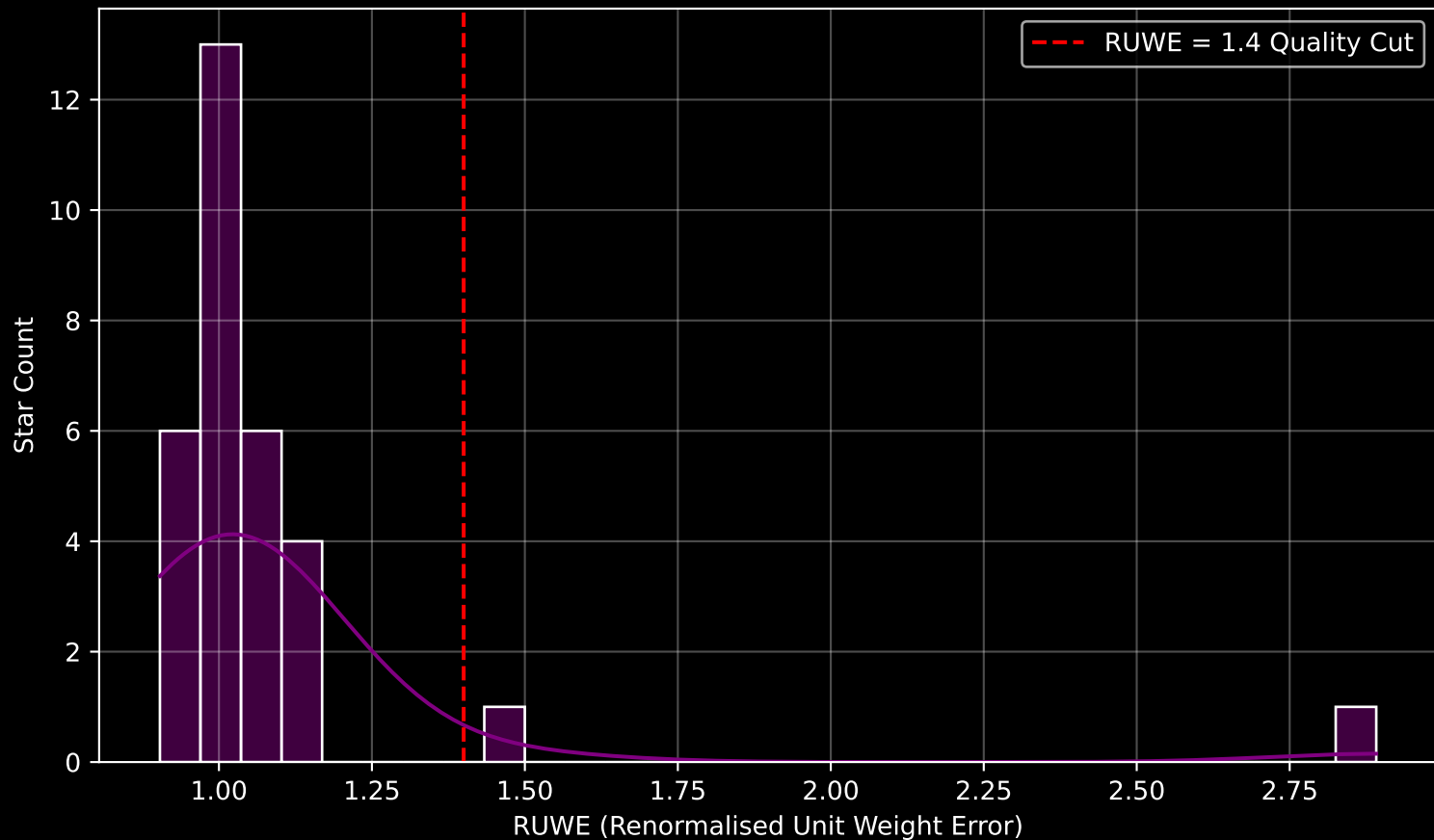
Gaia Cluster: [DBSB_104] RUWE Distribution (n= 31)
