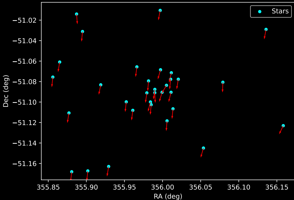
Gaia Cluster: [DBSB_104] Proper Motion Vectors for Gaia Star Field (n= 32)
