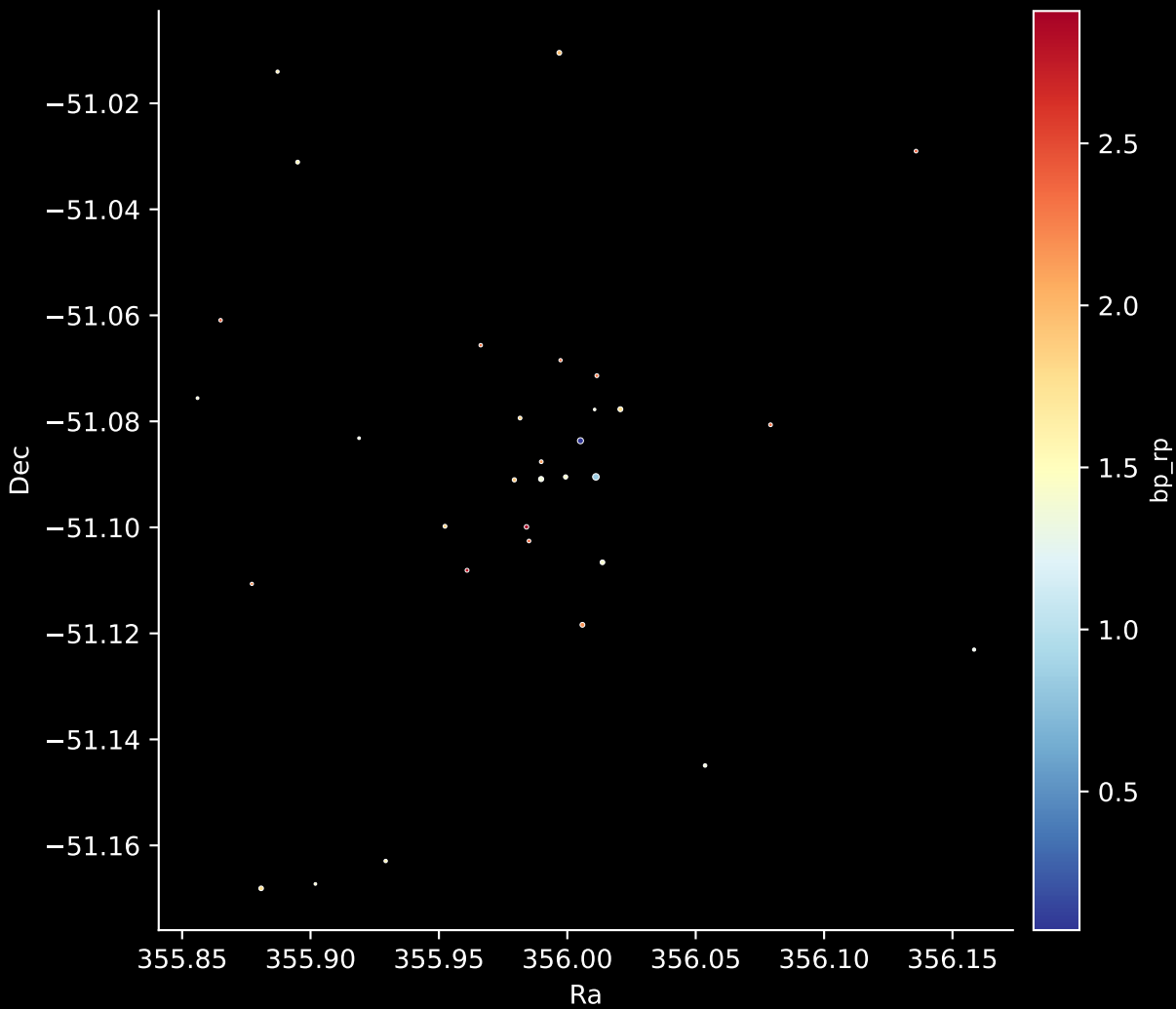
Gaia Cluster: [DBSB_104] Stars: 32
