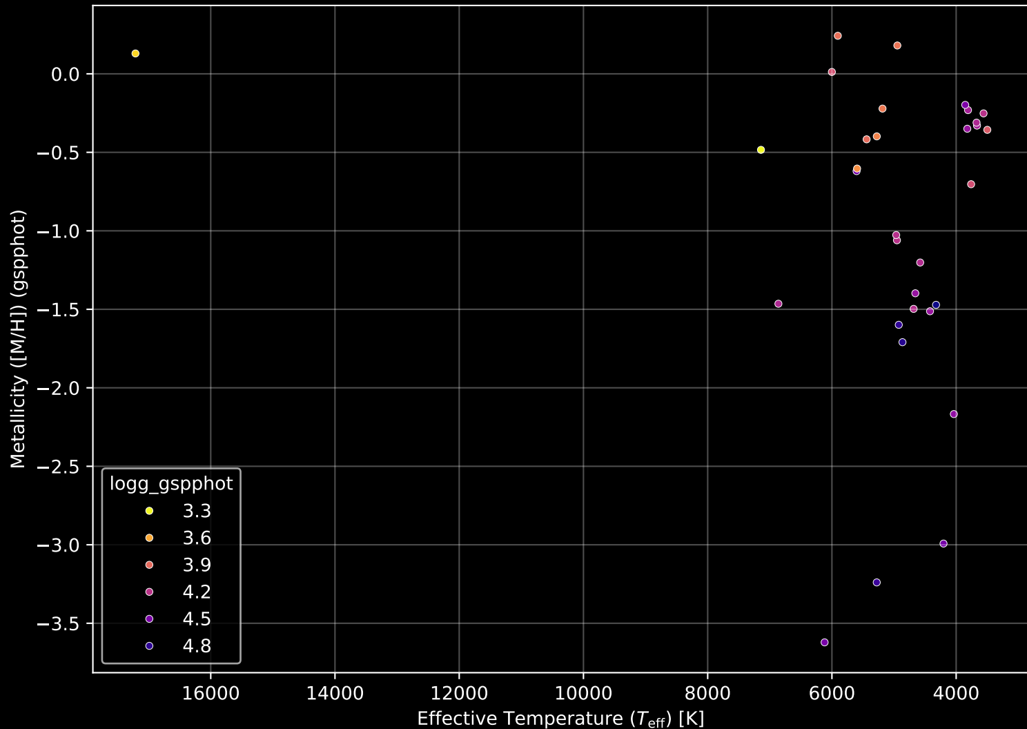
Gaia Cluster: [DBSB_104] Stellar Population Parameters (n= 32)
