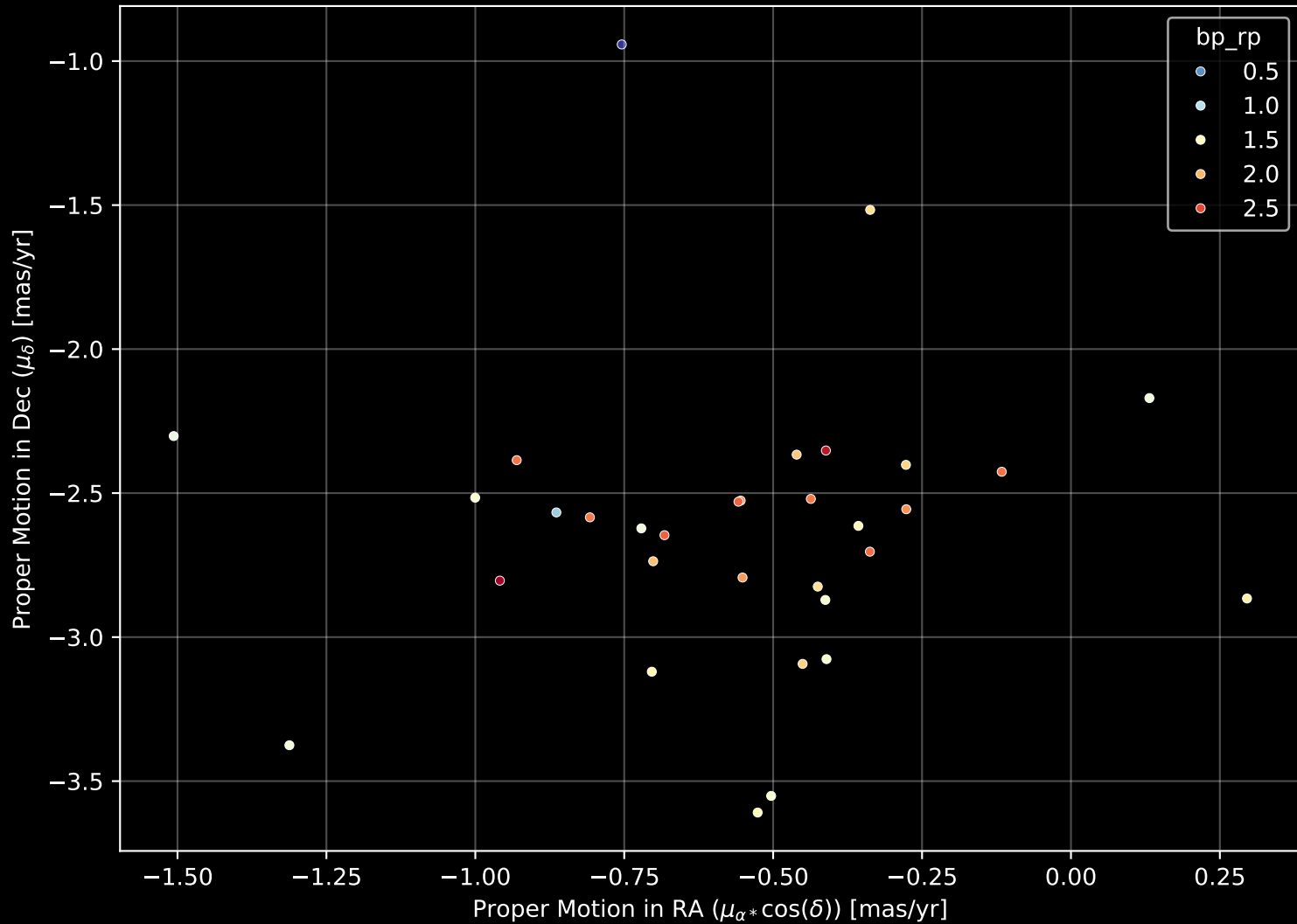
Gaia Cluster: [DBSB_104] Proper Motion Diagram (n= 32)
