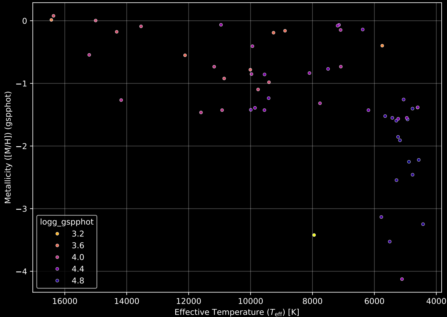
Gaia Cluster: [DBSB_3] Stellar Population Parameters (n= 56)
