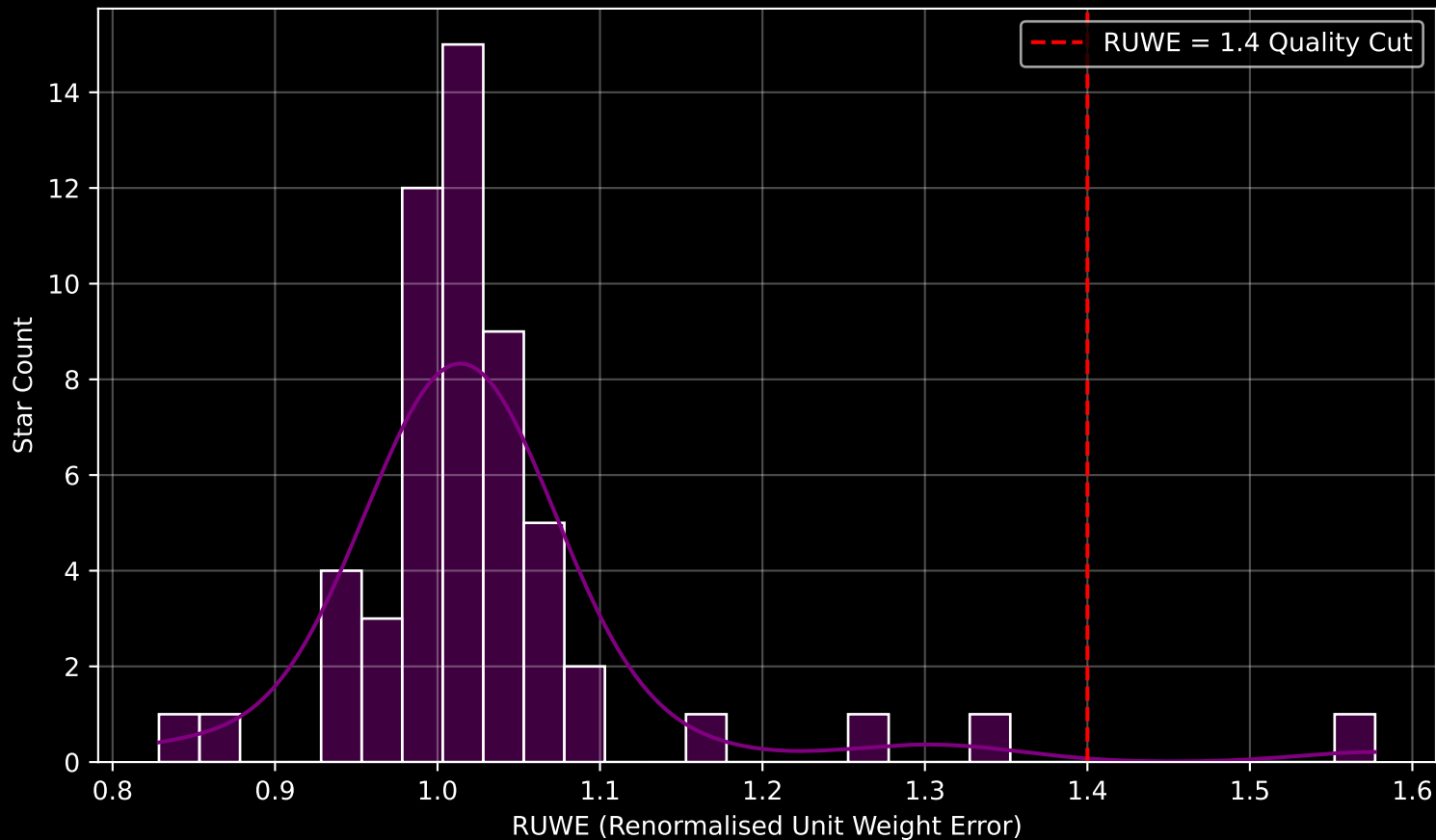
Gaia Cluster: [DBSB_3] RUWE Distribution (n= 56)
