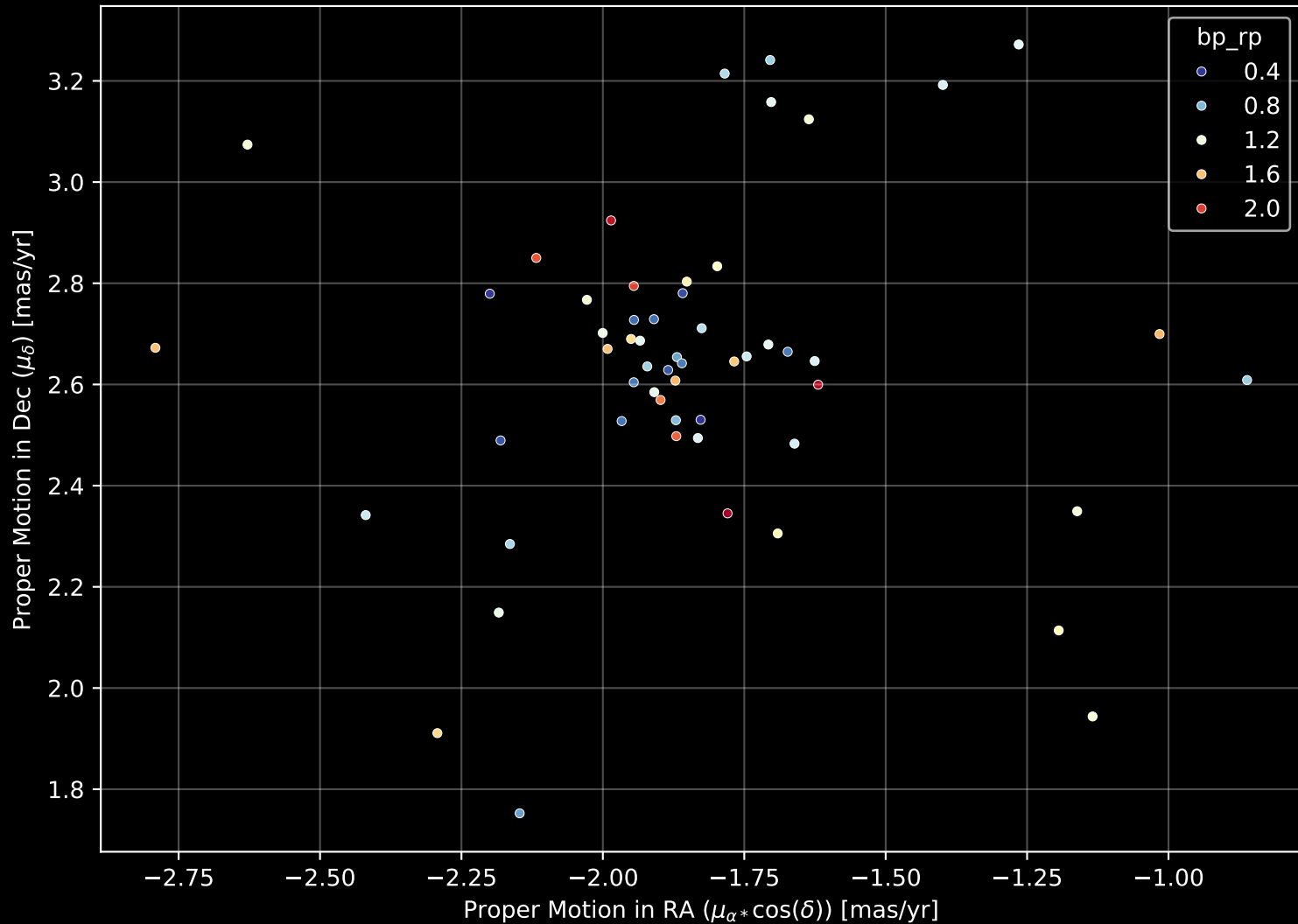
Gaia Cluster: [DBSB_3] Proper Motion Diagram (n= 56)
