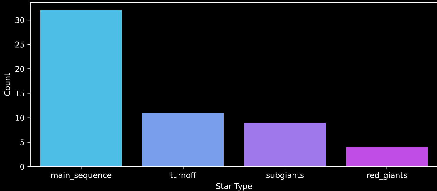
Gaia Cluster: [DBSB_3] Count plot of Star Type
