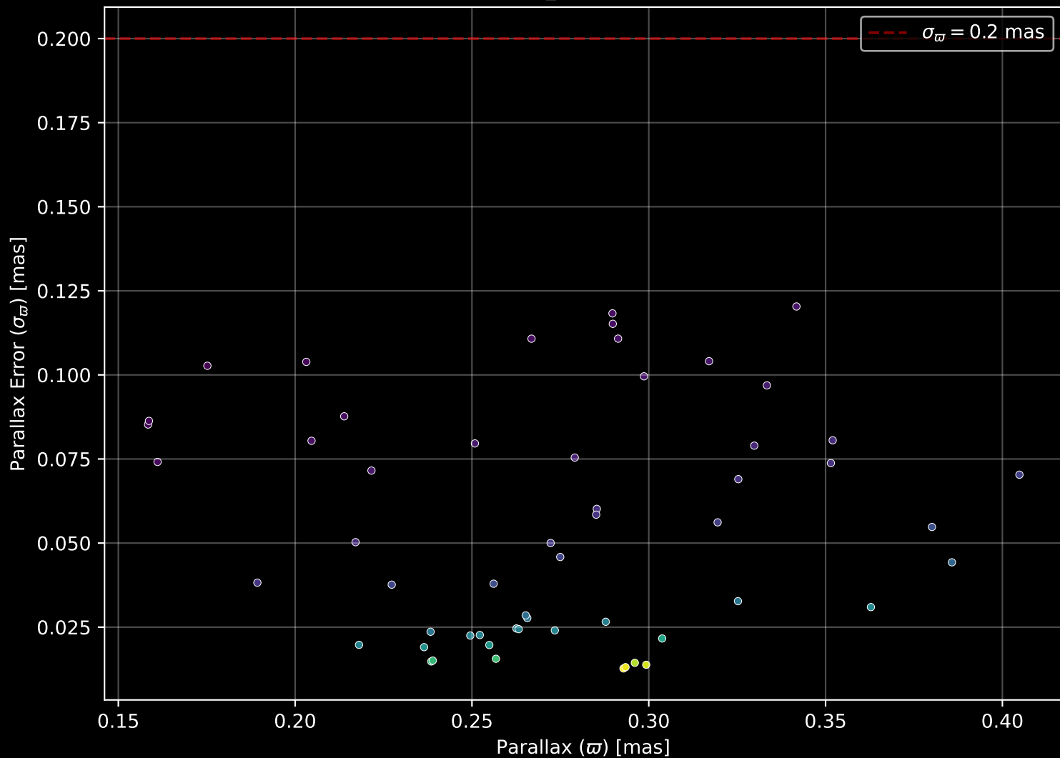
Gaia Cluster: [DBSB_3] Parallax Quality (n= 56)
