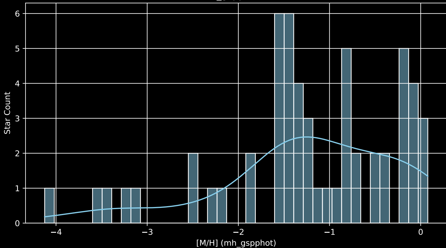
Gaia Cluster: [DBSB_3 [M/H] (mh_gspphot) (n= 56)
