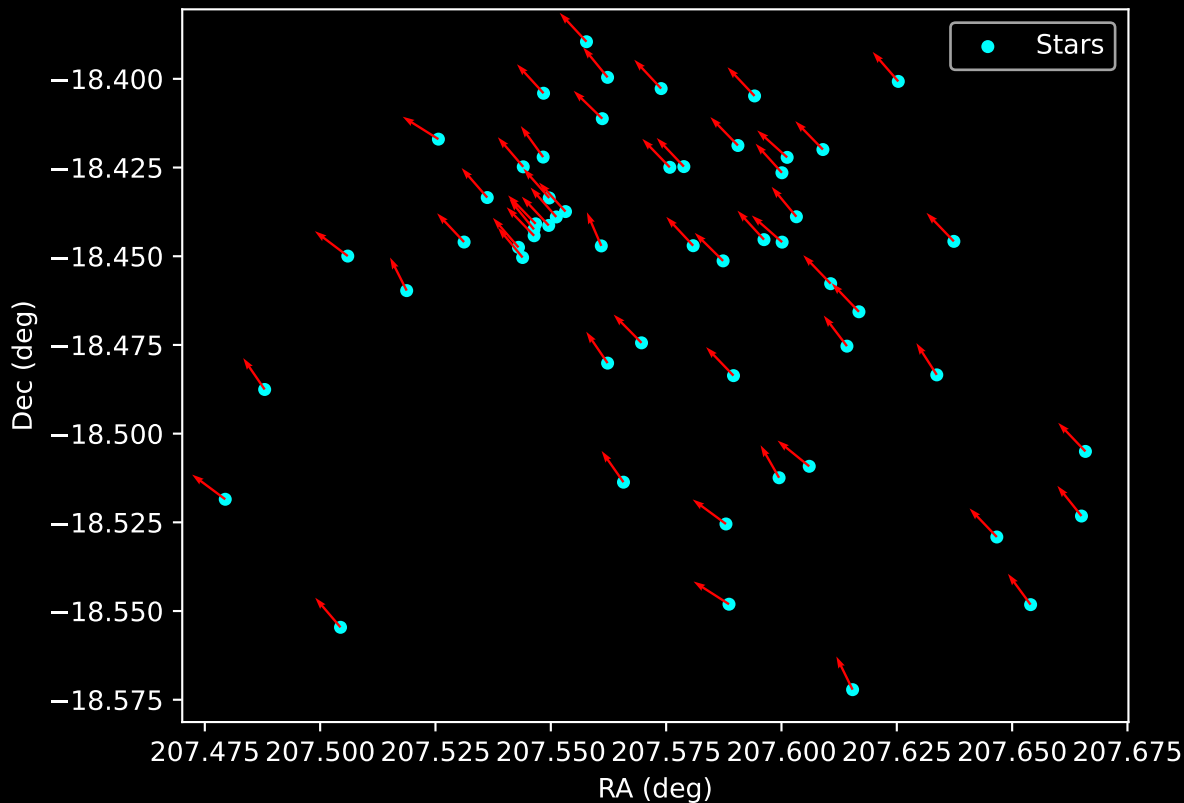
Gaia Cluster: [DBSB_3] Proper Motion Vectors for Gaia Star Field (n= 56)
