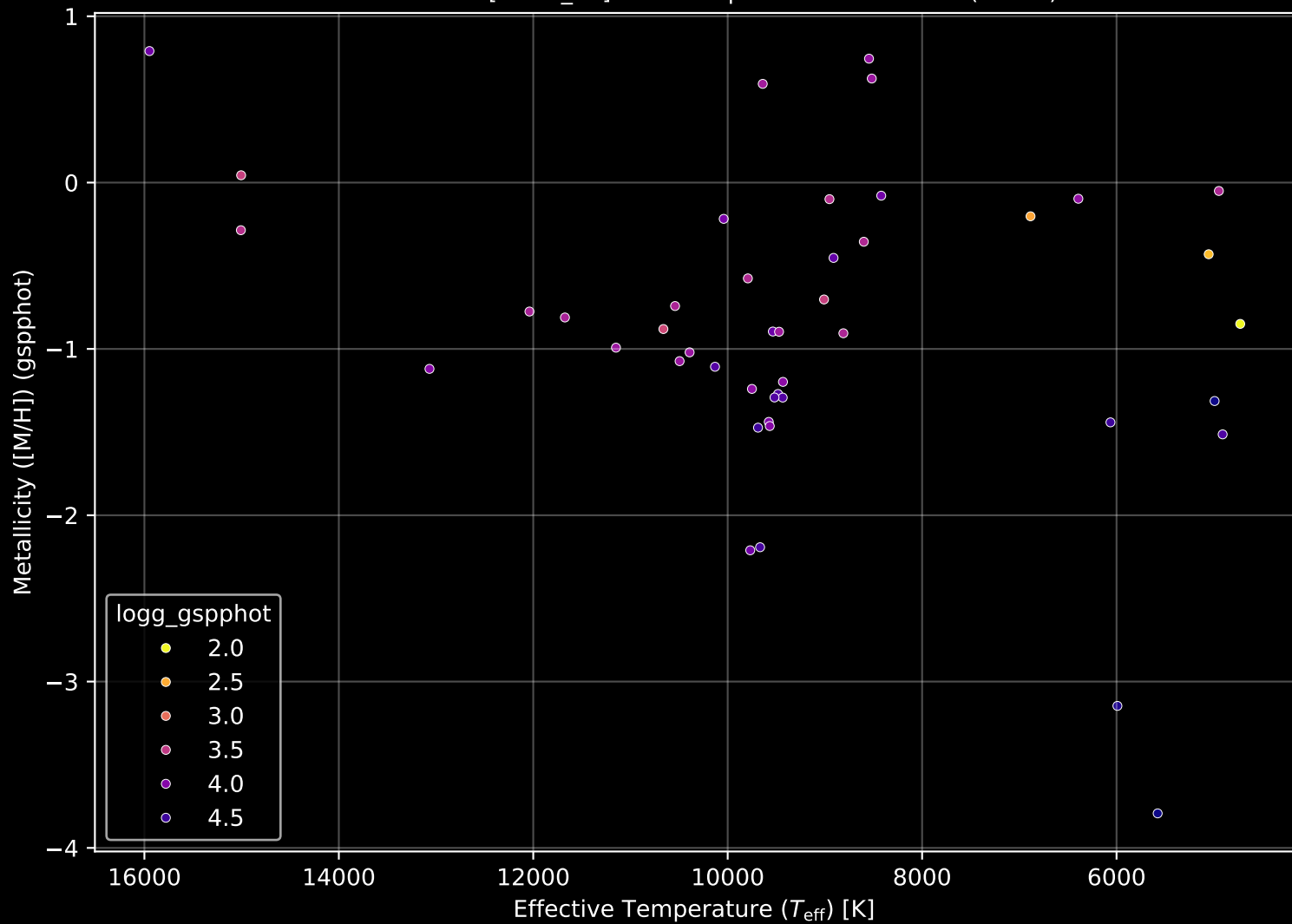
Gaia Cluster: [DBSB_43] Stellar Population Parameters (n= 45)
