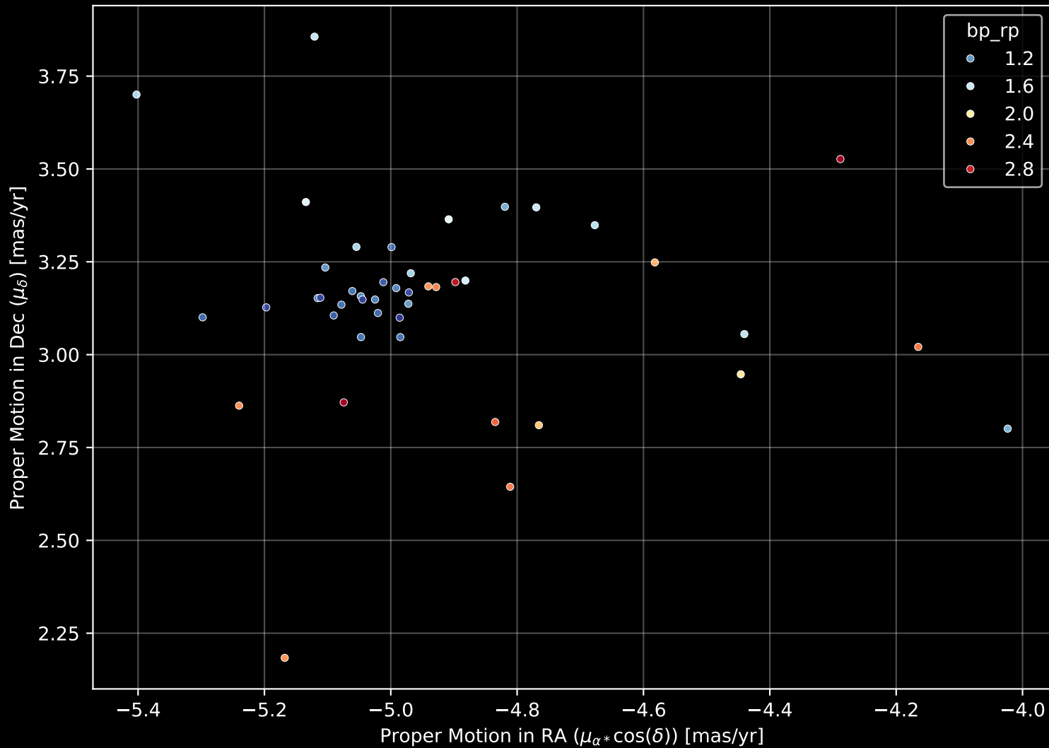
Gaia Cluster: [DBSB_43] Proper Motion Diagram (n= 45)
