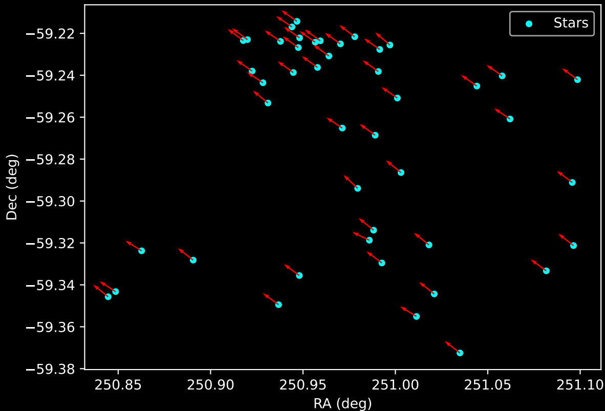
Gaia Cluster: [DBSB_43] Proper Motion Vectors for Gaia Star Field (n= 45)
