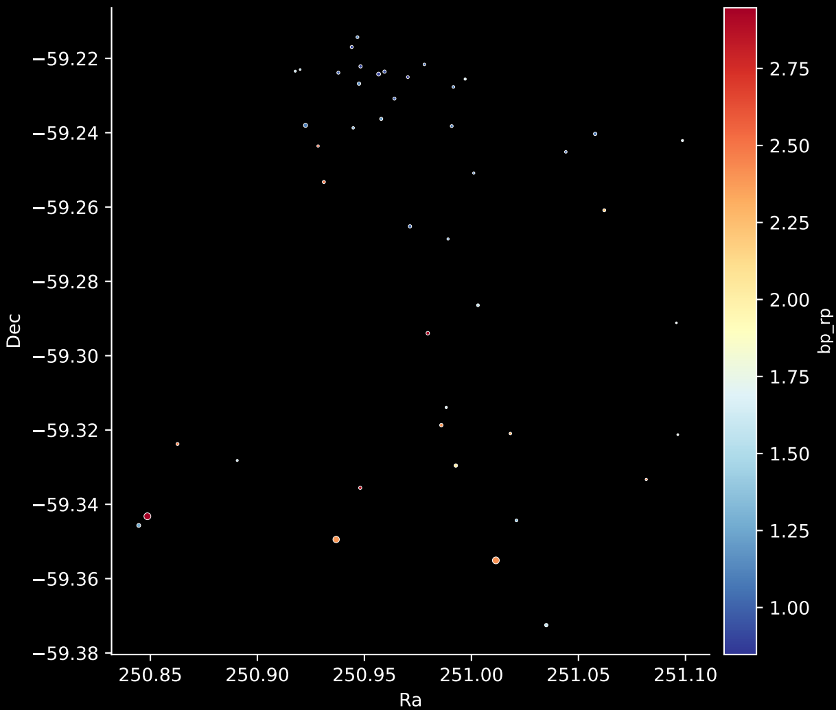
Gaia Cluster: [DBSB_43] Stars: 45
