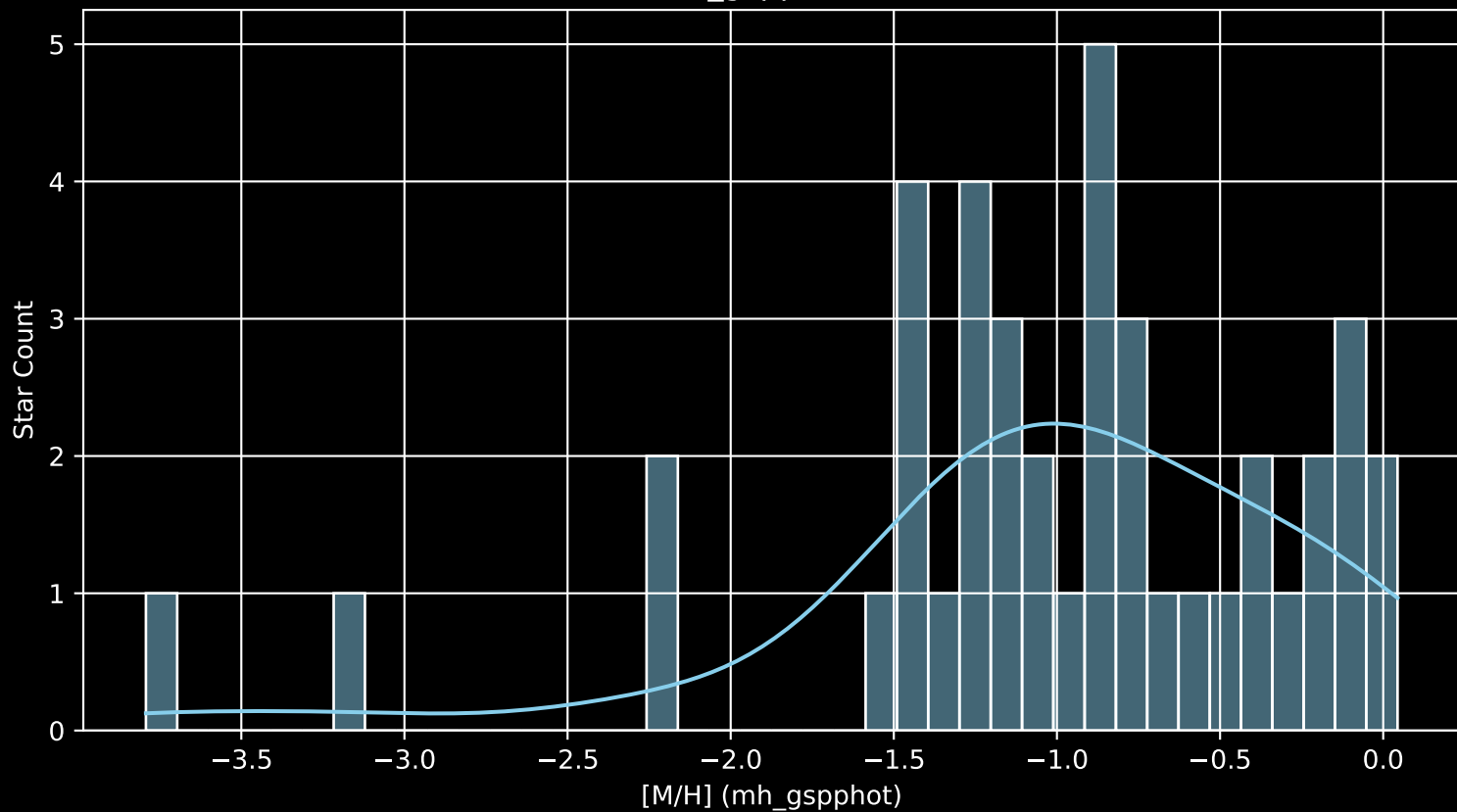
Gaia Cluster: [DBSB_43 [M/H] (mh_gspphot) (n= 41)
