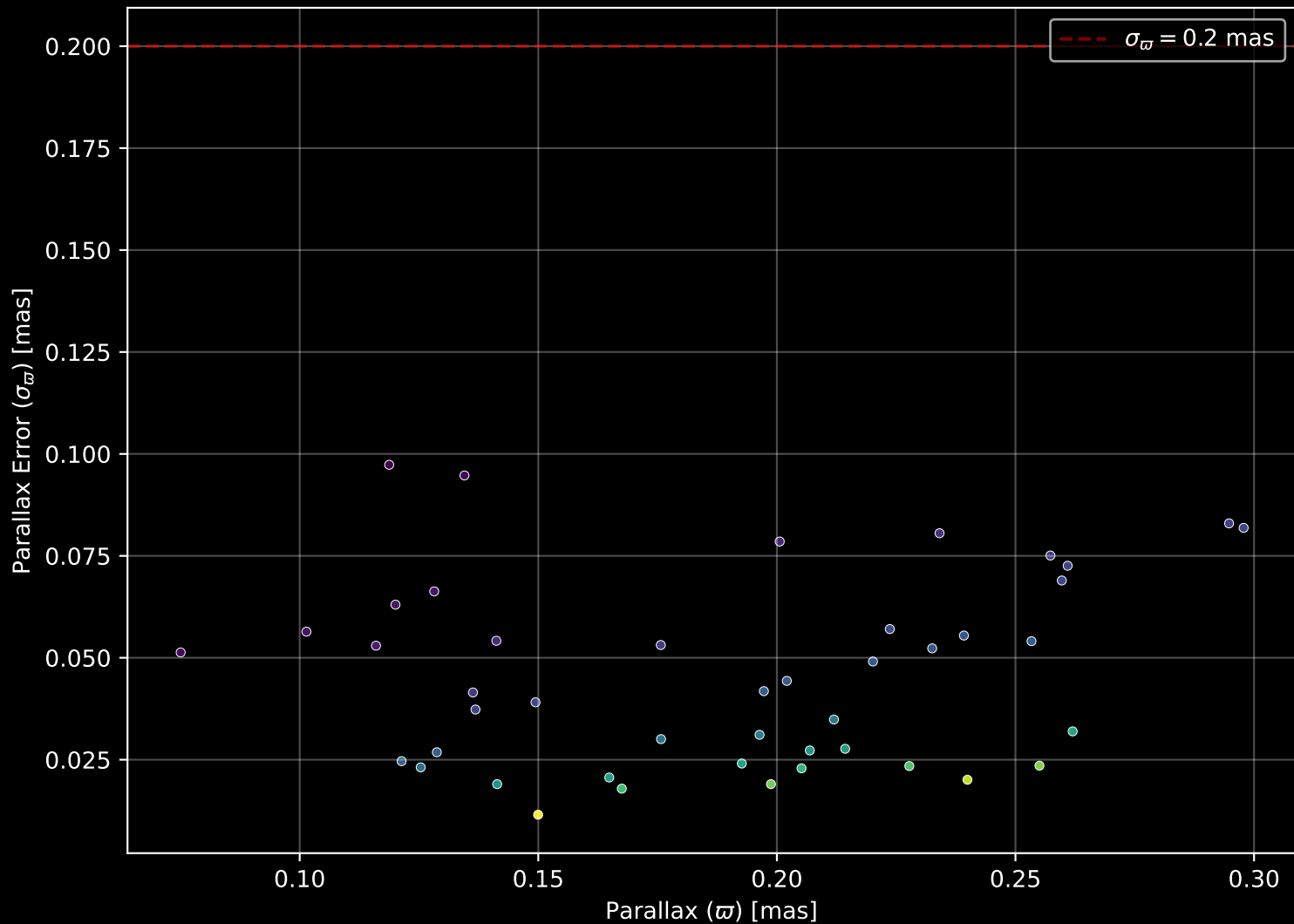
Gaia Cluster: [DBSB_43] Parallax Quality (n= 45)
