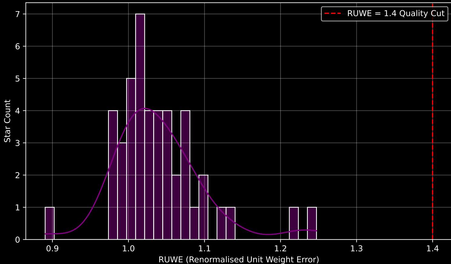
Gaia Cluster: [DBSB_43] RUWE Distribution (n= 45)
