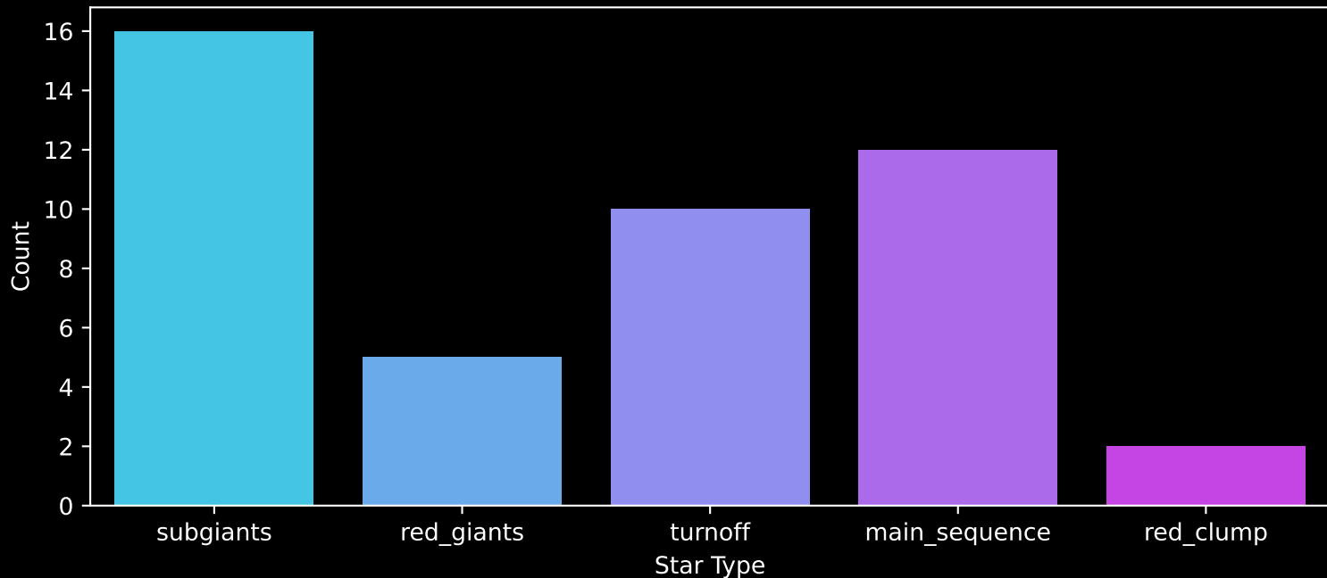
Gaia Cluster: [DBSB_43] Count plot of Star Type
