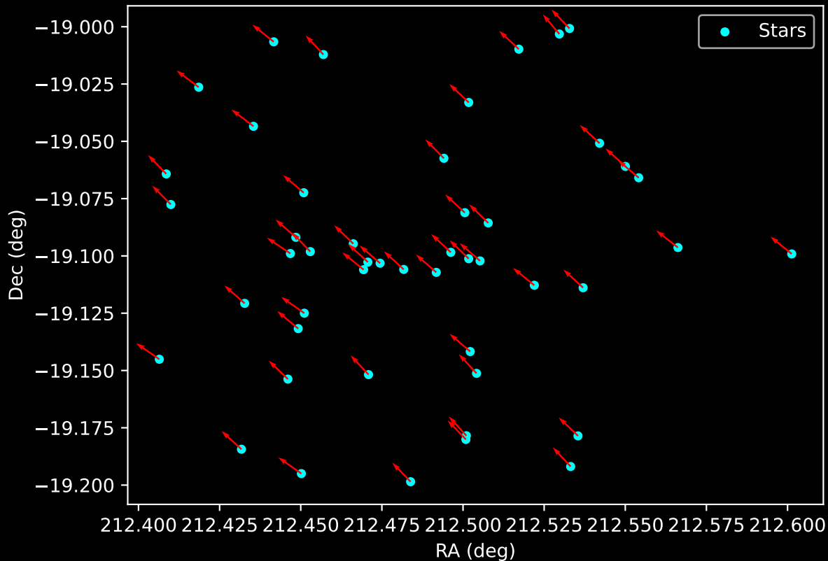
Gaia Cluster: [DBSB_6] Proper Motion Vectors for Gaia Star Field (n= 48)
