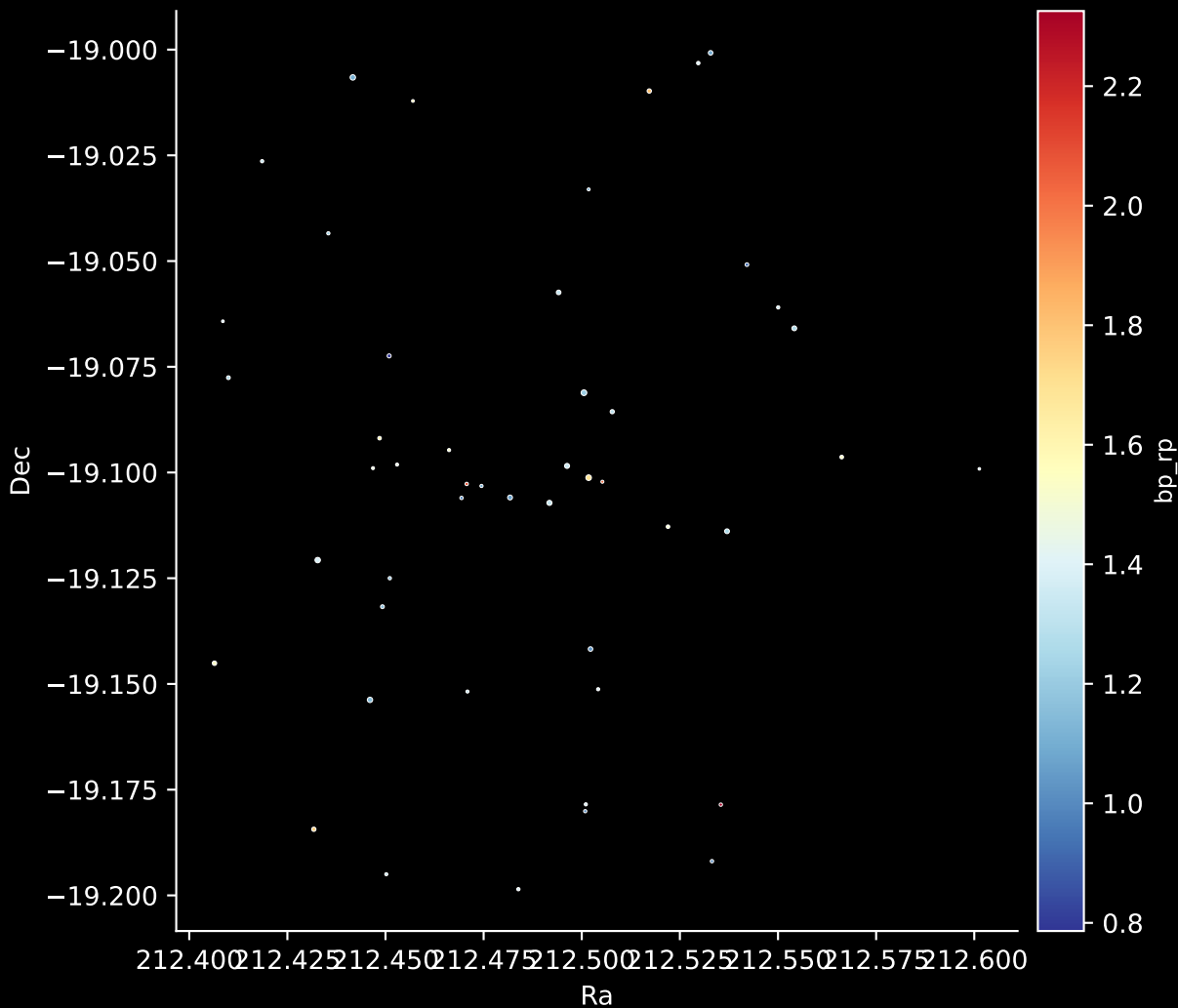
Gaia Cluster: [DBSB_6] Stars: 48
