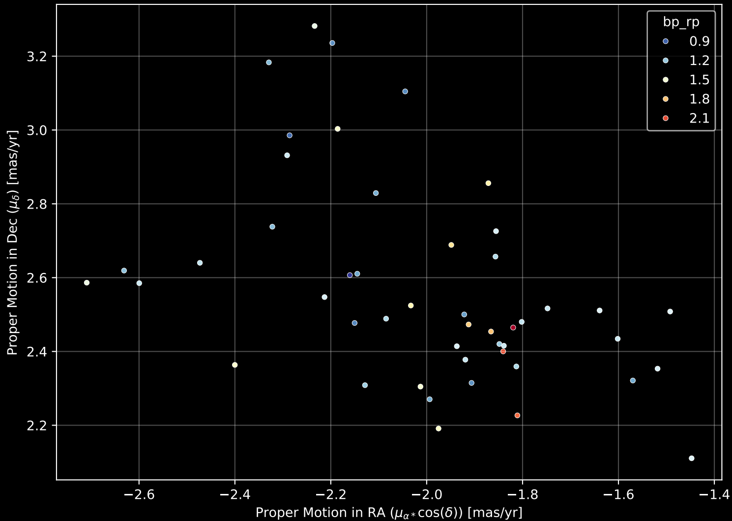
Gaia Cluster: [DBSB_6] Proper Motion Diagram (n= 48)
