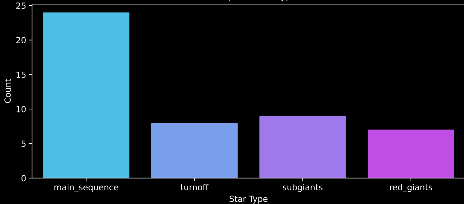
Gaia Cluster: [DBSB_6] Count plot of Star Type
