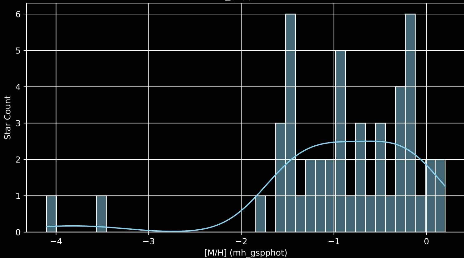
Gaia Cluster: [DBSB_6 [M/H] (mh_gspphot) (n= 48)
