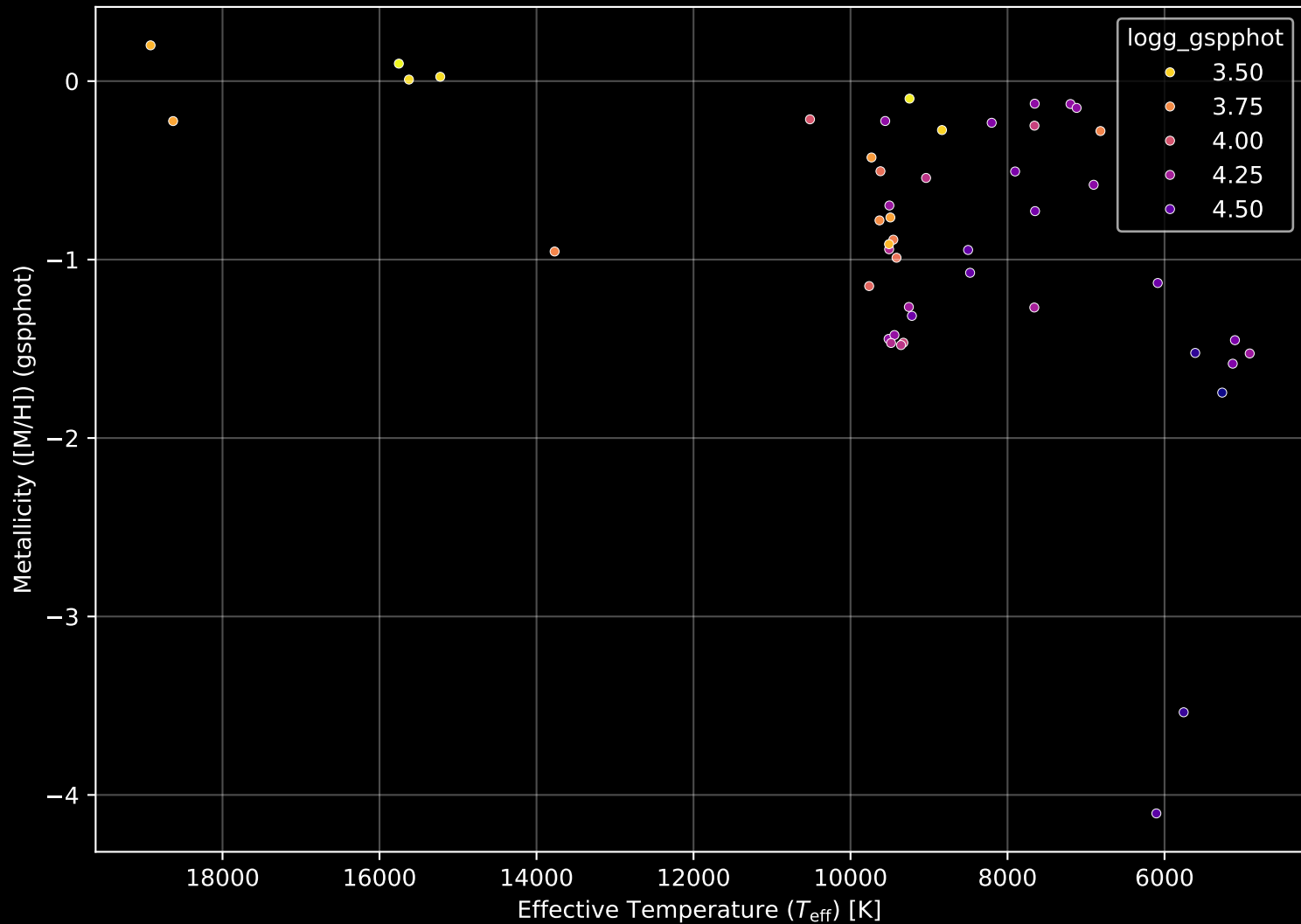
Gaia Cluster: [DBSB_6] Stellar Population Parameters (n= 48)
