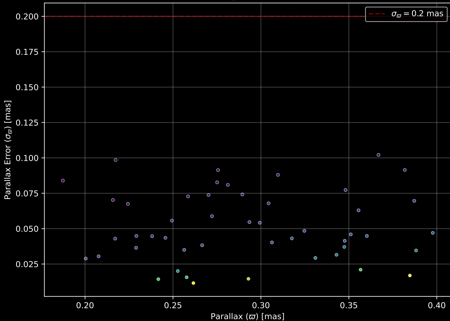
Gaia Cluster: [DBSB_6] Parallax Quality (n= 48)
