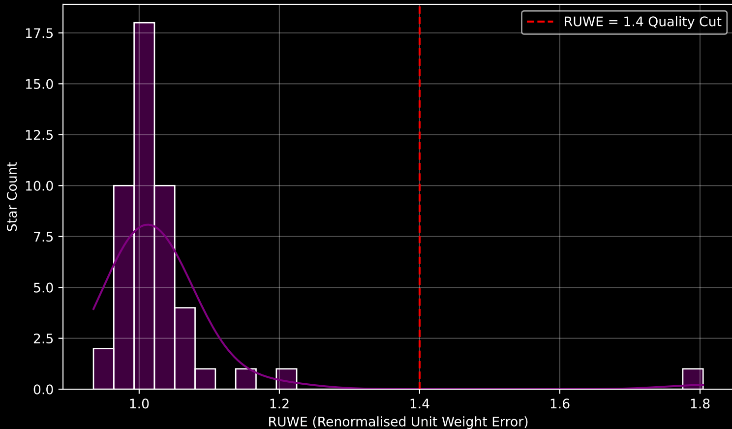
Gaia Cluster: [DBSB_6] RUWE Distribution (n= 48)
