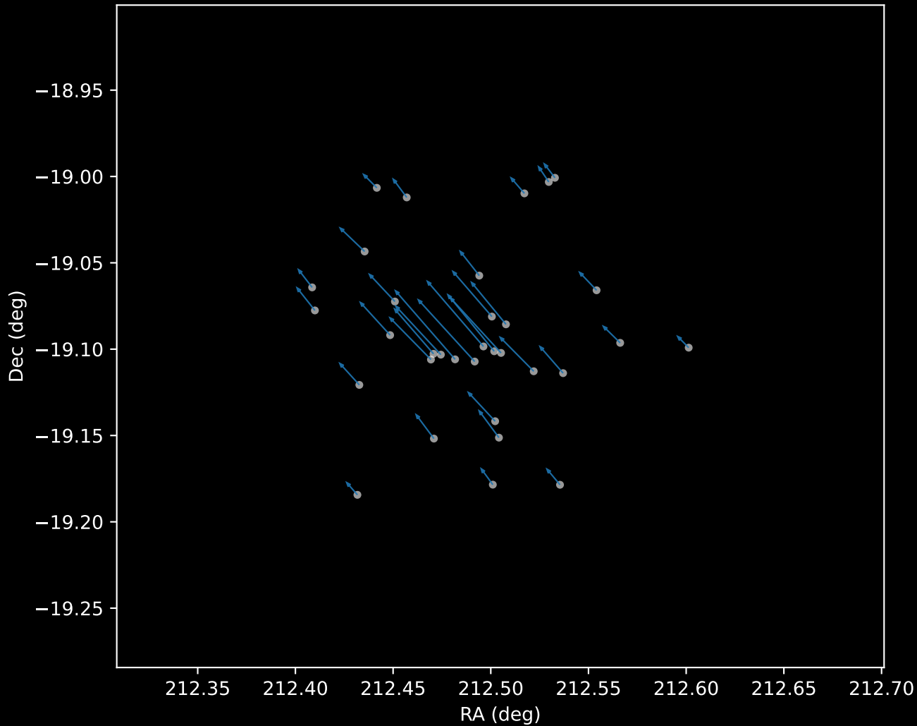
Gaia DR3 Cluster 0 Proper Motion Vectors (n=33)
