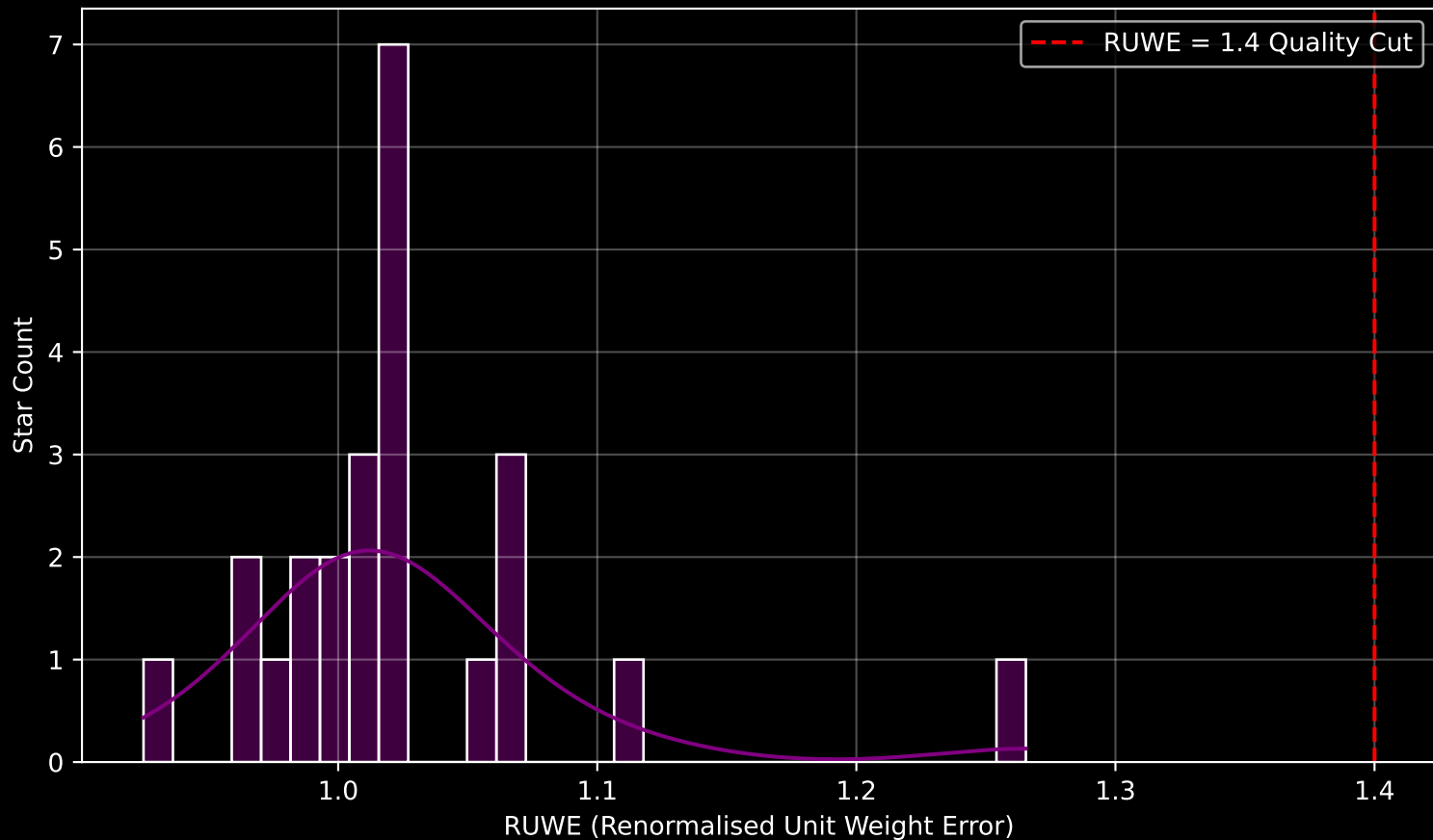
Gaia Cluster: [DBSB_60] RUWE Distribution (n= 24)
