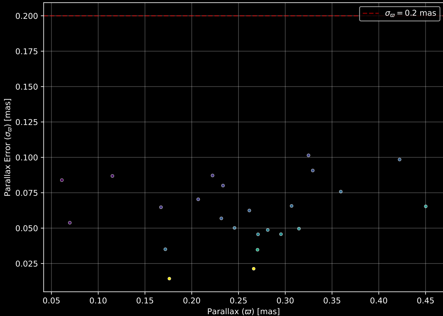
Gaia Cluster: [DBSB_60] Parallax Quality (n= 24)
