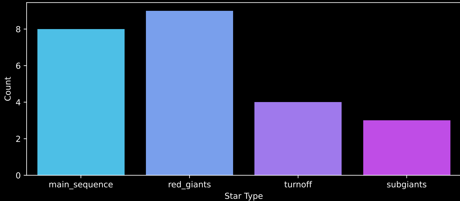
Gaia Cluster: [DBSB_60] Count plot of Star Type
