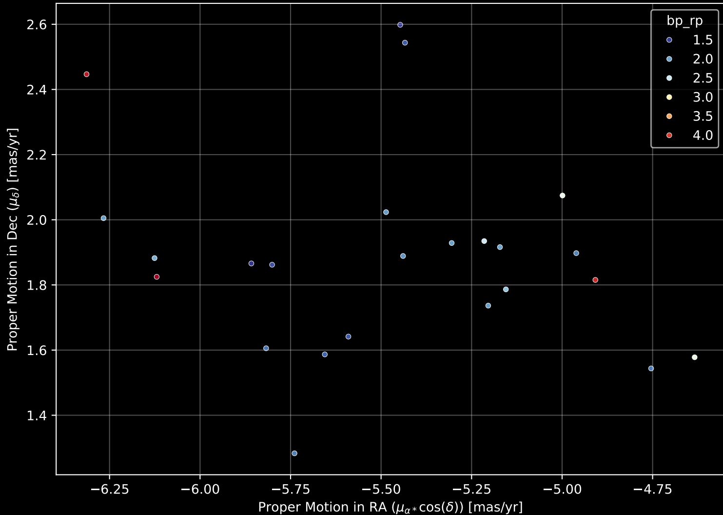
Gaia Cluster: [DBSB_60] Proper Motion Diagram (n= 24)
