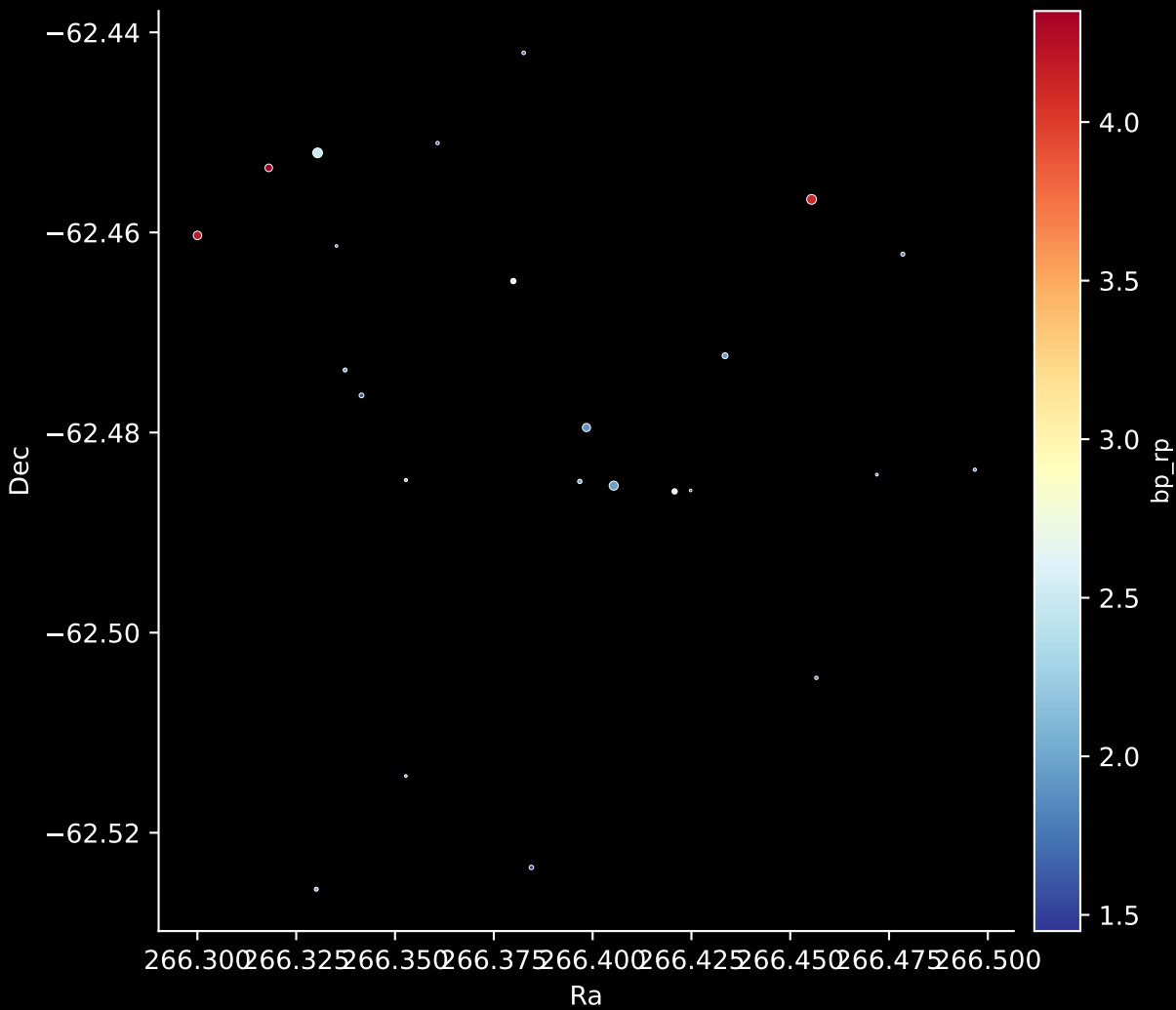
Gaia Cluster: [DBSB_60] Stars: 24
