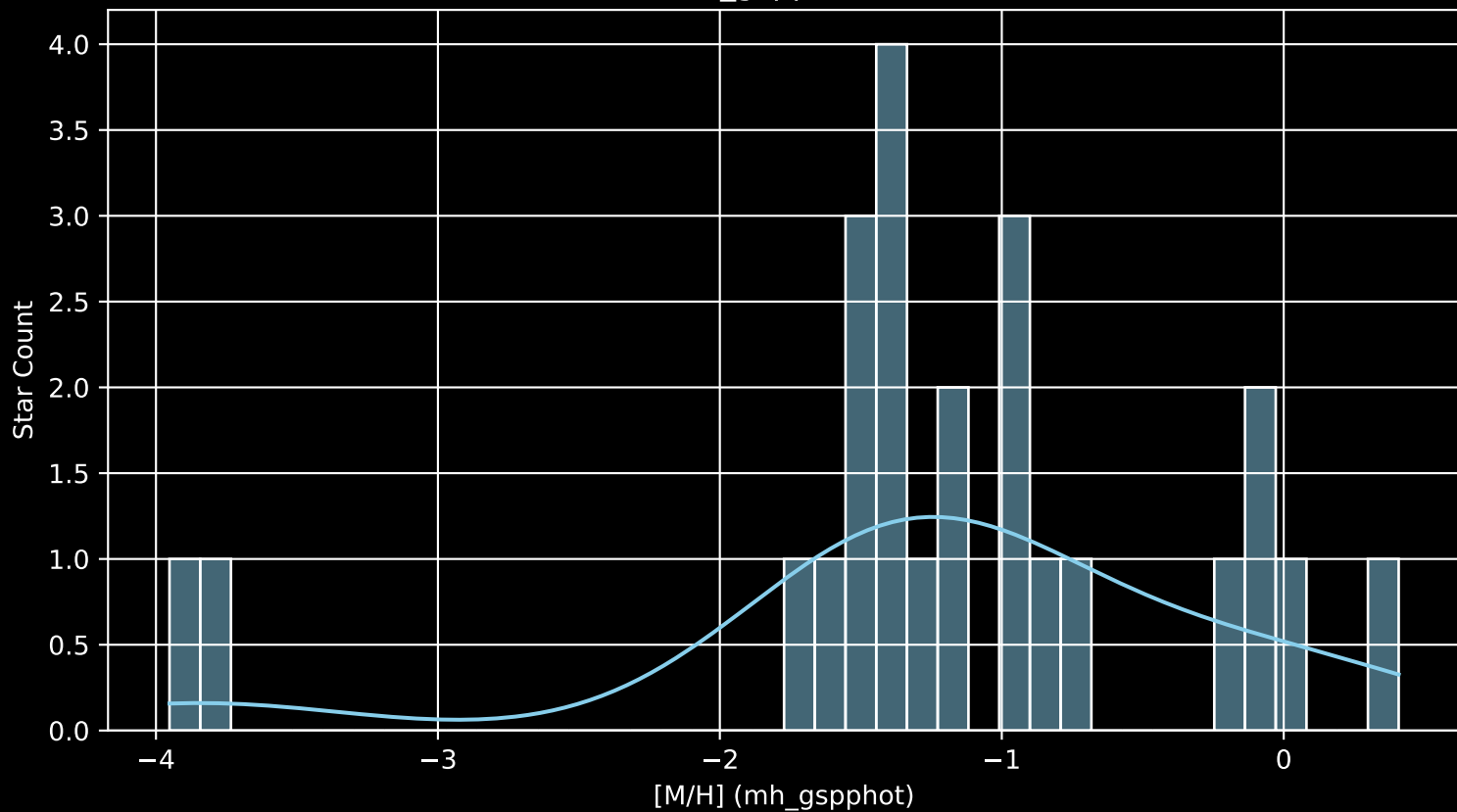
Gaia Cluster: [DBSB_60 [M/H] (mh_gspphot) (n= 24)
