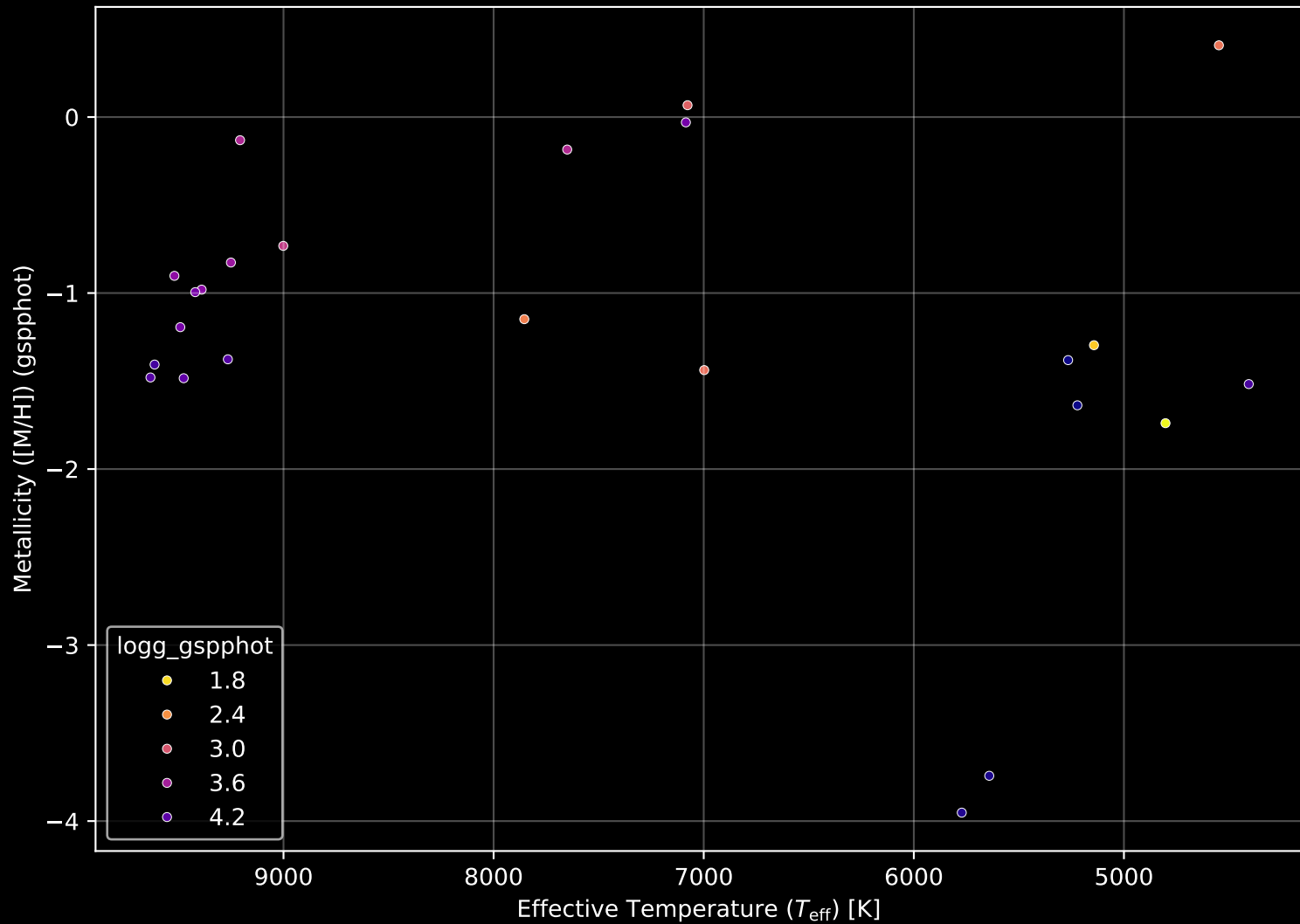
Gaia Cluster: [DBSB_60] Stellar Population Parameters (n= 24)
