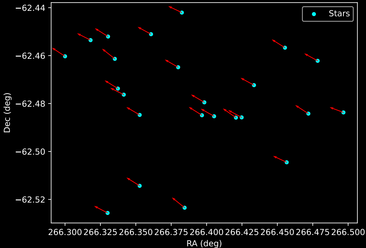
Gaia Cluster: [DBSB_60] Proper Motion Vectors for Gaia Star Field (n= 24)
