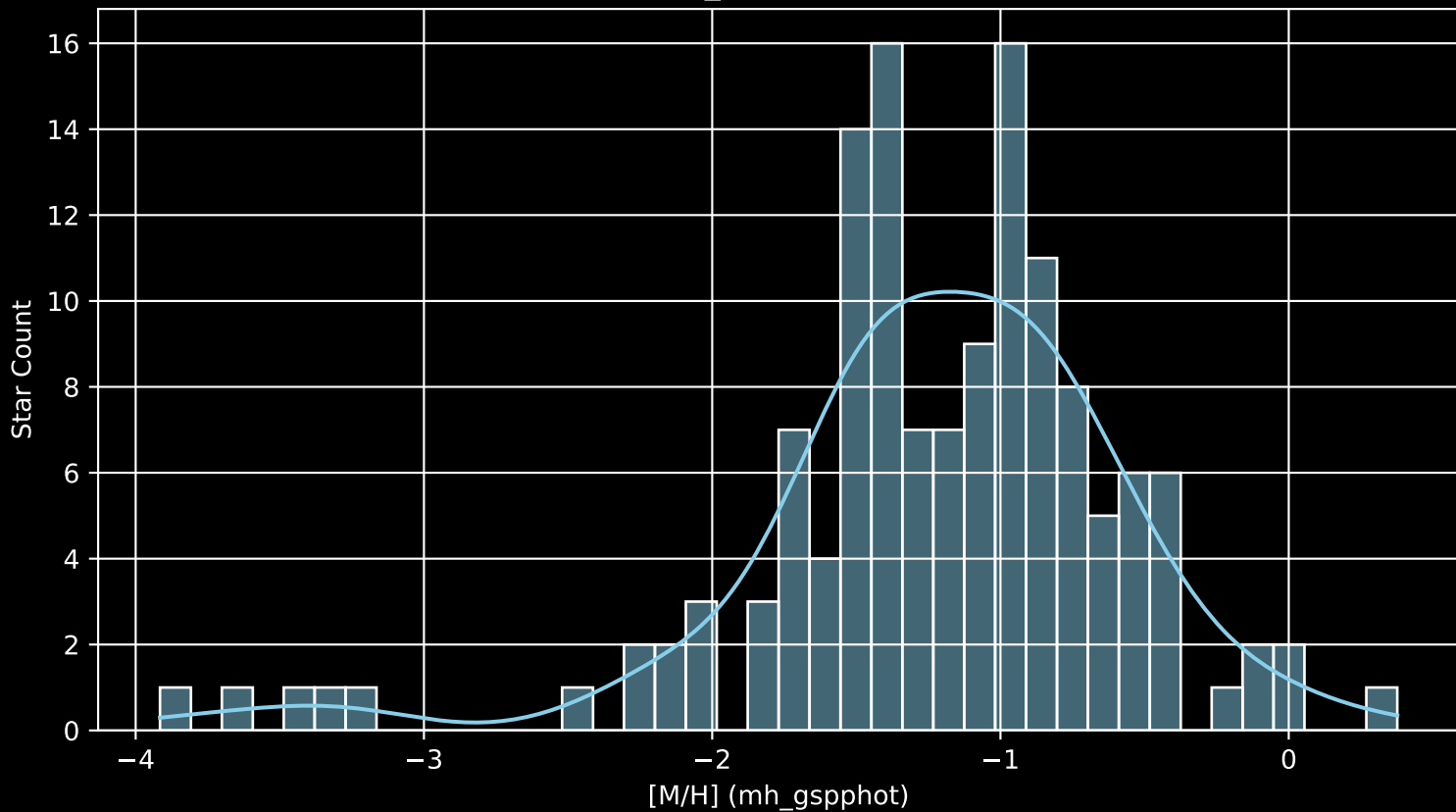
Gaia Cluster: [DC_5 [M/H] (mh_gspphot) (n= 138)
