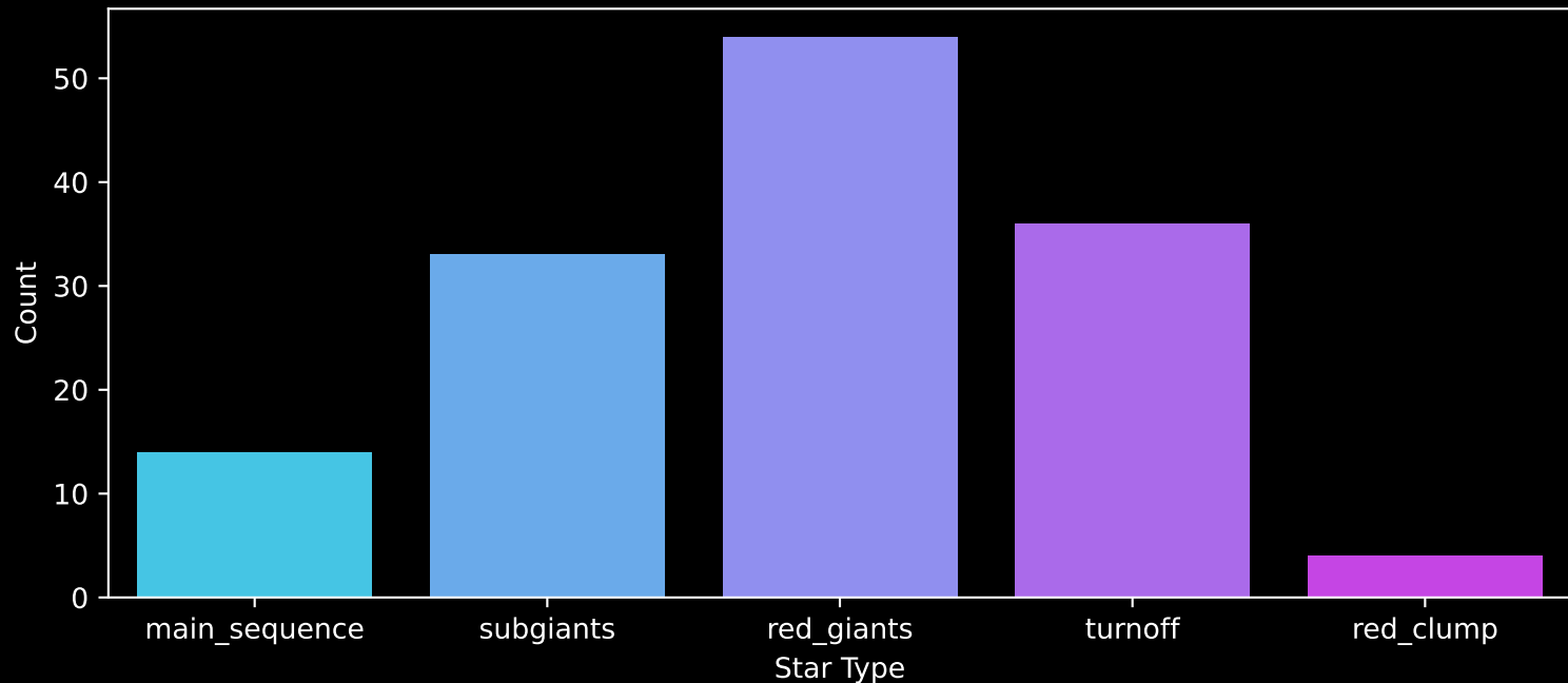
Gaia Cluster: [DC_5] Count plot of Star Type
