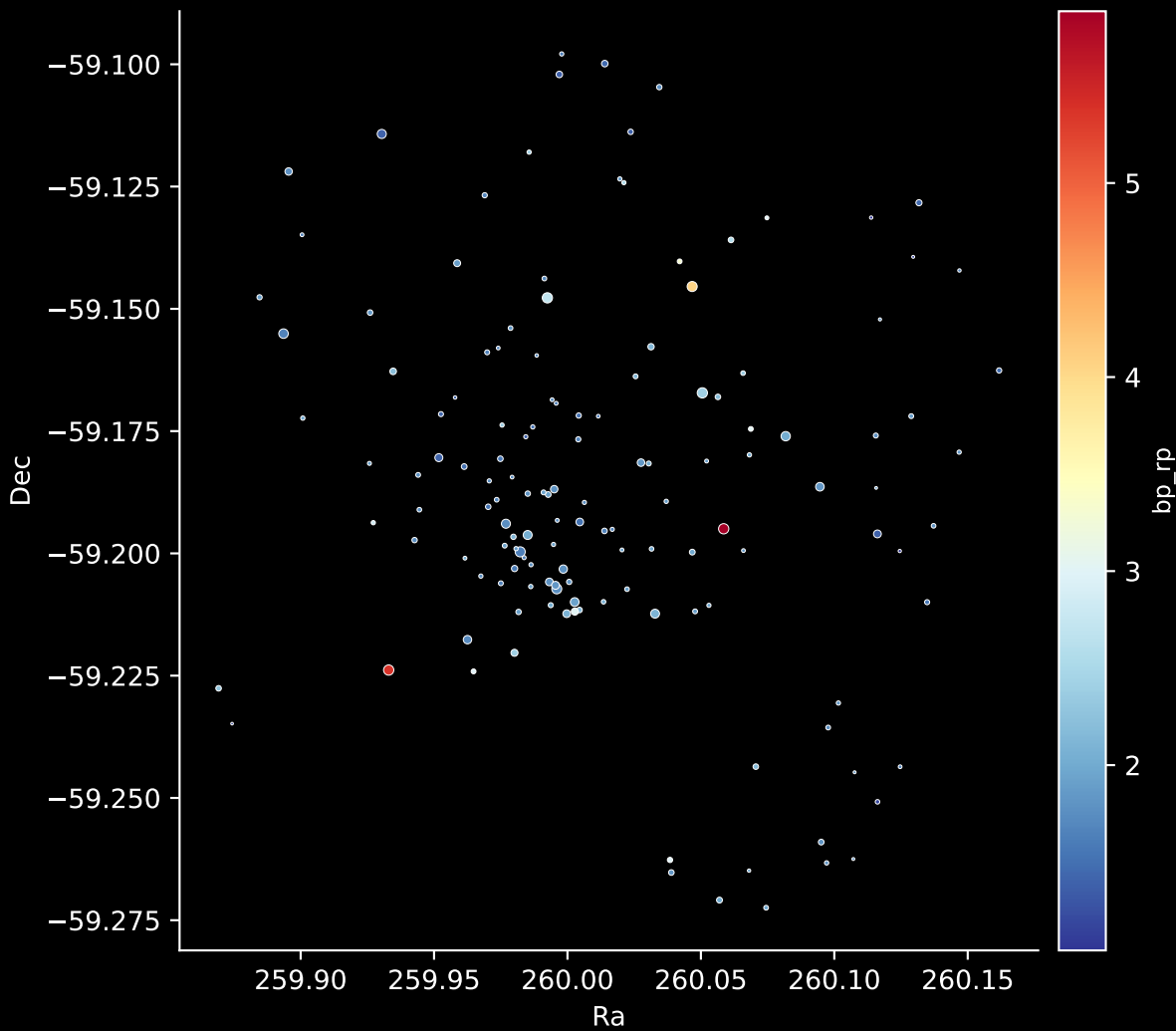
Gaia Cluster: [DC_5] Stars: 141
