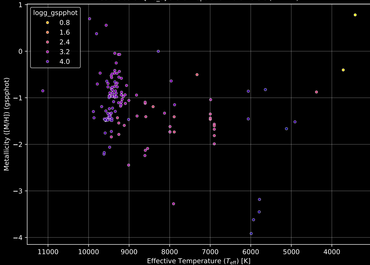
Gaia Cluster: [DC_5] Stellar Population Parameters (n= 141)
