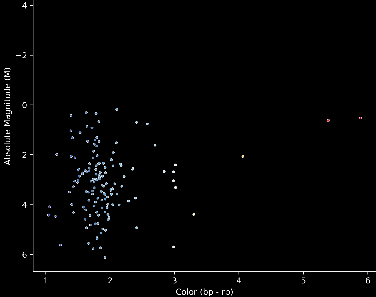
Gaia Cluster: [DC_5] Stars (n= 141) Hertzsprung-Russel Diagram
