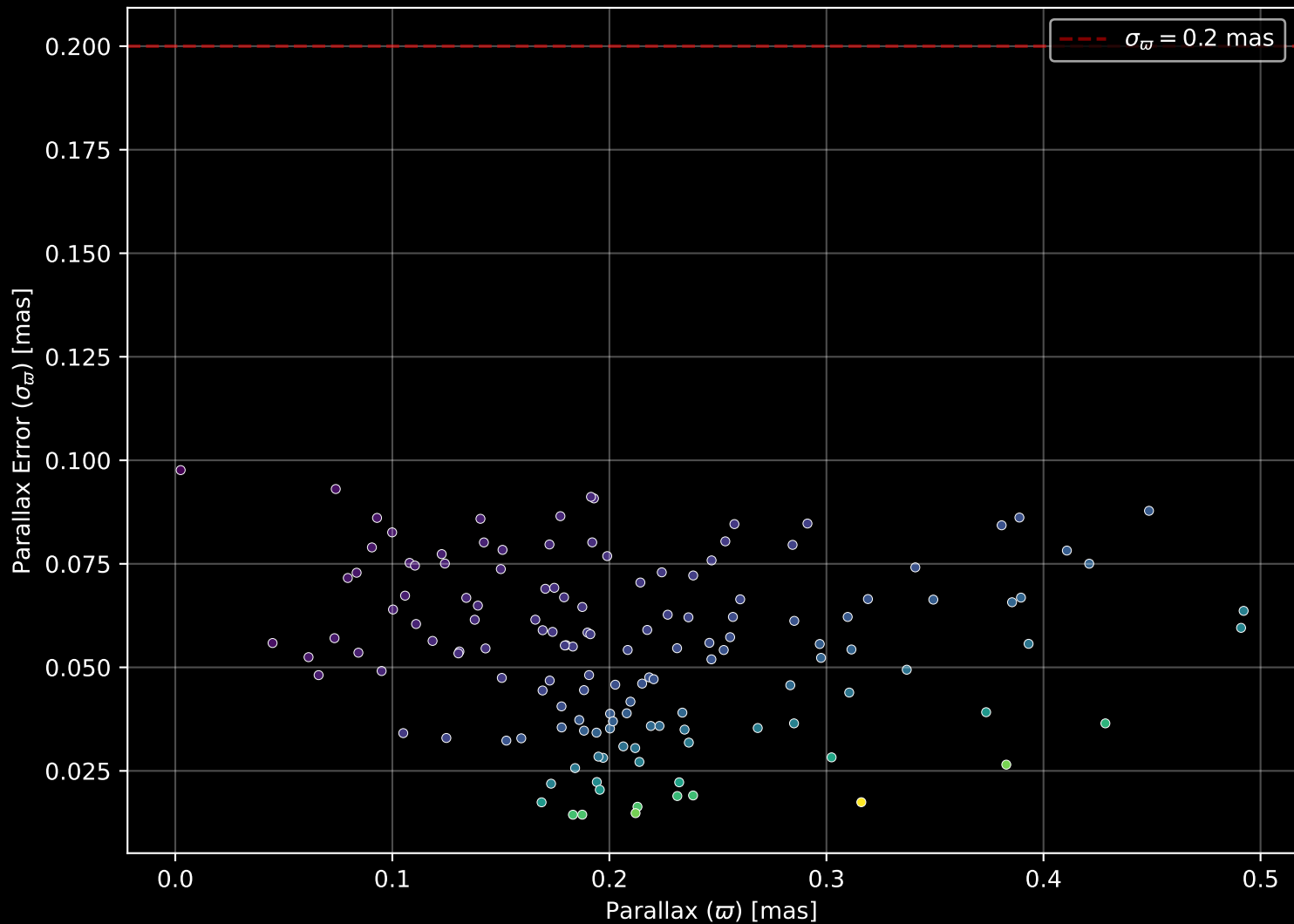
Gaia Cluster: [DC_5] Parallax Quality (n= 141)
