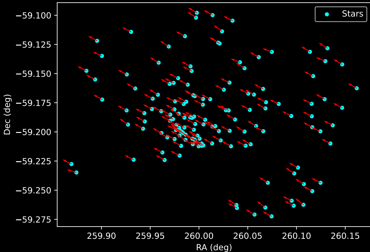
Gaia Cluster: [DC_5] Proper Motion Vectors for Gaia Star Field (n= 141)
