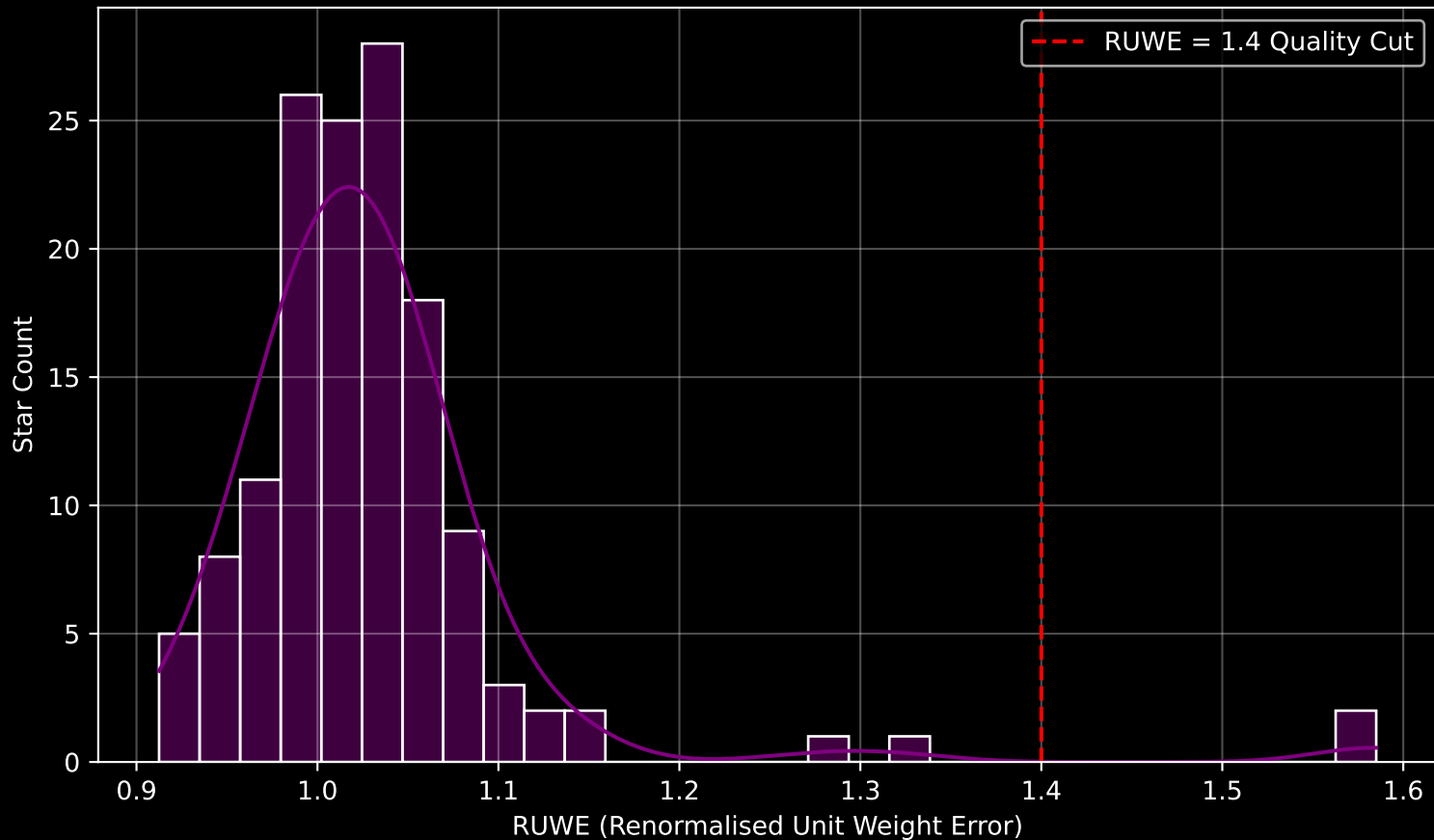
Gaia Cluster: [DC_5] RUWE Distribution (n= 141)
