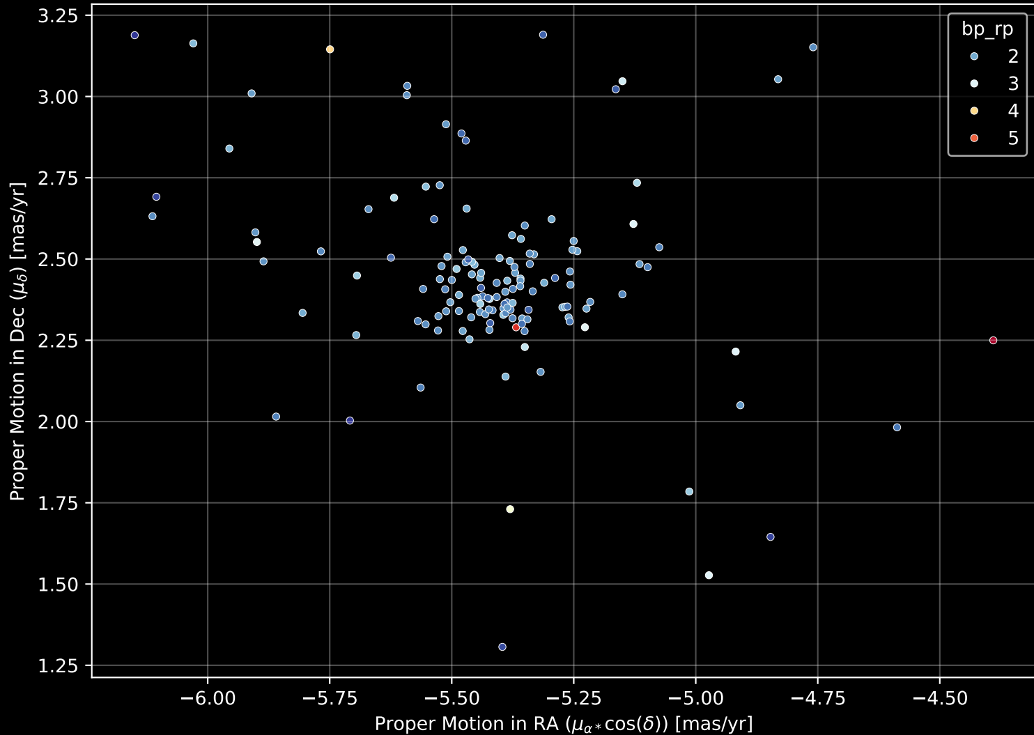
Gaia Cluster: [DC_5] Proper Motion Diagram (n= 141)
