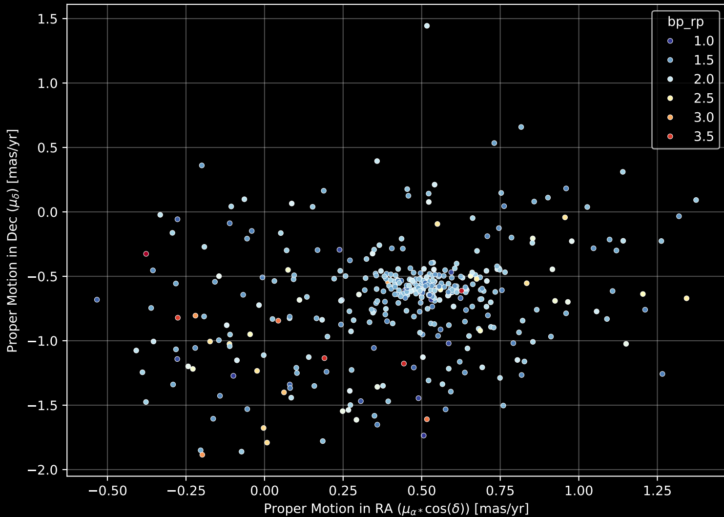
Gaia Cluster: [Dias_6] Proper Motion Diagram (n= 384)
