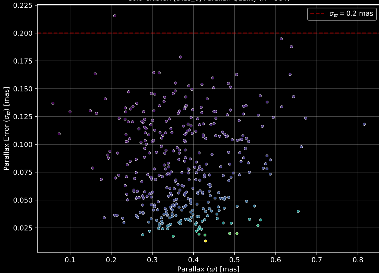
Gaia Cluster: [Dias_6] Parallax Quality (n= 384)
