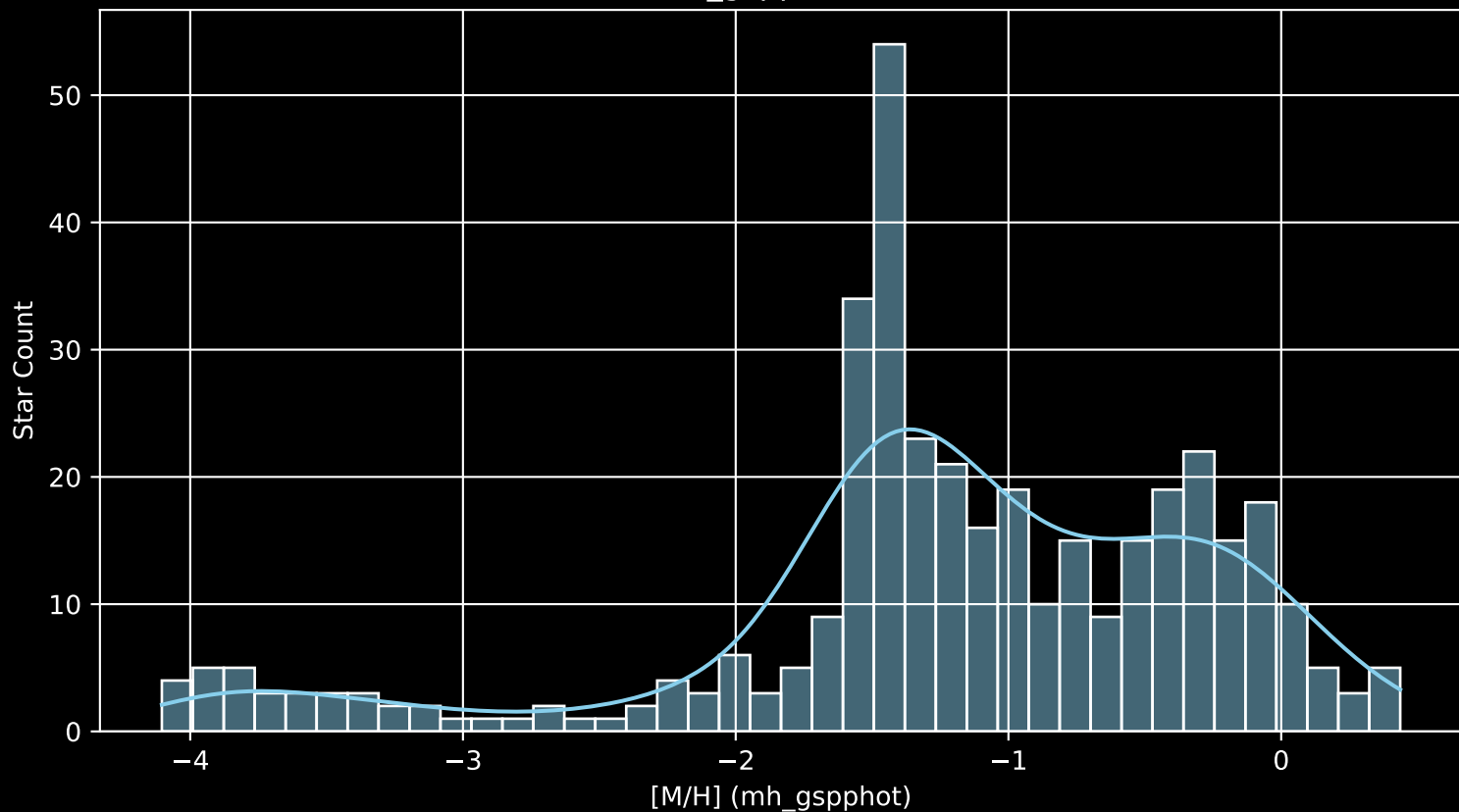
Gaia Cluster: [Dias_6 [M/H] (mh_gspphot) (n= 382)
