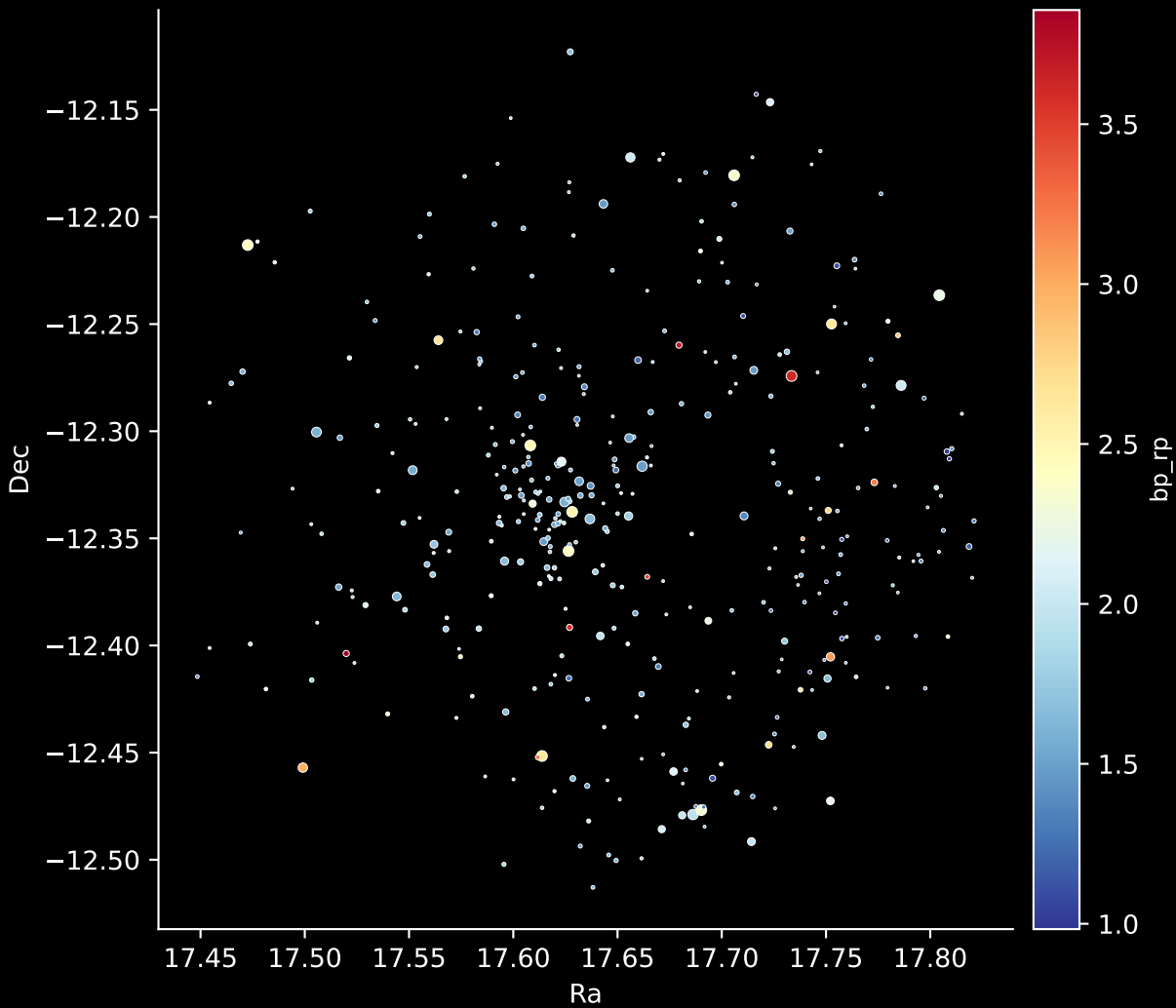
Gaia Cluster: [Dias_6] Stars: 384
