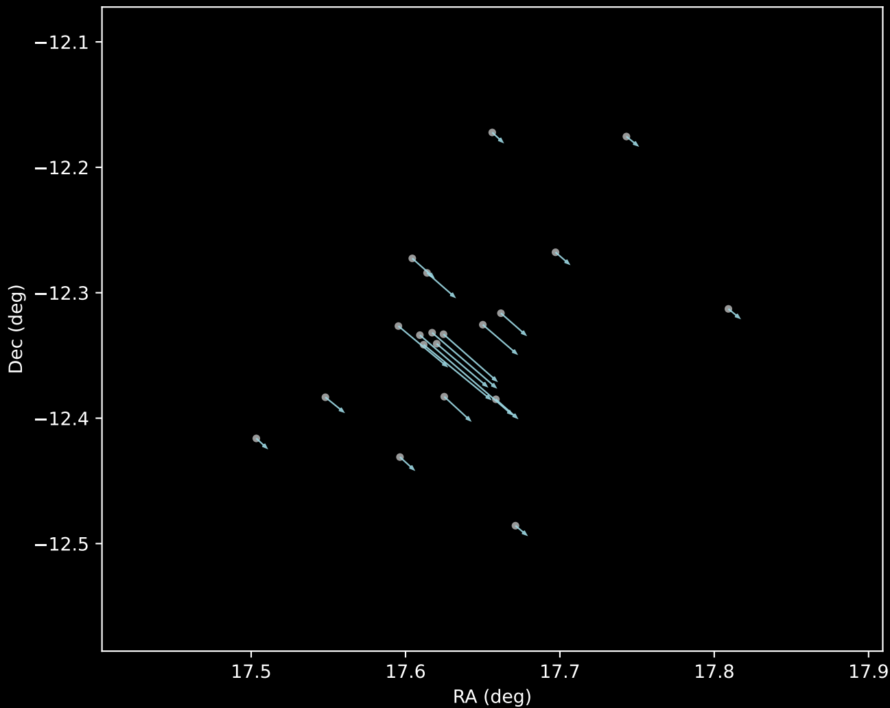
Gaia DR3 Cluster 19 Proper Motion Vectors (n=20)
