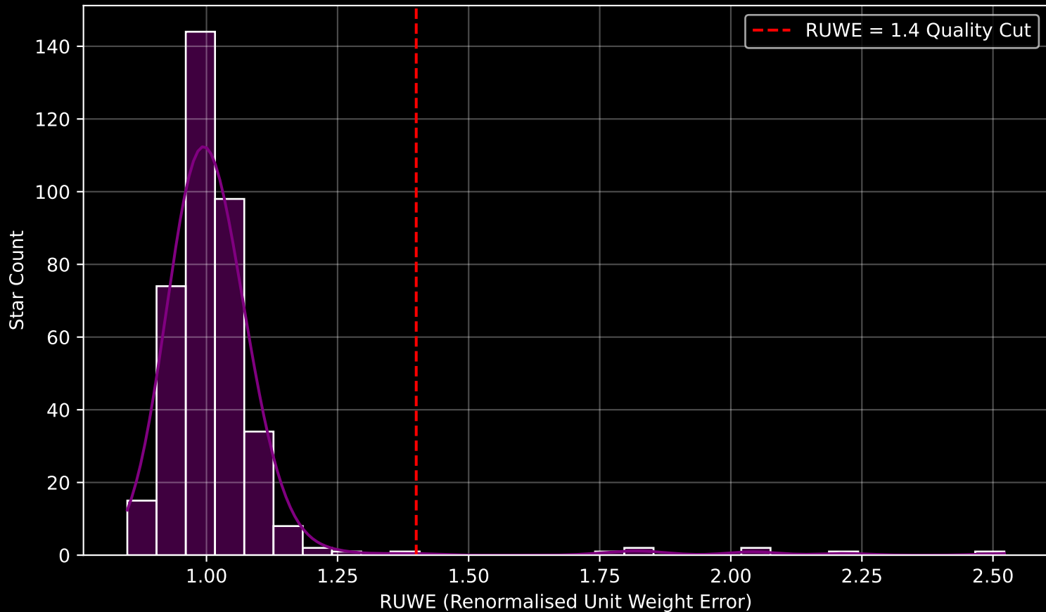
Gaia Cluster: [Dias_6] RUWE Distribution (n= 384)
