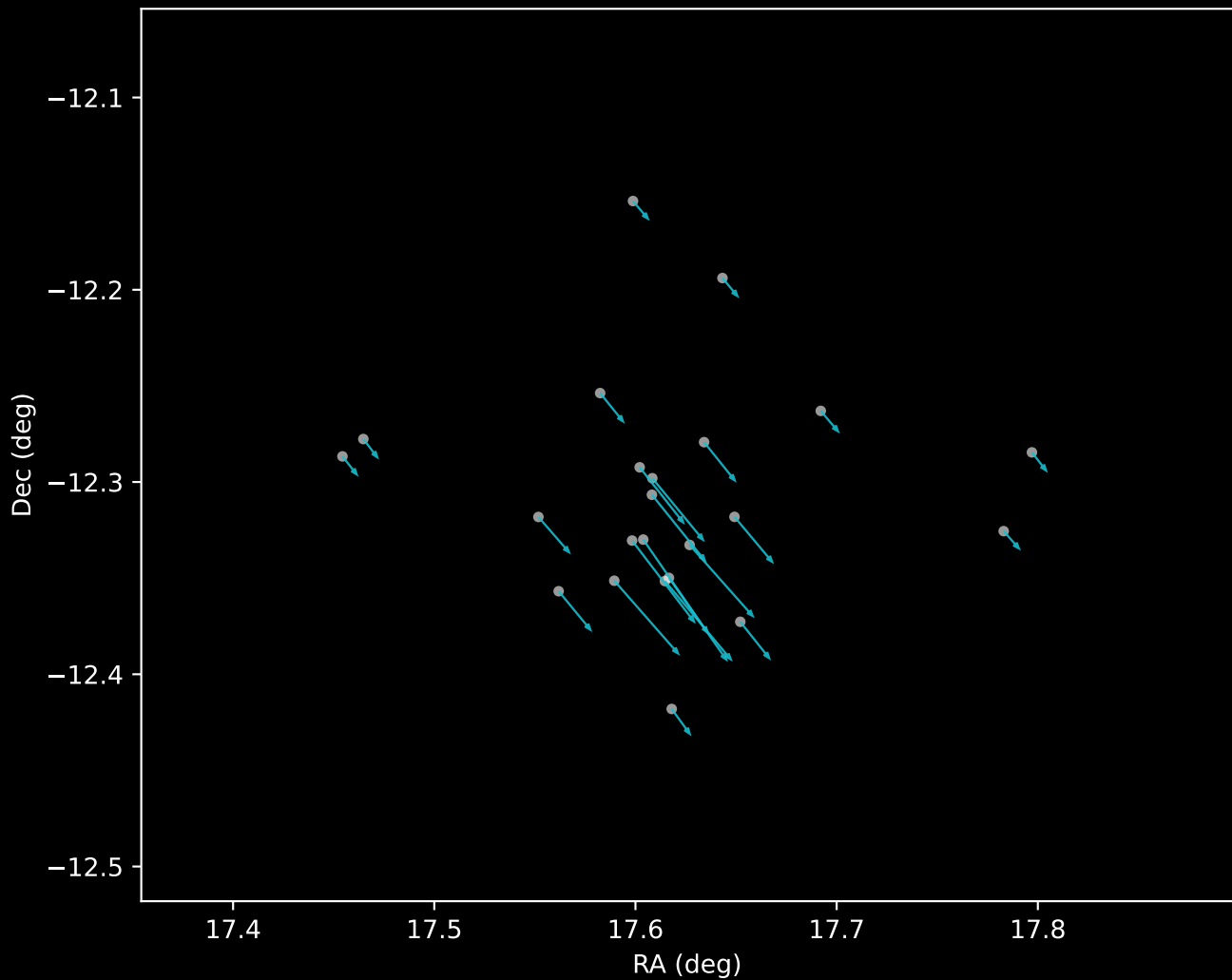
Gaia DR3 Cluster 18 Proper Motion Vectors (n=23)
