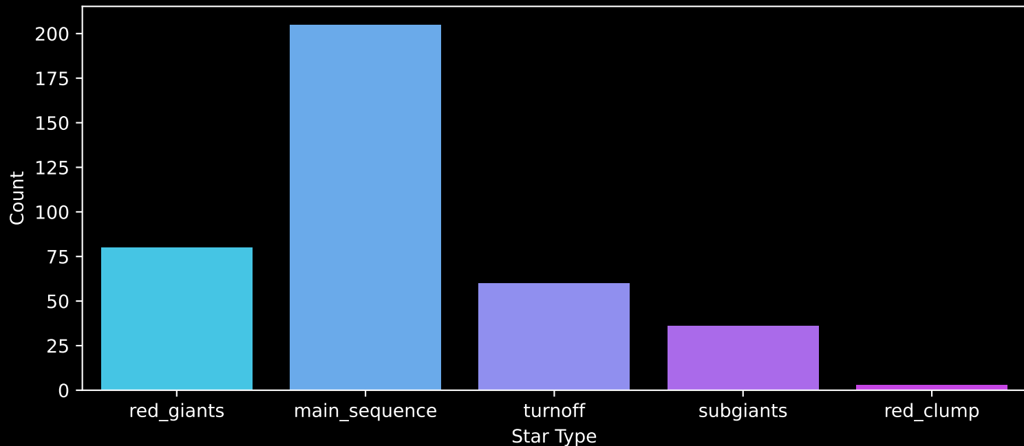
Gaia Cluster: [Dias_6] Count plot of Star Type
