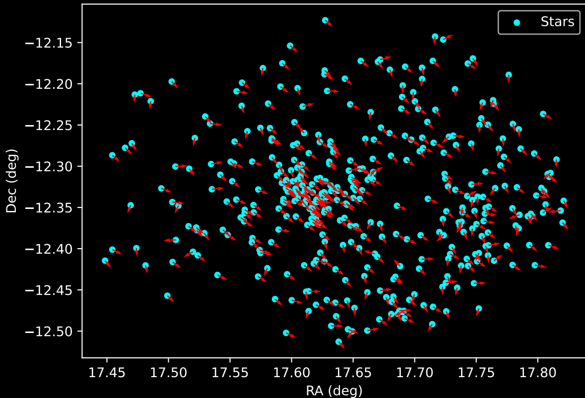
Gaia Cluster: [Dias_6] Proper Motion Vectors for Gaia Star Field (n= 384)
