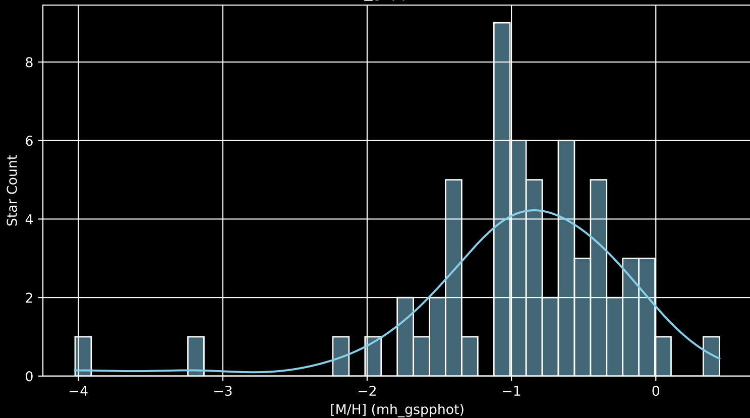
Gaia Cluster: [Dolidze_16 [M/H] (mh_gspphot) (n= 61)
