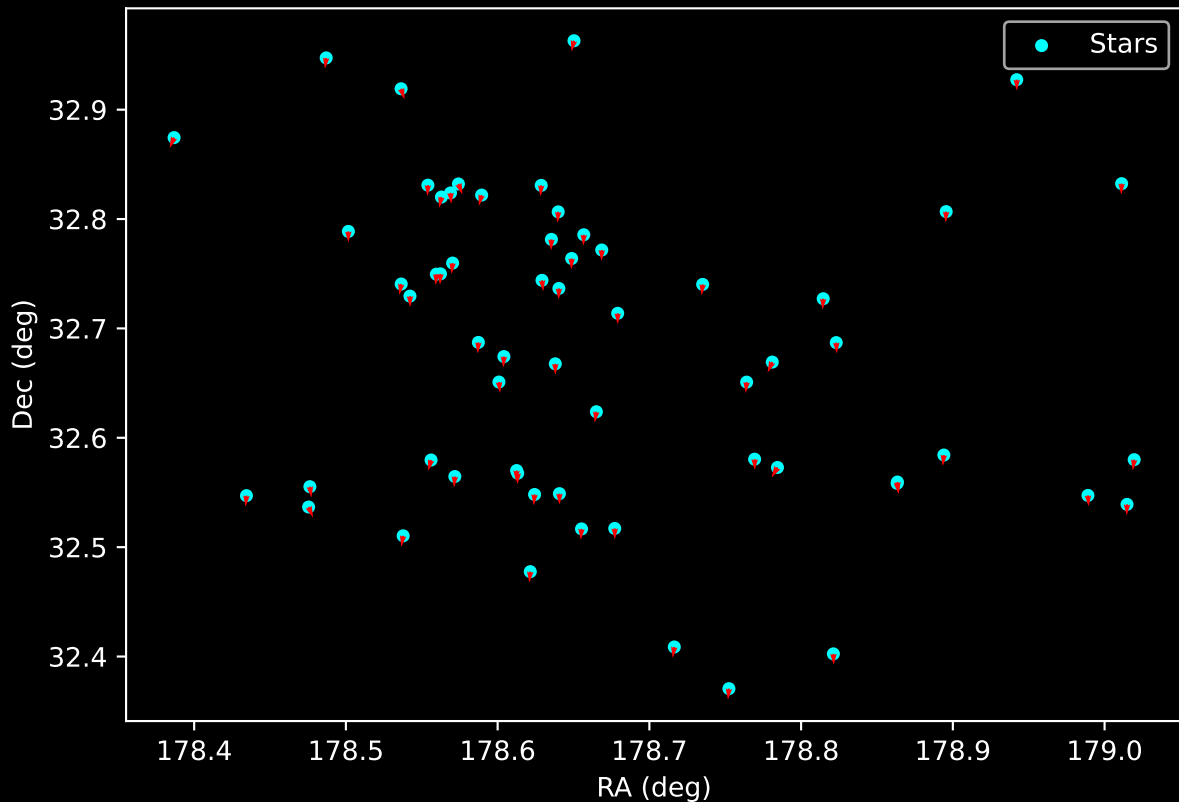
Gaia Cluster: [Dolidze_16] Proper Motion Vectors for Gaia Star Field (n= 61)
