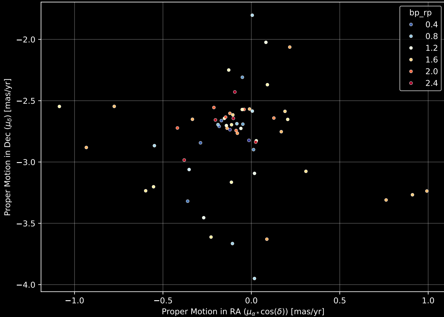
Gaia Cluster: [Dolidze_16] Proper Motion Diagram (n= 61)
