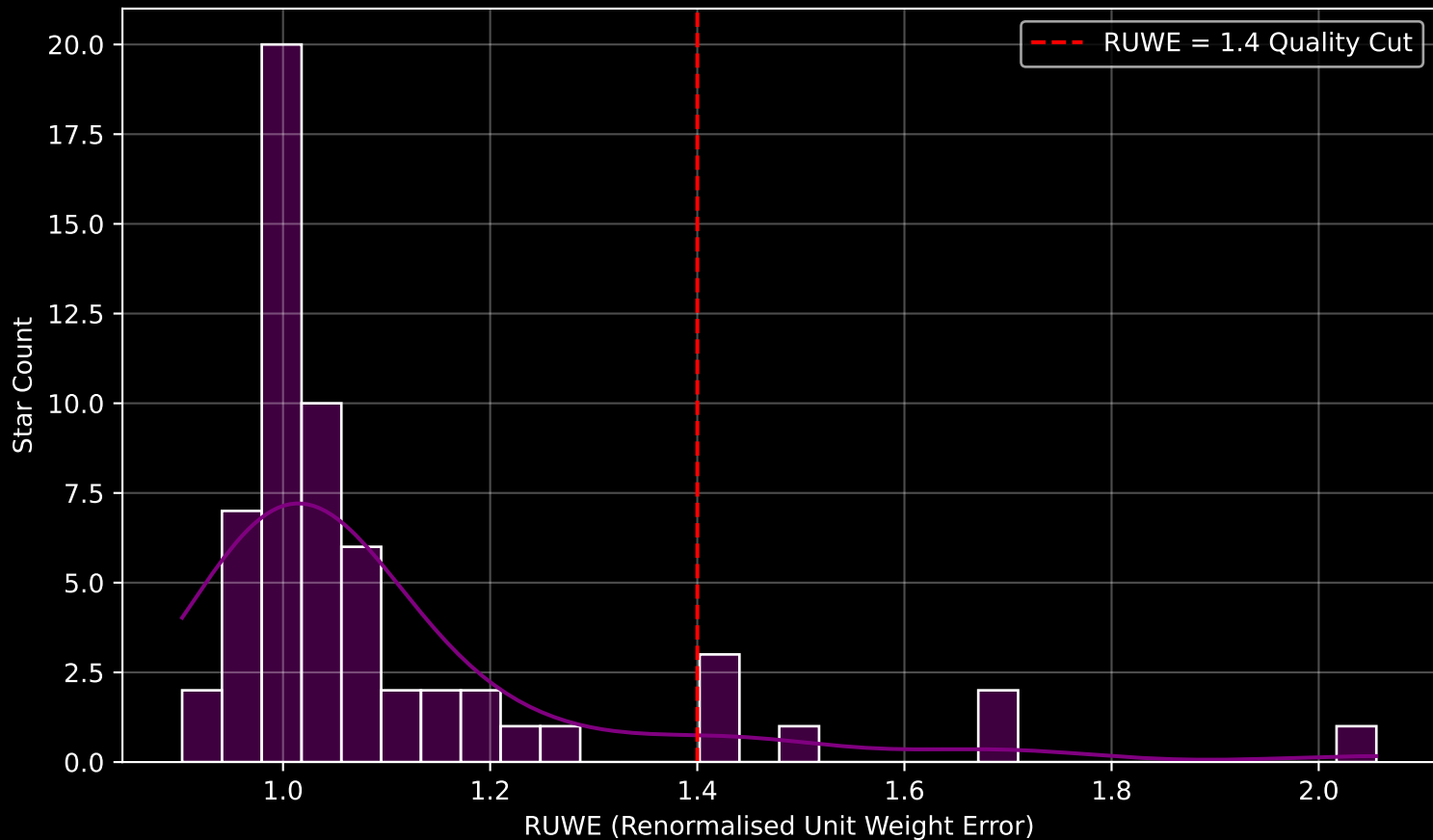
Gaia Cluster: [Dolidze_16] RUWE Distribution (n= 60)
