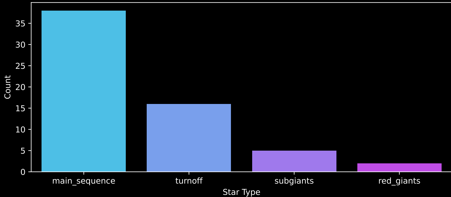
Gaia Cluster: [Dolidze_16] Count plot of Star Type
