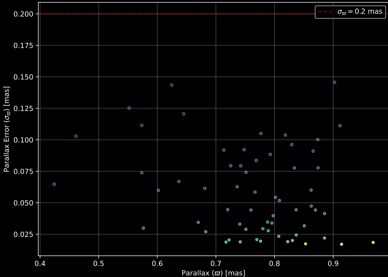
Gaia Cluster: [Dolidze_16] Parallax Quality (n= 61)
