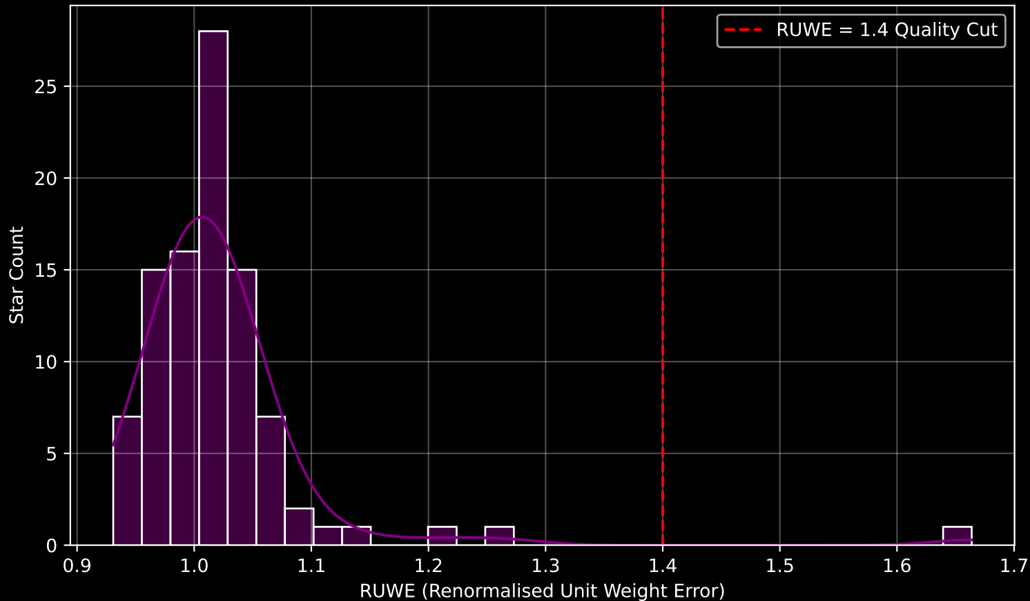
Gaia Cluster: [Dolidze_5] RUWE Distribution (n= 95)
