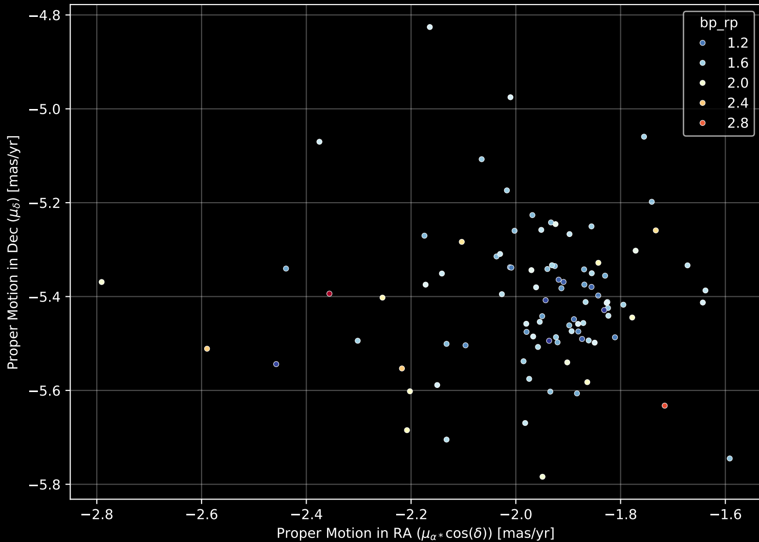
Gaia Cluster: [Dolidze_5] Proper Motion Diagram (n= 95)
