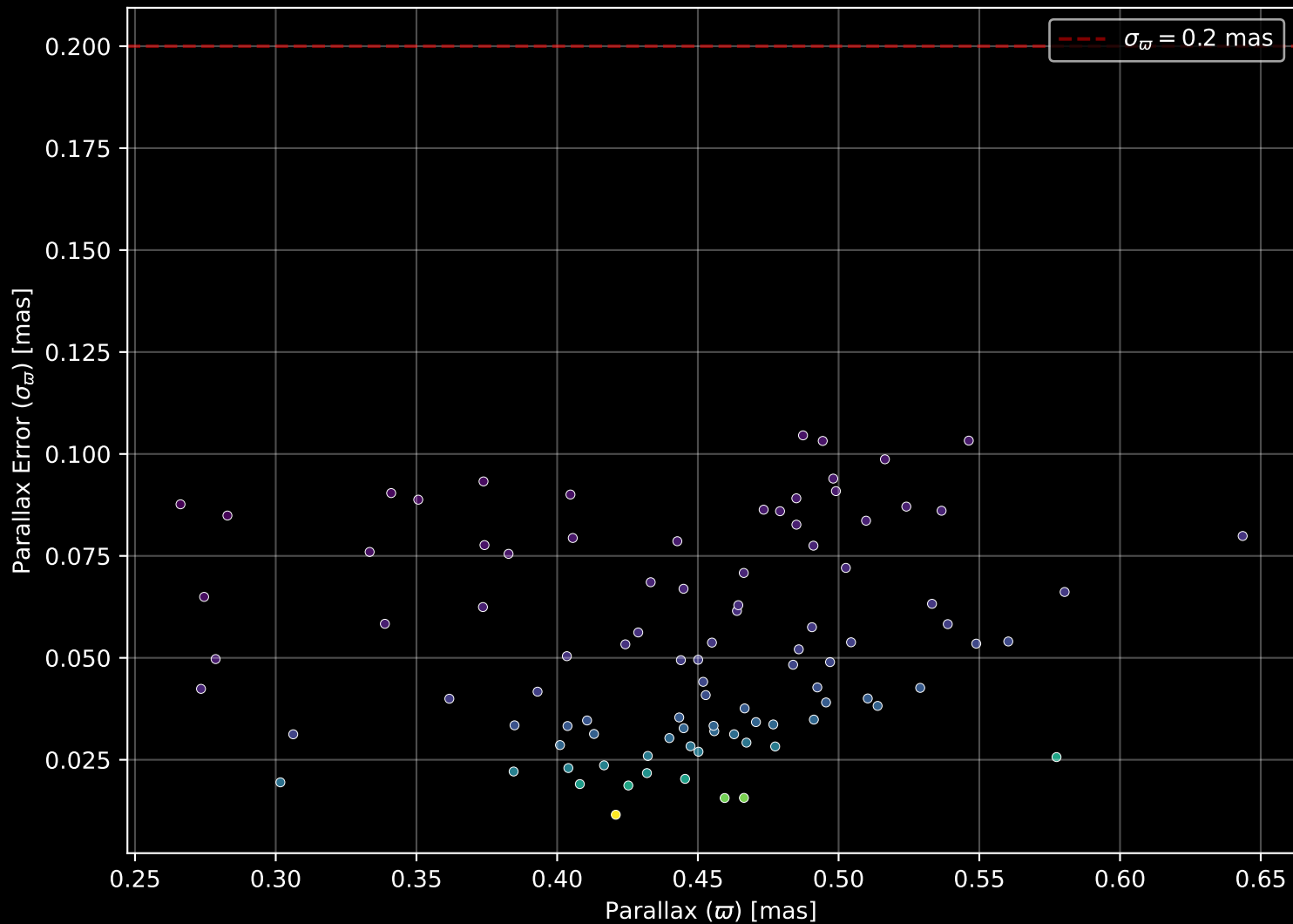
Gaia Cluster: [Dolidze_5] Parallax Quality (n= 95)
