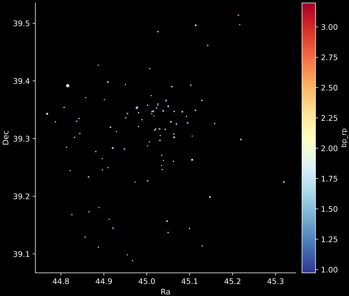
Gaia Cluster: [Dolidze_5] Stars: 95
