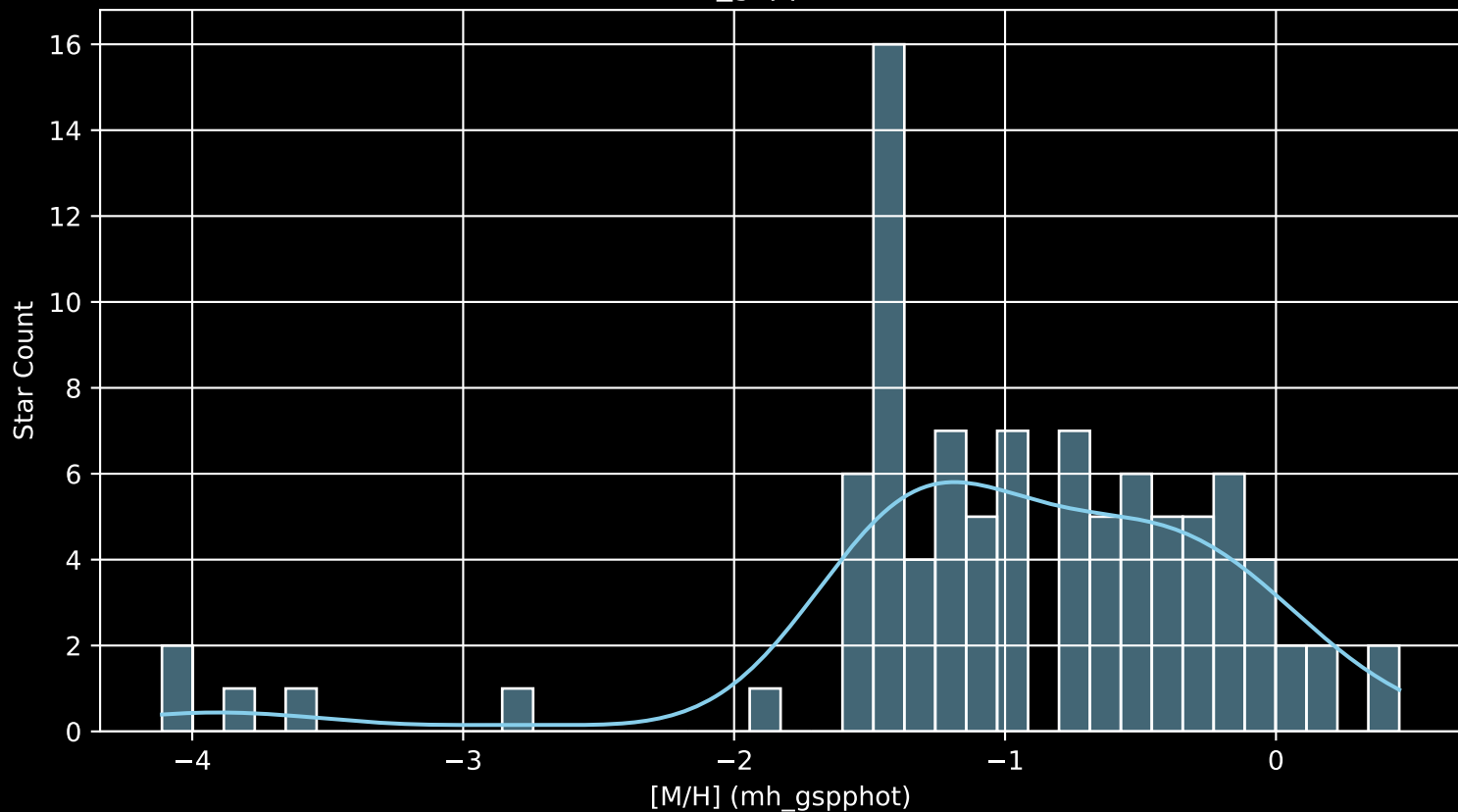
Gaia Cluster: [Dolidze_5 [M/H] (mh_gspphot) (n= 95)
