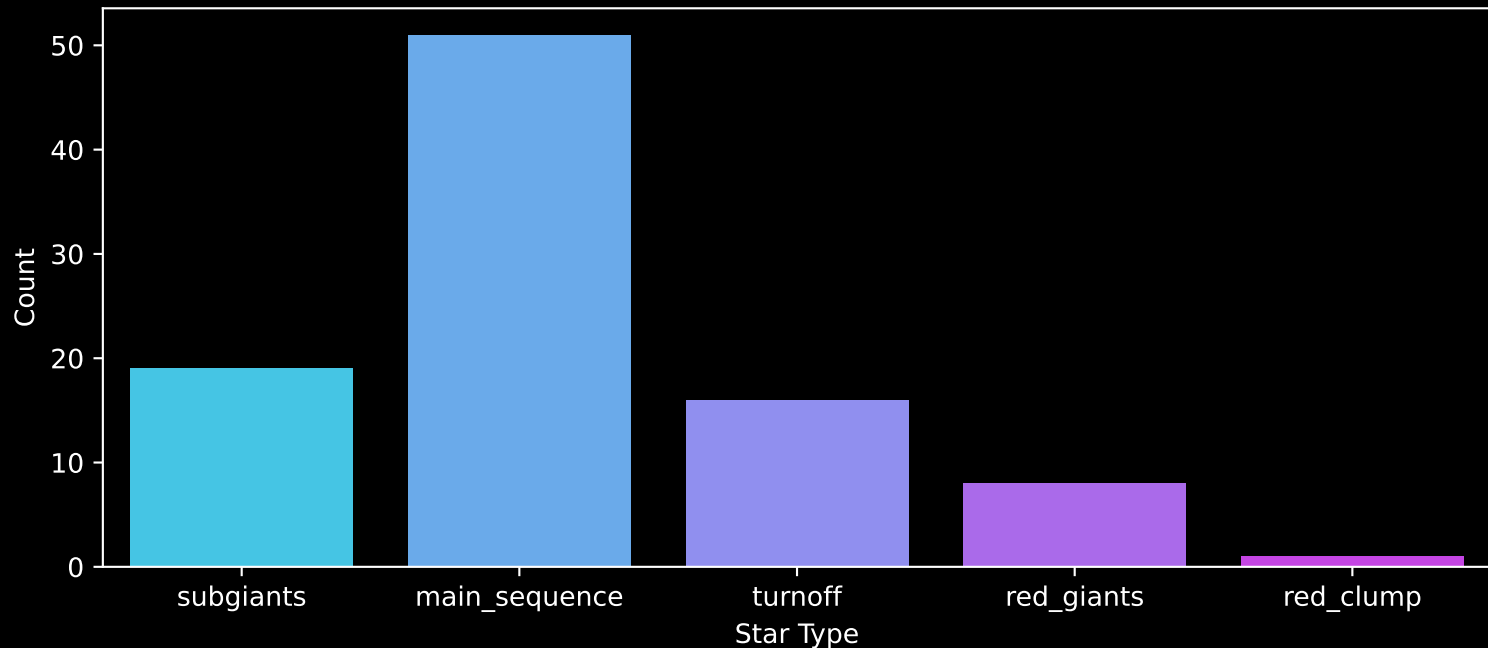
Gaia Cluster: [Dolidze_5] Count plot of Star Type
