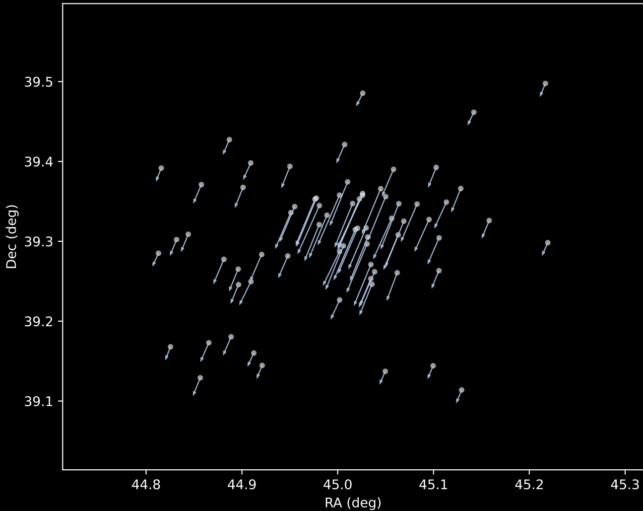
Gaia DR3 Cluster 1 Proper Motion Vectors (n=70)
