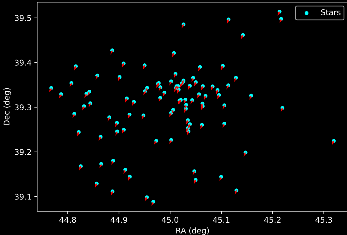
Gaia Cluster: [Dolidze_5] Proper Motion Vectors for Gaia Star Field (n= 95)
