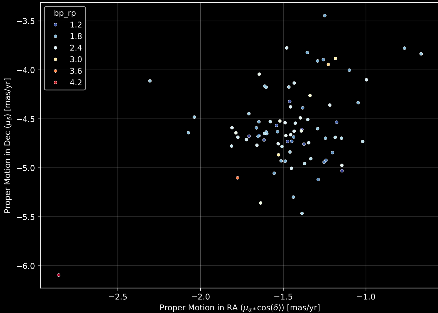
Gaia Cluster: [Dolidze_53] Proper Motion Diagram (n= 87)
