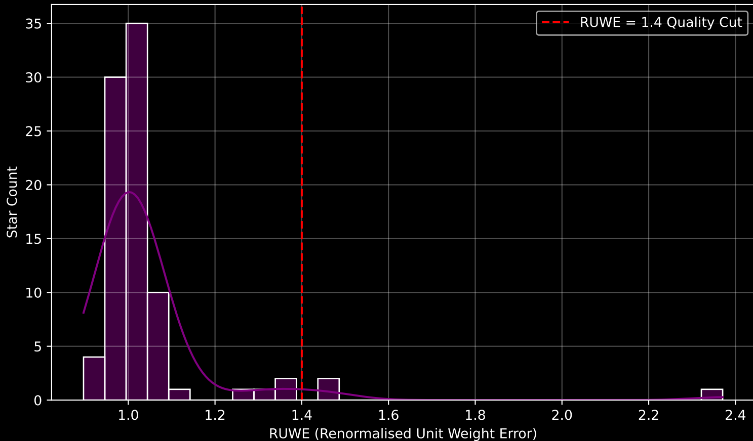
Gaia Cluster: [Dolidze_53] RUWE Distribution (n= 87)
