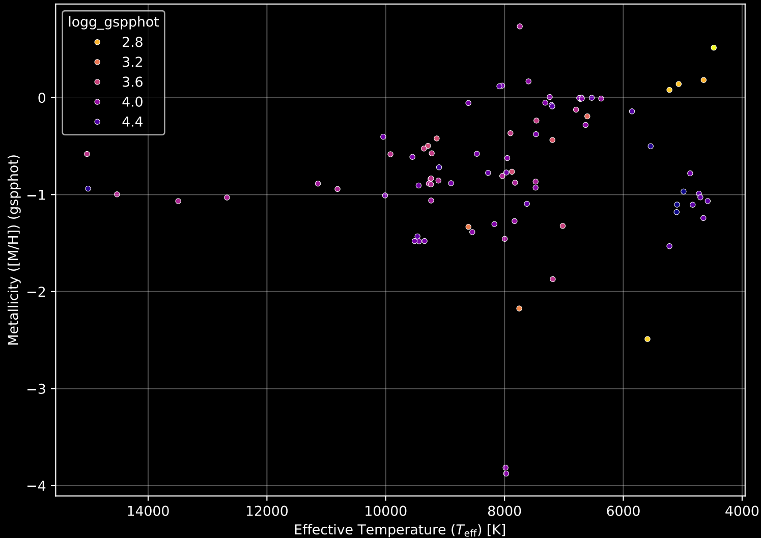
Gaia Cluster: [Dolidze_53] Stellar Population Parameters (n= 87)
