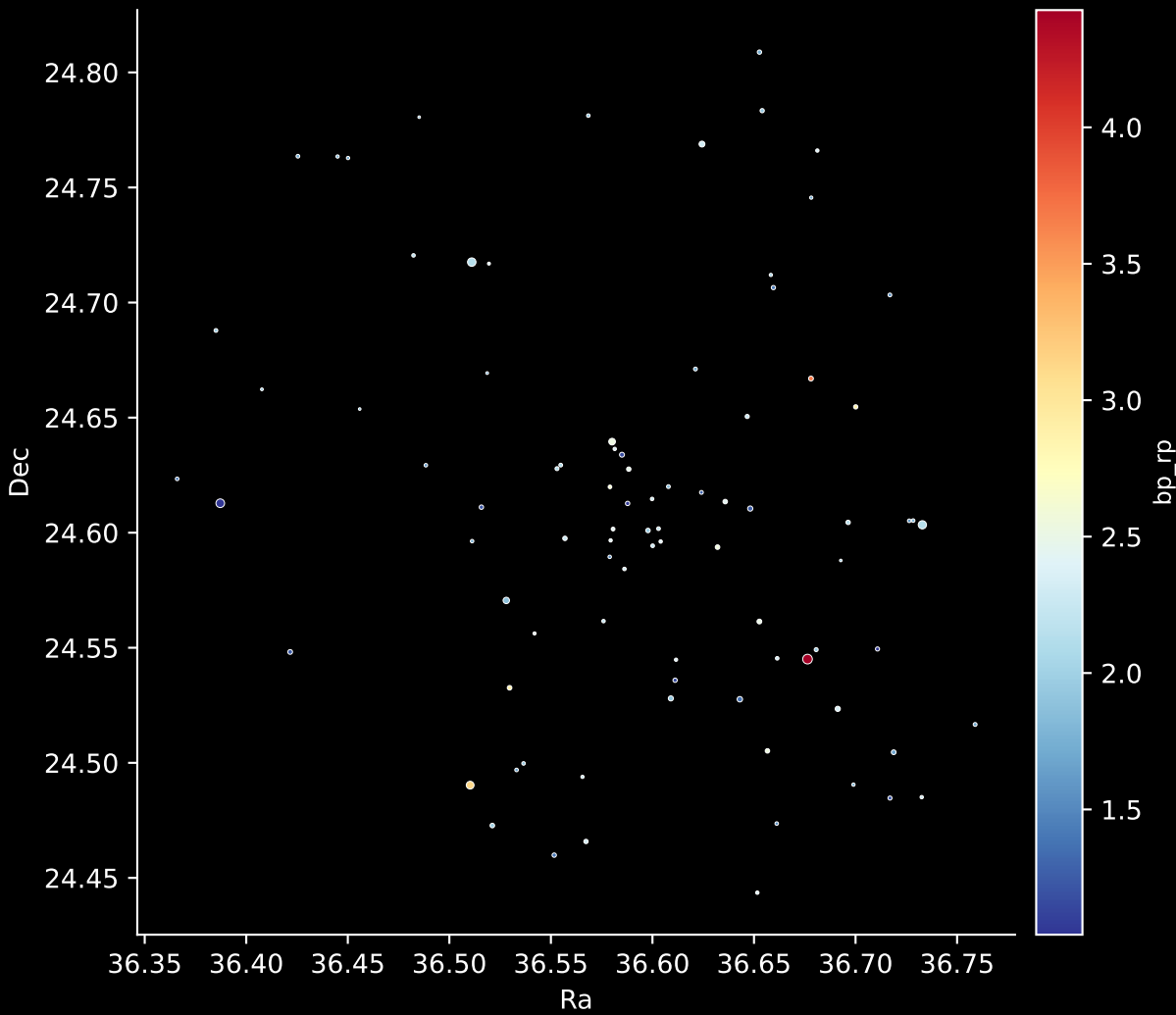
Gaia Cluster: [Dolidze_53] Stars: 87
