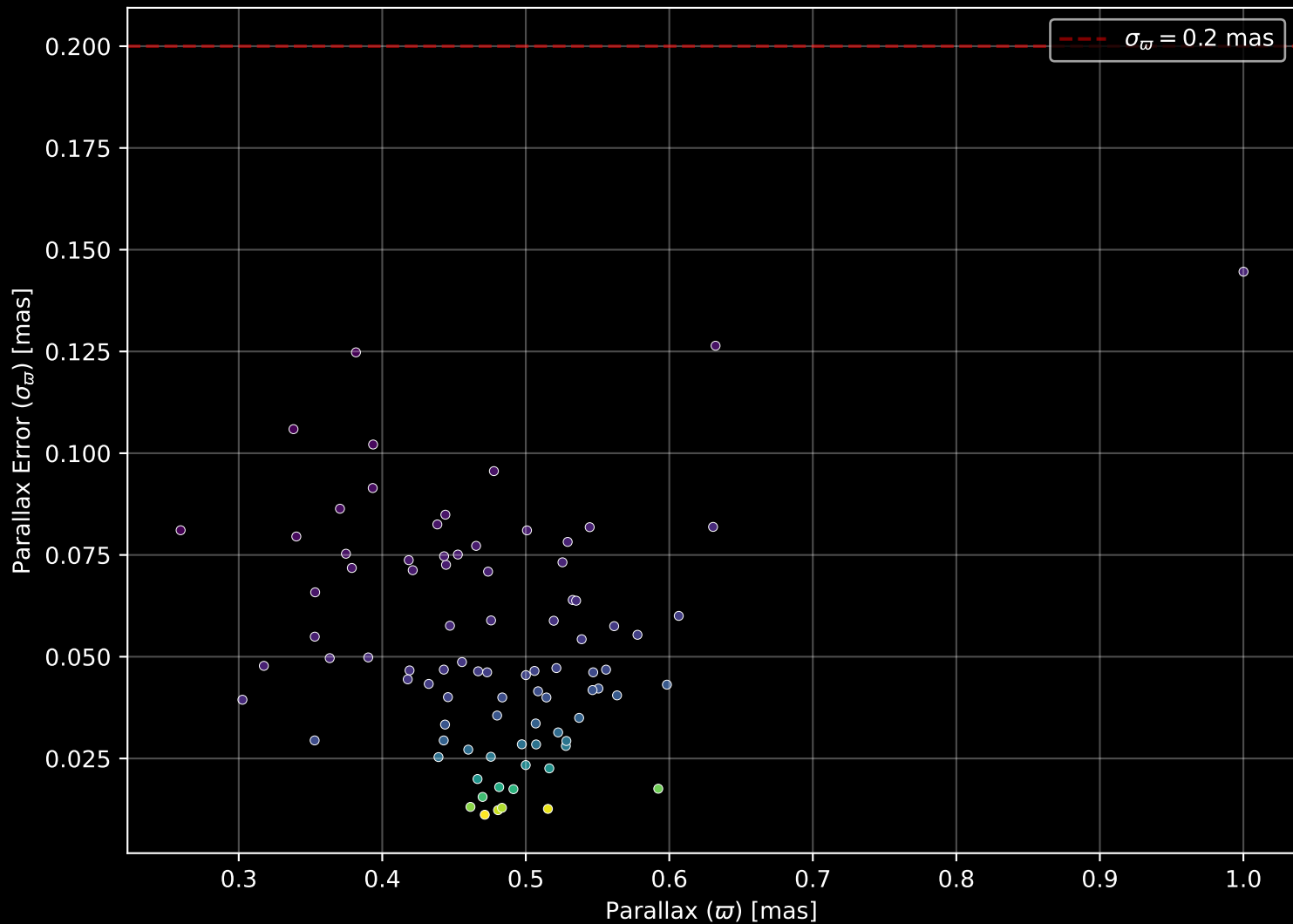
Gaia Cluster: [Dolidze_53] Parallax Quality (n= 87)
