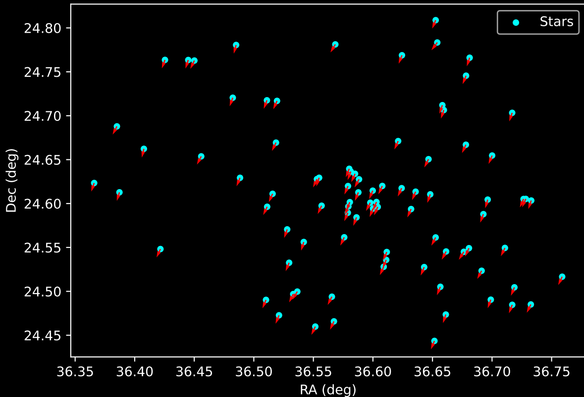
Gaia Cluster: [Dolidze_53] Proper Motion Vectors for Gaia Star Field (n= 87)
