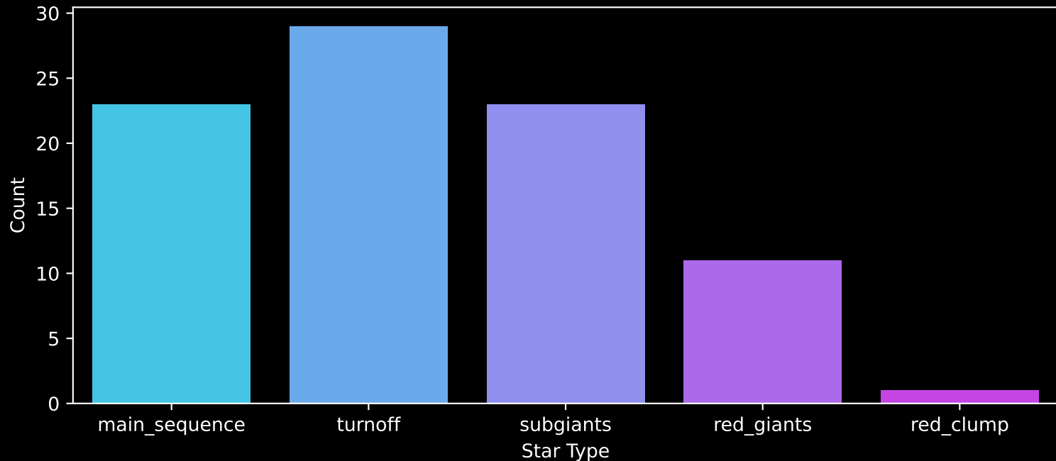
Gaia Cluster: [Dolidze_53] Count plot of Star Type
