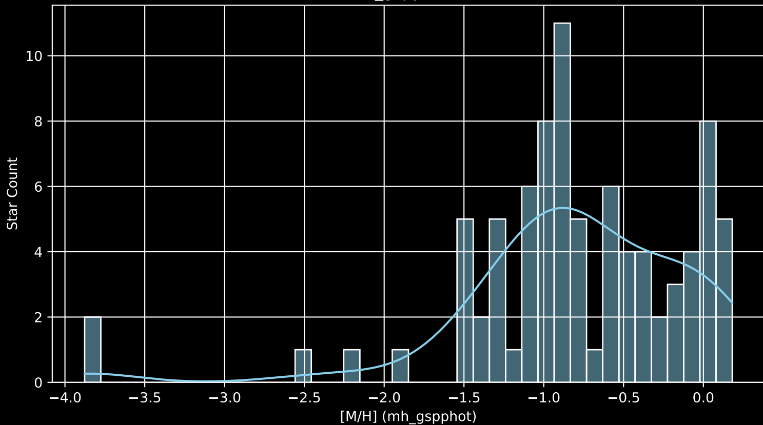
Gaia Cluster: [Dolidze_53 [M/H] (mh_gspphot) (n= 85)
