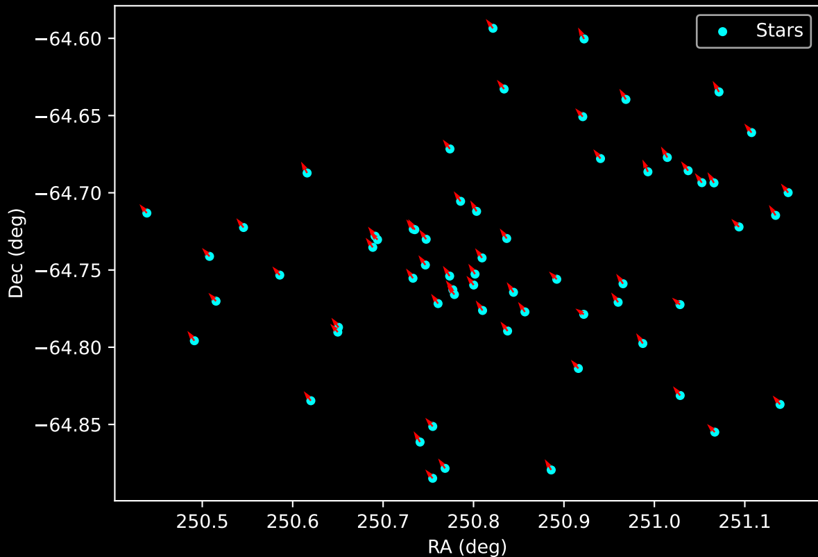
Gaia Cluster: [ESO_092_05] Proper Motion Vectors for Gaia Star Field (n= 64)
