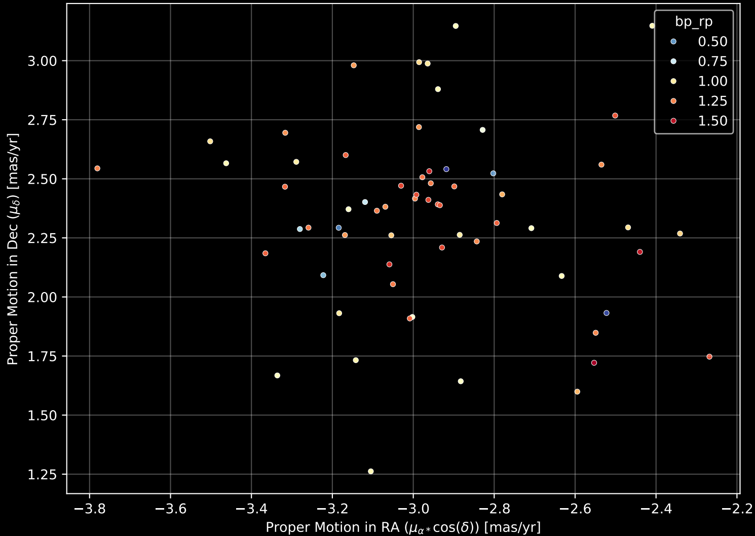
Gaia Cluster: [ESO 092 05] Proper Motion Diagram (n= 64)
