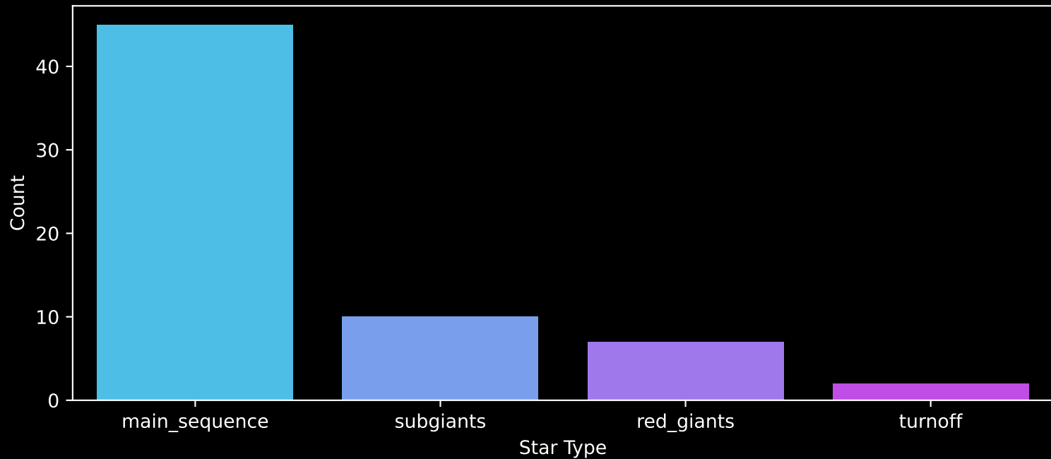
Gaia Cluster: [ESO_092_05] Count plot of Star Type
