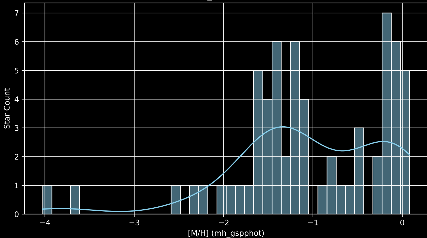
Gaia Cluster: [ESO_092_05 [M/H] (mh_gspphot) (n= 64)
