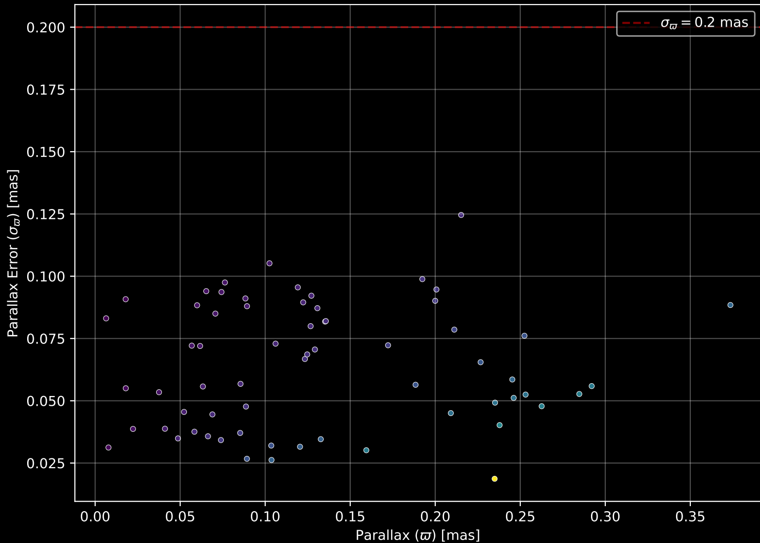
Gaia Cluster: [ESO_092_05] Parallax Quality (n= 64)
