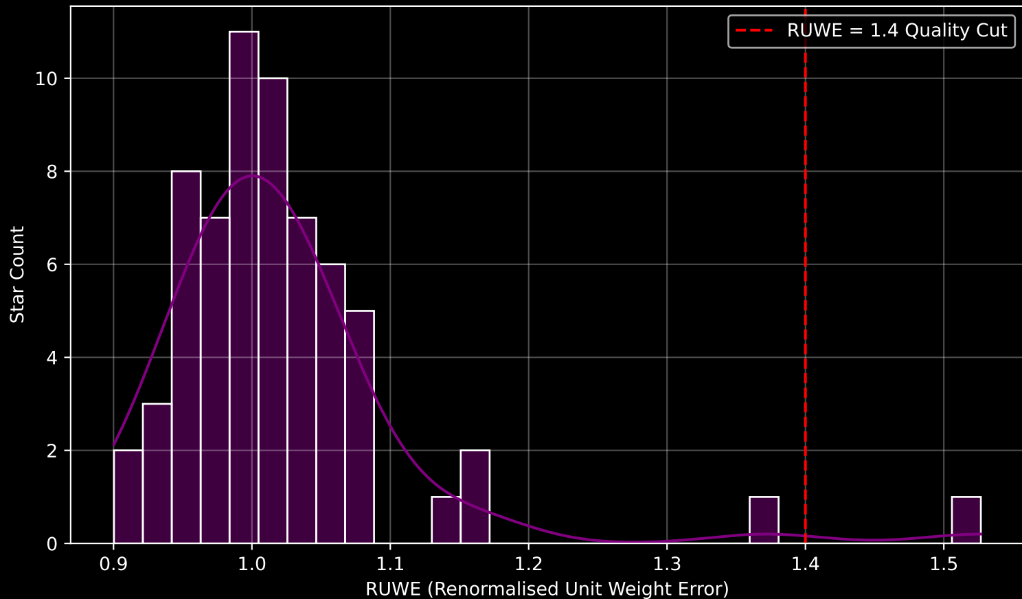
Gaia Cluster: [ESO_092_05] RUWE Distribution (n= 64)
