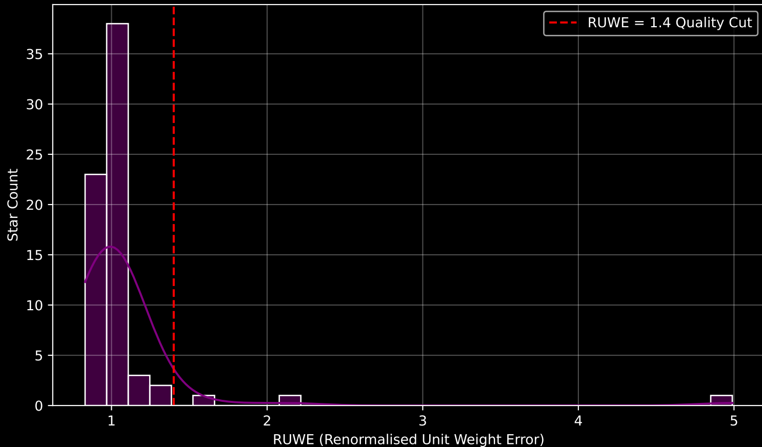
Gaia Cluster: [ESO_130_06] RUWE Distribution (n= 69)
