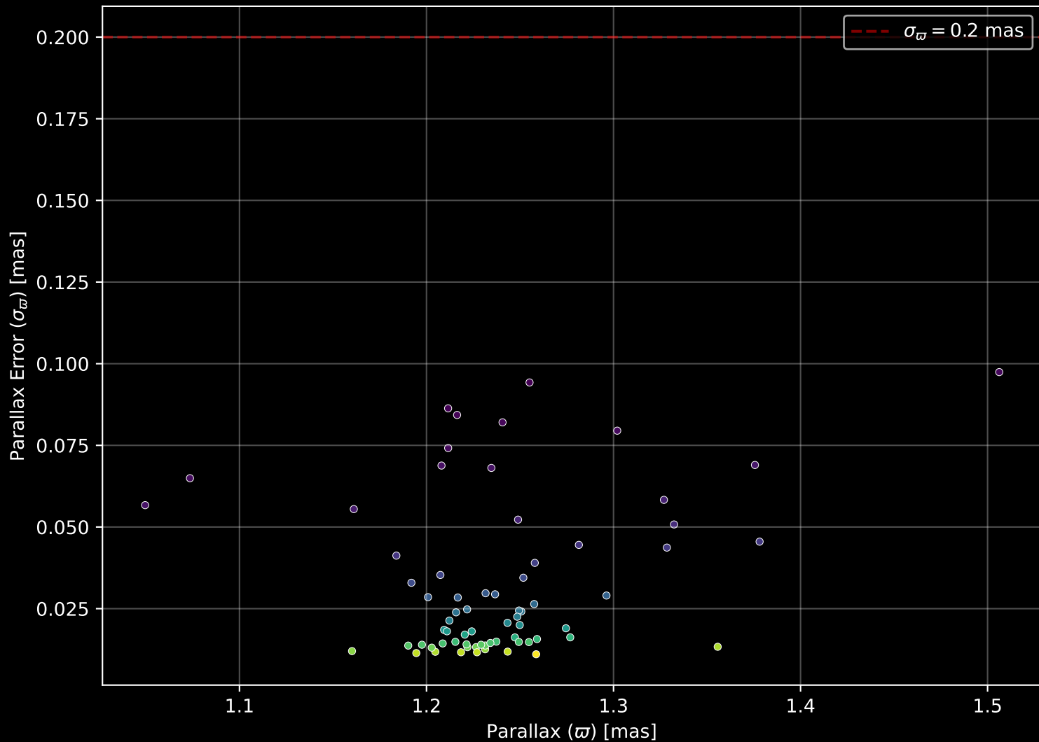
Gaia Cluster: [ESO_130_06] Parallax Quality (n= 69)
