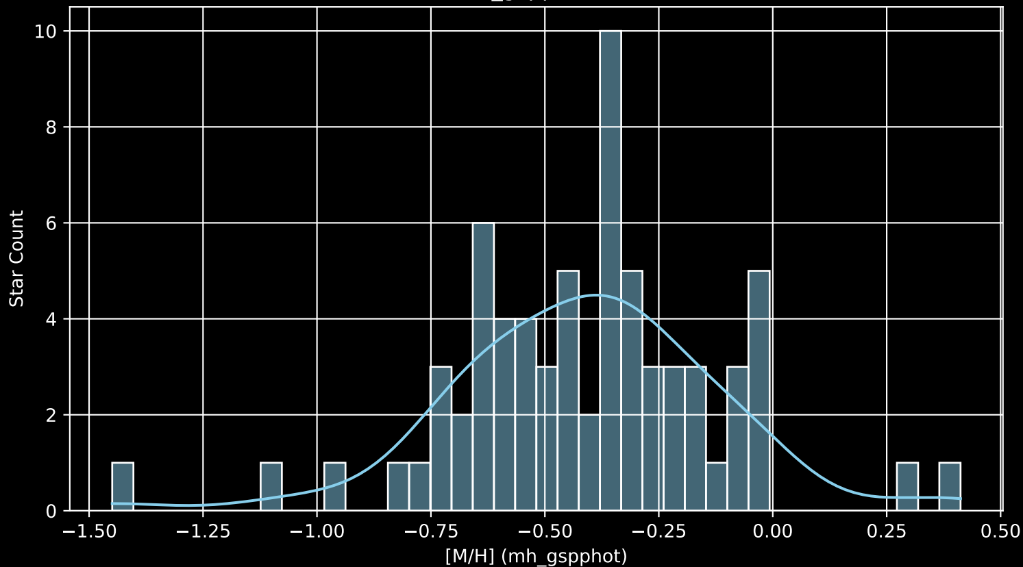
Gaia Cluster: [ESO_130_06 [M/H] (mh_gspphot) (n= 69)
