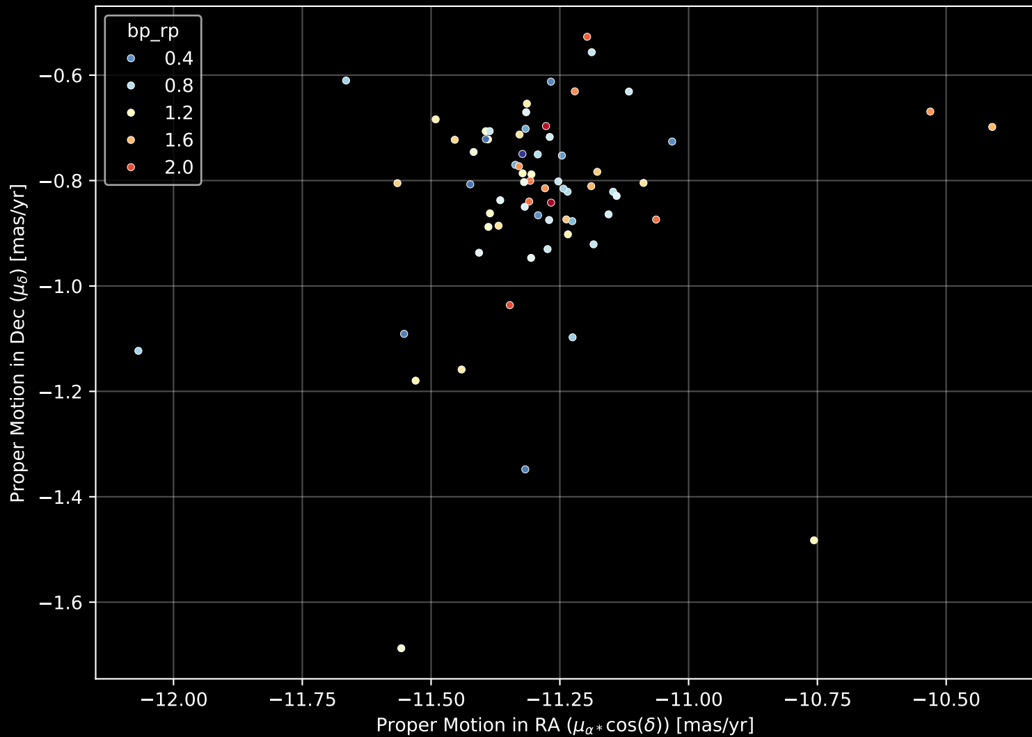
Gaia Cluster: [ESO_130_06] Proper Motion Diagram (n= 69)
