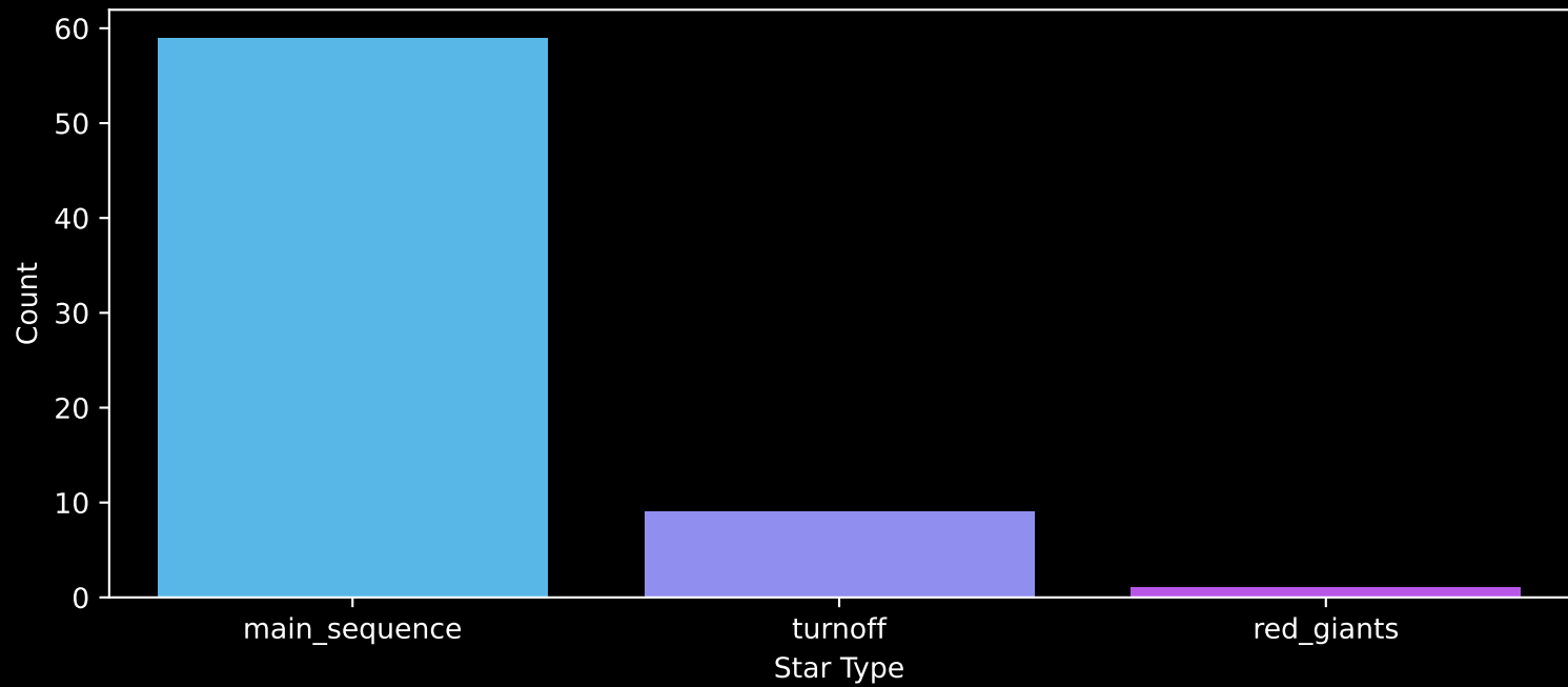
Gaia Cluster: [ESO_130_06] Count plot of Star Type
