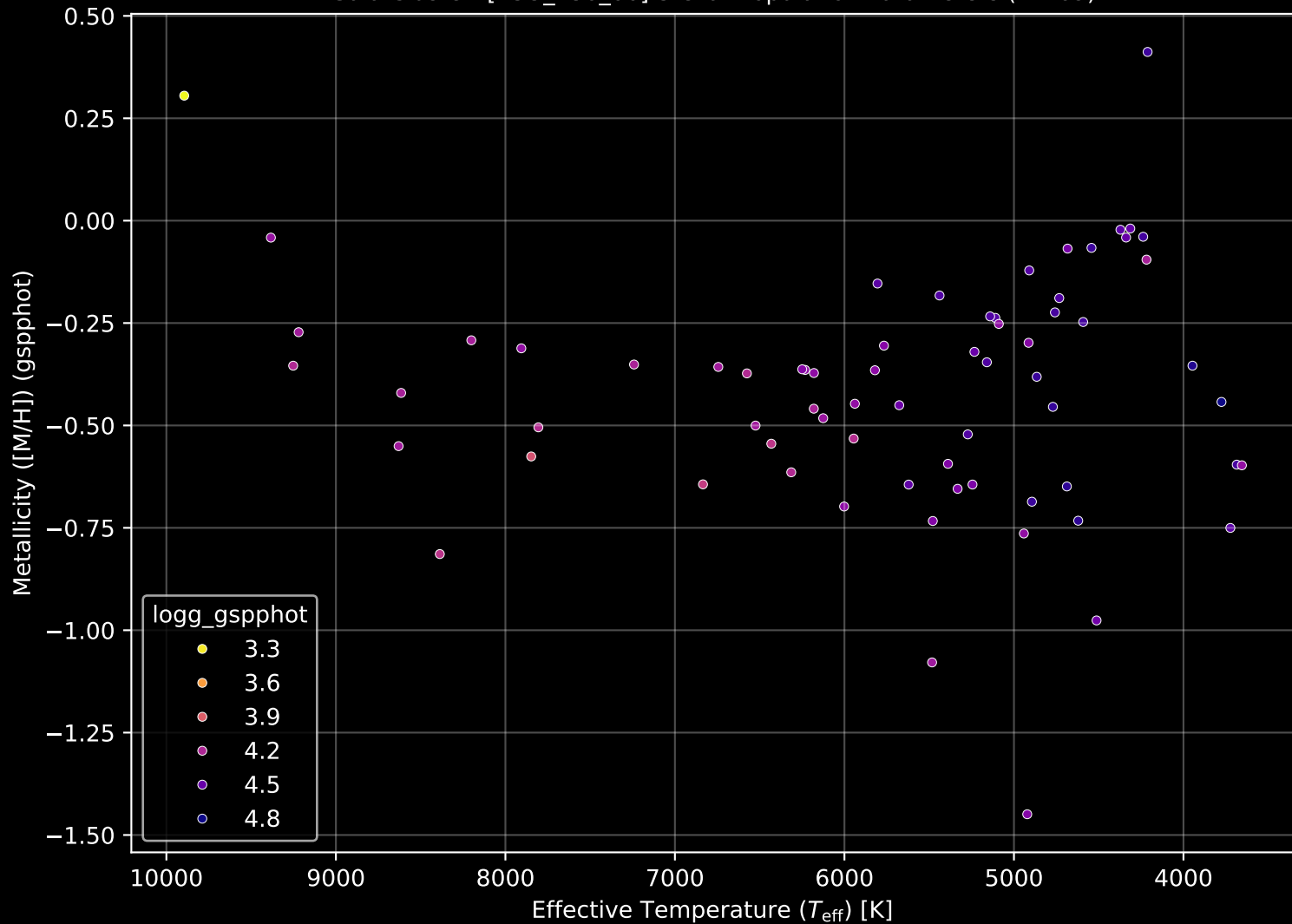
Gaia Cluster: [ESO_130_06] Stellar Population Parameters (n= 69)
