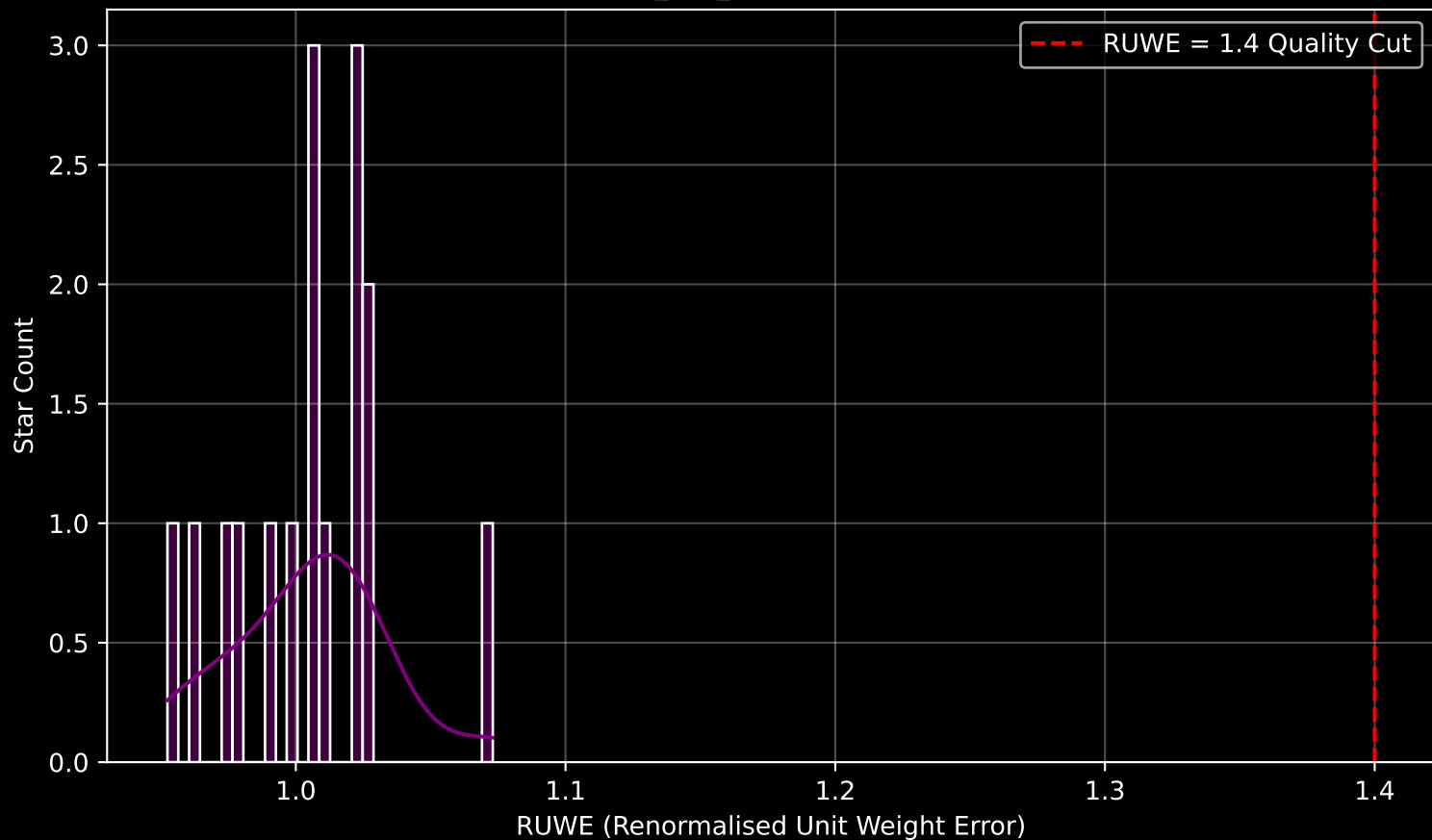
Gaia Cluster: [ESO_211_09] RUWE Distribution (n= 16)
