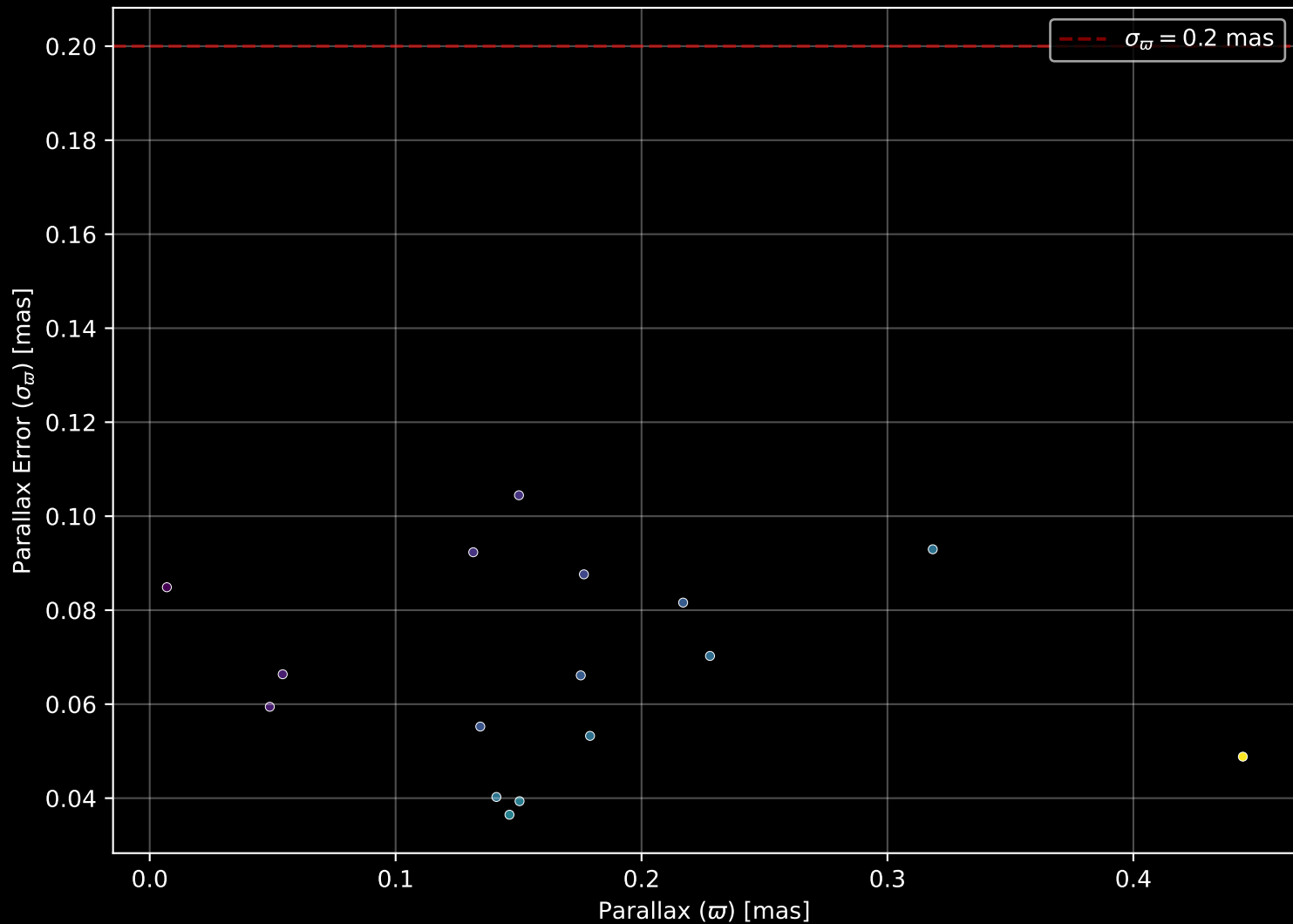
Gaia Cluster: [ESO_211_09] Parallax Quality (n= 16)
