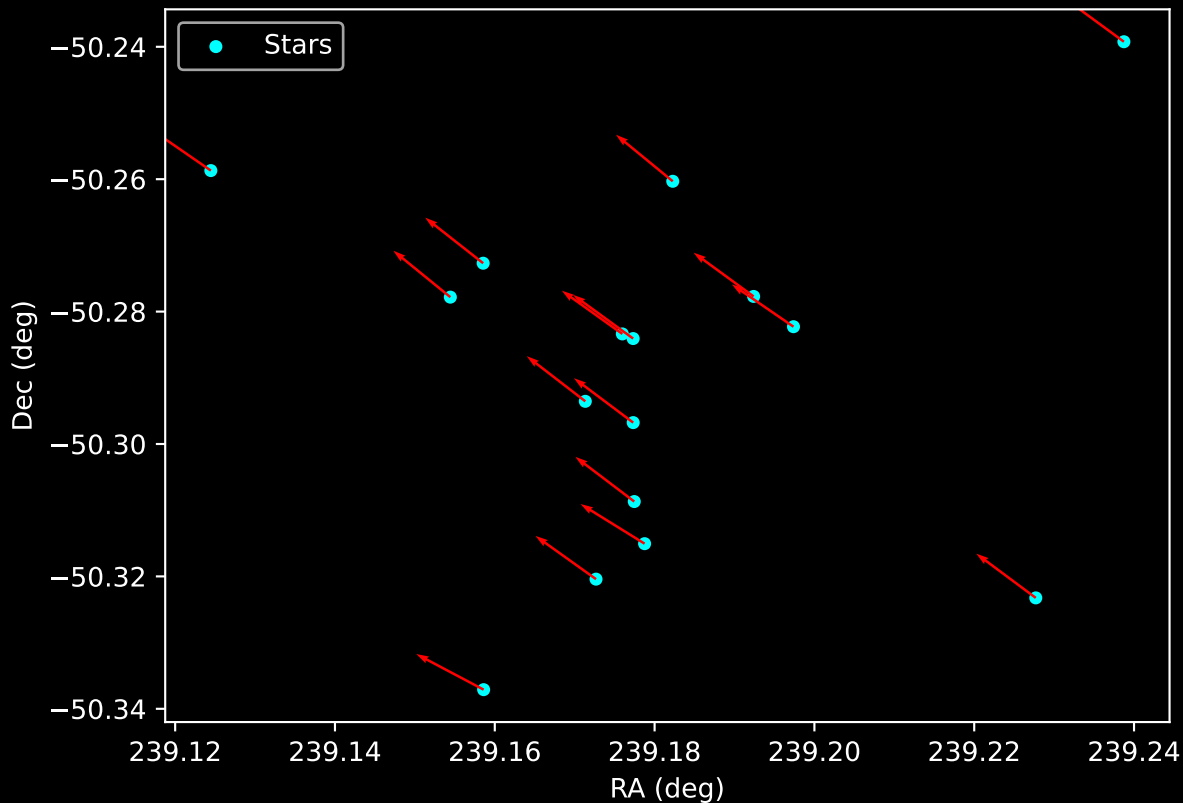
Gaia Cluster: [ESO_211_09] Proper Motion Vectors for Gaia Star Field (n= 16)
