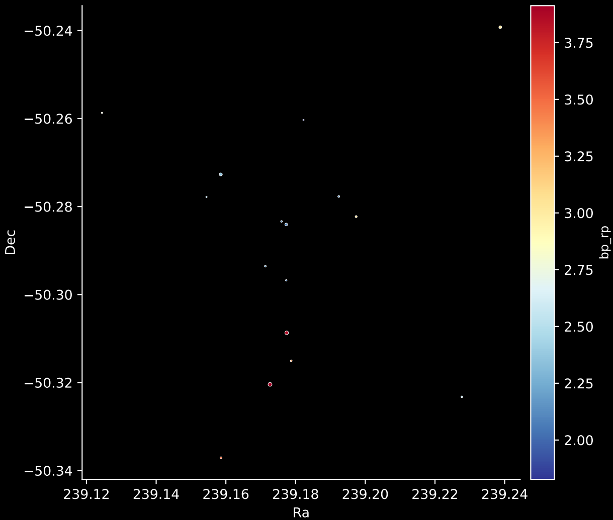
Gaia Cluster: [ESO_211_09] Stars: 16
