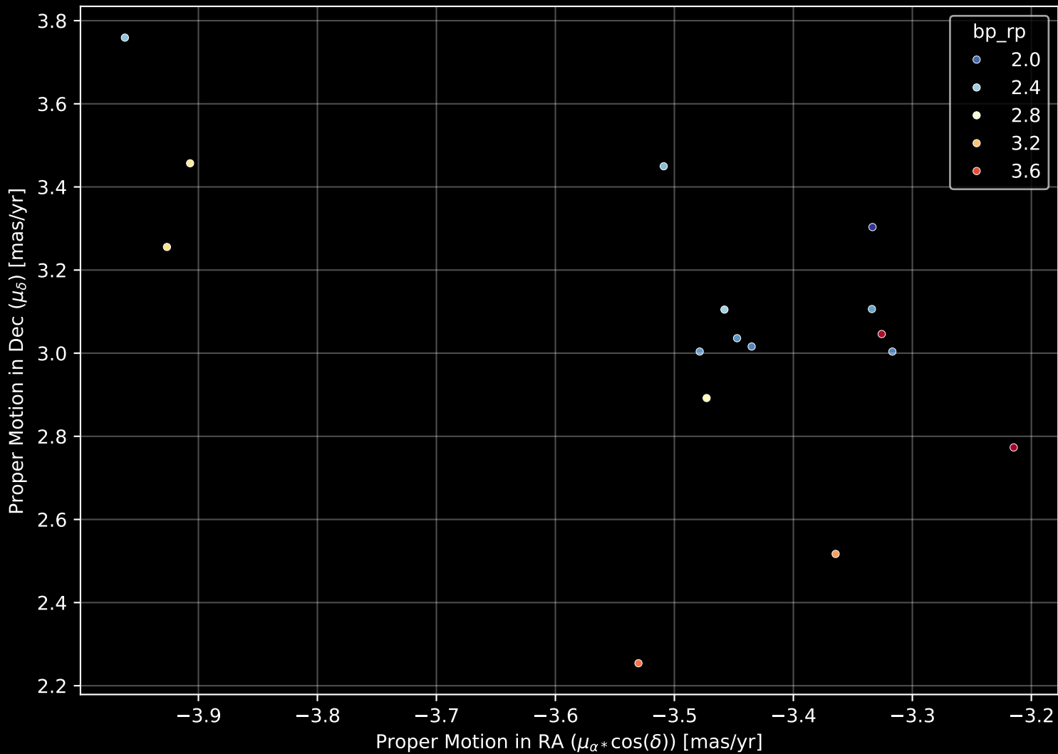
Gaia Cluster: [ESO_211_09] Proper Motion Diagram (n= 16)
