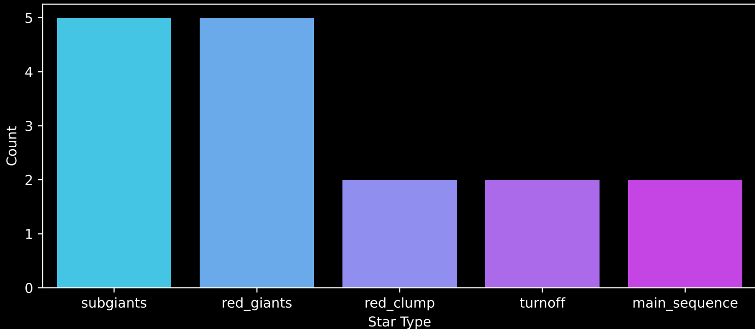
Gaia Cluster: [ESO_211_09] Count plot of Star Type
