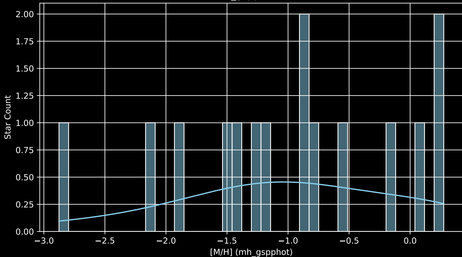
Gaia Cluster: [ESO_211_09 [M/H] (mh_gspphot) (n= 15)
