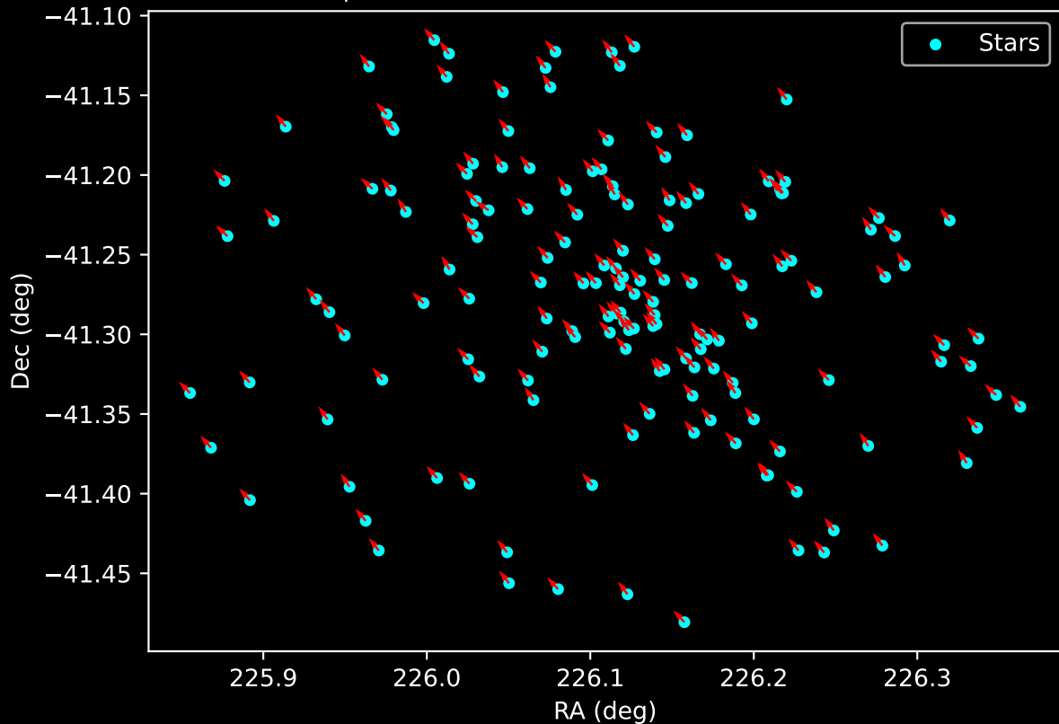
Gaia Cluster: [ESO_312_03] Proper Motion Vectors for Gaia Star Field (n= 159)
