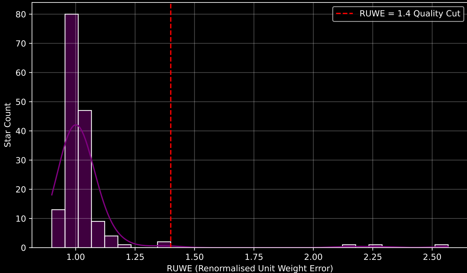
Gaia Cluster: [ESO_312_03] RUWE Distribution (n= 159)
