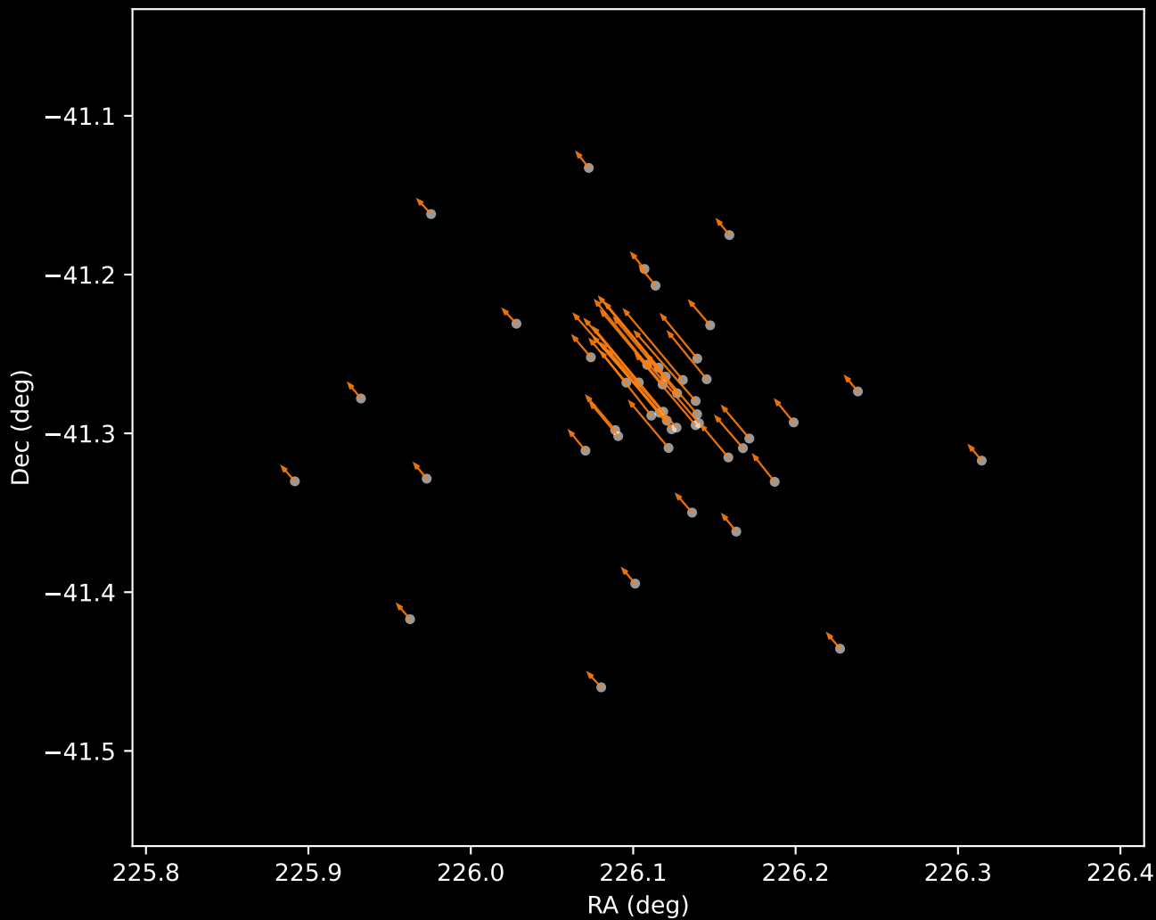
Gaia DR3 Cluster 2 Proper Motion Vectors (n=48)
