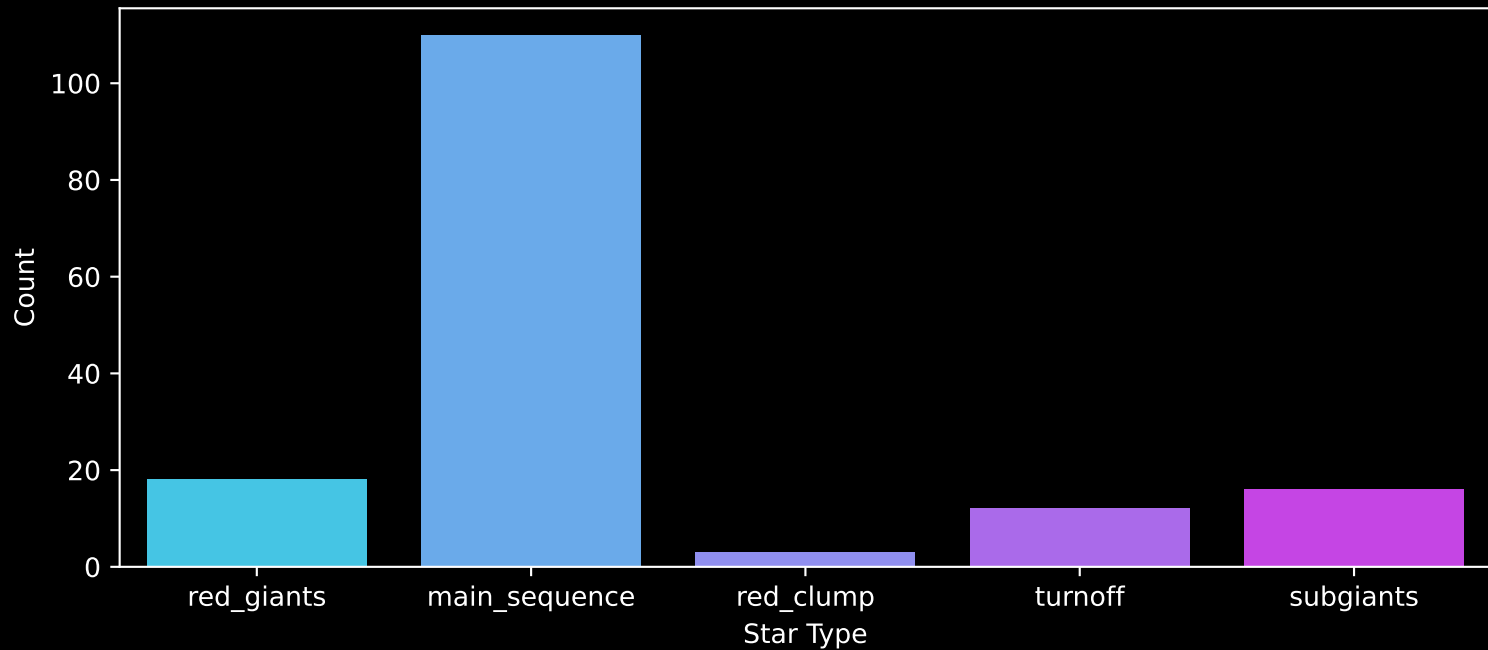
Gaia Cluster: [ESO_312_03] Count plot of Star Type
