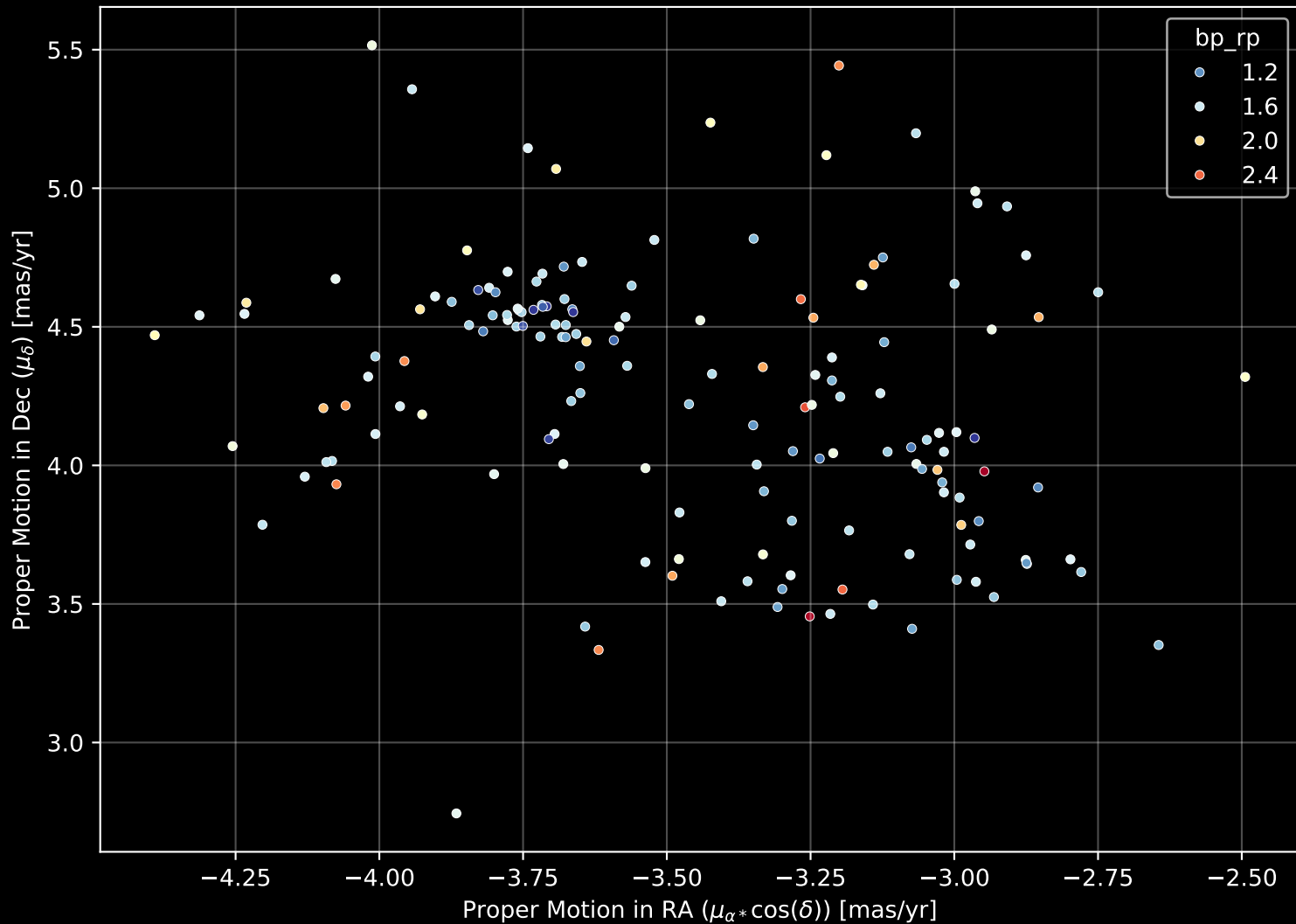
Gaia Cluster: [ESO_312_03] Proper Motion Diagram (n= 159)
