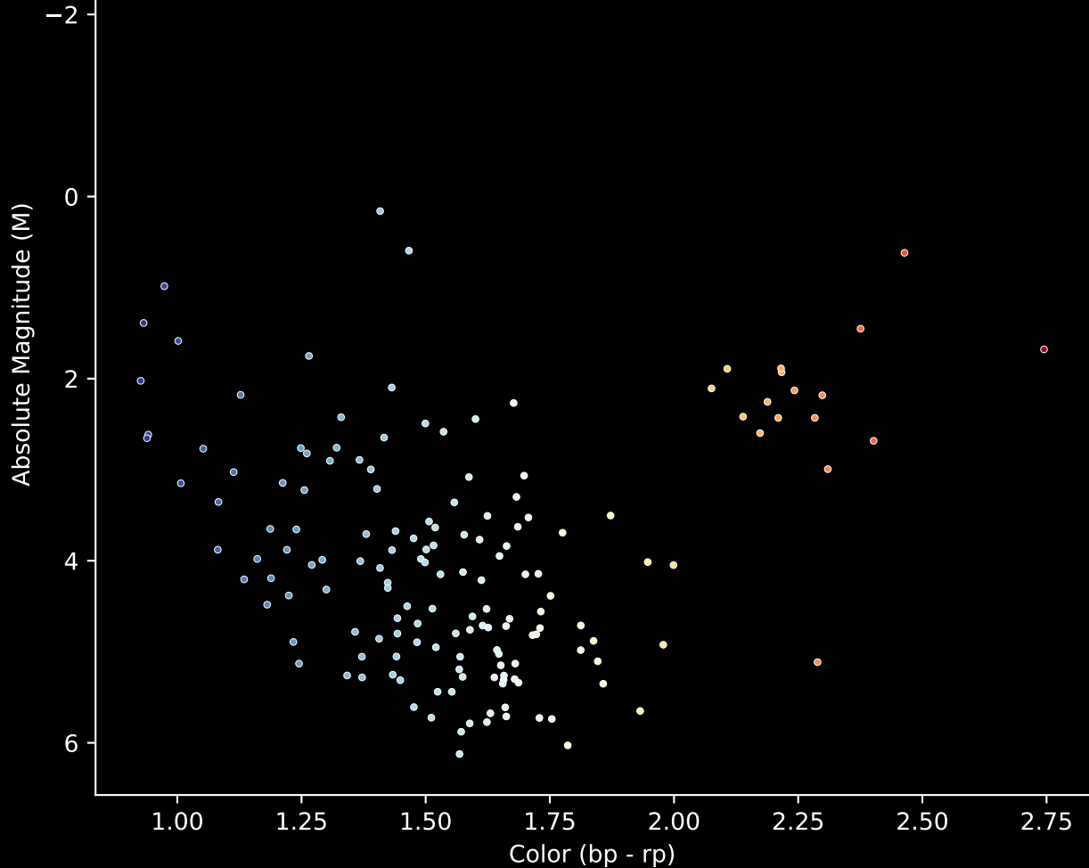
Gaia Cluster: [ESO_312_03] Stars (n= 159) Hertzprung-Russel Diagram
