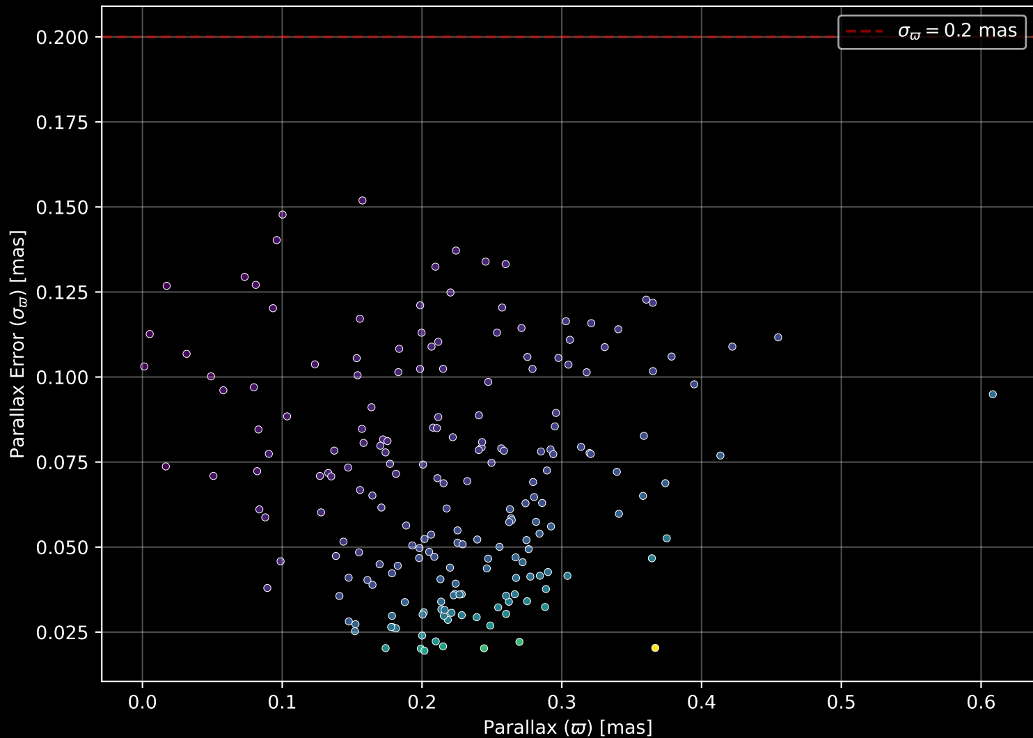
Gaia Cluster: [FSR_0123] Parallax Quality (n= 201)
