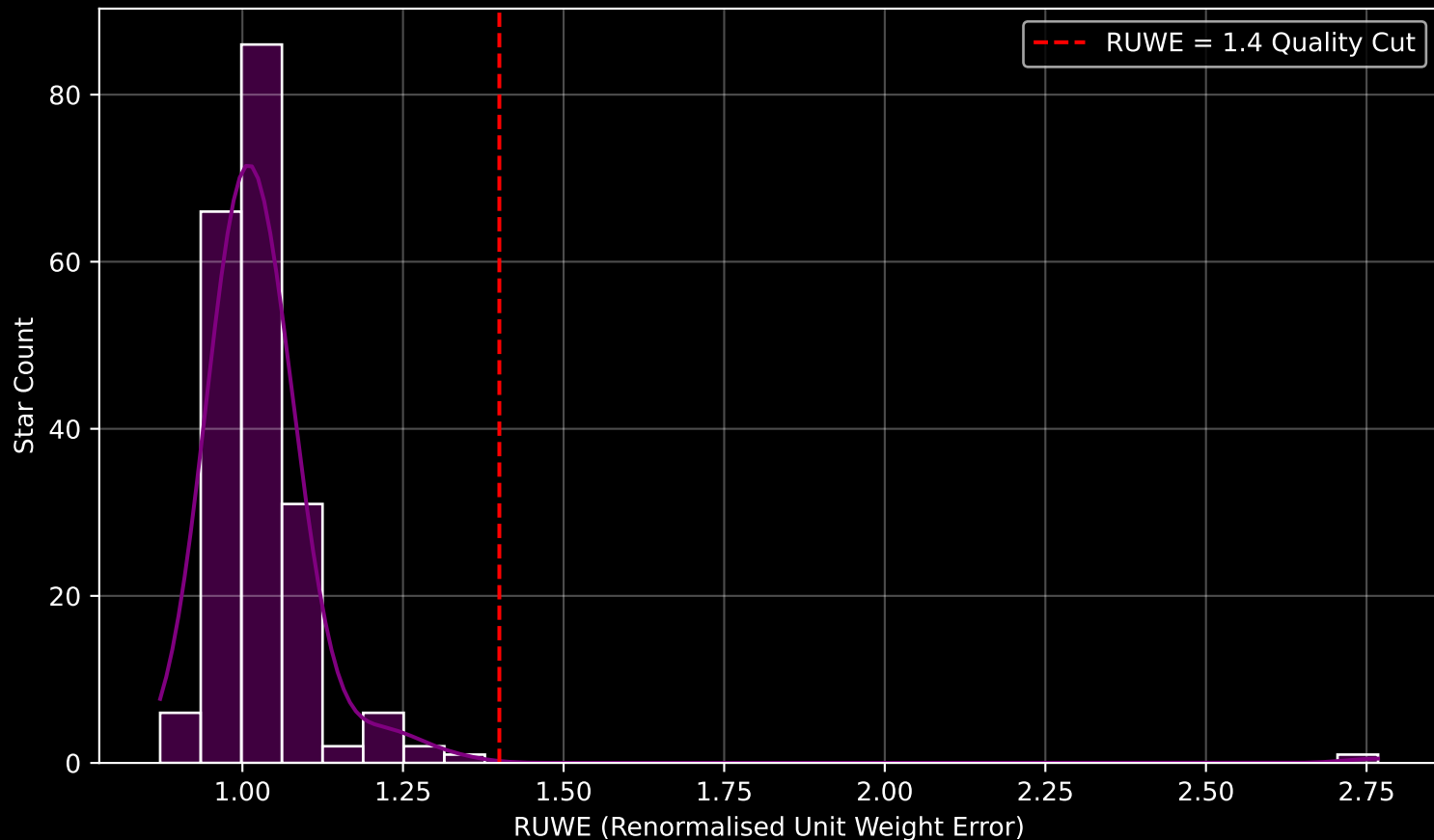
Gaia Cluster: [FSR_0123] RUWE Distribution (n= 201)
