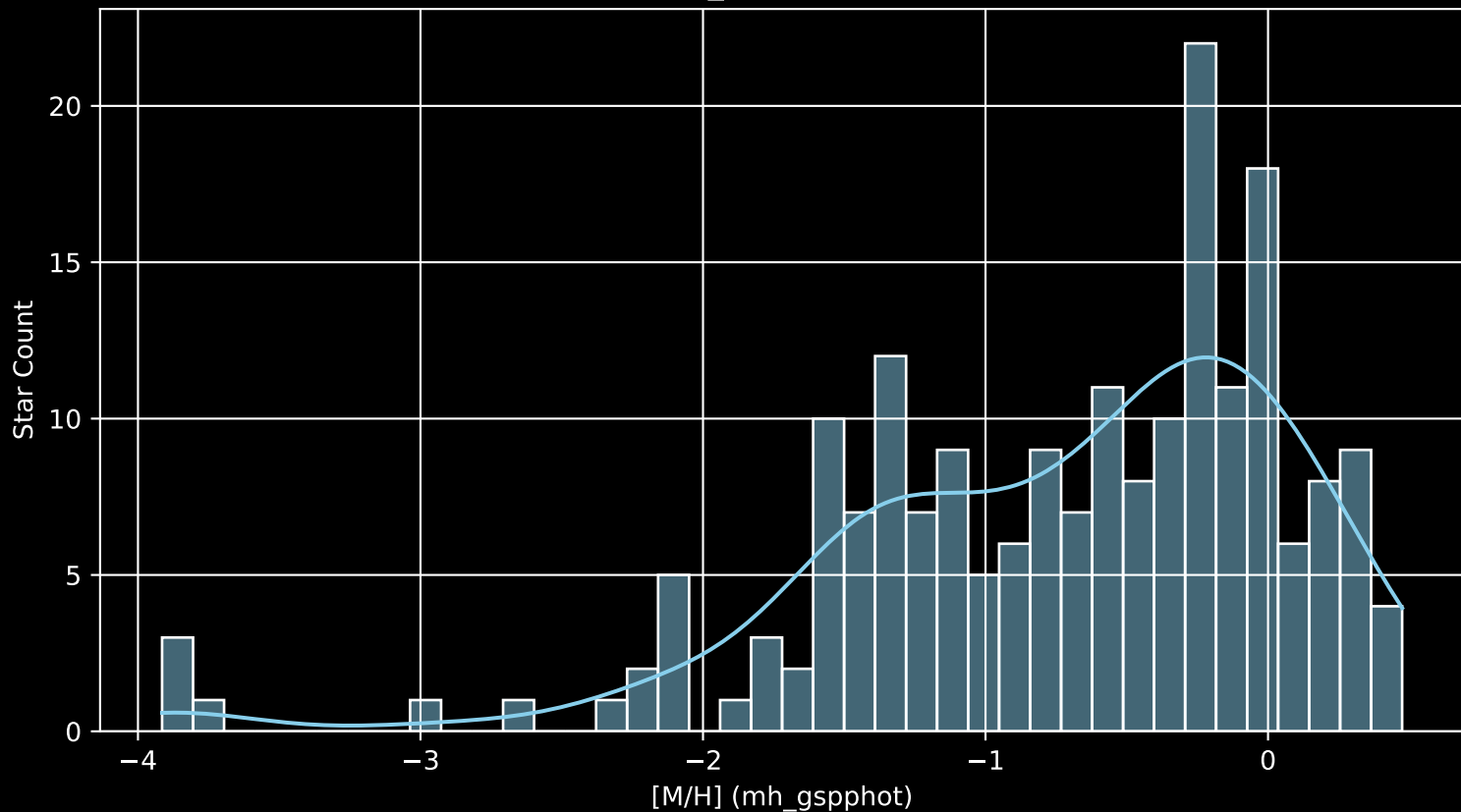
Gaia Cluster: [FSR_0123 [M/H] (mh_gspphot) (n= 199)
