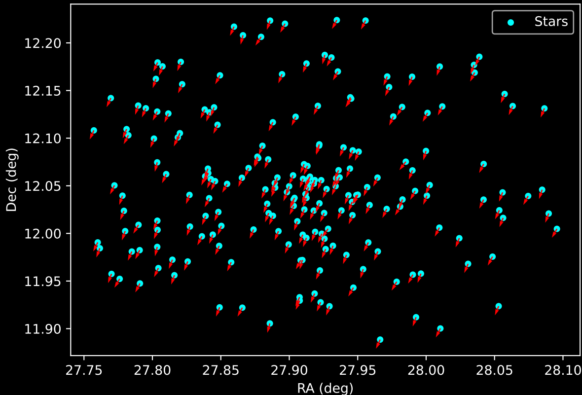
Gaia Cluster: [FSR_0123] Proper Motion Vectors for Gaia Star Field (n= 201)
