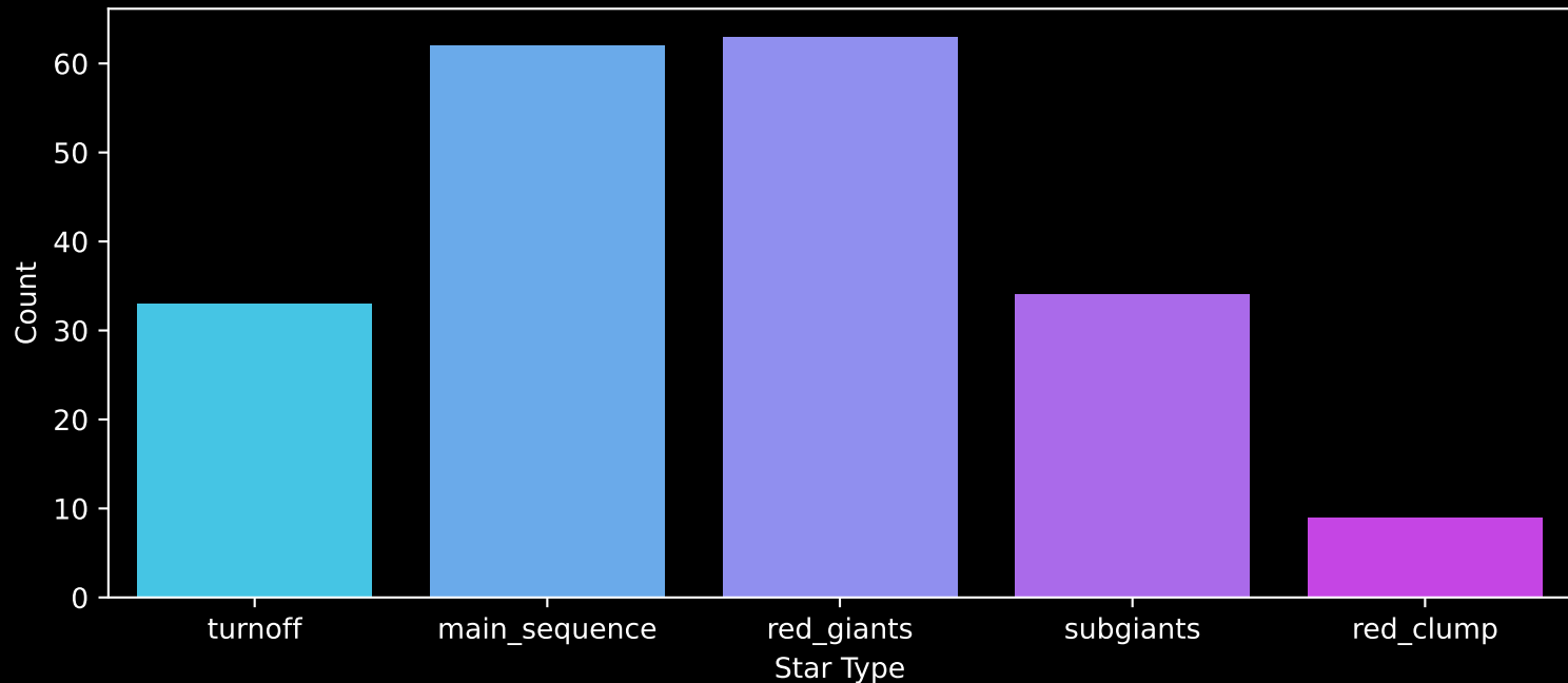
Gaia Cluster: [FSR_0123] Count plot of Star Type
