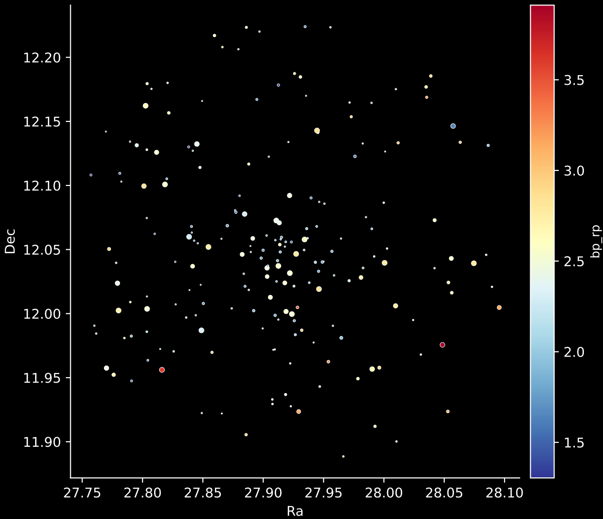
Gaia Cluster: [FSR_0123] Stars: 201
