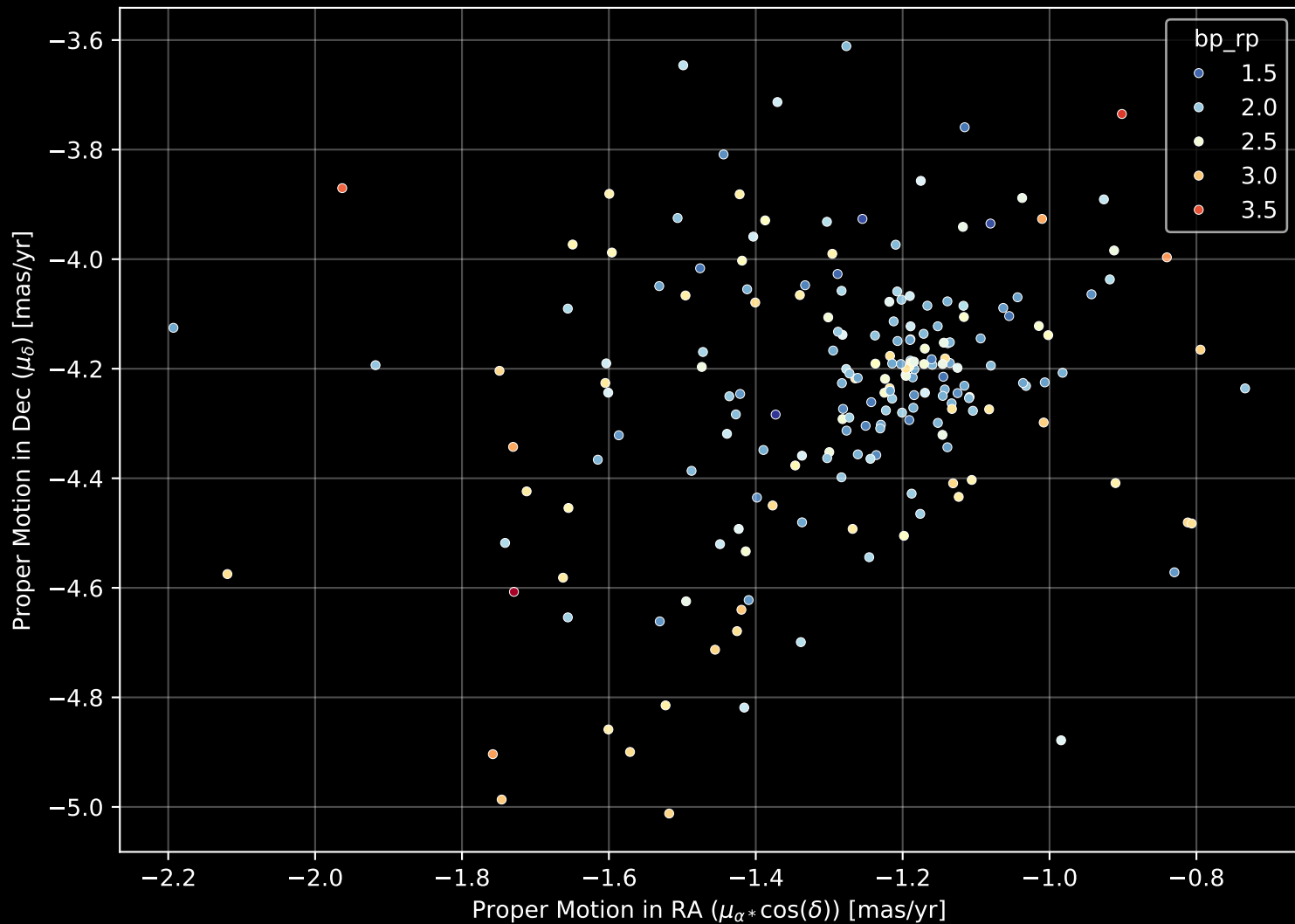
Gaia Cluster: [FSR_0123] Proper Motion Diagram (n= 201)
