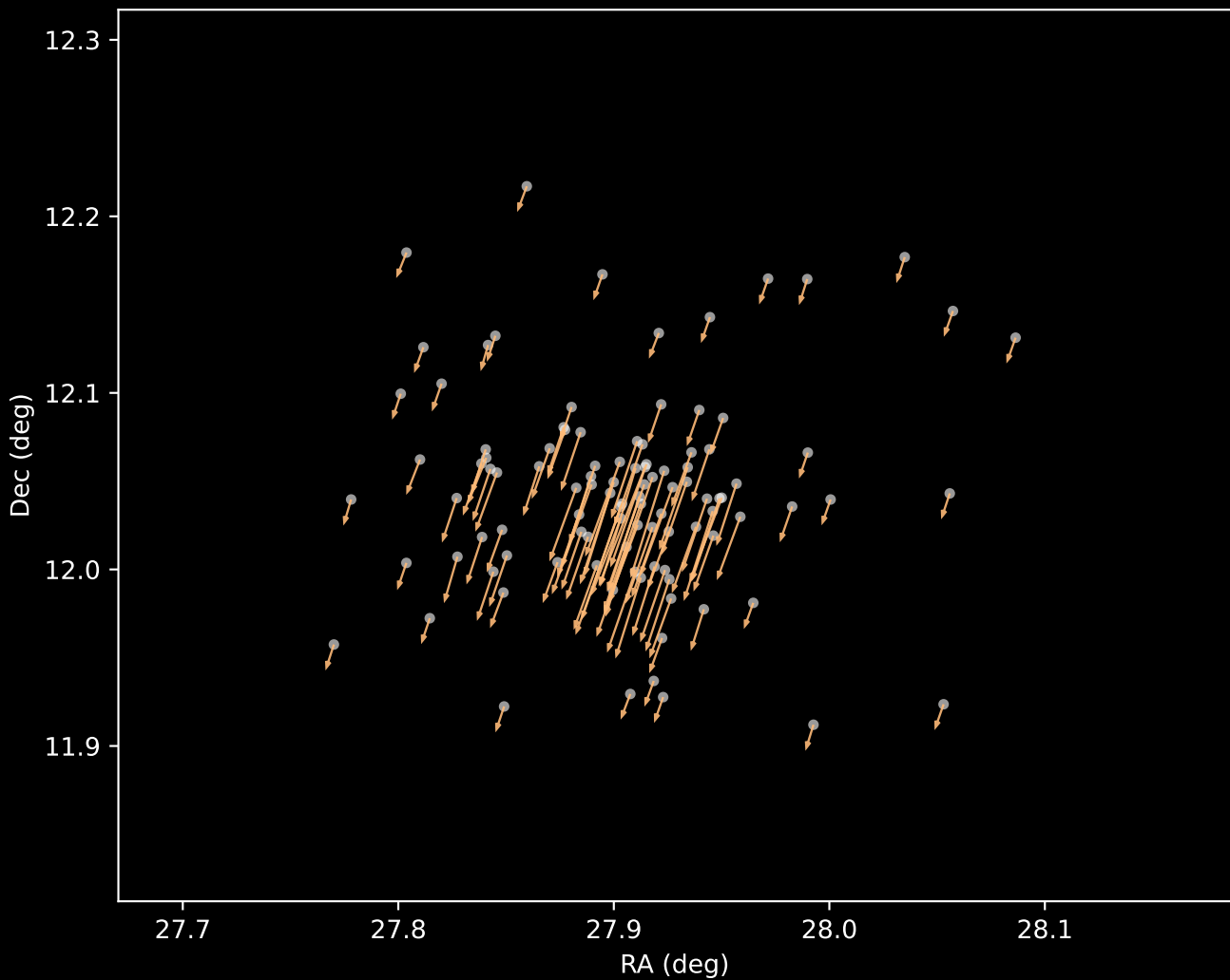
Gaia DR3 Cluster 3 Proper Motion Vectors (n=104)
