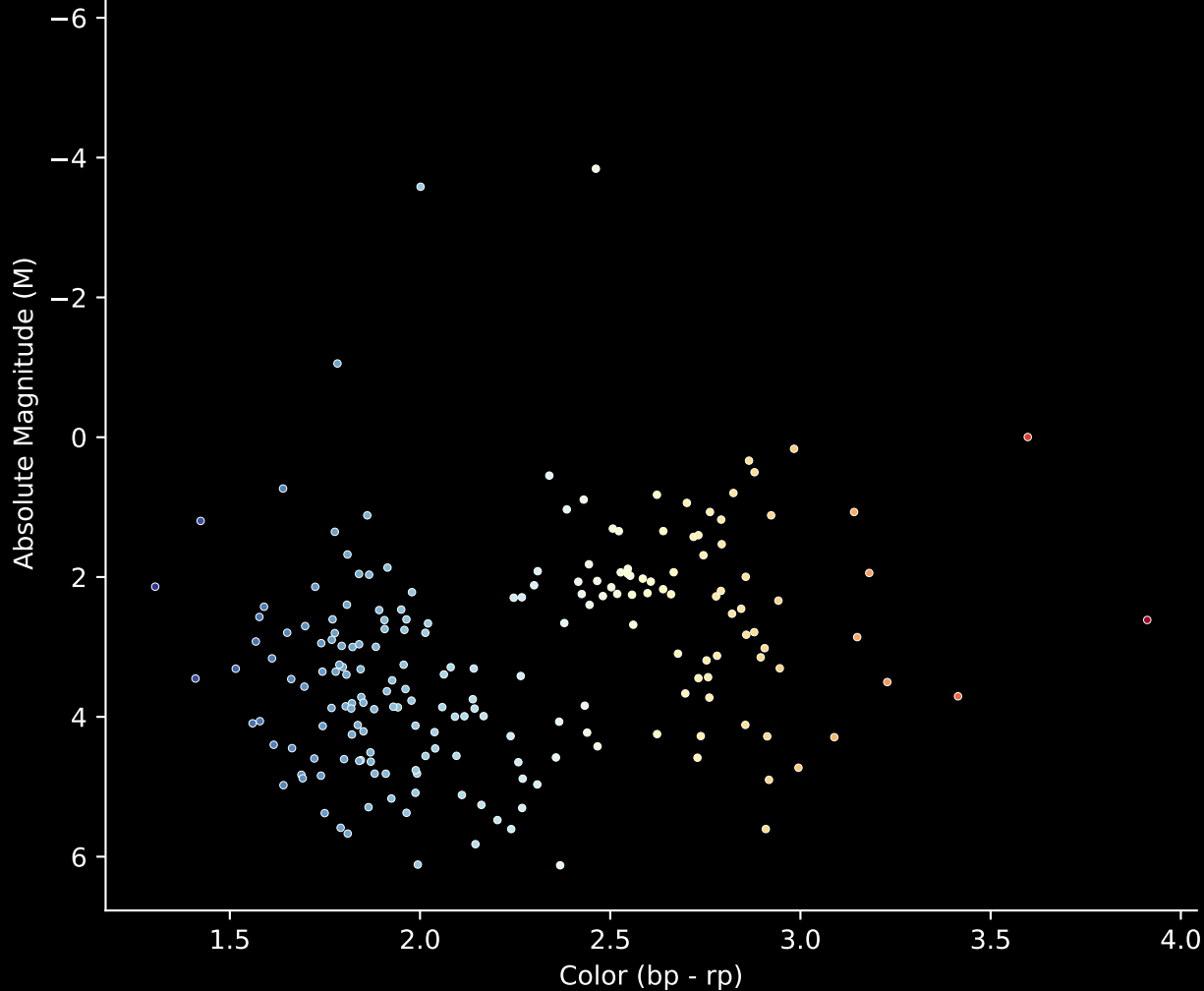
Gaia Cluster: [FSR_0123] Stars (n= 201) Hertzsprung-Russel Diagram
