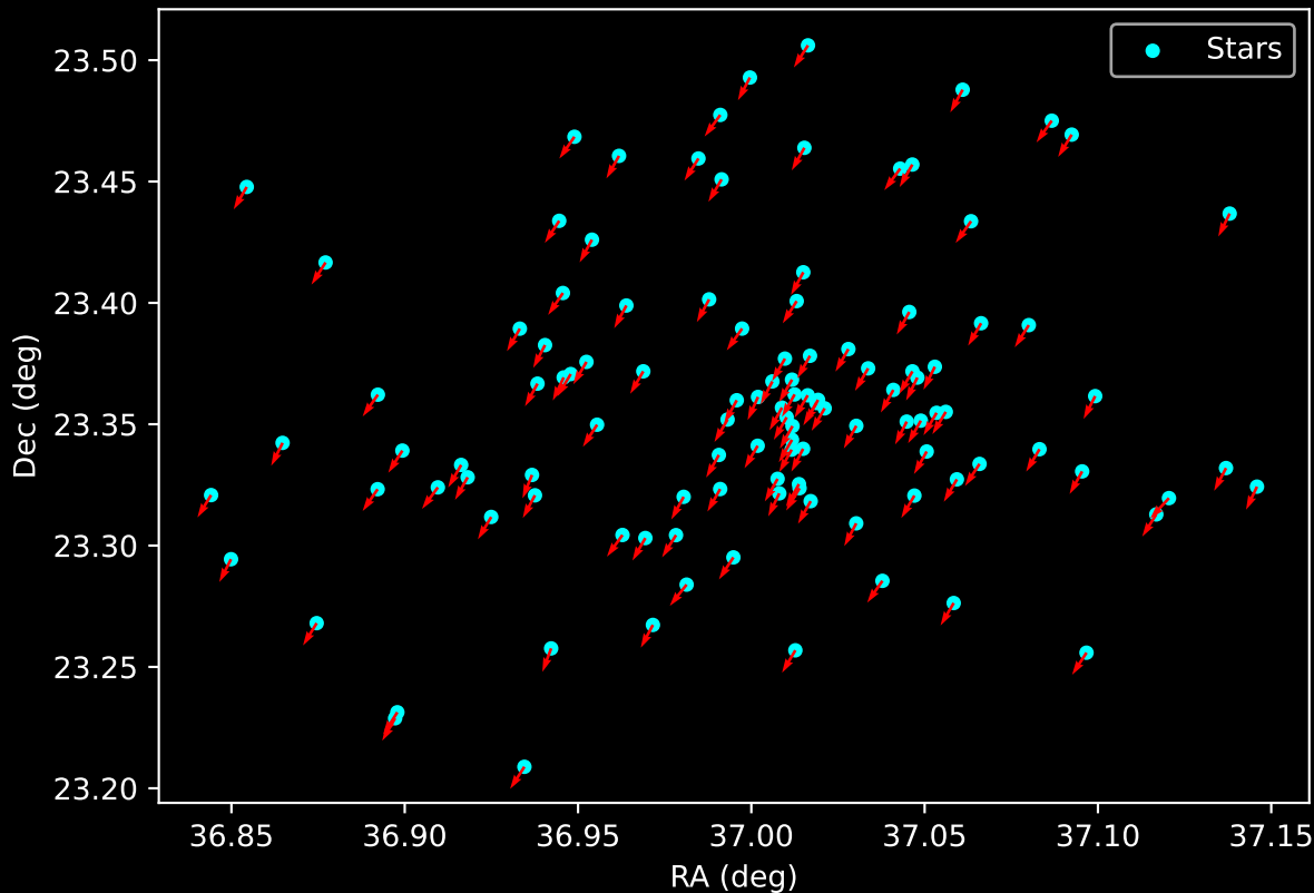
Gaia Cluster: [FSR_0154] Proper Motion Vectors for Gaia Star Field (n= 113)
