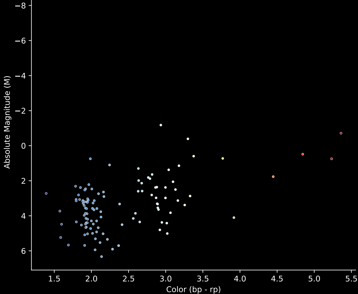
Gaia Cluster: [FSR_0154] Stars (n= 113) Hertzprung-Russel Diagram
