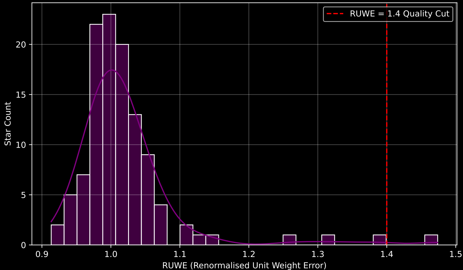
Gaia Cluster: [FSR_0154] RUWE Distribution (n= 113)
