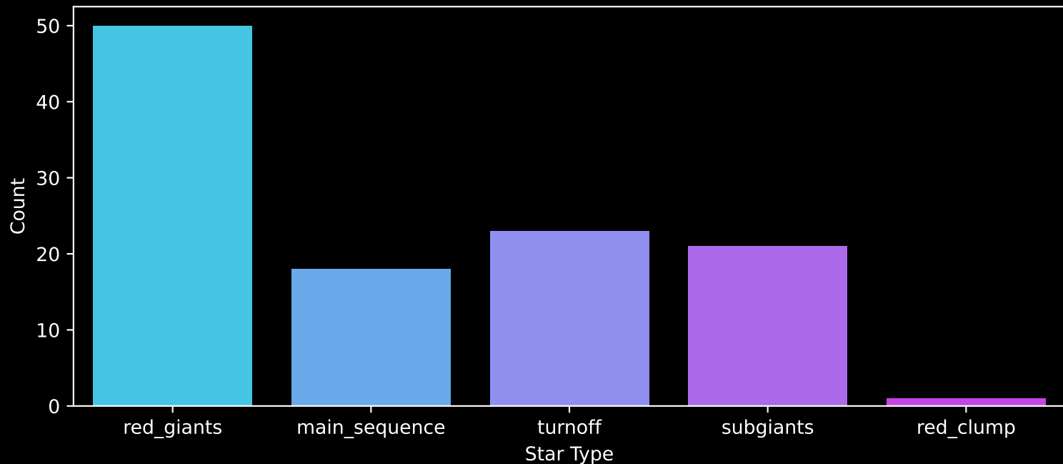
Gaia Cluster: [FSR_0154] Count plot of Star Type
