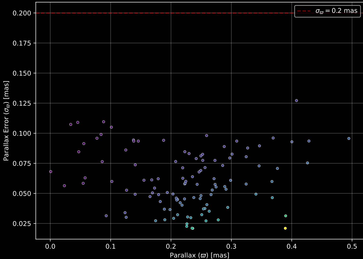
Gaia Cluster: [FSR_0154] Parallax Quality (n= 113)
