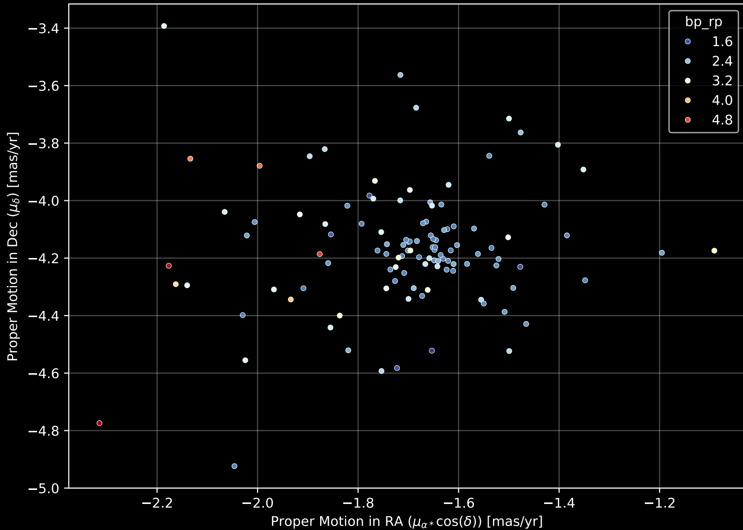
Gaia Cluster: [FSR_0154] Proper Motion Diagram (n= 113)
