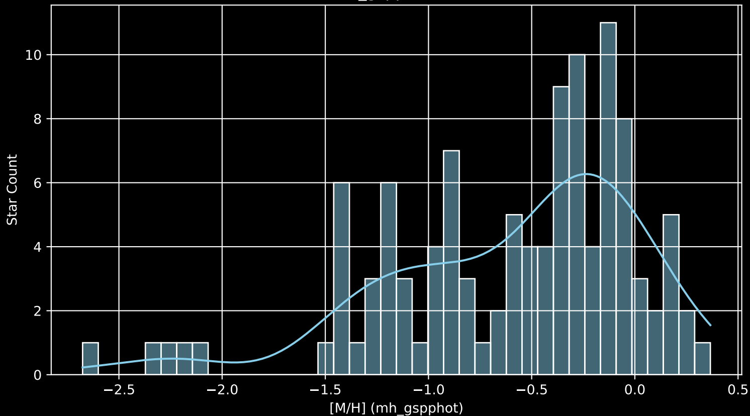
Gaia Cluster: [FSR_0154 [M/H] (mh_gspphot) (n= 111)
