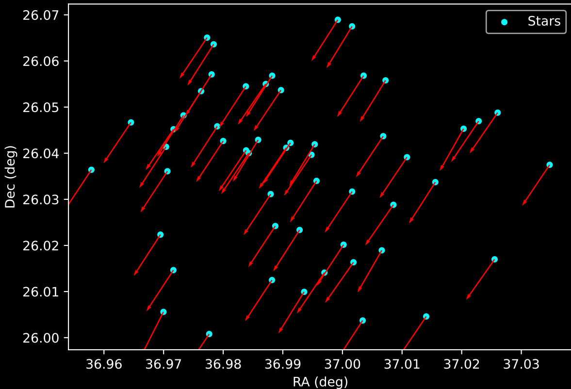
Gaia Cluster: [FSR_0158] Proper Motion Vectors for Gaia Star Field (n= 53)
