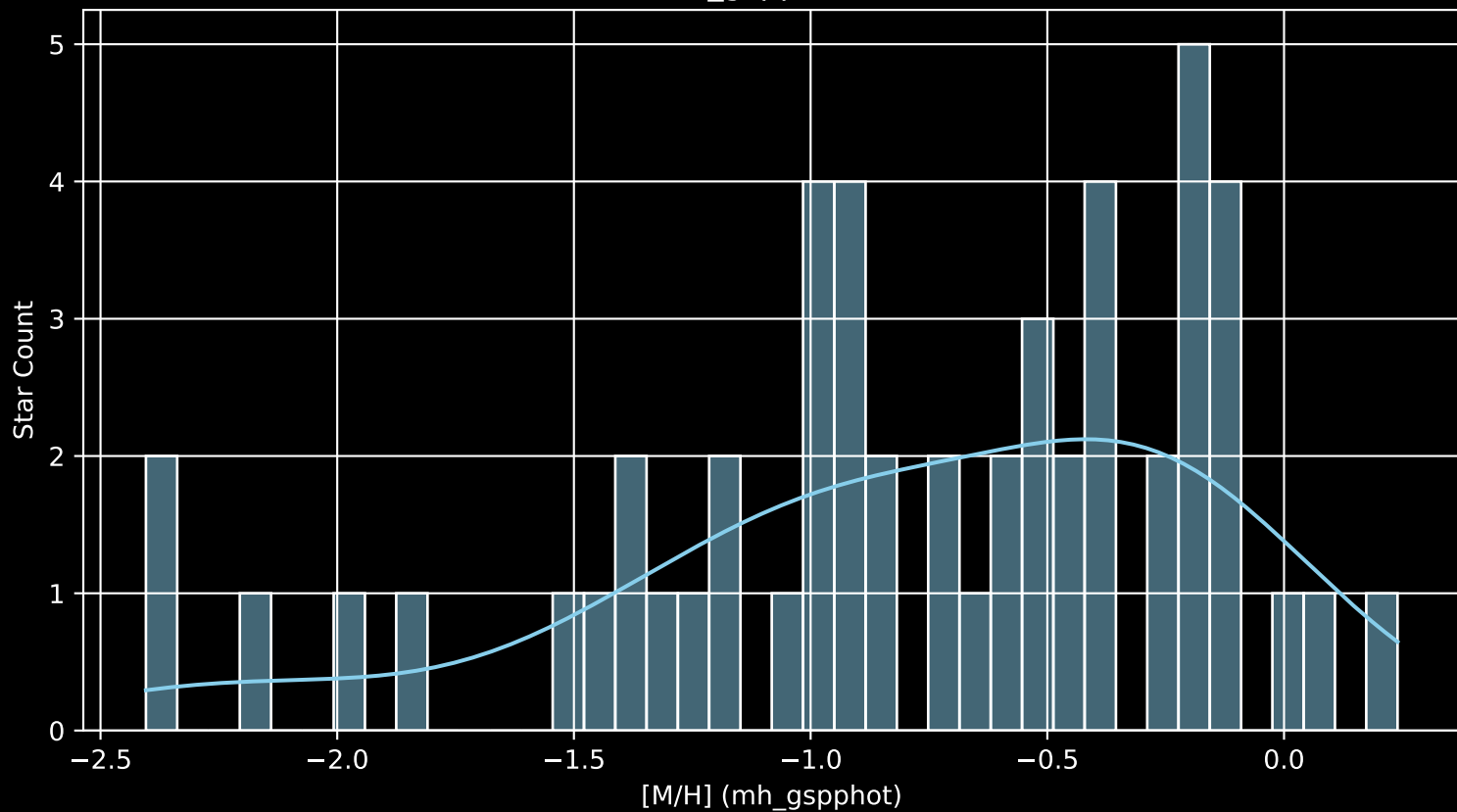
Gaia Cluster: [FSR_0158 [M/H] (mh_gspphot) (n= 52)
