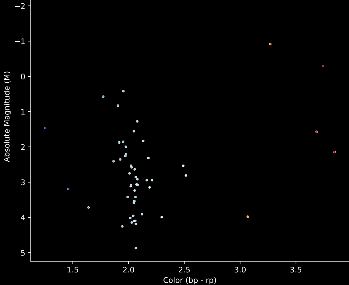
Gaia Cluster: [FSR_0158] Stars (n= 53) Hertzsprung-Russel Diagram
