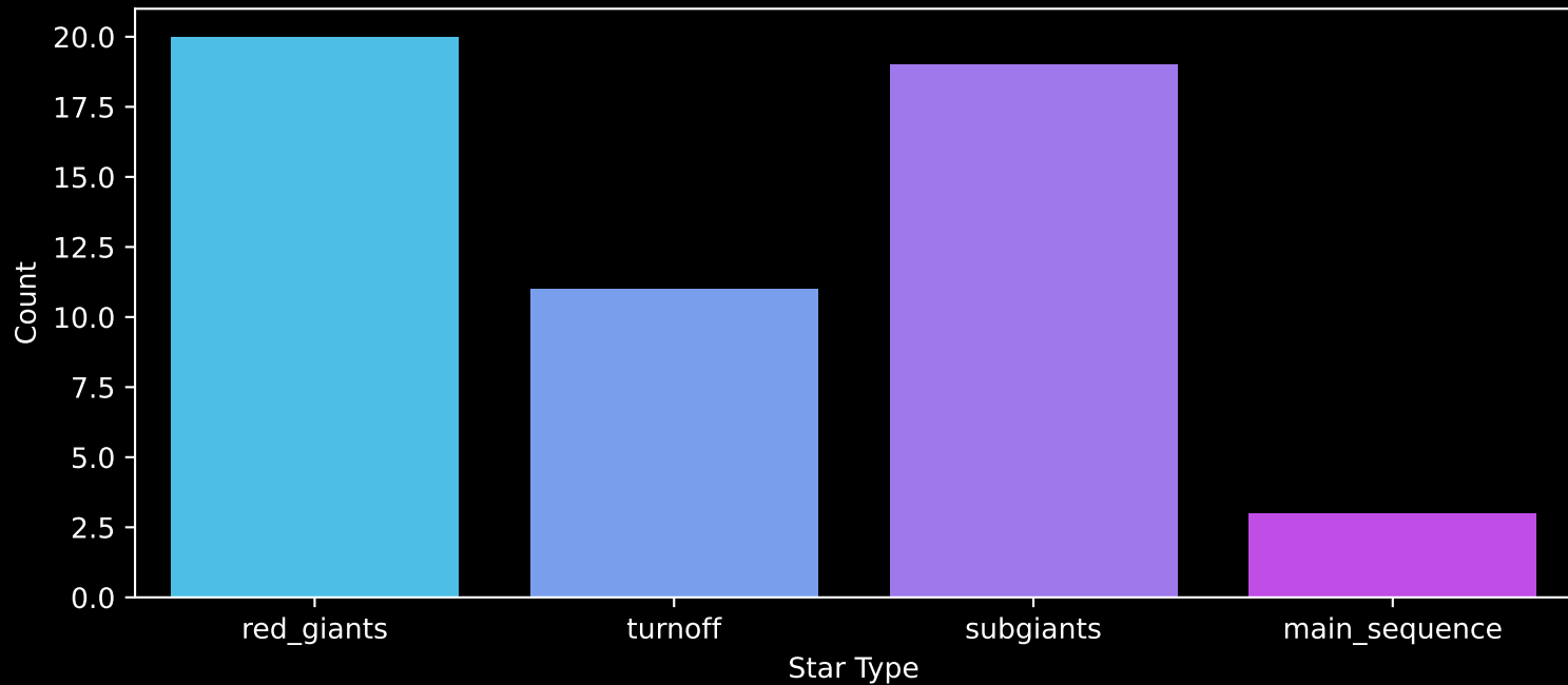
Gaia Cluster: [FSR_0158] Count plot of Star Type
