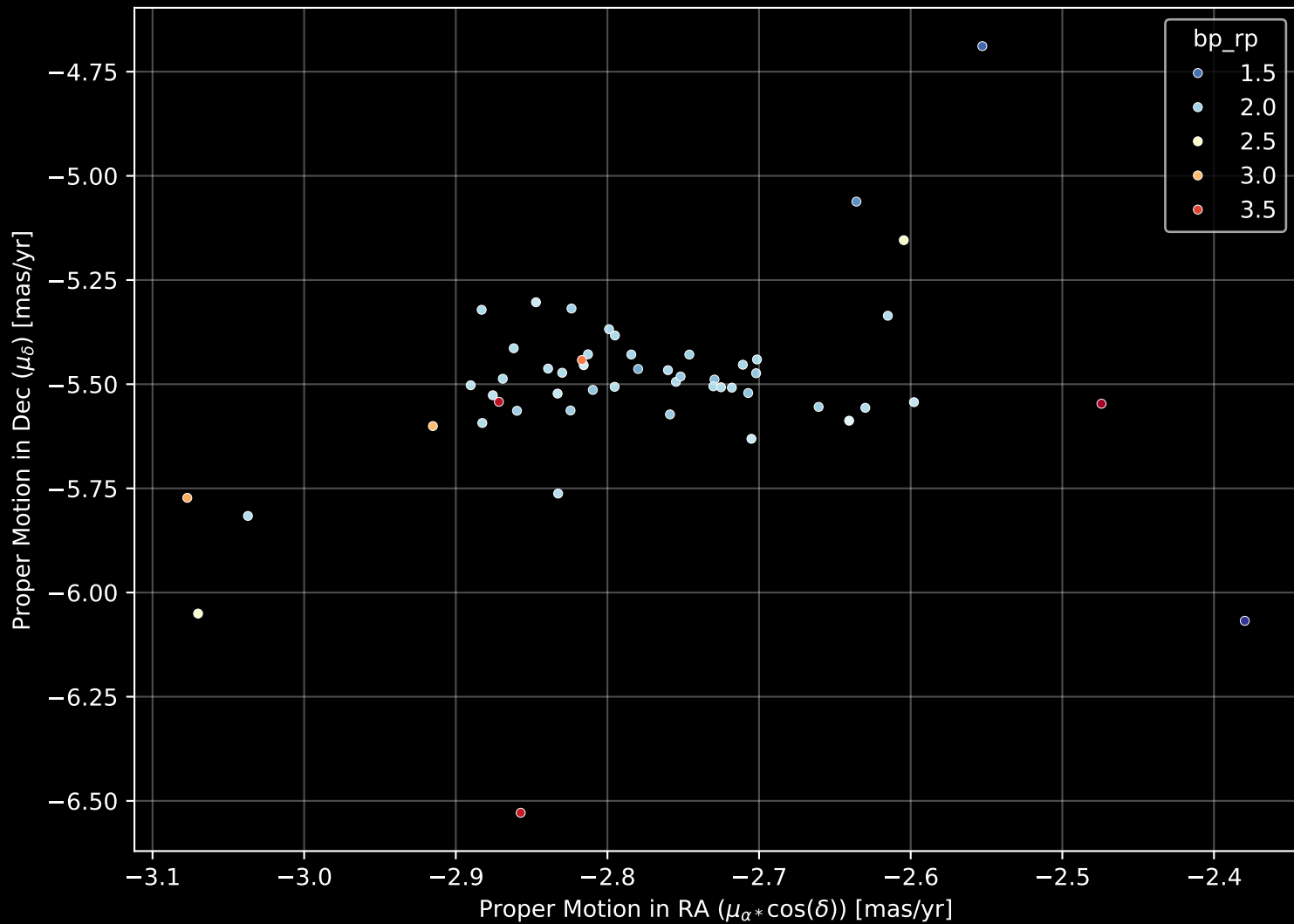
Gaia Cluster: [FSR_0158] Proper Motion Diagram (n= 53)
