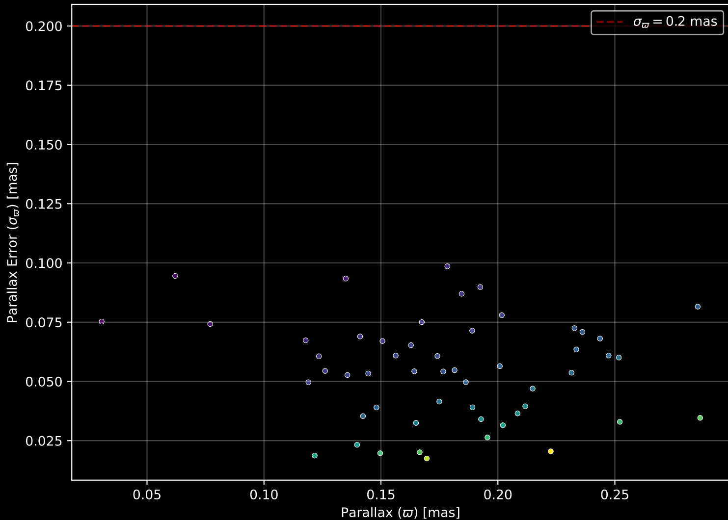
Gaia Cluster: [FSR_0158] Parallax Quality (n= 53)
