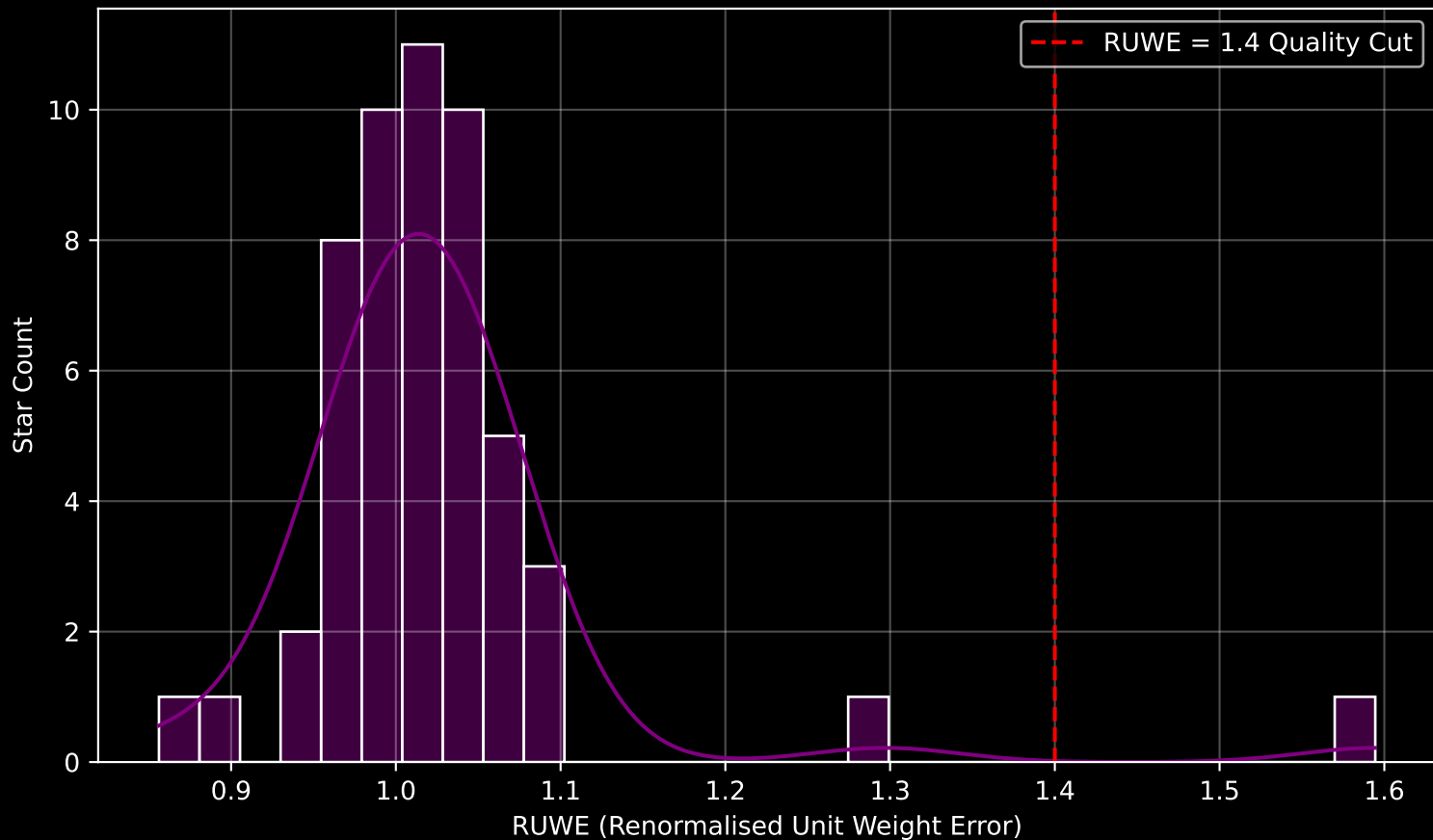
Gaia Cluster: [FSR_0158] RUWE Distribution (n= 53)
