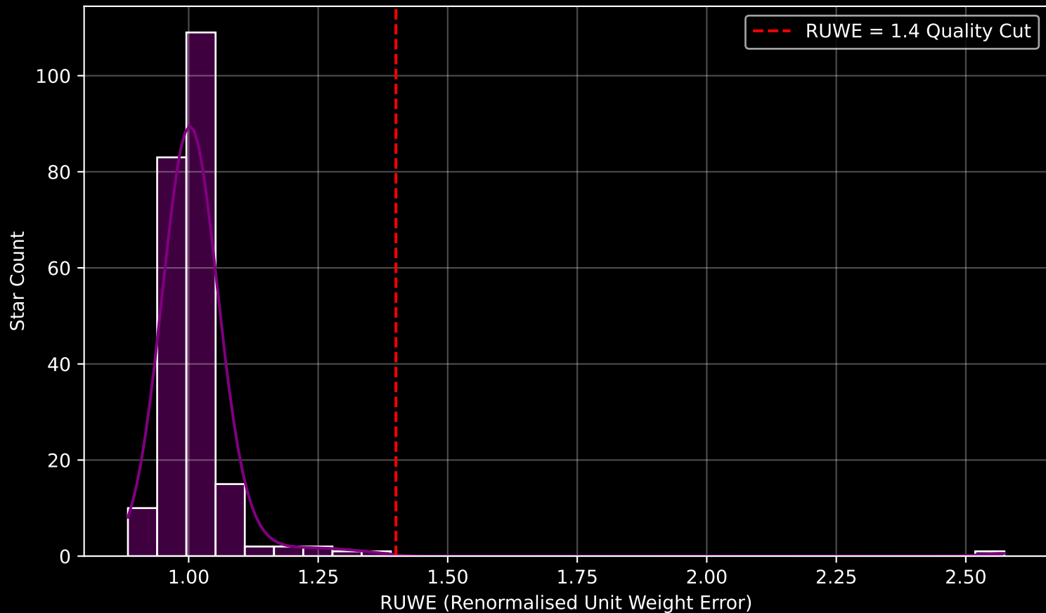
Gaia Cluster: [FSR_0165] RUWE Distribution (n= 226)
