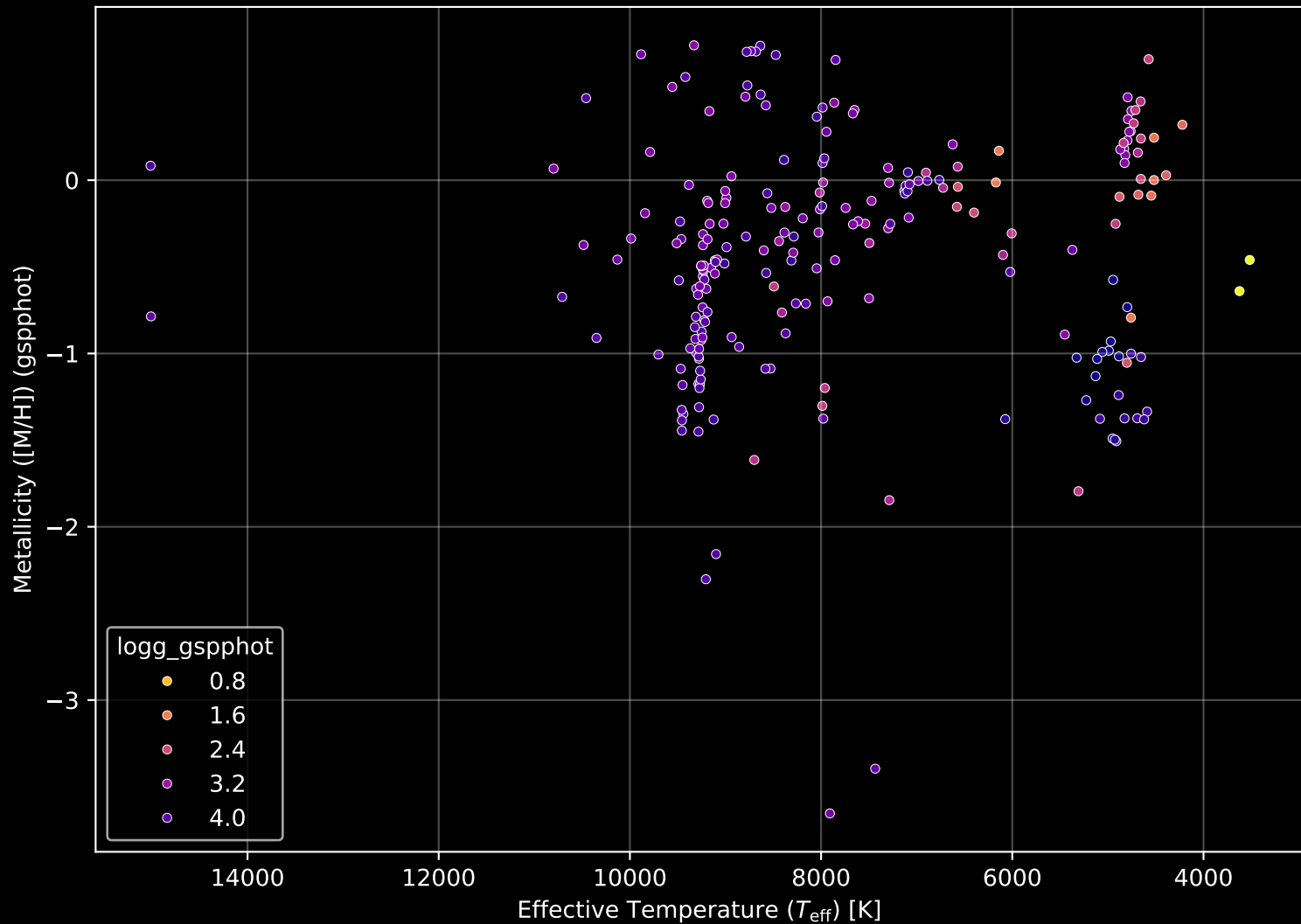
Gaia Cluster: [FSR_0165] Stellar Population Parameters (n= 226)
