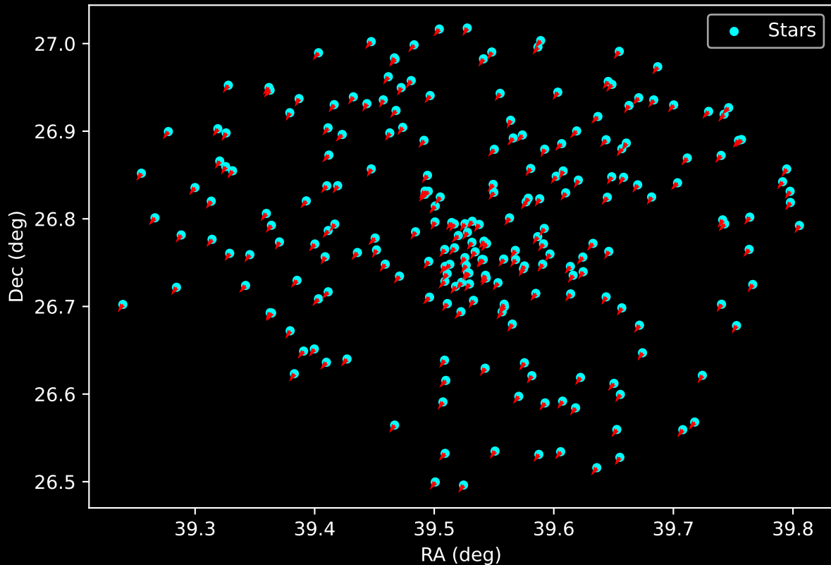
Gaia Cluster: [FSR_0165] Proper Motion Vectors for Gaia Star Field (n= 226)
