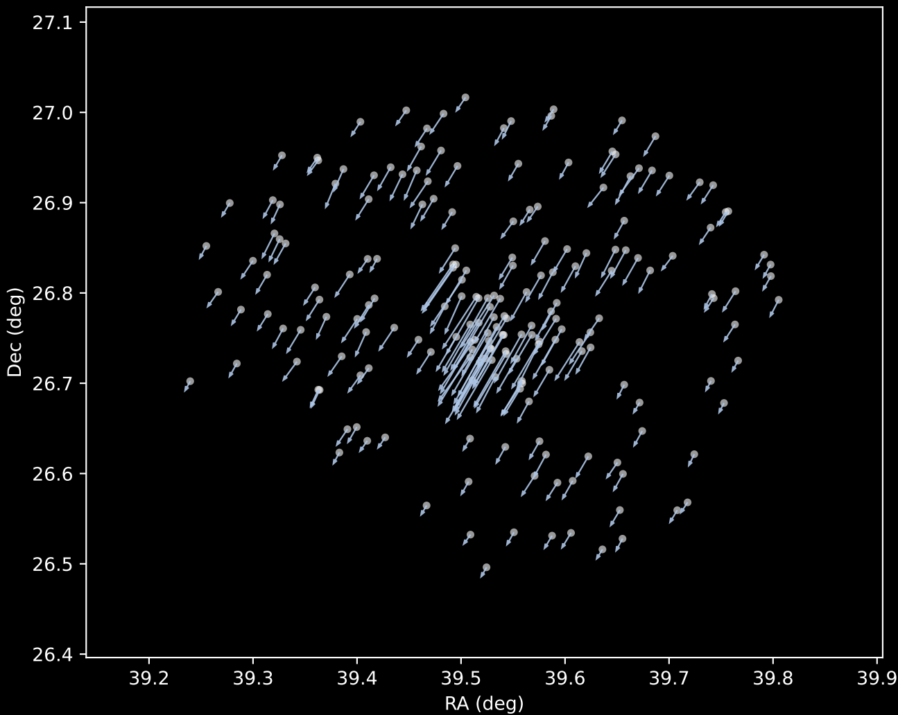
Gaia DR3 Cluster 1 Proper Motion Vectors (n=197)
