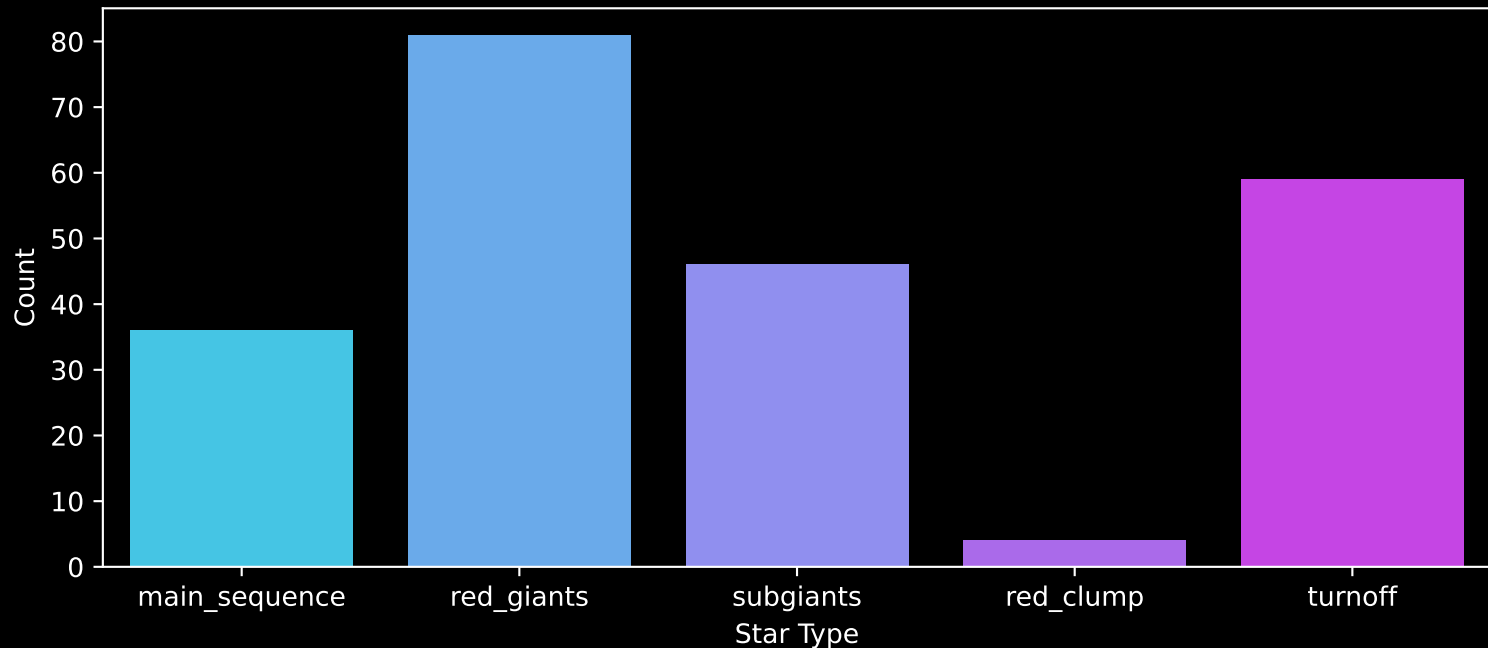
Gaia Cluster: [FSR_0165] Count plot of Star Type
