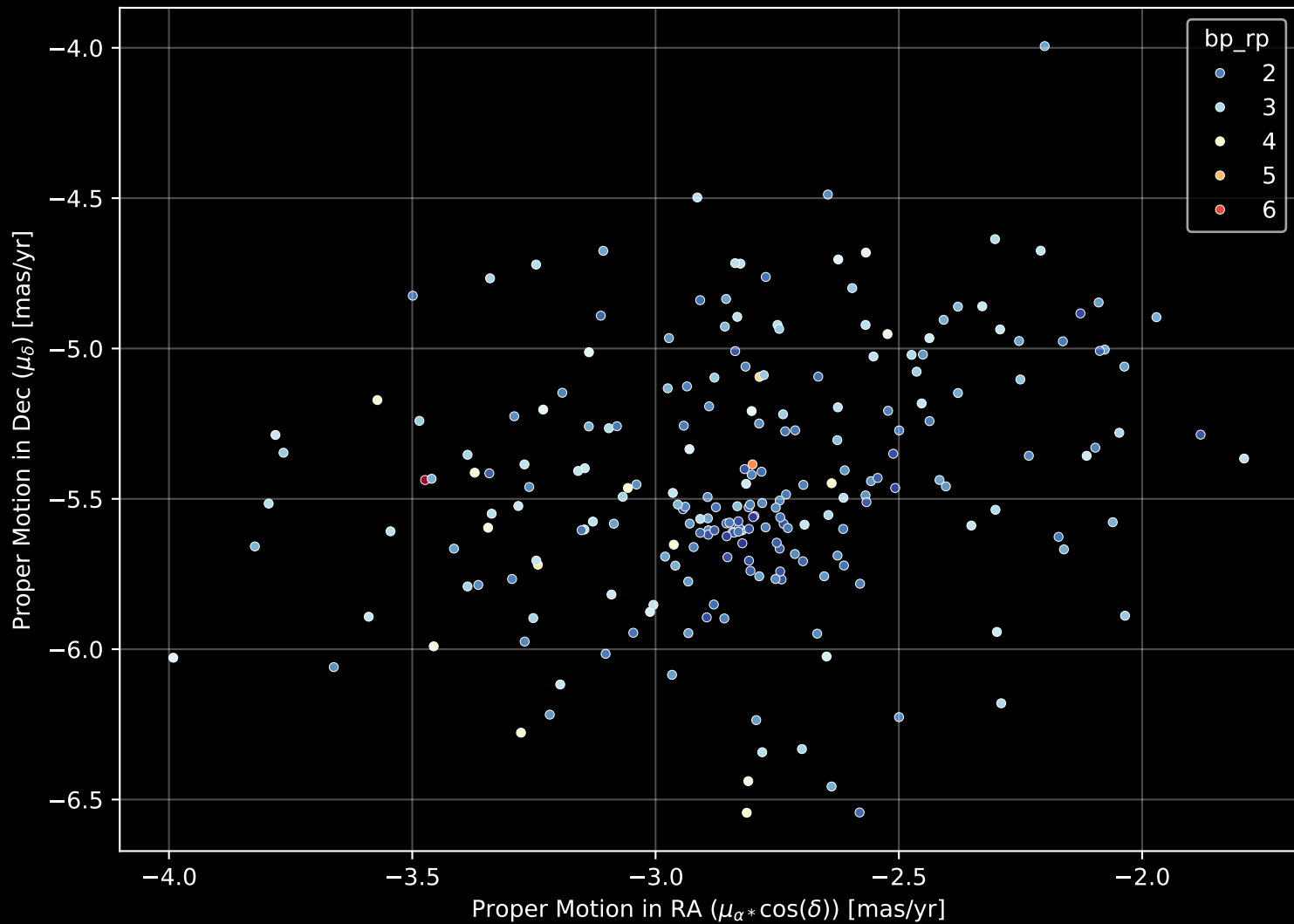
Gaia Cluster: [FSR_0165] Proper Motion Diagram (n= 226)
