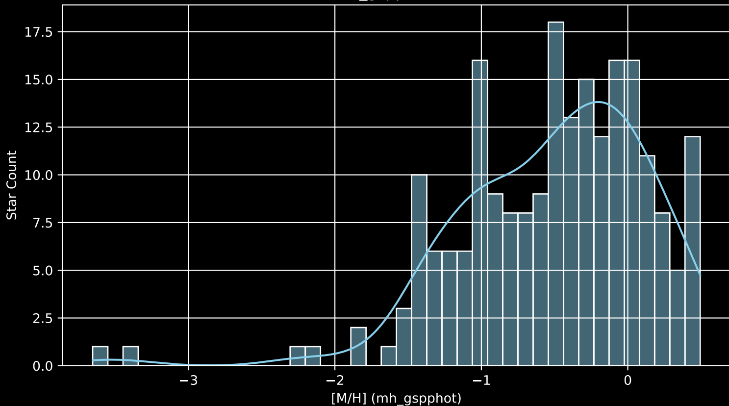
Gaia Cluster: [FSR_0165 [M/H] (mh_gspphot) (n= 214)
