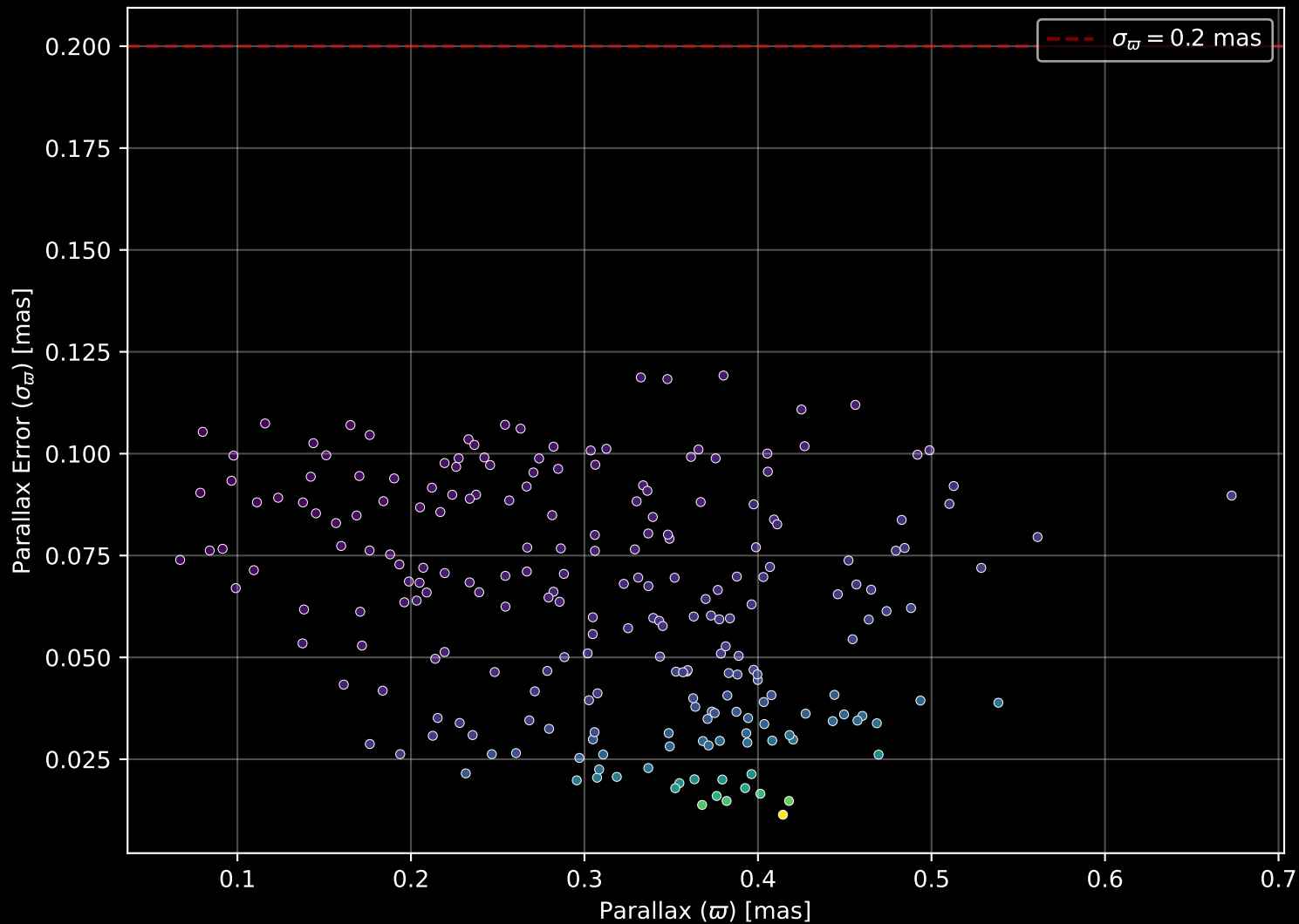
Gaia Cluster: [FSR_0165] Parallax Quality (n= 226)
