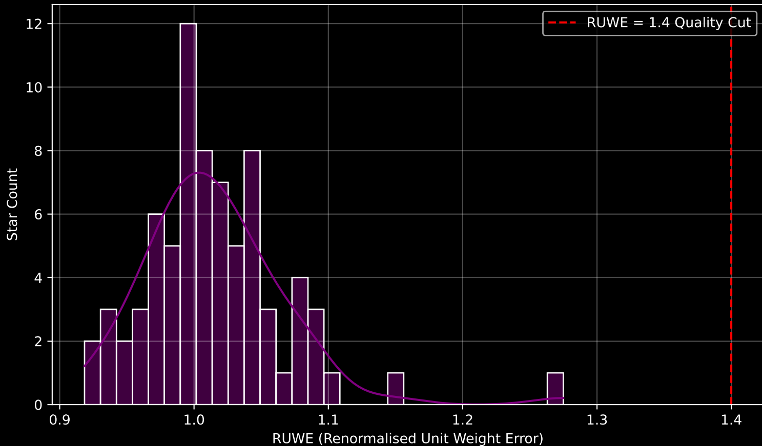
Gaia Cluster: [FSR_0172] RUWE Distribution (n= 75)
