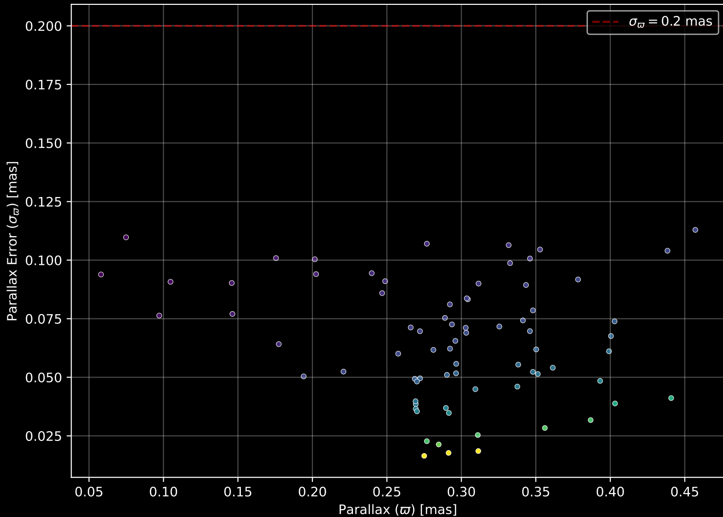
Gaia Cluster: [FSR_0172] Parallax Quality (n= 75)
