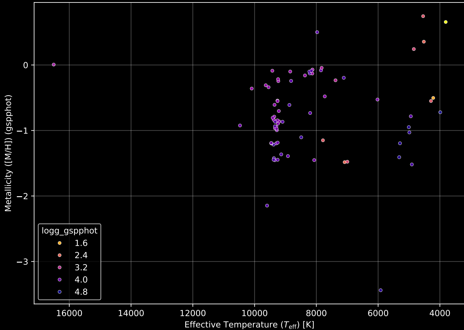
Gaia Cluster: [FSR_0172] Stellar Population Parameters (n= 75)
