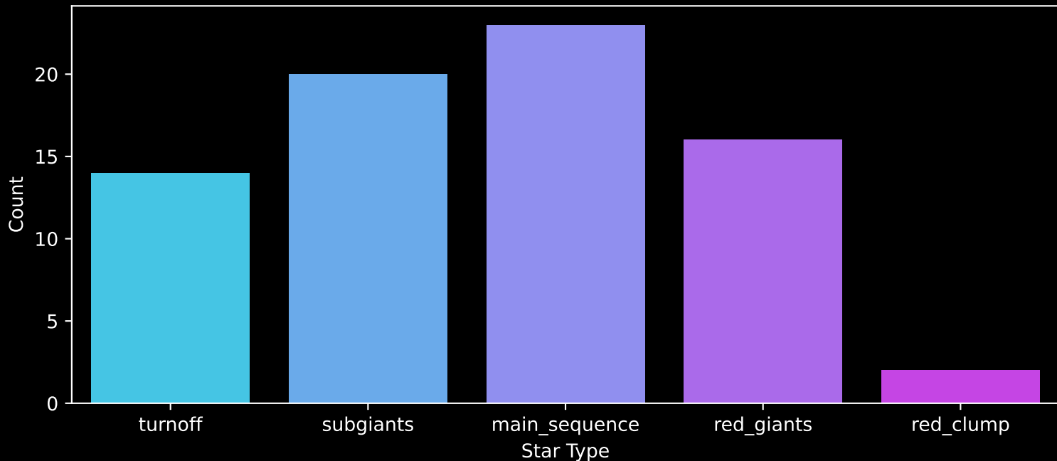
Gaia Cluster: [FSR_0172] Count plot of Star Type
