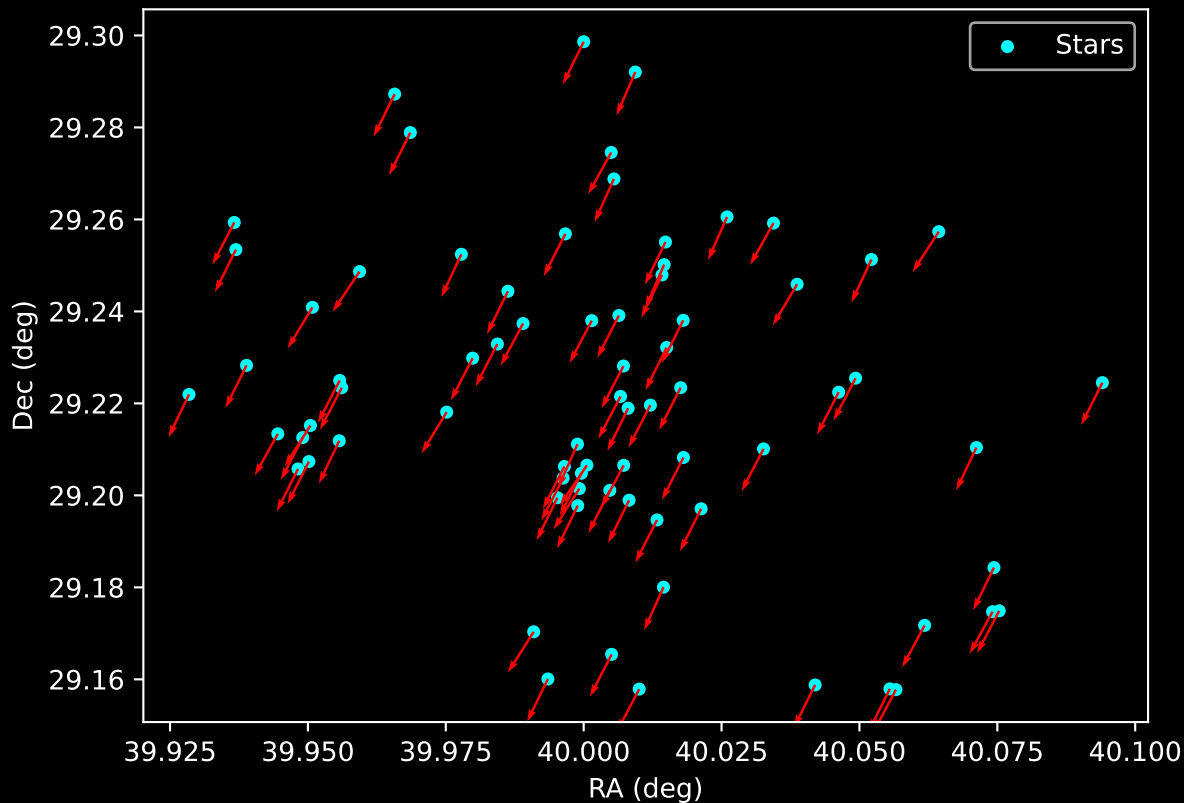
Gaia Cluster: [FSR_0172] Proper Motion Vectors for Gaia Star Field (n= 75)
