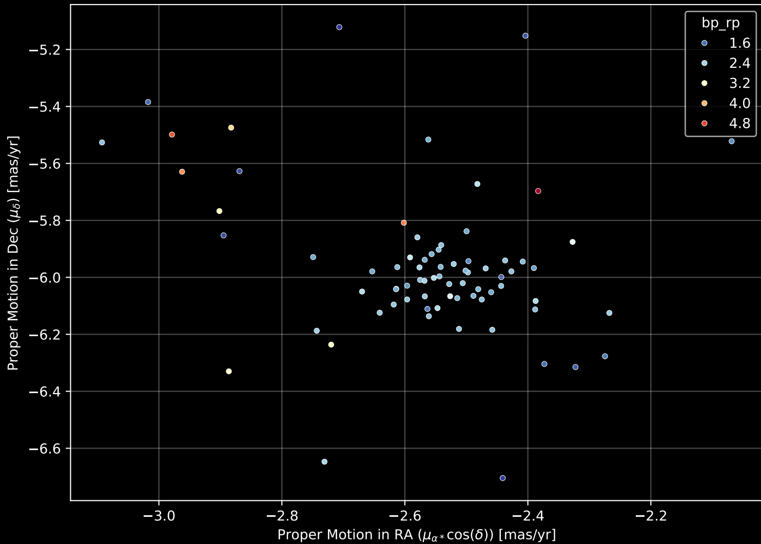
Gaia Cluster: [FSR_0172] Proper Motion Diagram (n= 75)
