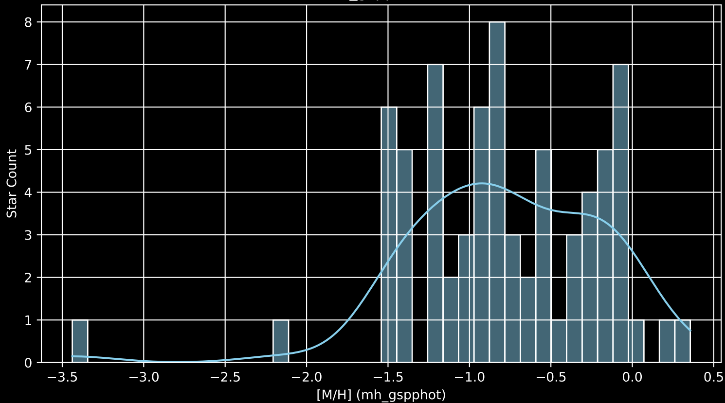
Gaia Cluster: [FSR_0172 [M/H] (mh_gspphot) (n= 72)
