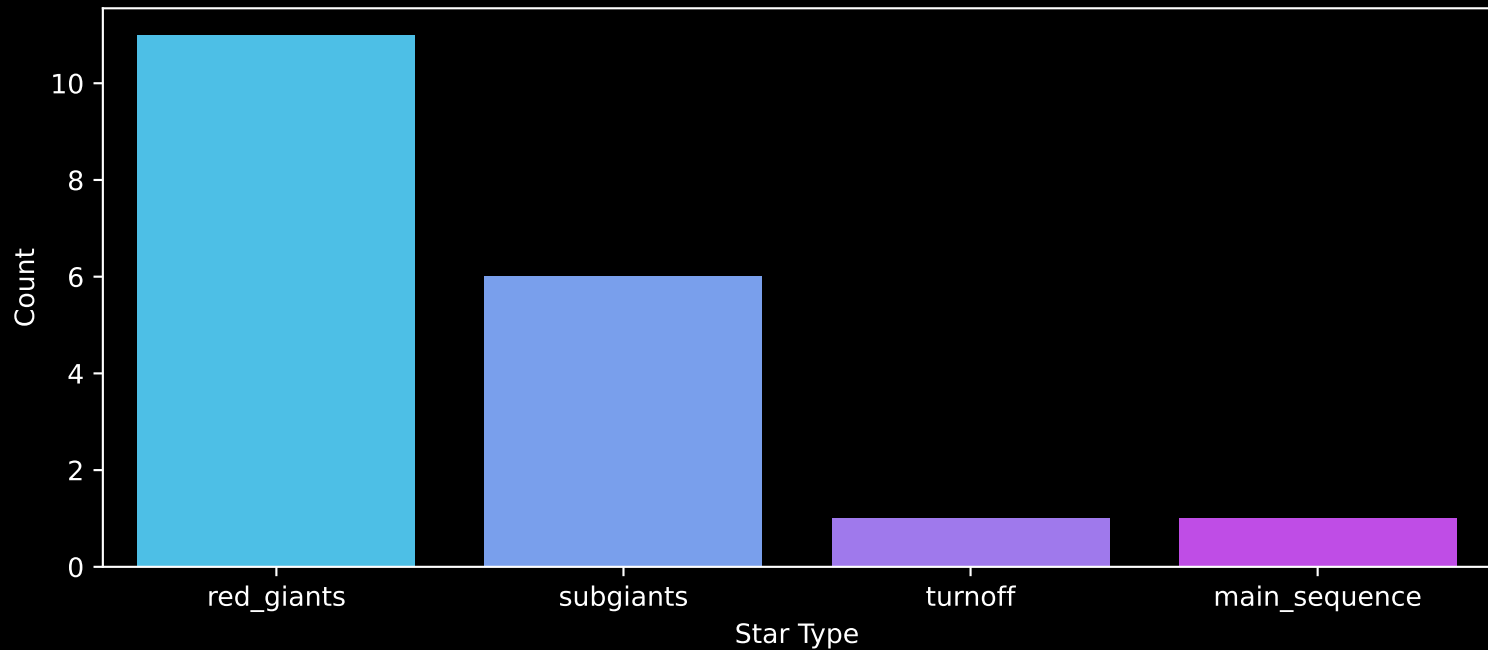
Gaia Cluster: [FSR_0238] Count plot of Star Type
