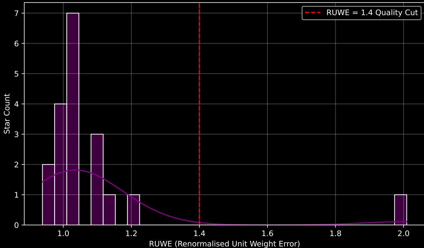
Gaia Cluster: [FSR_0238] RUWE Distribution (n= 19)
