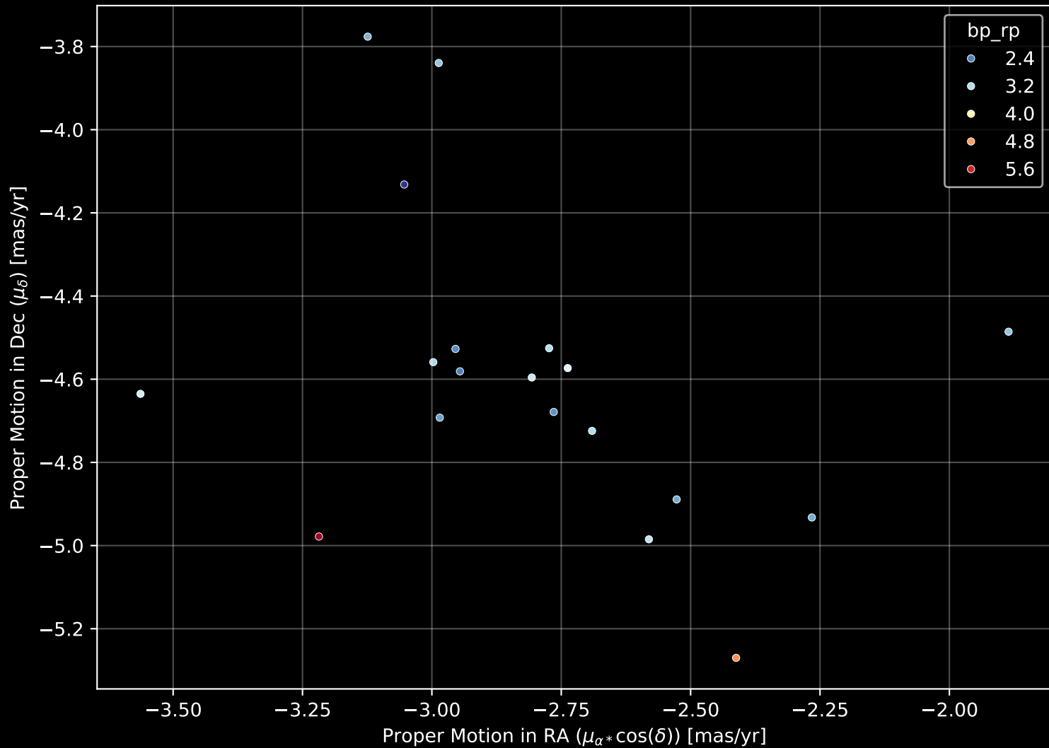
Gaia Cluster: [FSR_0238] Proper Motion Diagram (n= 19)
