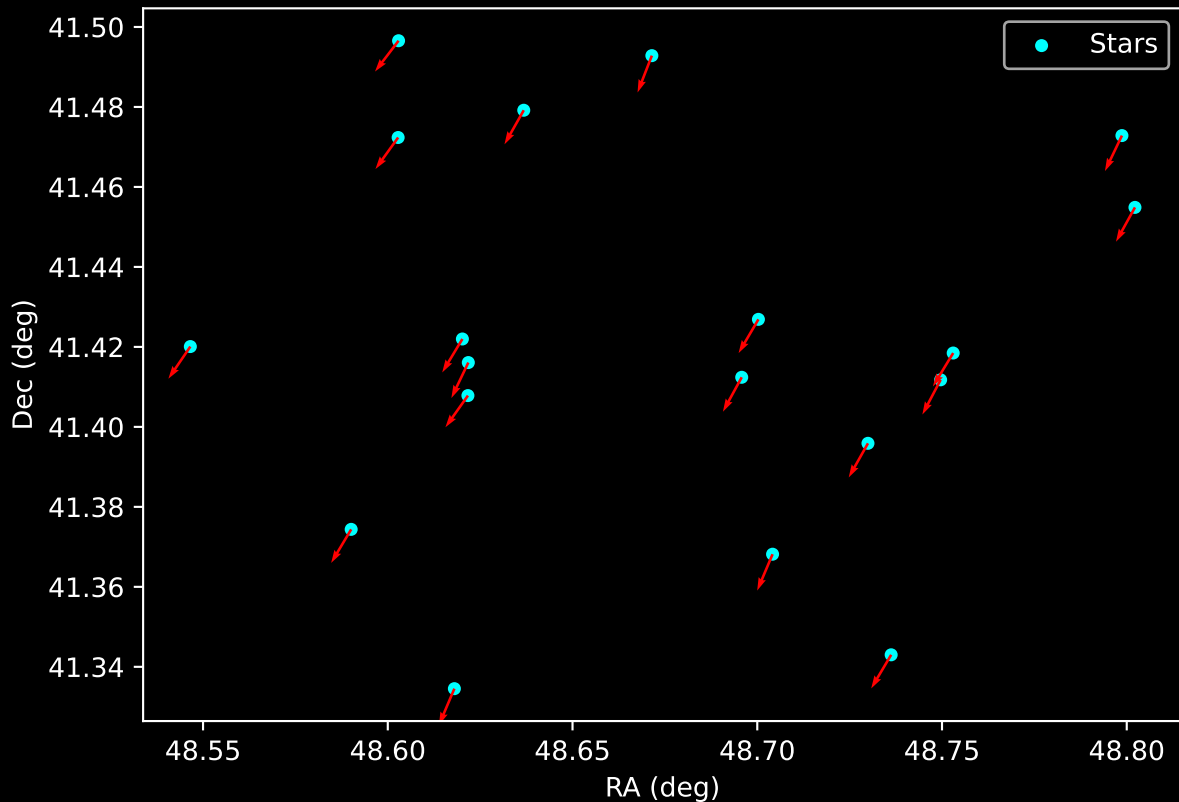
Gaia Cluster: [FSR_0238] Proper Motion Vectors for Gaia Star Field (n= 19)
