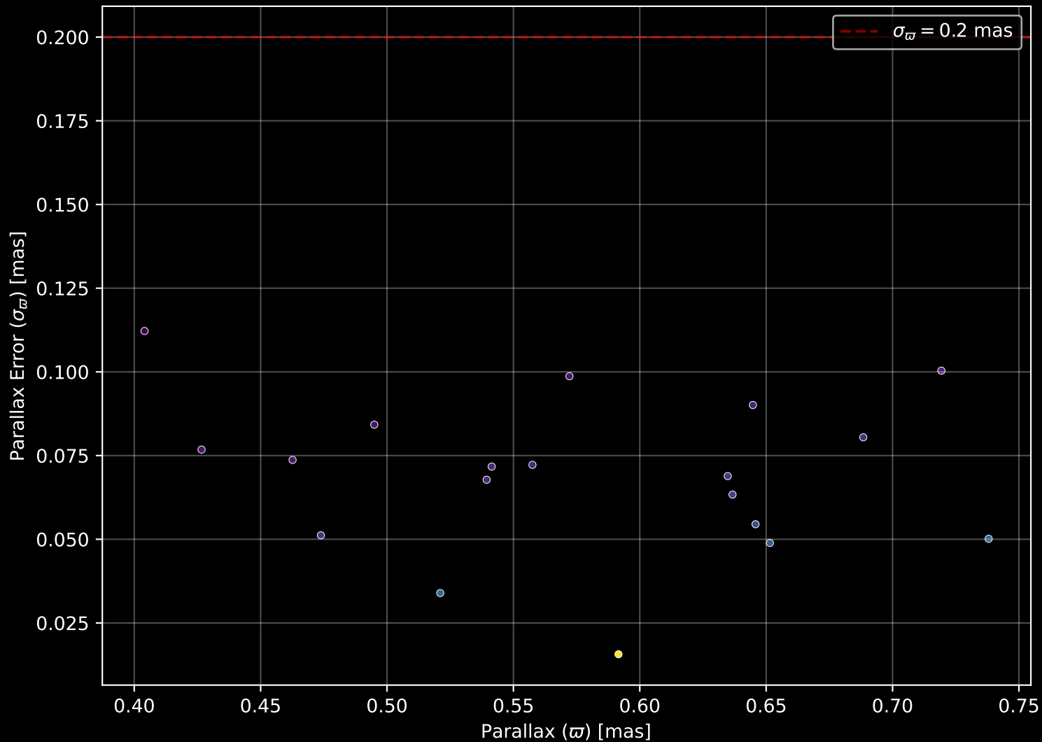
Gaia Cluster: [FSR_0238] Parallax Quality (n= 19)
