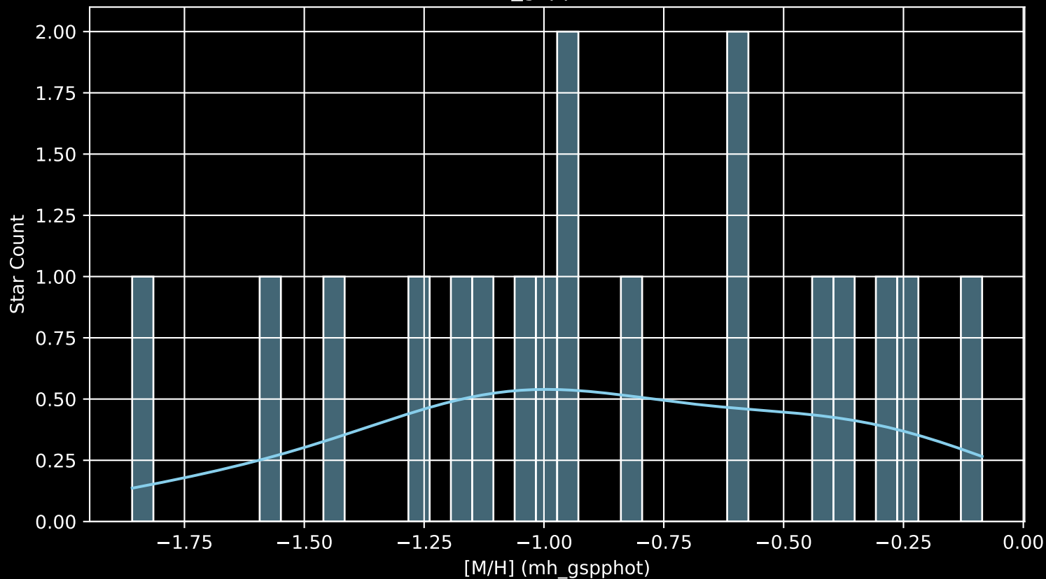
Gaia Cluster: [FSR_0238 [M/H] (mh_gspphot) (n= 18)
