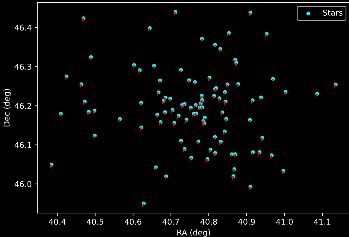
Gaia Cluster: [FSR_0241] Proper Motion Vectors for Gaia Star Field (n= 96)
