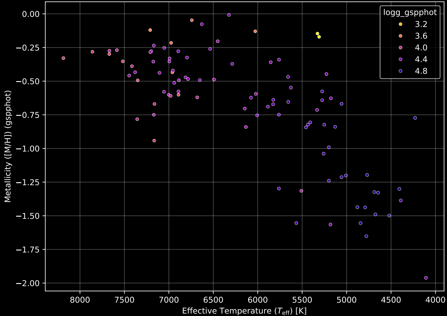
Gaia Cluster: [FSR_0241] Stellar Population Parameters (n= 96)
