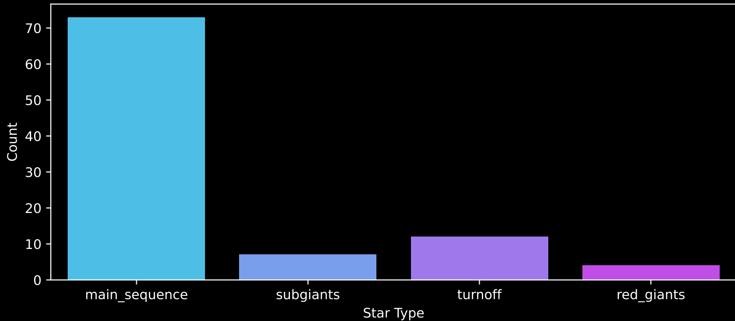
Gaia Cluster: [FSR_0241] Count plot of Star Type
