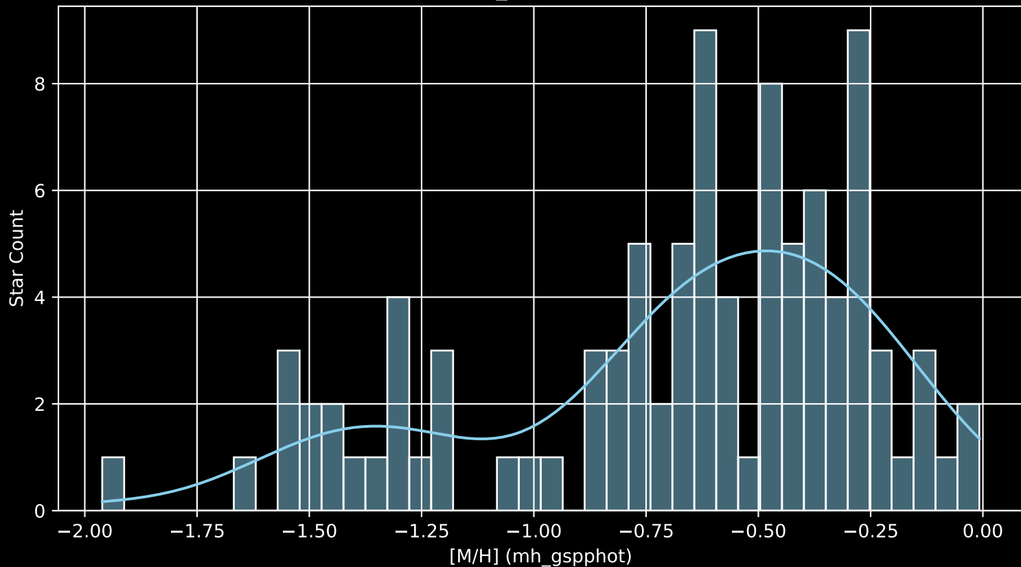
Gaia Cluster: [FSR_0241 [M/H] (mh_gspphot) (n= 96)
