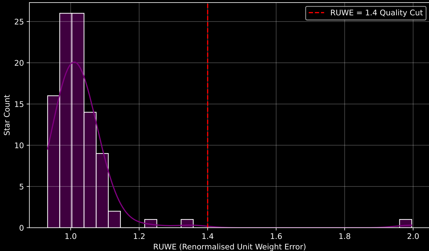
Gaia Cluster: [FSR_0241] RUWE Distribution (n= 96)
