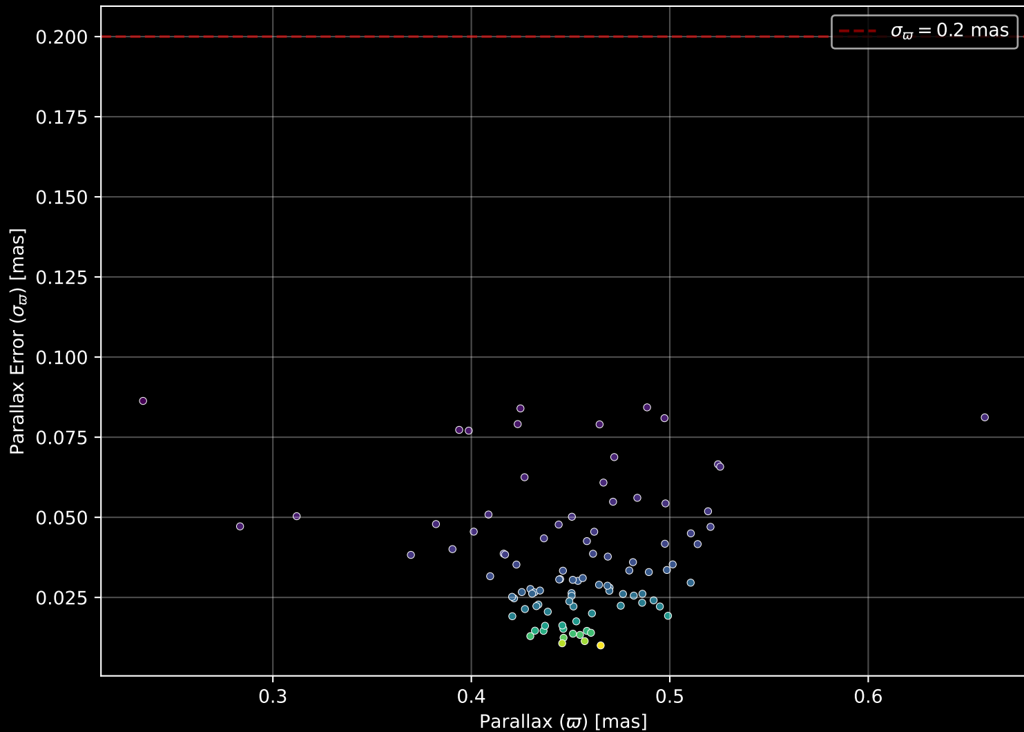
Gaia Cluster: [FSR_0241] Parallax Quality (n= 96)
